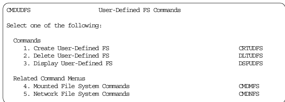
Figure 51. CMDUDFS menu
