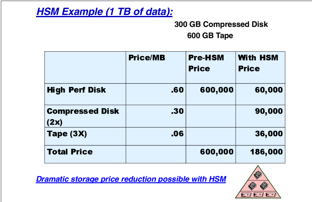
Figure 25. Savings example with HSM and DASD compression
