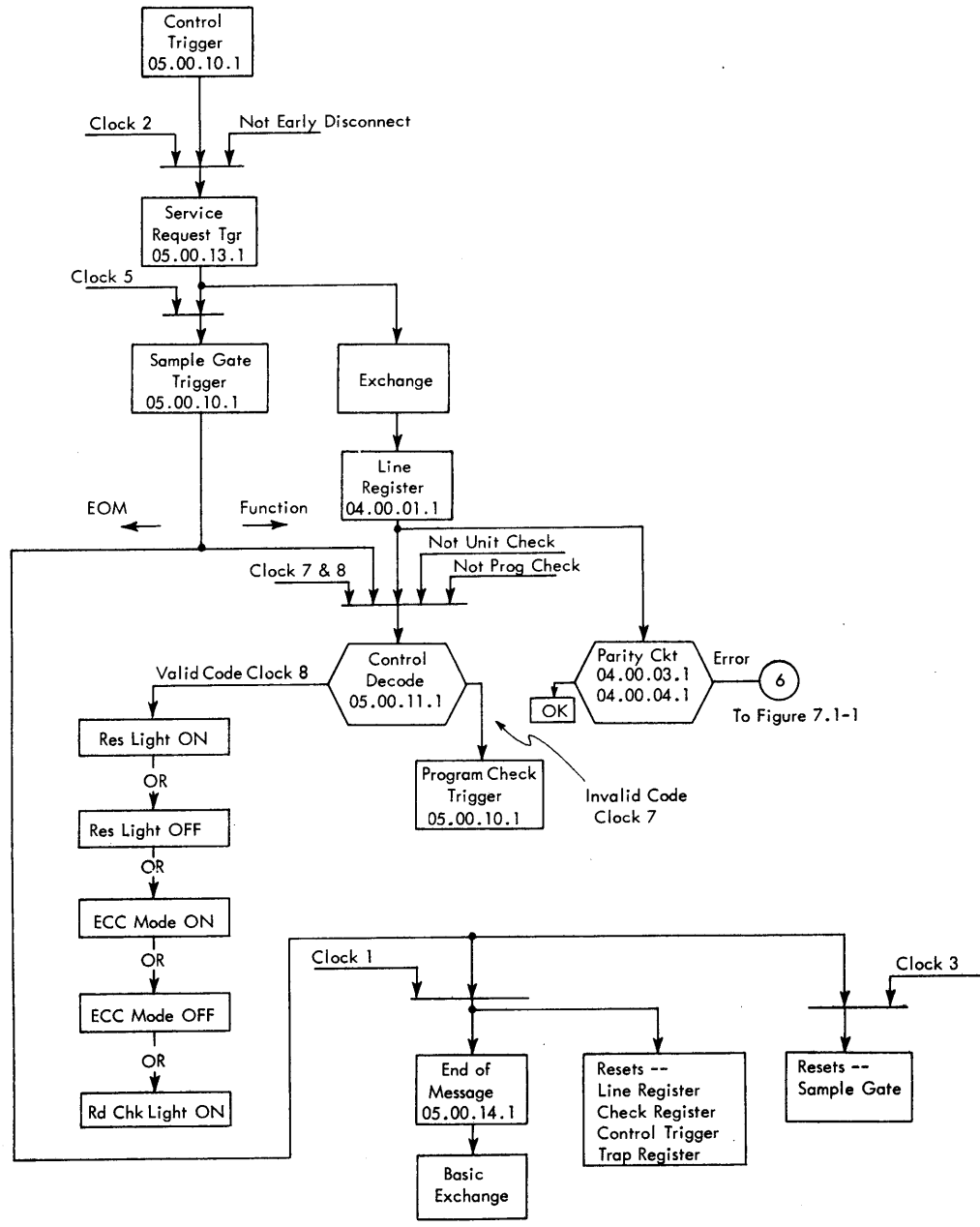
FIGURE 6.4-2. CARD READER, CONTROL FUNCTION
