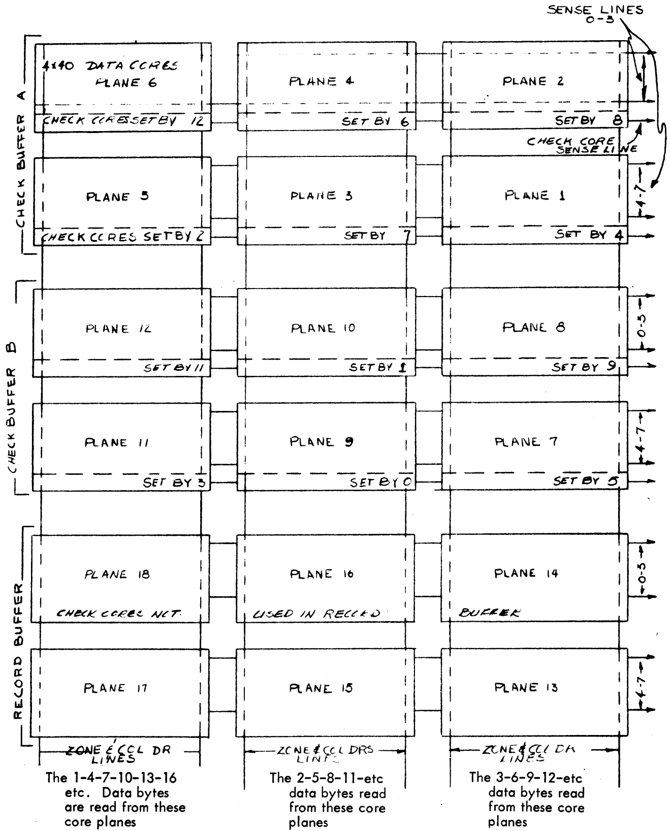
FIGURE 5.1-4. READ-OUT CONFIGURATION OF BUFFERS
