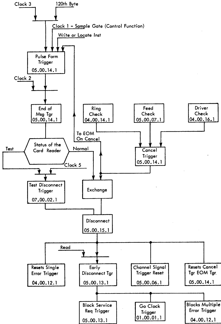
FIGURE 6.8-1. CARD READER, DISCONNECT
