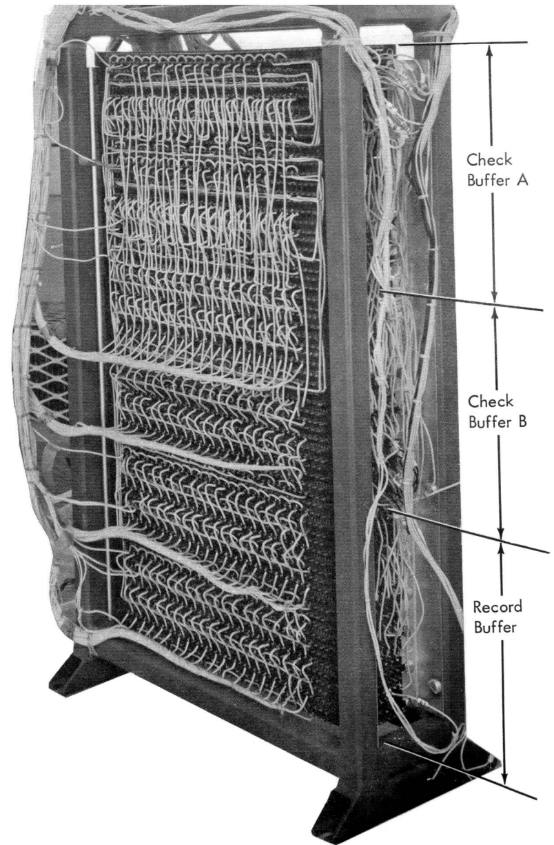
FIGURE 5.1-2. CORE ARRAY
