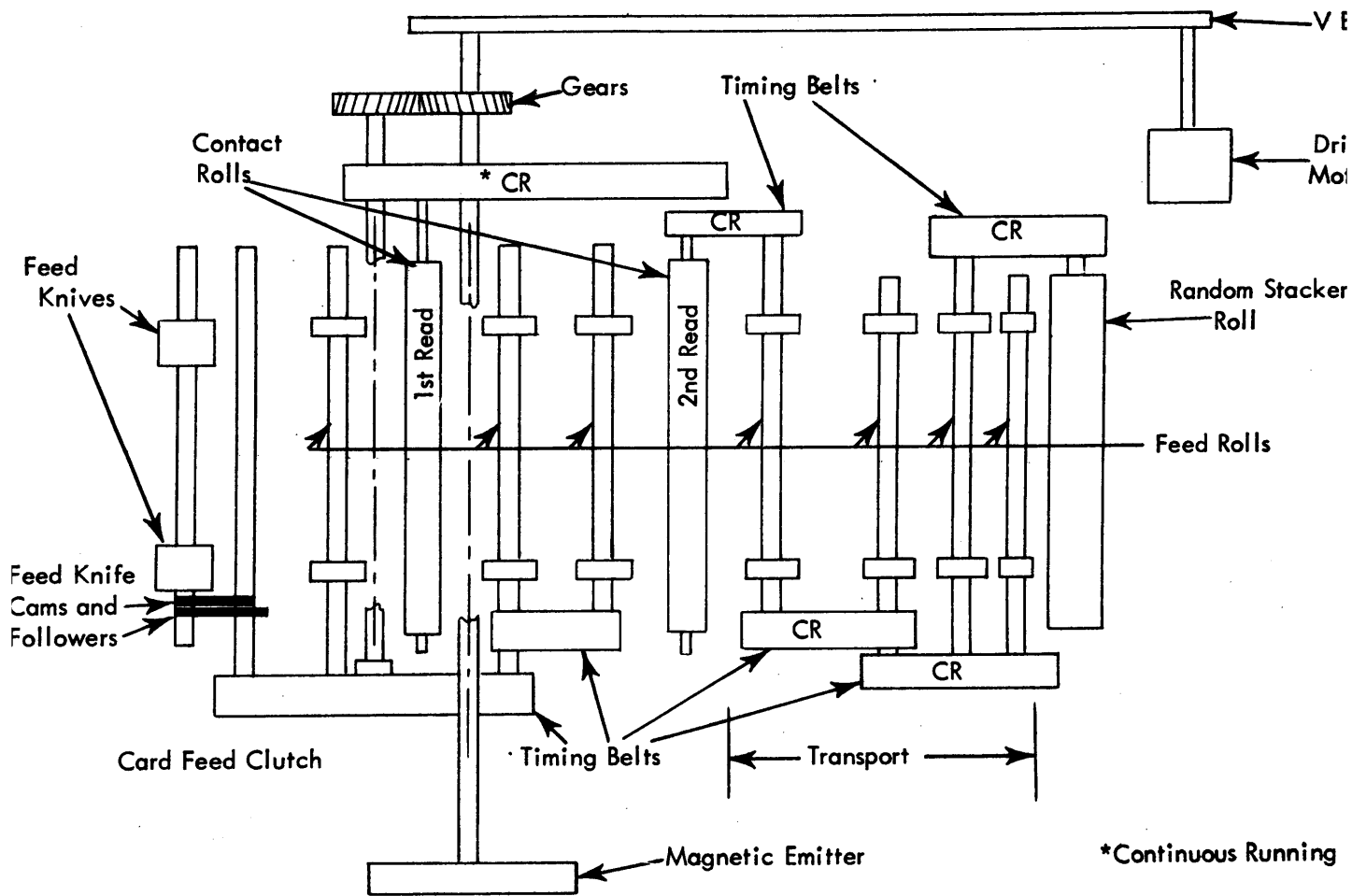
FIGURE 2.1-1. CARD FEED MECHANISM, SIMPLIFIED SCHEMATIC
