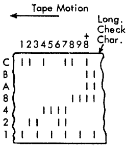
Figure 23. One-Word Tape Record with Longitudinal Check
