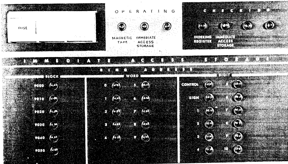
Figure 35. IBM 653 Console Display Lights
