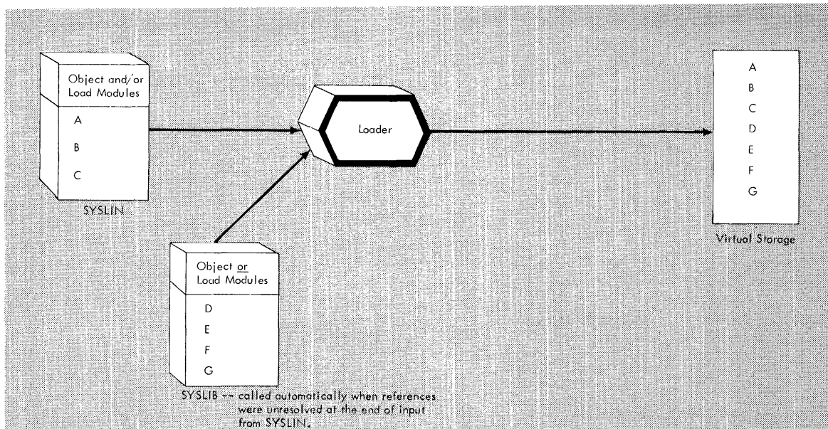
Figure 49. Loader Processing -- SYSLIB Resolution
