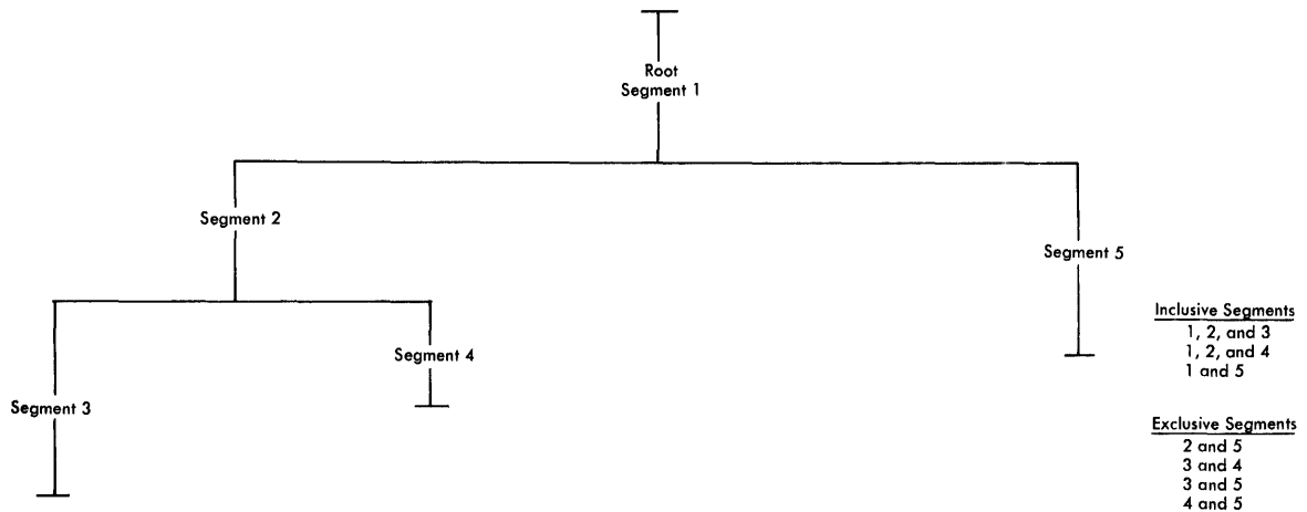
Figure 26. Inclusive and Exclusive Segments
