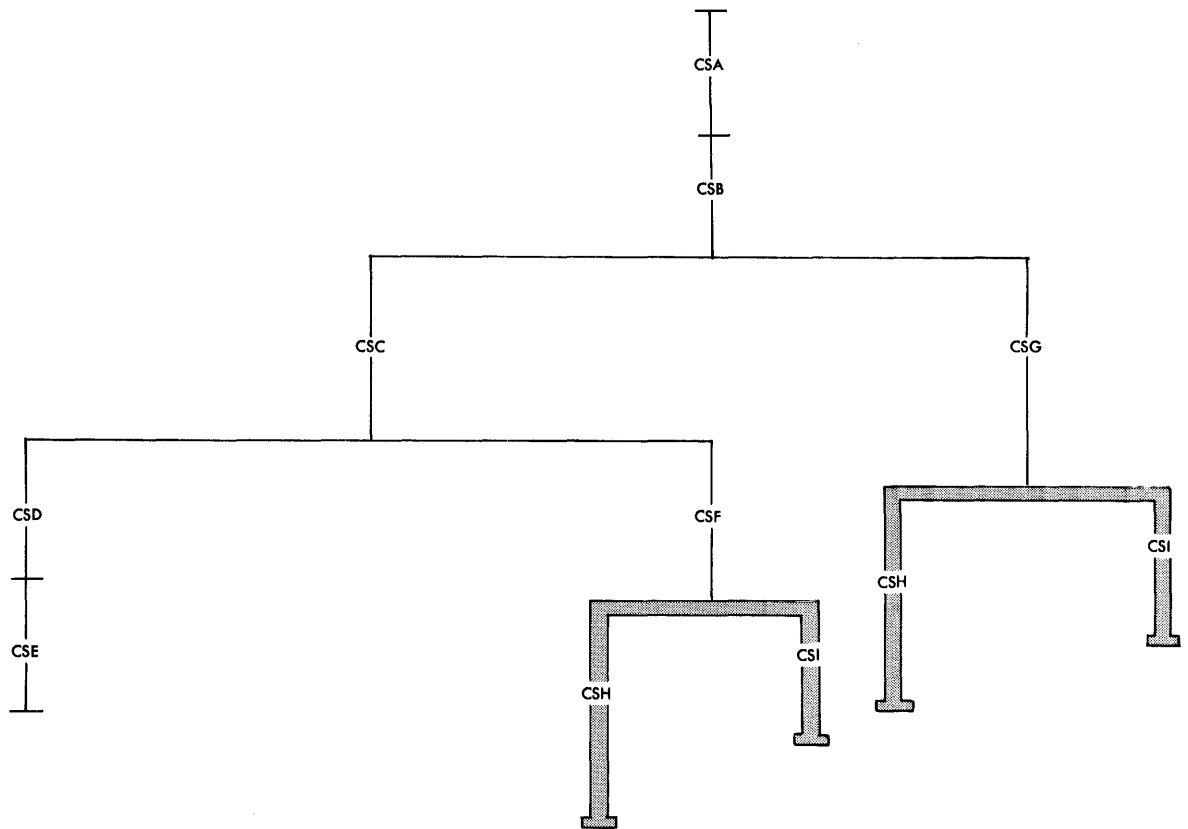
Figure 29. Control Sections Used by Several Paths
