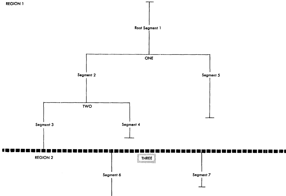
Figure 32. Symbolic Segment and Region Origin in Multiple-Region Program
