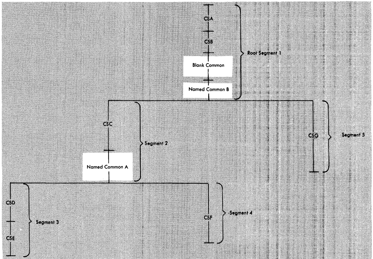
Figure 34. Common Areas After Processing
