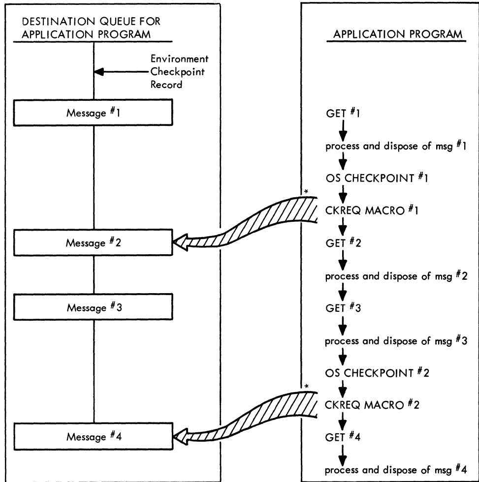
Figure 34. Example of Using the CKREQ Macro Instruction for Checkpoint Coordination
