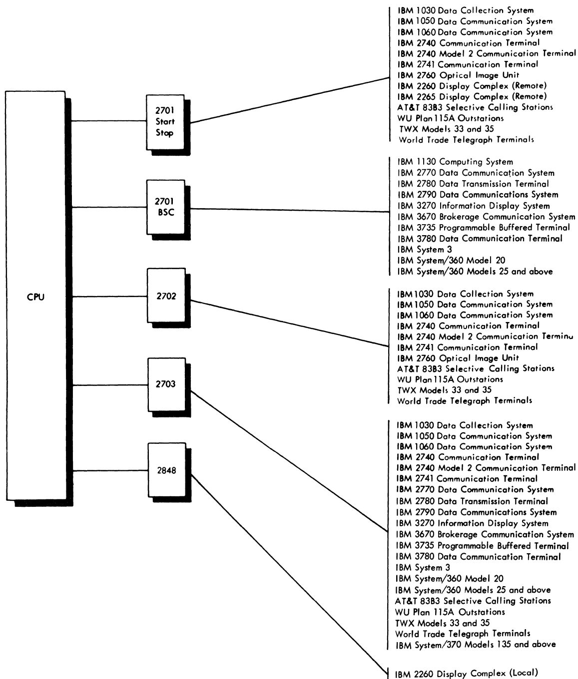
Figure 39. Device Configurations Supported by TCAM (Part 1 of 3)
