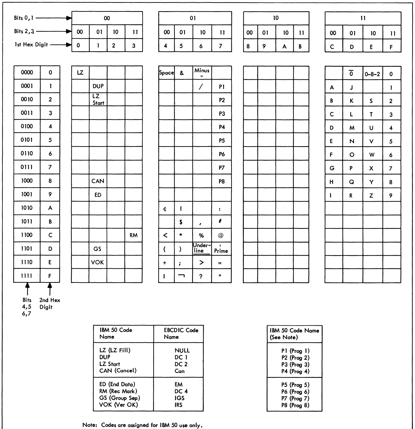
Figure 58. IBM 50 MDI Control Codes
