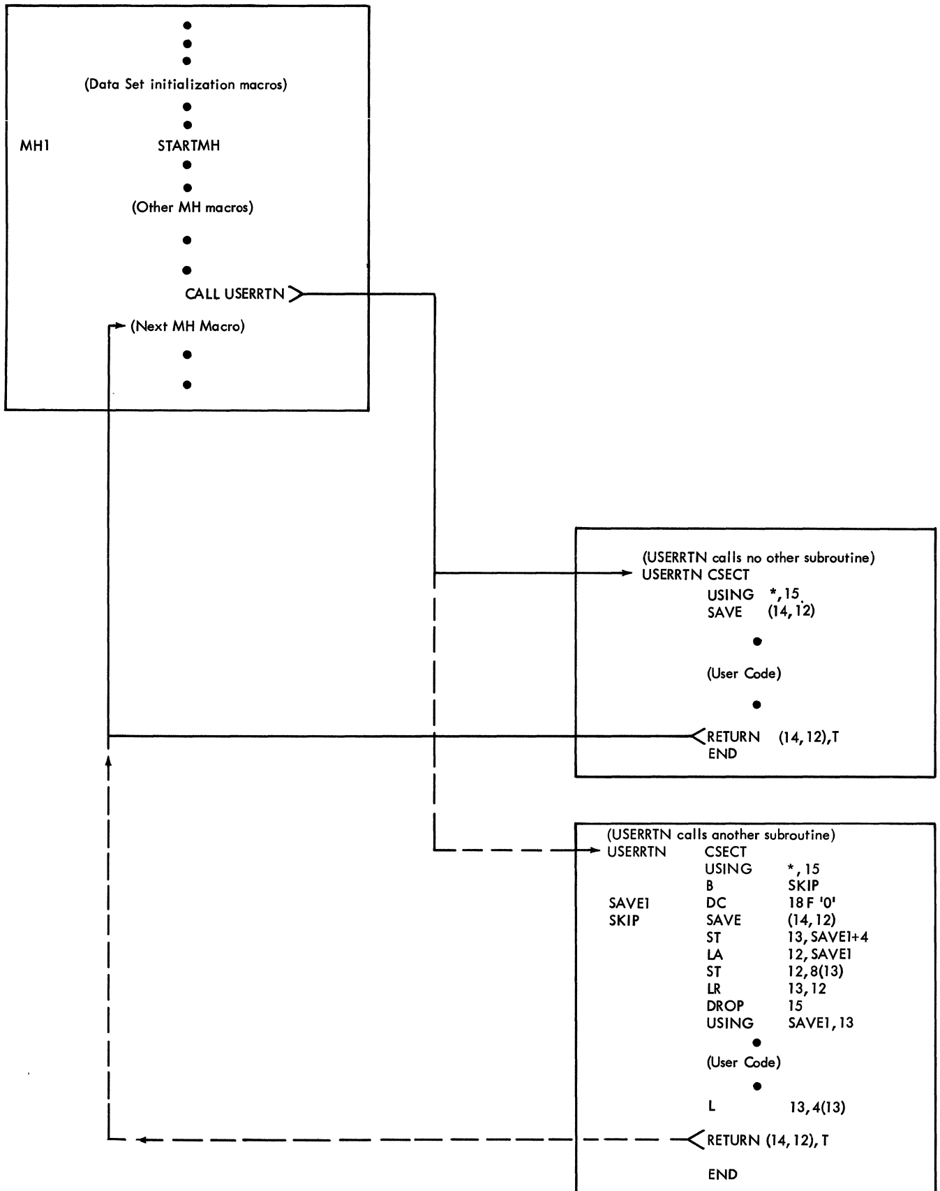
Figure 19. Activation of a Closed, User-Written Subroutine
