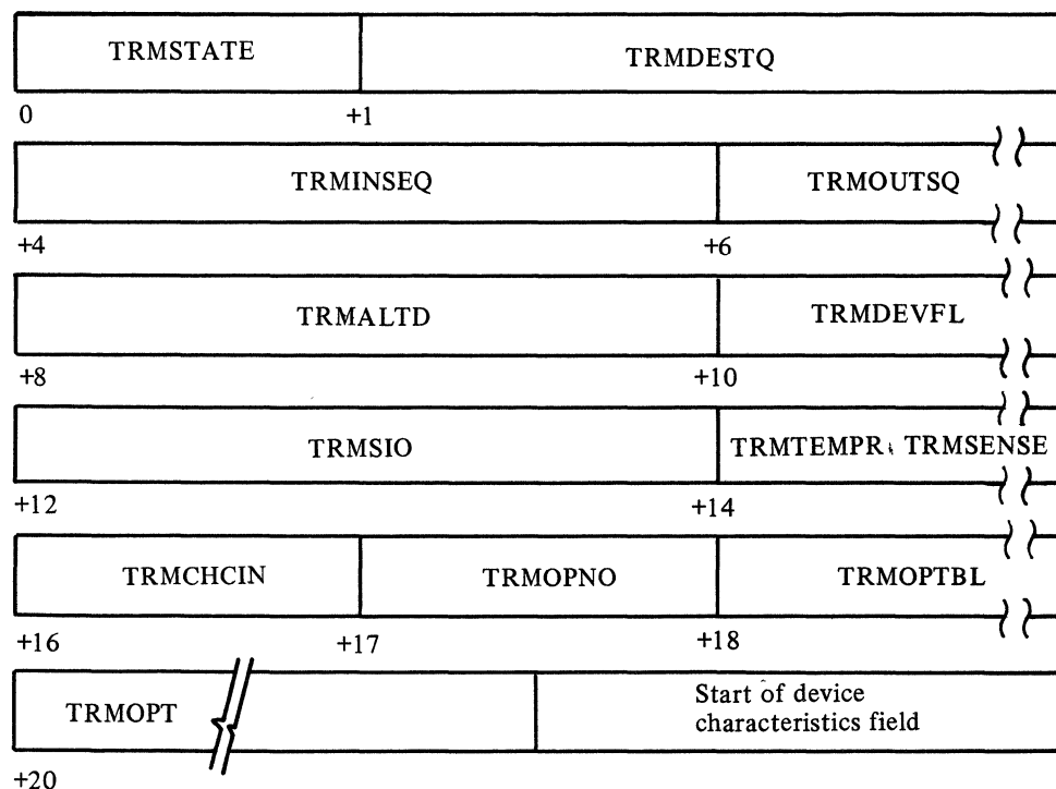
Figure 32. Terminal Table DSECT for Single, Line, and Group Entries
