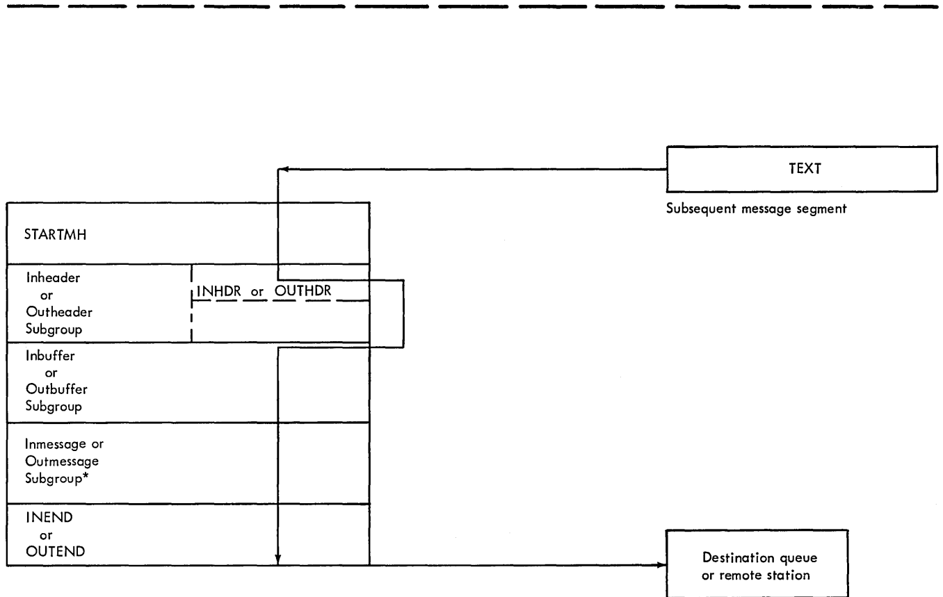
Figure 15. Flow of a Two-segment Message with a Single-buffer Header through an MH
