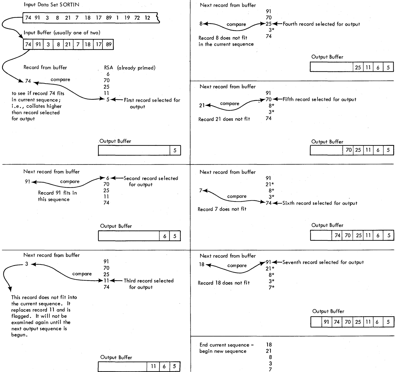
Figure 4. Replacement Selection Sorting Technique
