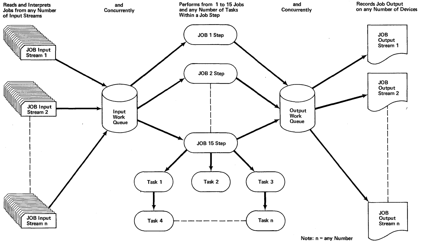
Figure 39. Concurrent Processing, by an MVT Control Program, of Job Steps, Job Support Tasks, and Tasks Within Job Steps
