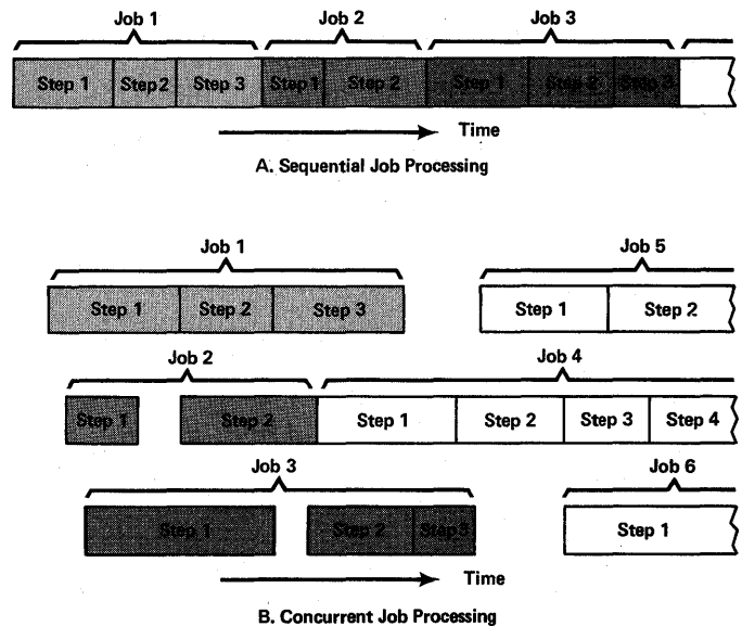
Figure 47. Sequential and Concurrent Job Processing
