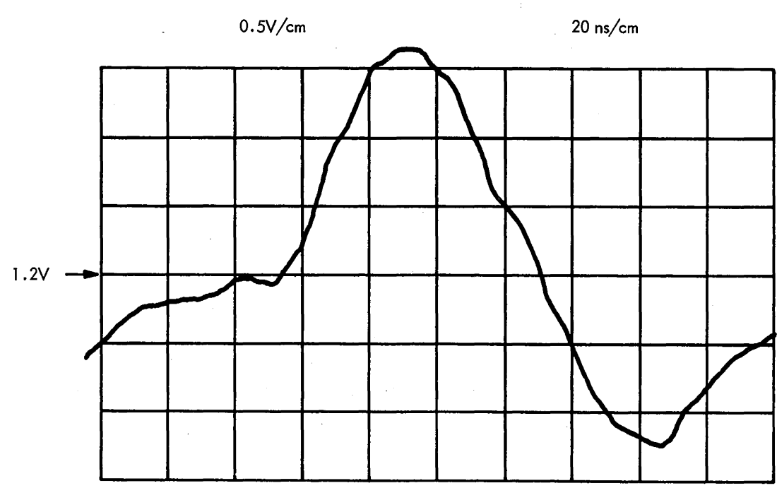
Figure 4-13. ROS Sense Amplifier, Average/Weak/Strong Waveshapes
