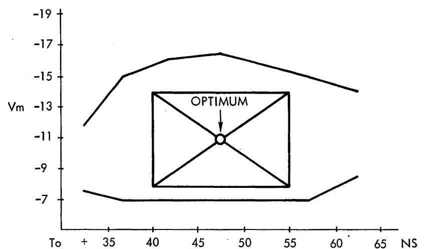
Figure 4-12. Acceptable Shmoo
