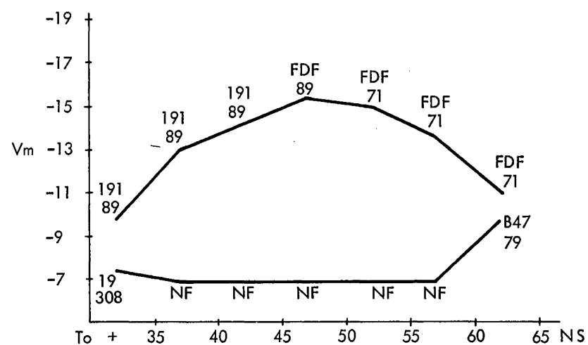
Figure 4-10. Typical Shmoo
