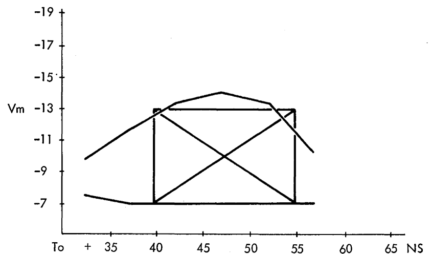
Figure 4-11. Unacceptable Shmoo
