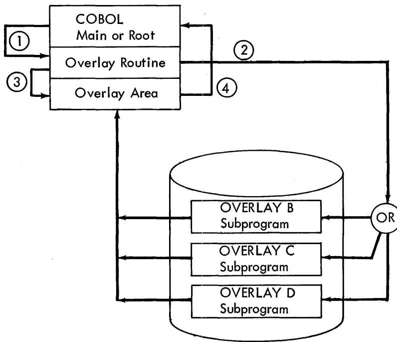
Figure 16. Flow Diagram of Overlay Logic
