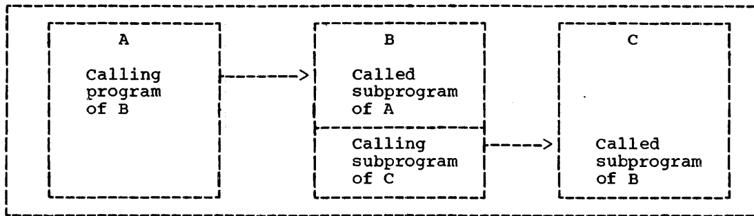
Figure 19. Called and Calling Programs
