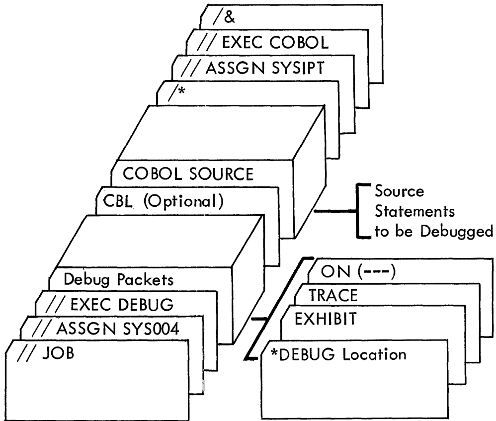
Figure 9. Example of a Debug Packet
