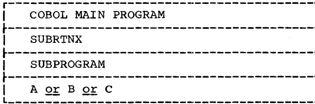
Figure 15. Storage Layout for Overlay Processing
