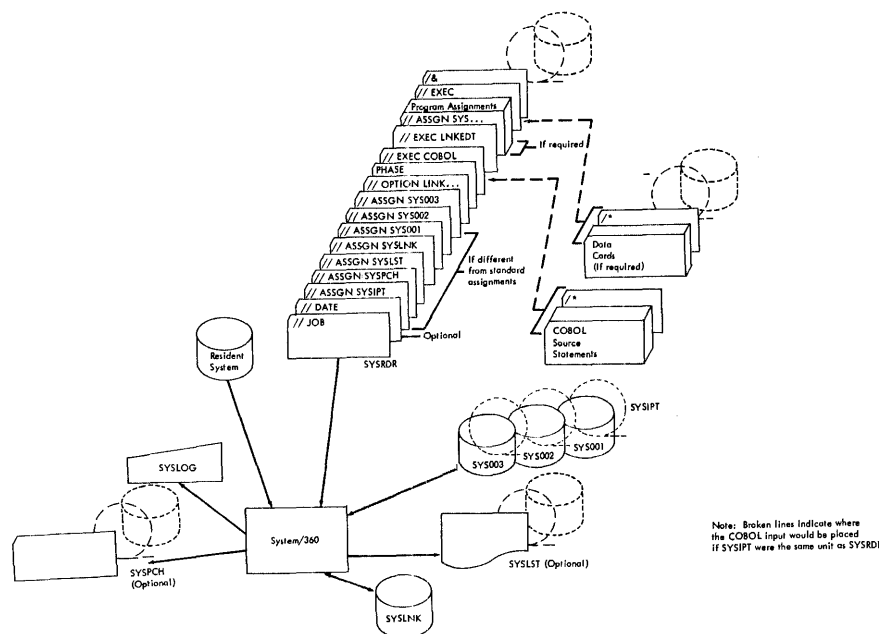
Figure 4. Input/Output Units Used by COBOL Program in a Disk System
