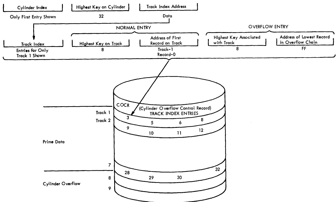
• Figure 17. Indexed Sequential File Without Overflow
