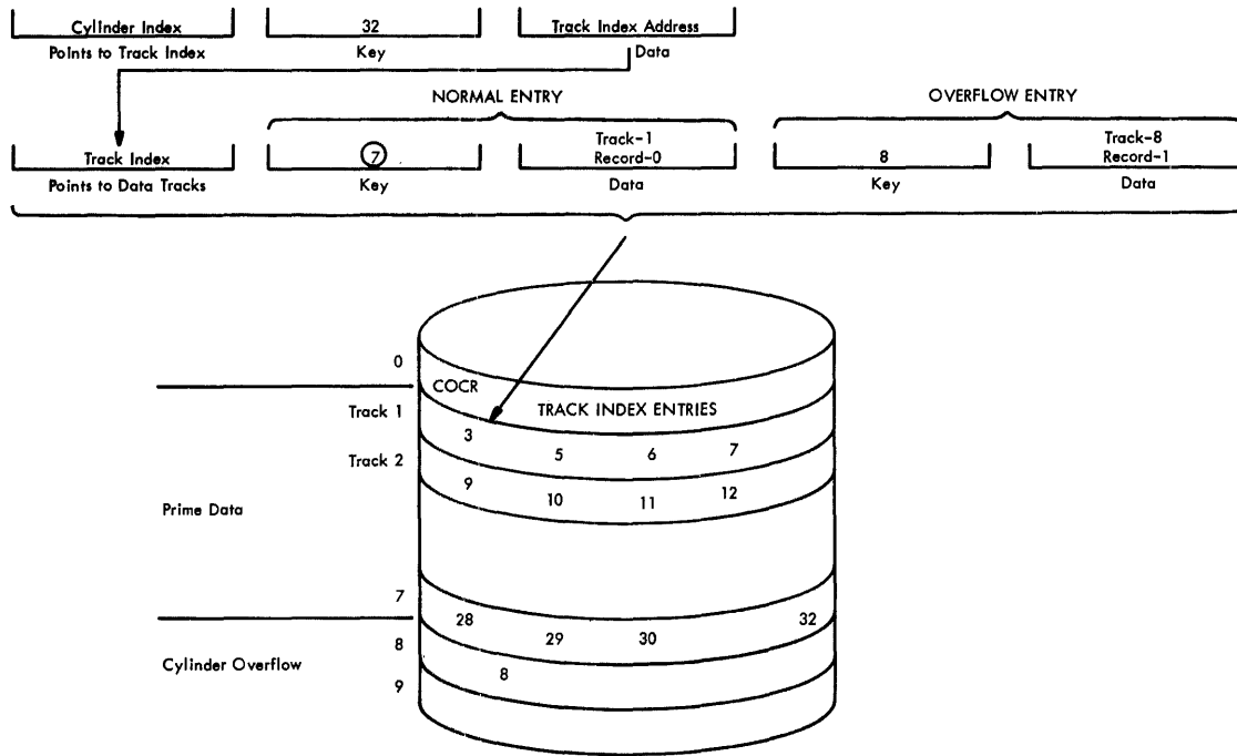
• Figure 18. Indexed Sequential File With Overflow
