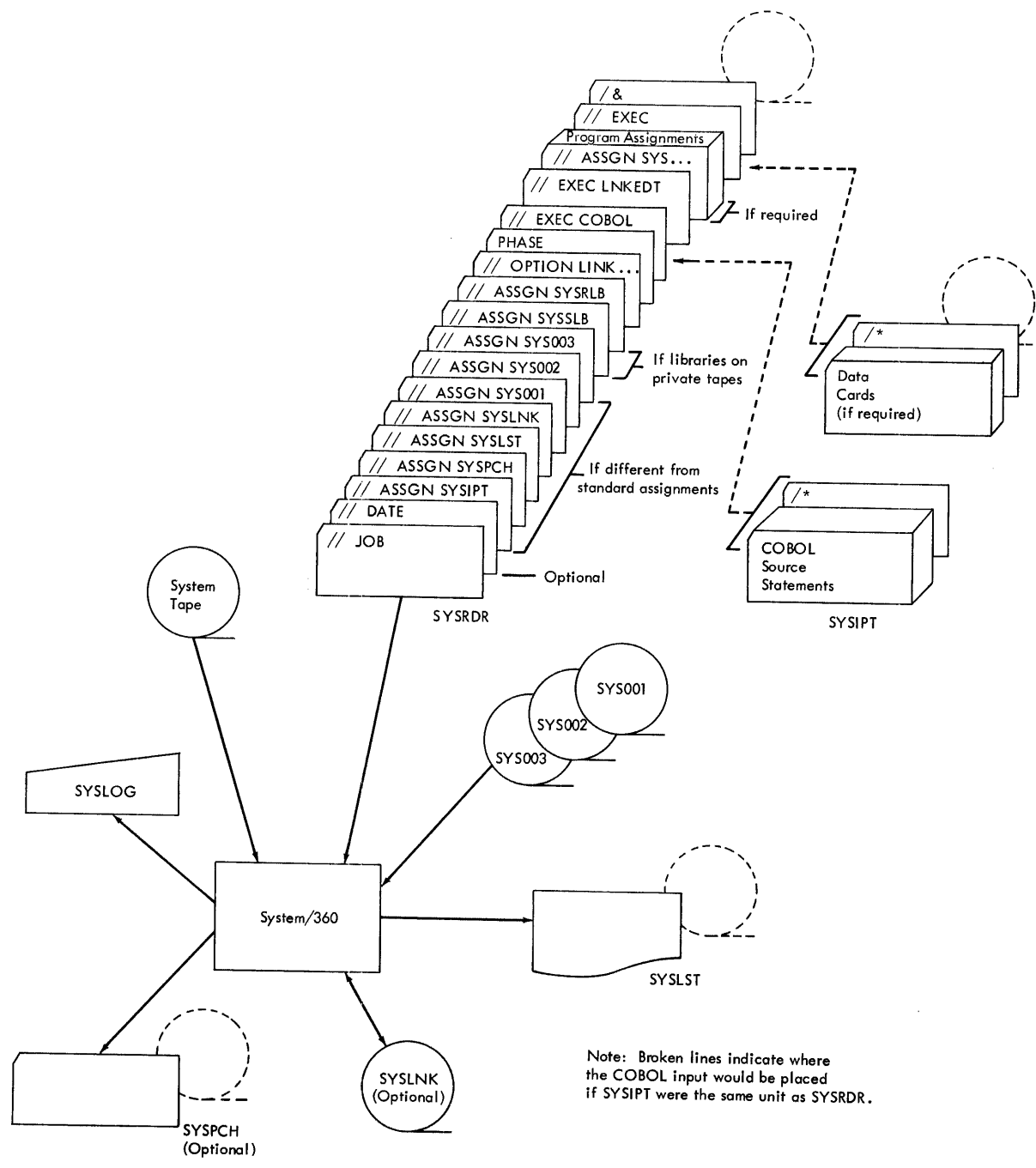
Figure 3. Input/output Units Used by COBOL Program in a Tape System
