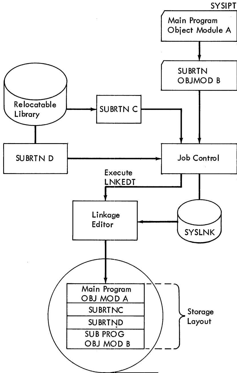
Figure 14. Example of Data Flow Logic in a Call Structure
