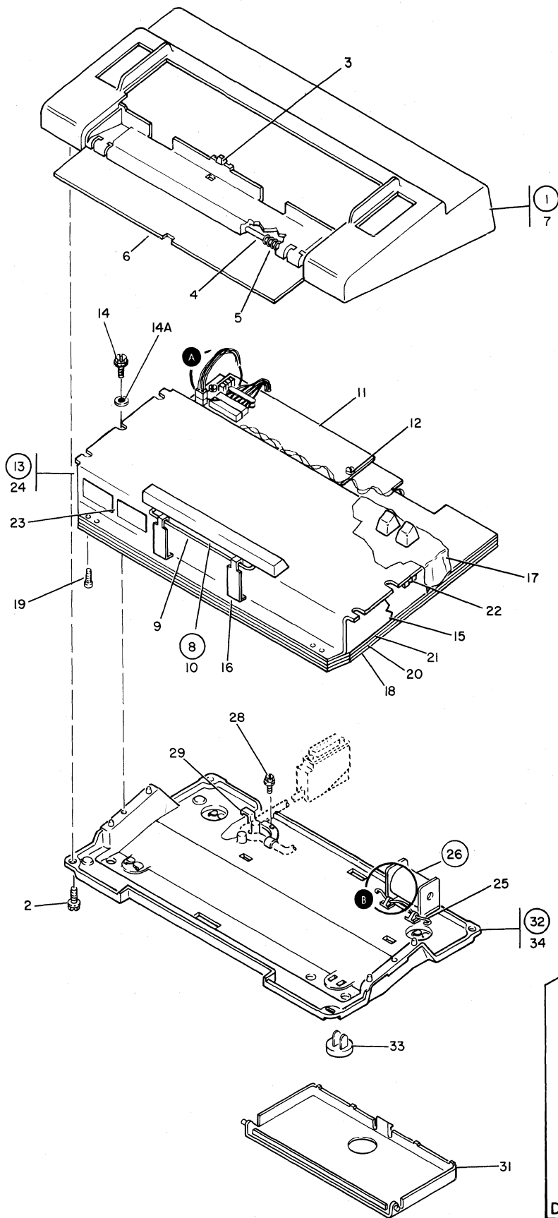
FIGURE 6. KEYBOARD FINAL ASSEMBLY.
