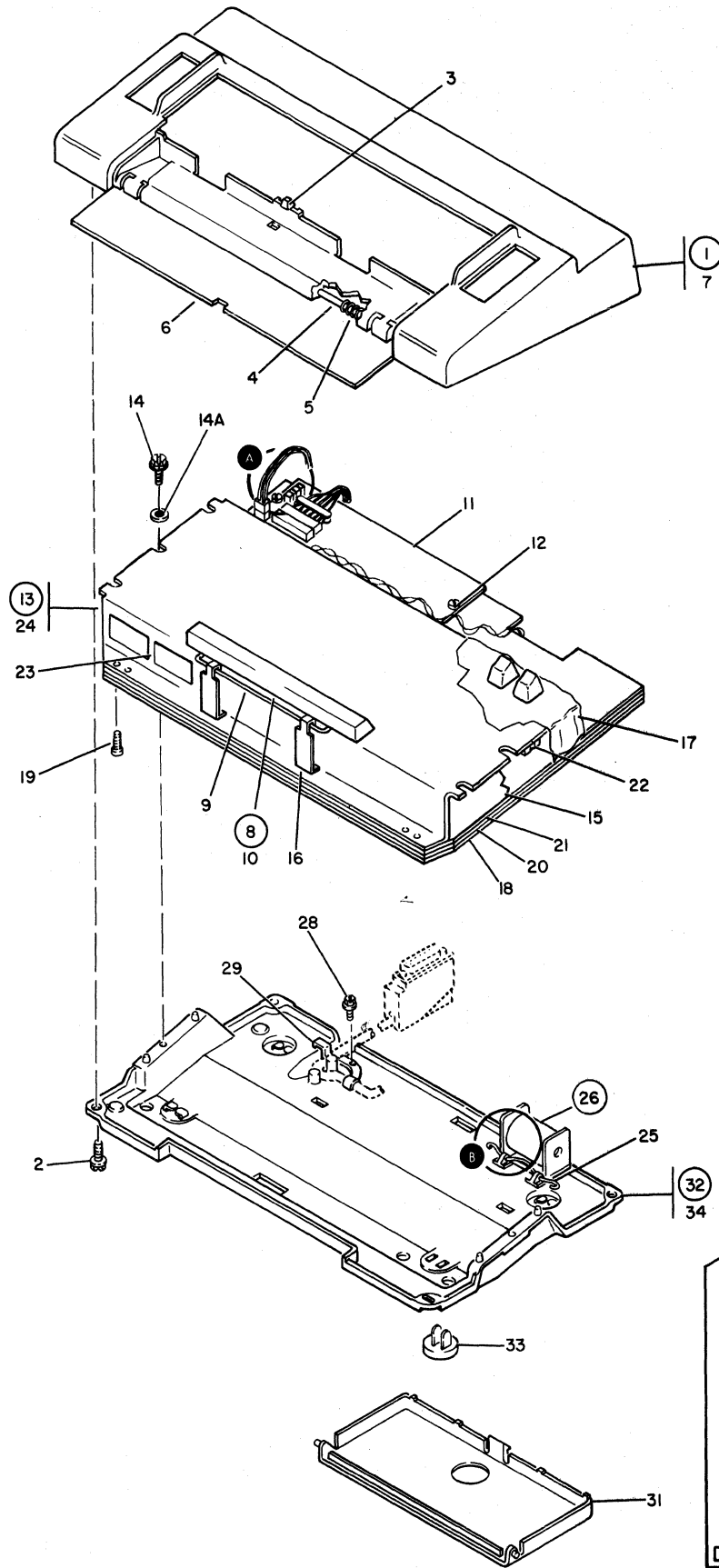
FIGURE 6. KEYBOARD FINAL ASSEMBLY.
