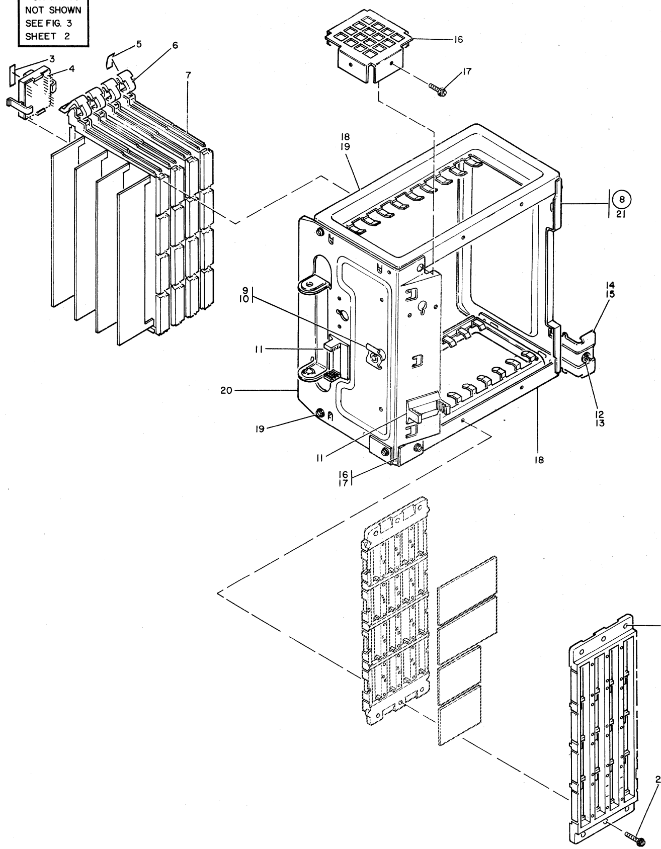
FIGURE 4. A GATE ASSEMBLY.
