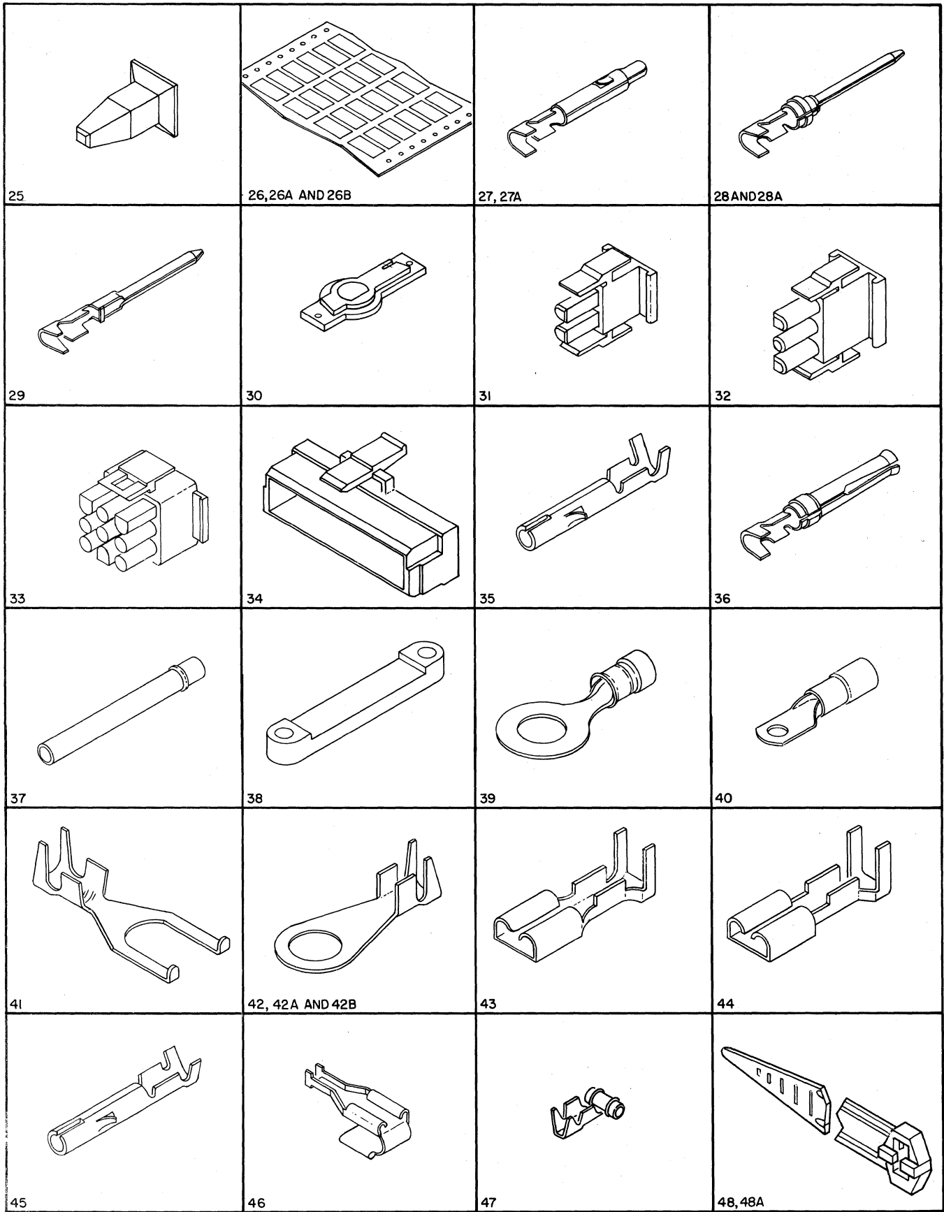
FIGURE 8. CABLE ASSEMBLIES WITH COMPONENT PARTS. SHEET 2 OF 3. INDEX NOS. 25-48A.
