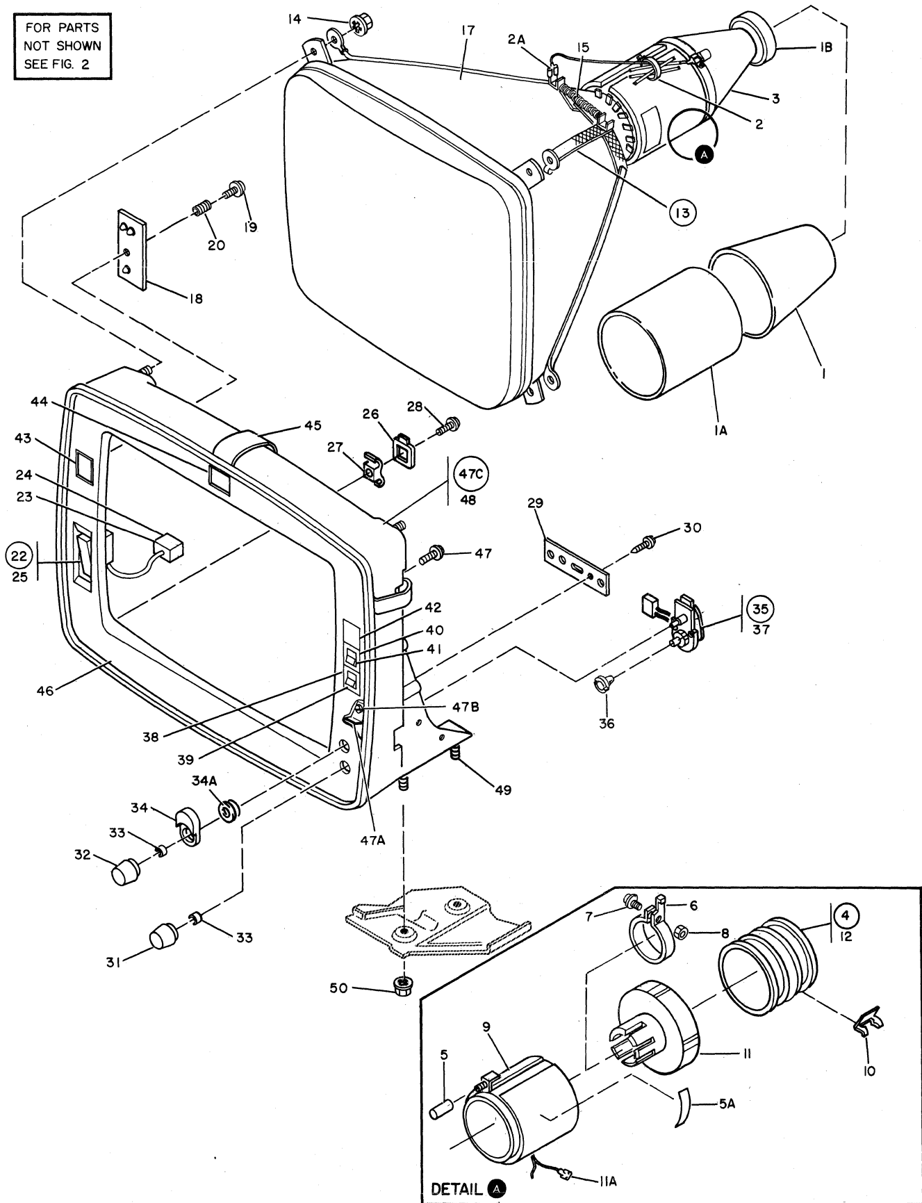
FIGURE 3. UPPER ASSEMBLY. SHEET 1 OF 2. INDEX NOS. 1-50.
