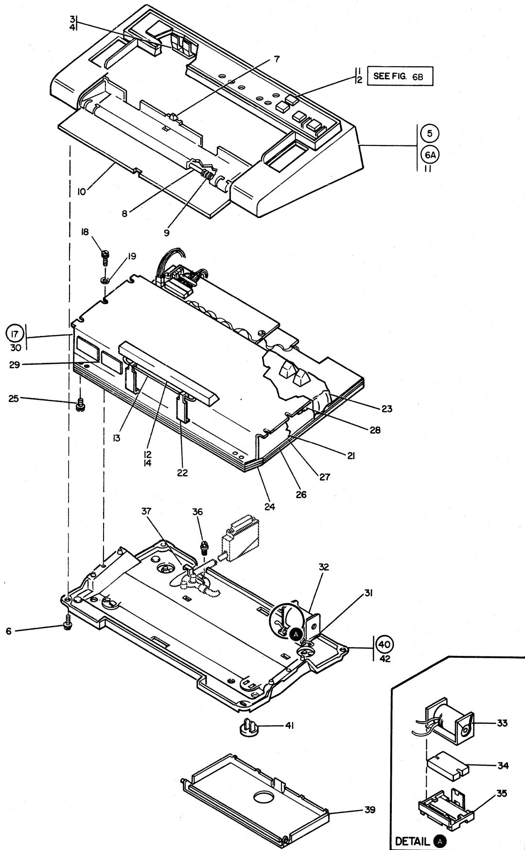
FIGURE 6A. KEYBOARD FINAL ASSEMBLY. SEE LIST 6A.
