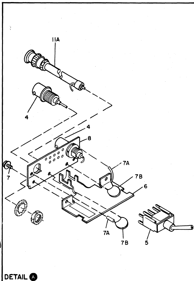
FIGURE 2A. CONTROLLER SWITCH ASSEMBLY. SEE LIST 2A.
