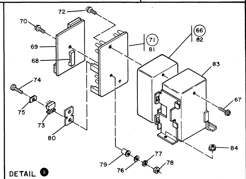
FIGURE 3. UPPER ASSEMBLY. SHEET 2 OF 2. INDEX NOS. 51-95
