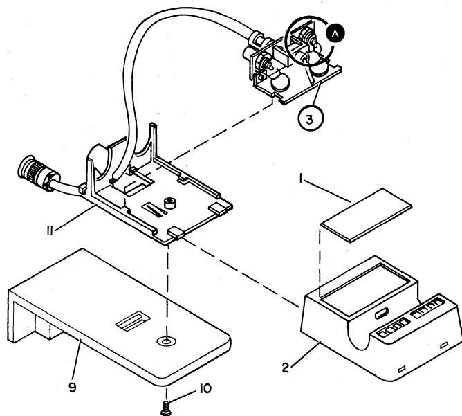
FIGURE 2A. CONTROLLER SWITCH ASSEMBLY. SEE LIST 2A.
