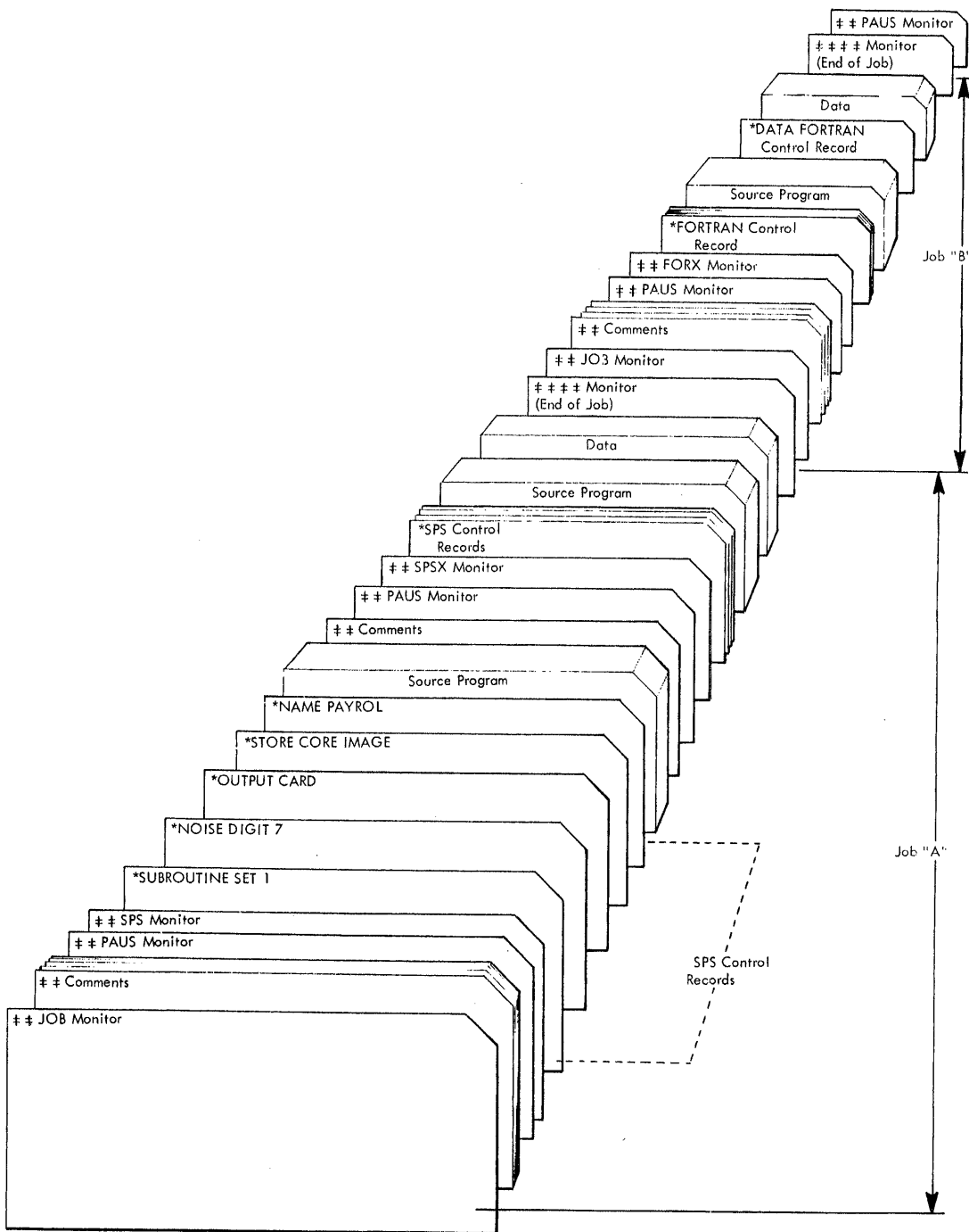
Figure 4. Stacked Input, SPS and FORTRAN Jobs
