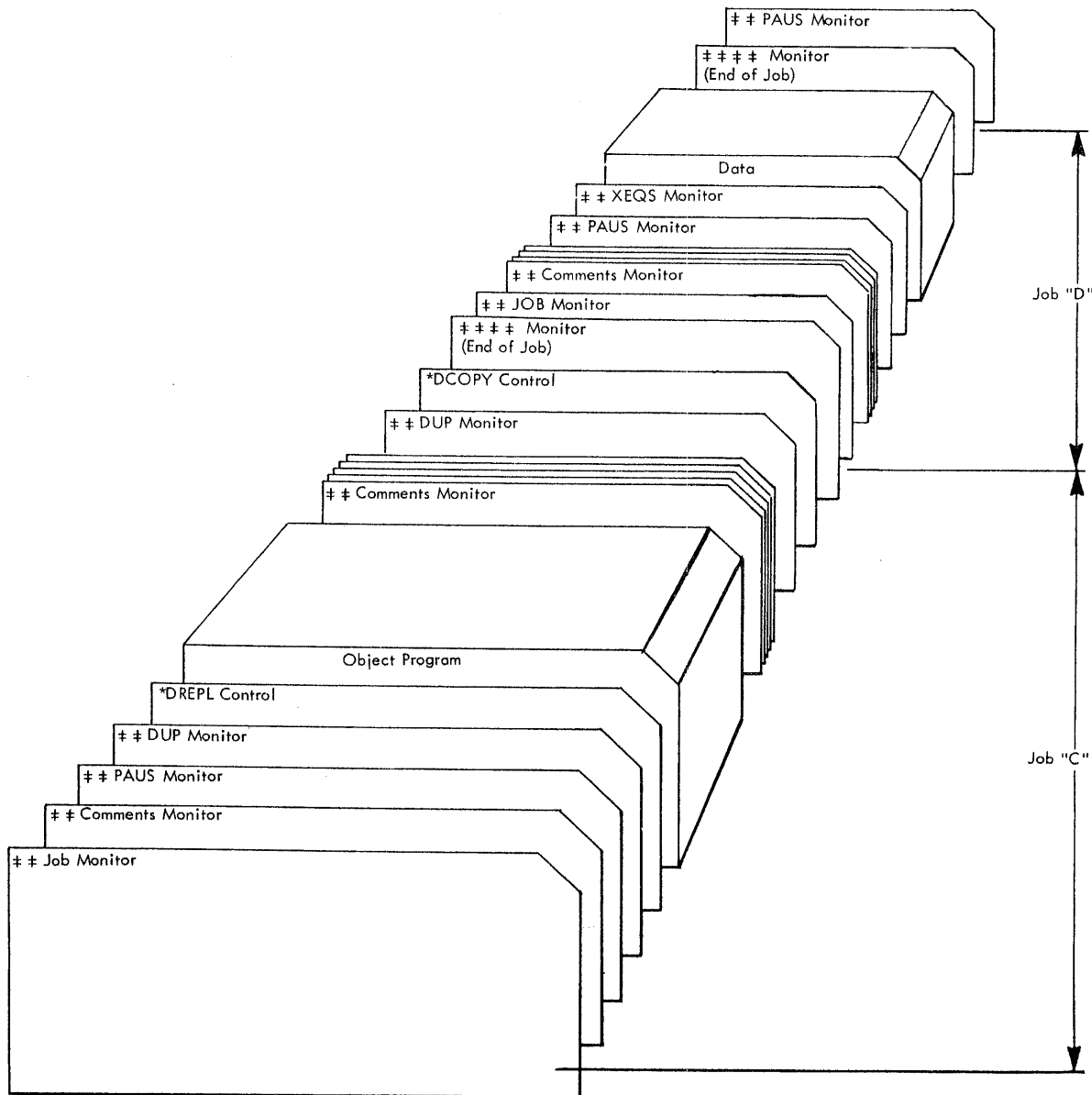
Figure 5 Stacked Input, DUP and XEQS Jobs
