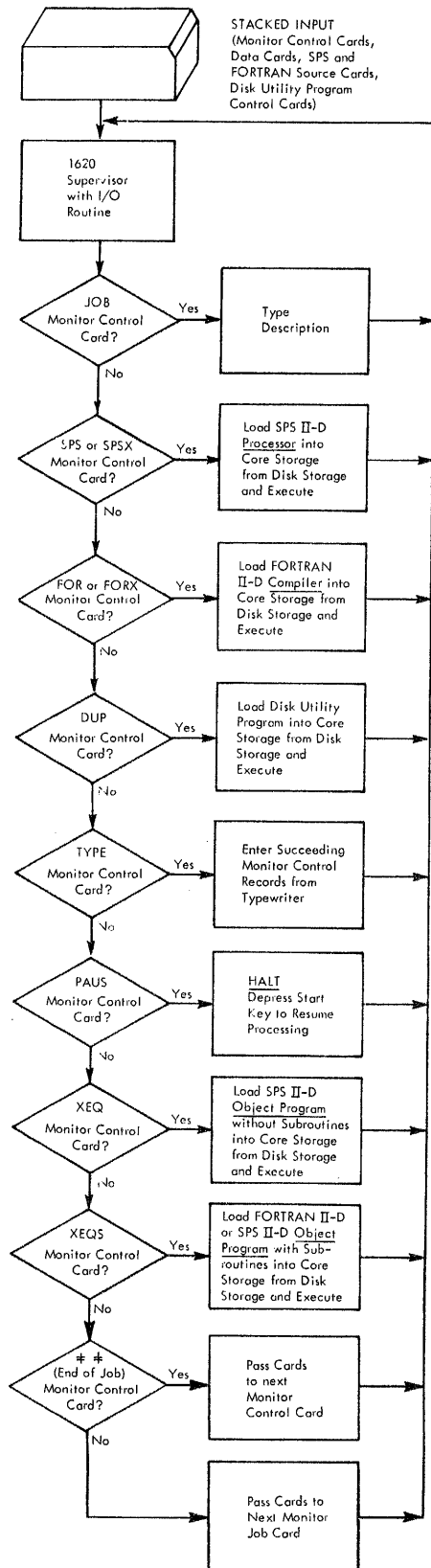
Figure 3. Logic of Supervisor
