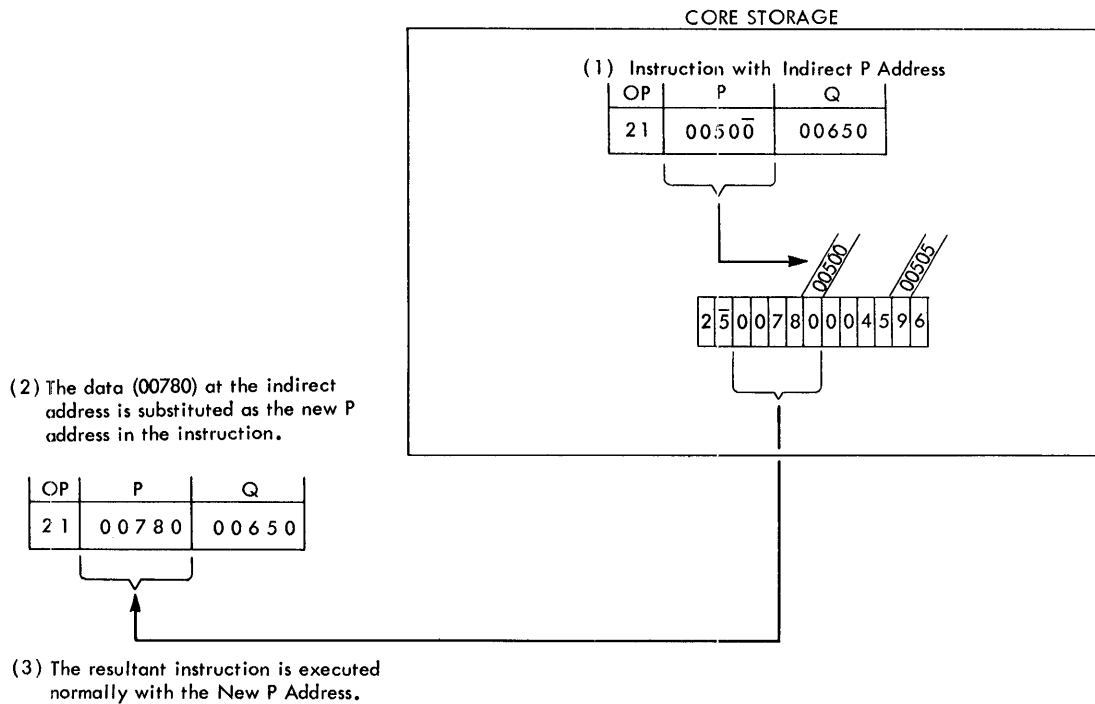
Figure 18. Indirect Addressing
