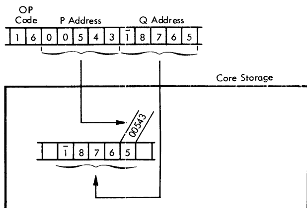
Figure 16. Transmit Field Immediate - Data Flow
