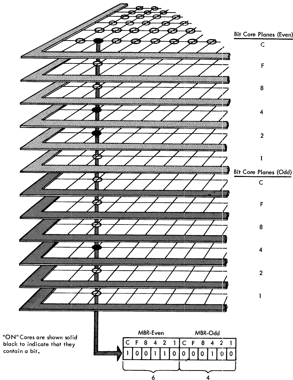
Figure 3. 1620 Core Storage Readout
