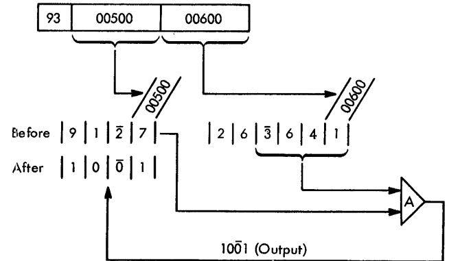
Figure 71. AND To Field - Data Flow
