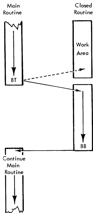
Figure 31. Subroutine Linkage
