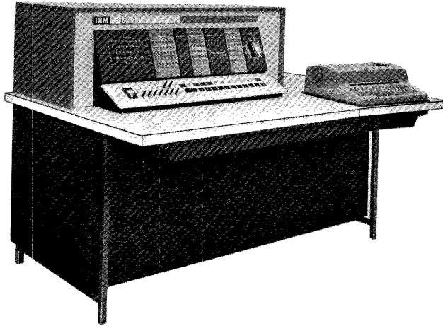
Figure 86. IBM 1620-2 with I/O Typewriter
