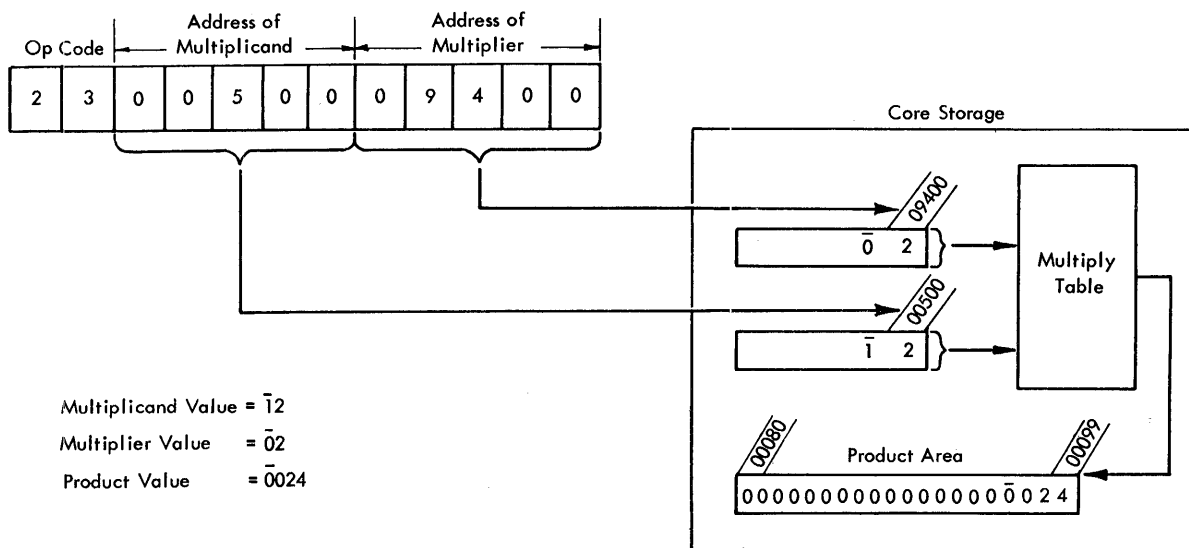
Figure 24. Multiply Instruction — Data Flow
