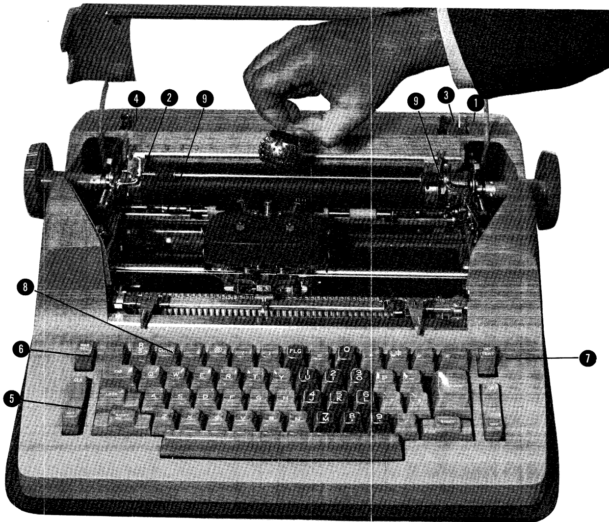
Figure 87. 1/0 Typewriter, Manual Controls and Keys
