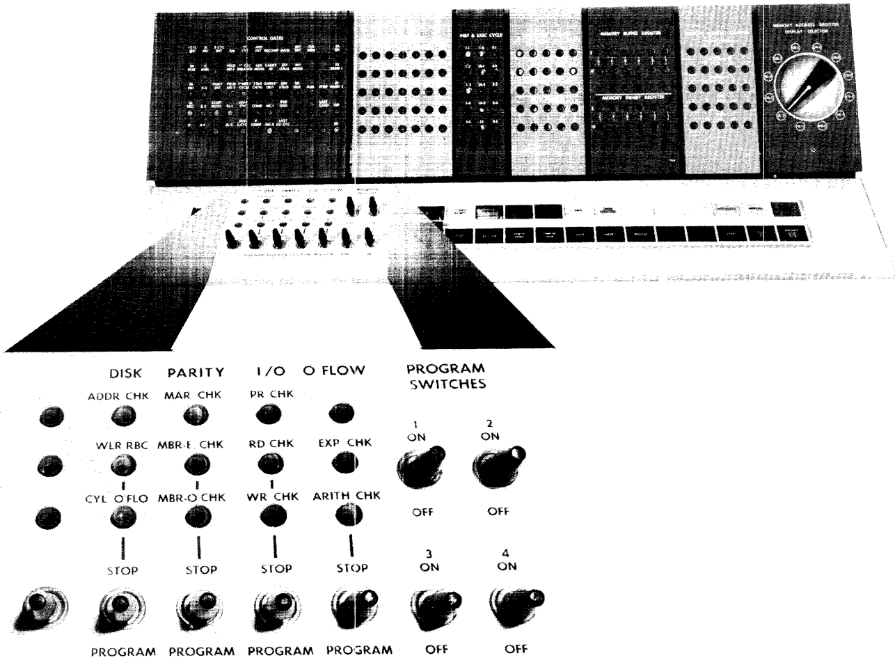
Figure 79. Indicator Lights and Switches
