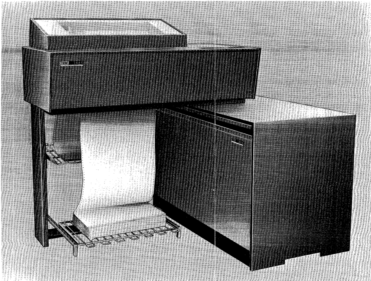
Figure 10. IBM 1443 Printer
