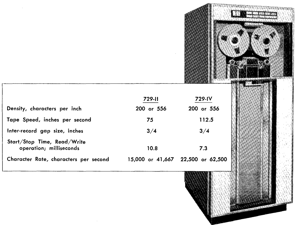
FIGURE 47. OPERATING CHARACTERISTICS OF IBM 729 TAPE UNITS
