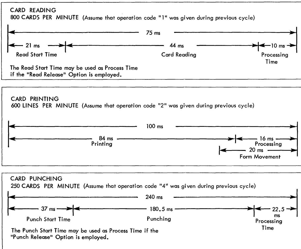
FIGURE 59. 1401 TIMINGS
