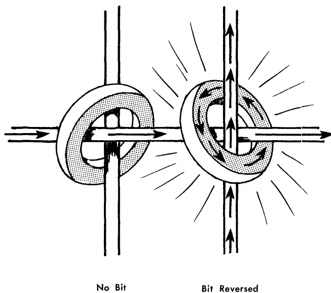
FIGURE 4. MAGNETIC CORE
