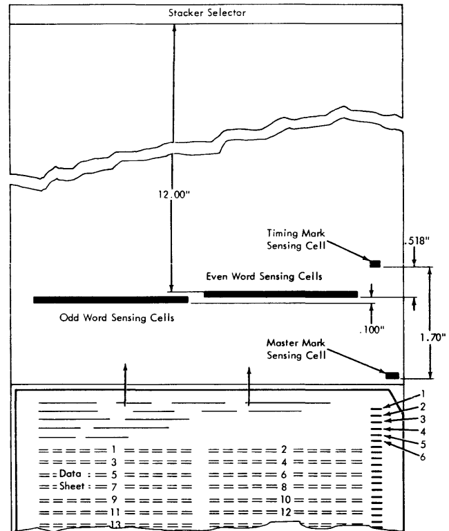
Figure 8. Reading Schematic
