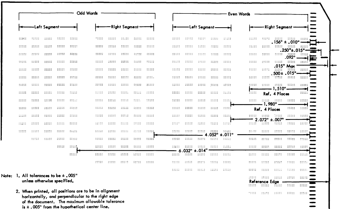
Figure 32. Horizontal Dimensions
