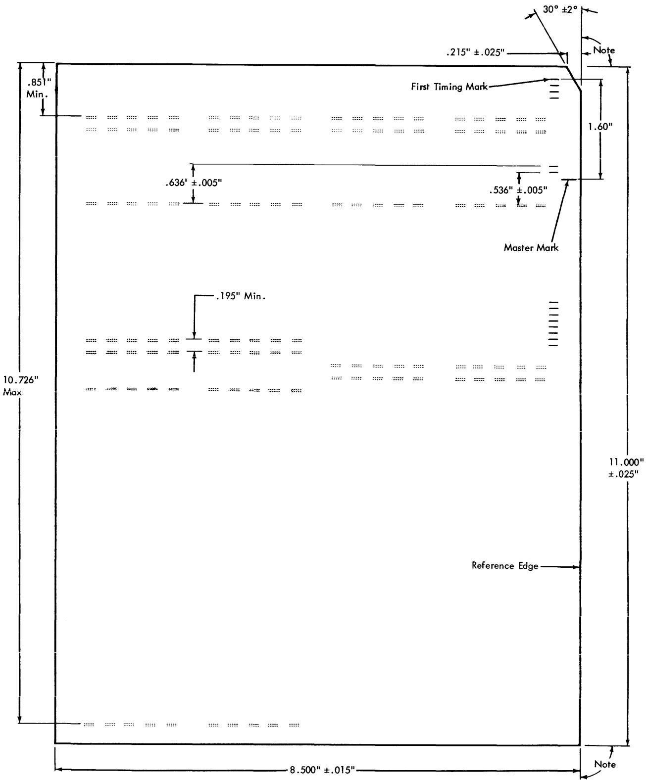
Figure 9. Vertical Dimensions
