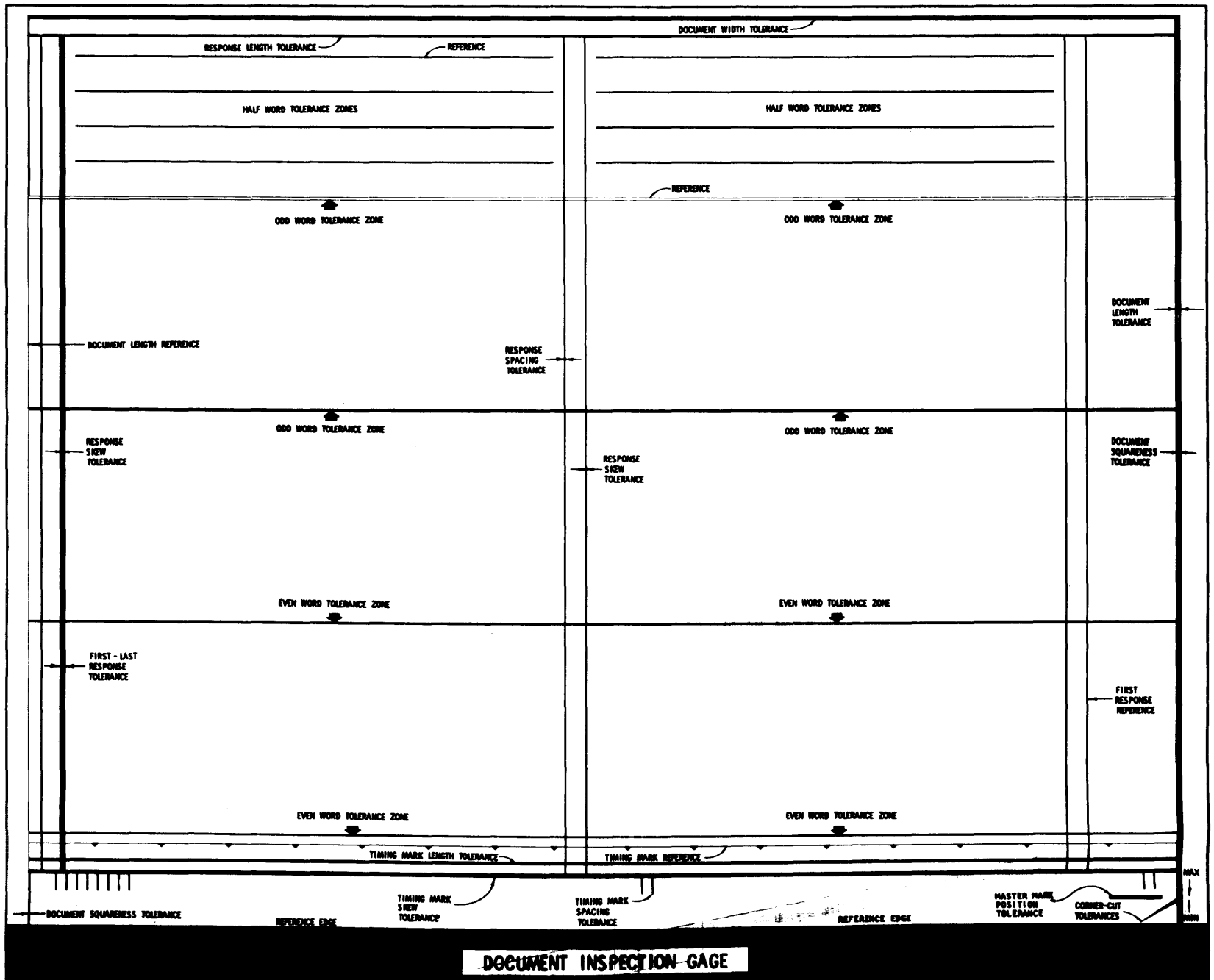
Figure 37. Document Gage
