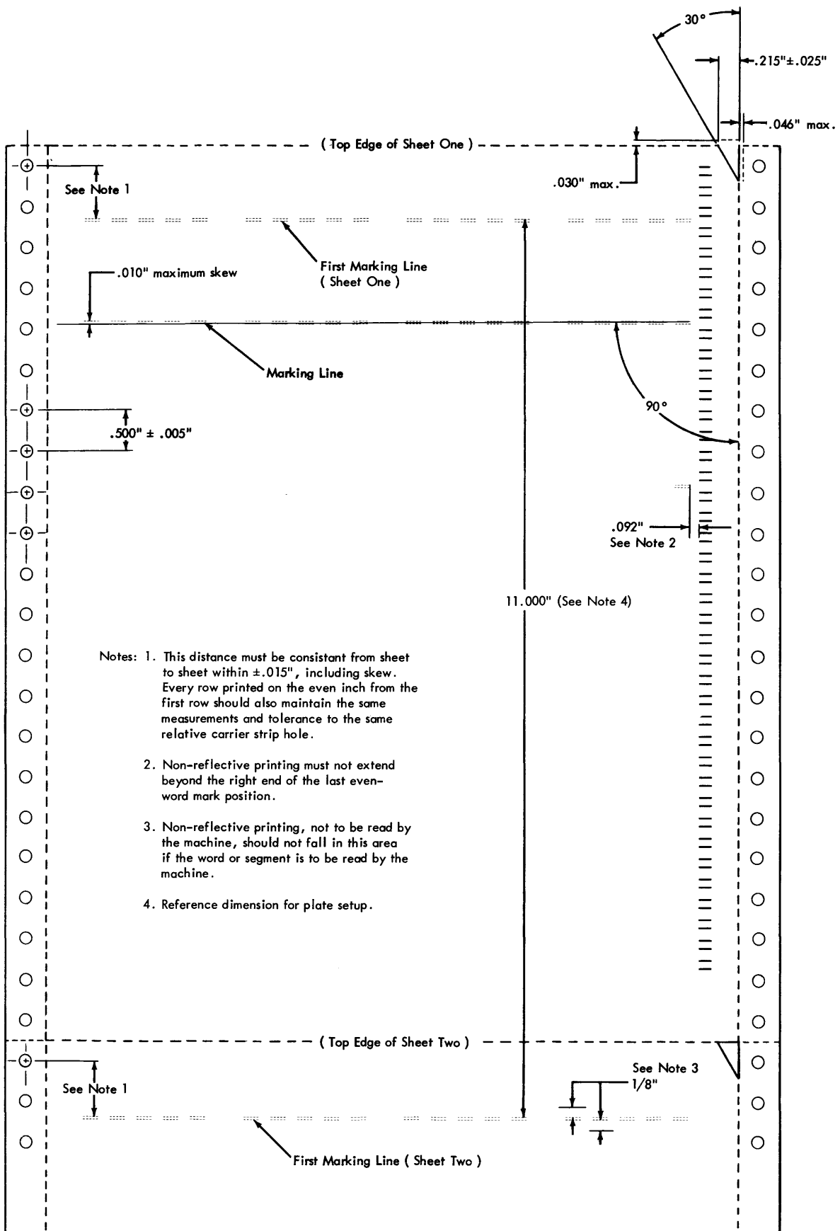
● Figure 30. Continuous Forms Dimensions
