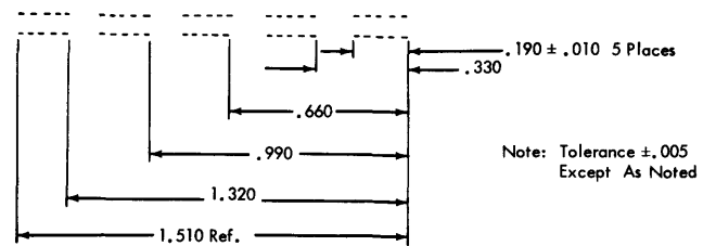
Figure 34. Segment Dimensions
