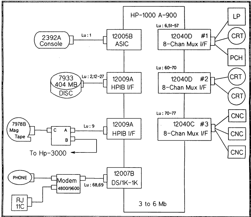
Figure-1. Typical HP-1000 A900 System
