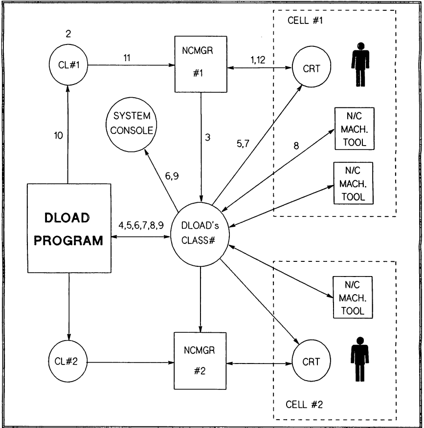
Figure-4. DLOAD Class I/O Communications
