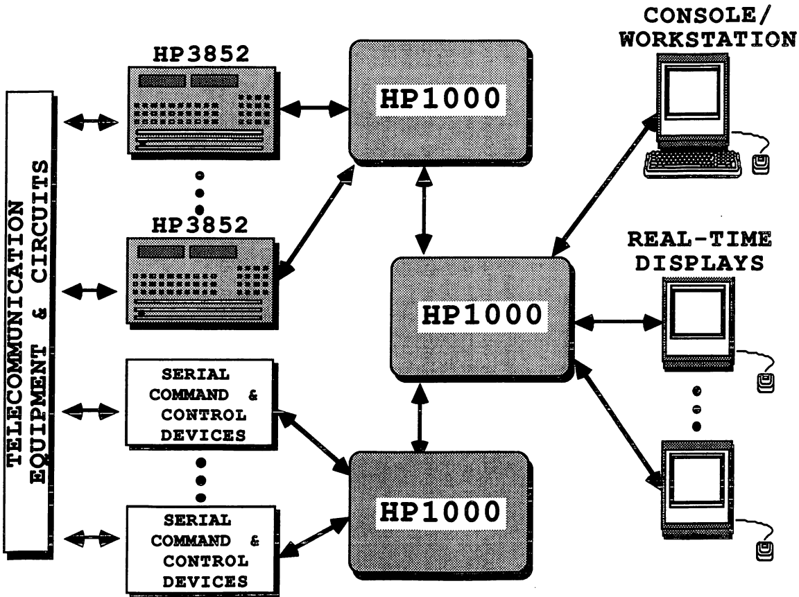
DAMS Configuration Figure 2
