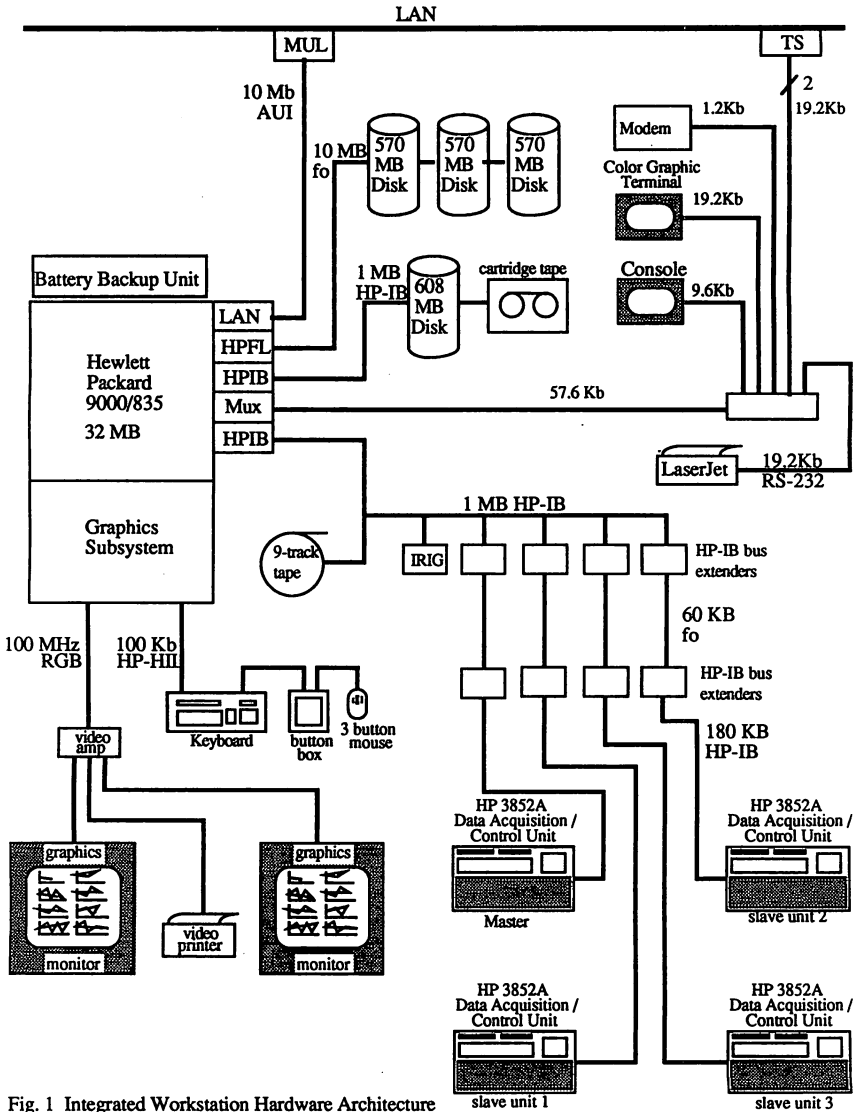
Fig. 1 Integrated Workstation Hardware Architecture
