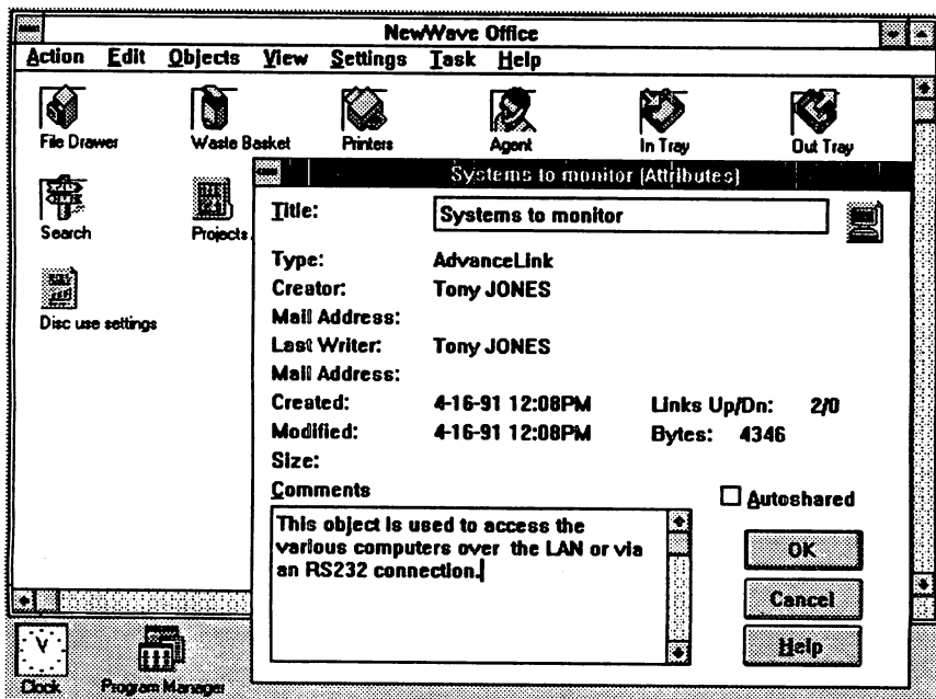
Figure 2: Object Attributes
