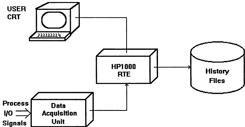
figure 2. Stand-alone system
