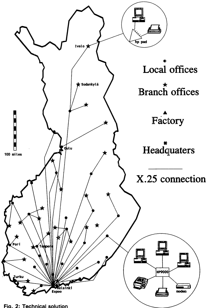
Fig. 2: Technical solution
