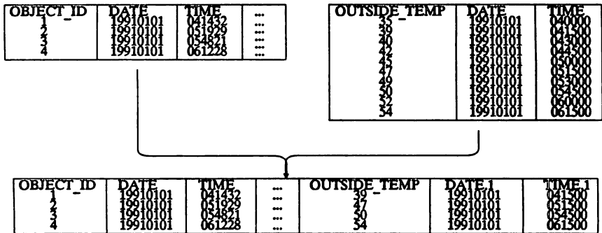
FIGURE 6 (JOIN by 'NEAREST' DATE, TIME )
