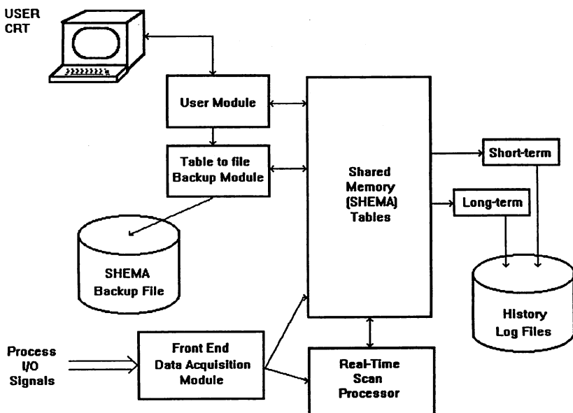
figure 1. Stand-alone system module layout
