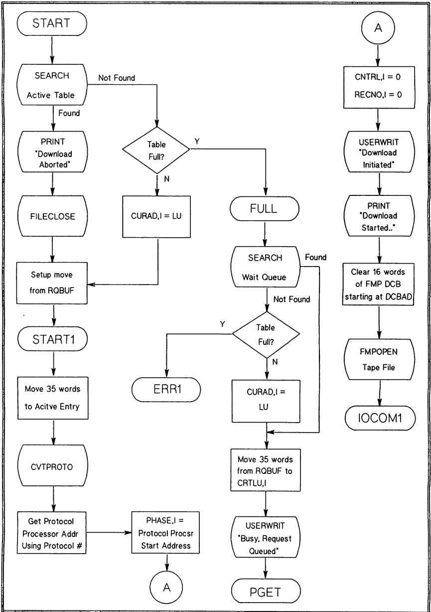
Figure-9. Start Download Section Flowchart
