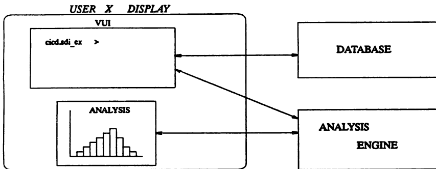
FIGURE 7 (VUI interaction)
