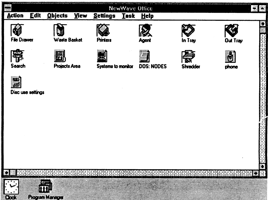
Figure 1: NewWave Environment
