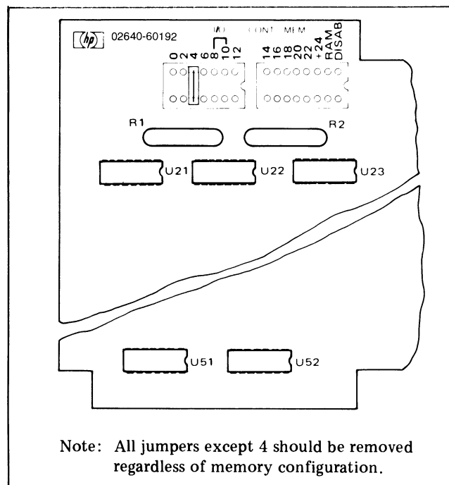
Figure 7-36. Second Control Memory PCA Jumper Configurations (HP 2641A)
