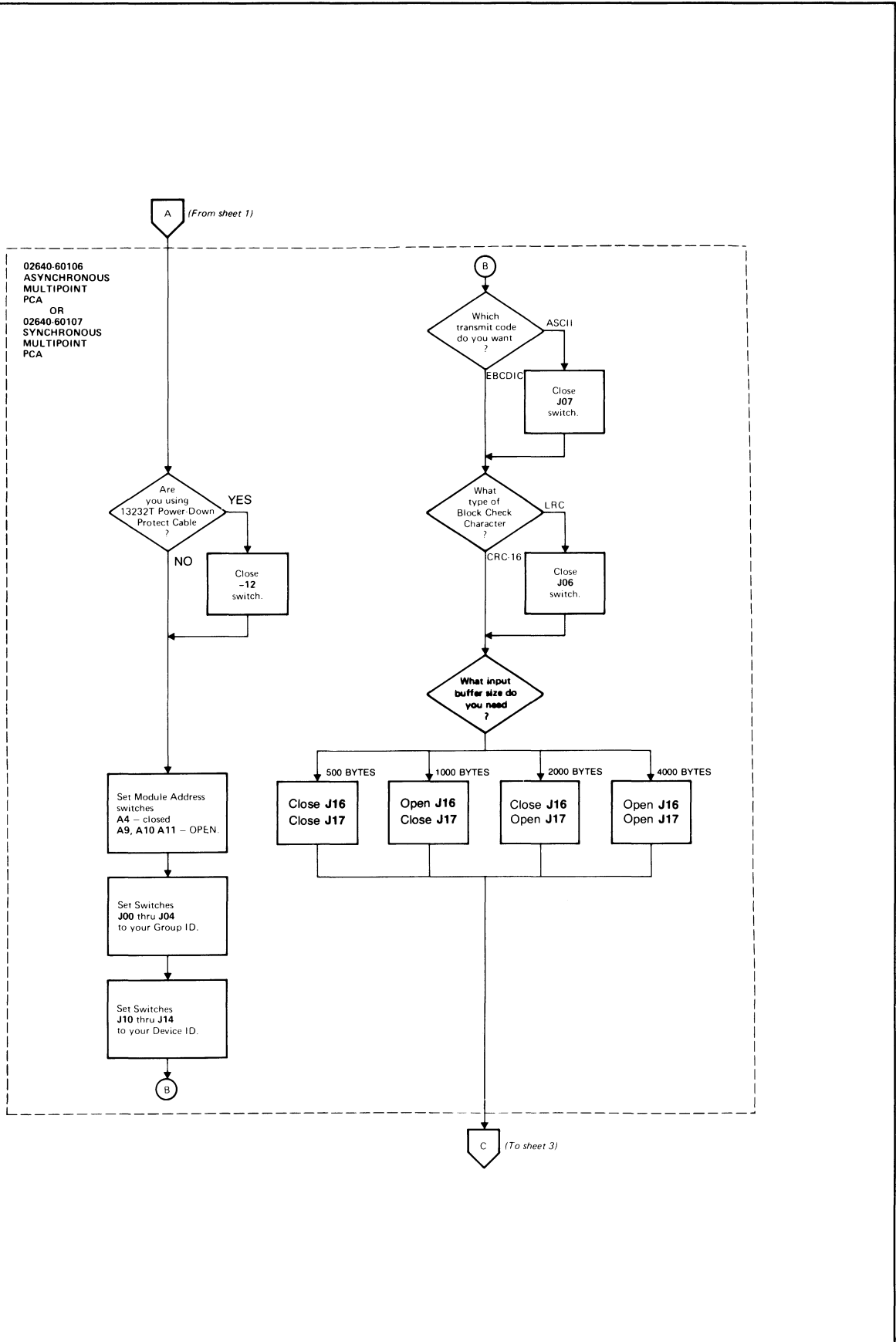
Figure 5-17. Multipoint Data Communications Configuration (Sheet 2 of 4)
