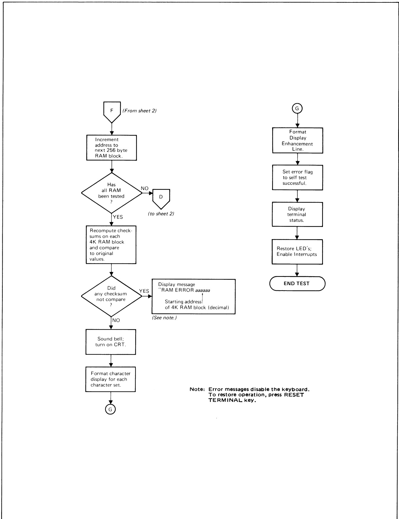
Figure 7-32. Basic Terminal Self-Test Flowchart (Sheet 3 of 3)
