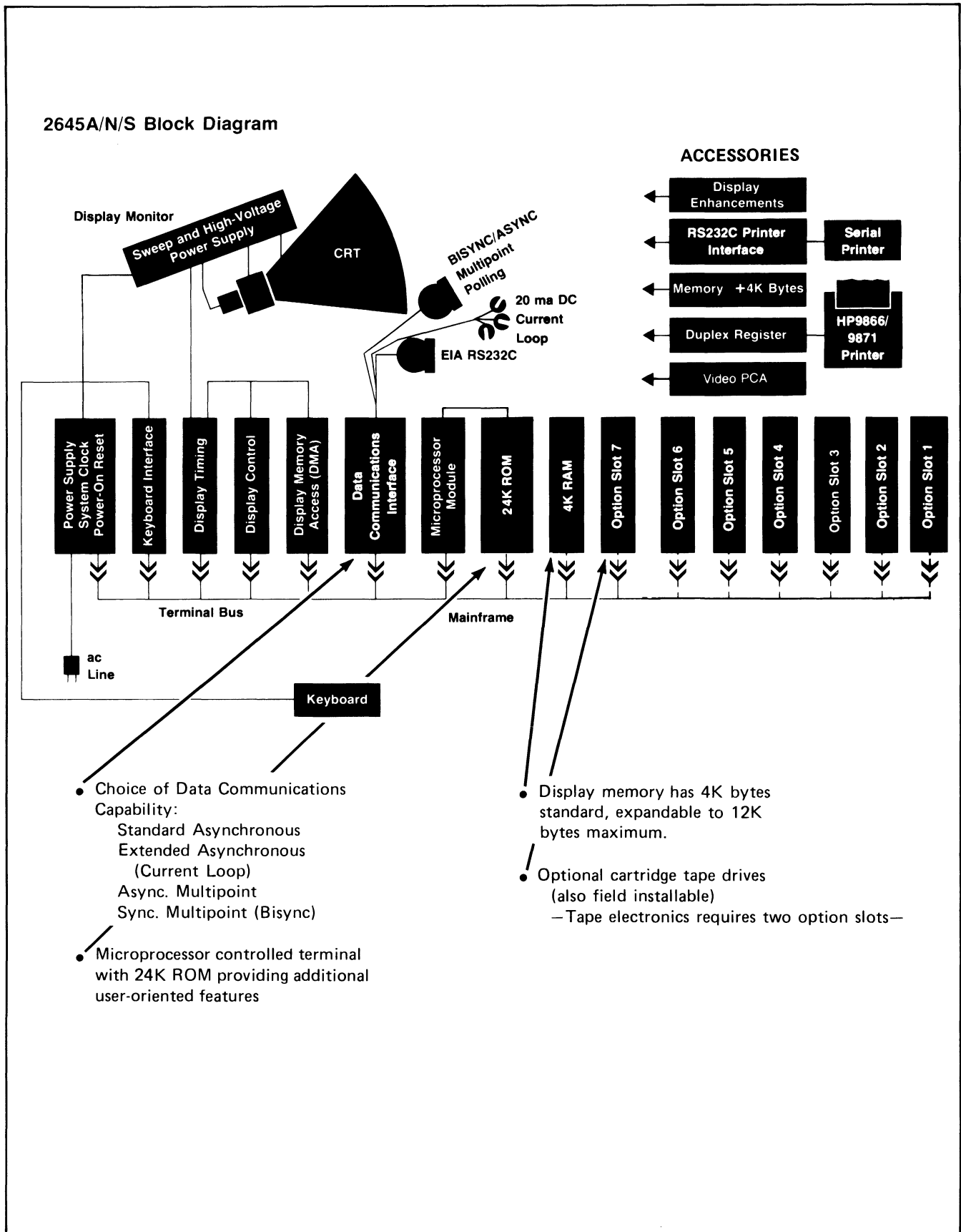
Figure 1-2. 2645A/N/S Architecture
