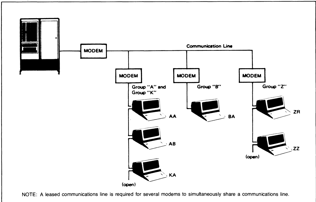
Figure 5-14. Terminal Addressing
