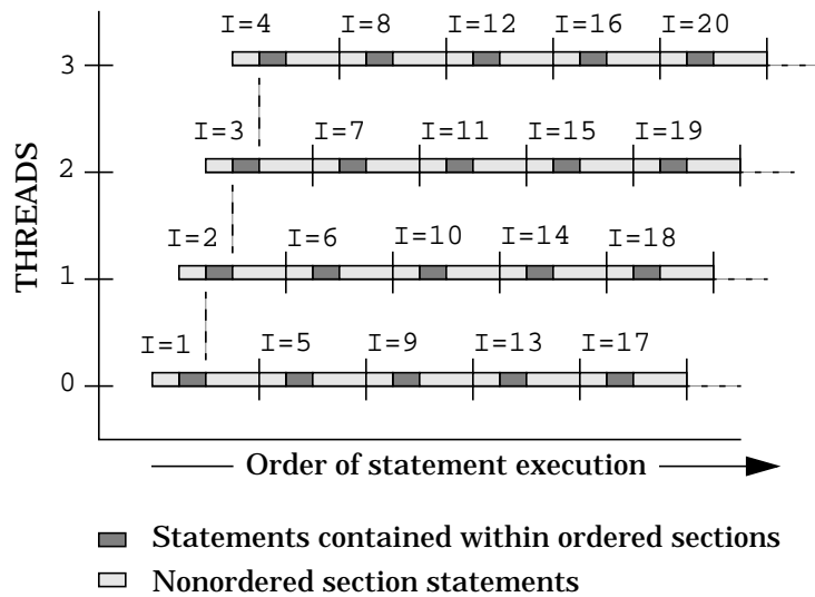
LOOP_PARALLEL(ORDERED) synchronization
