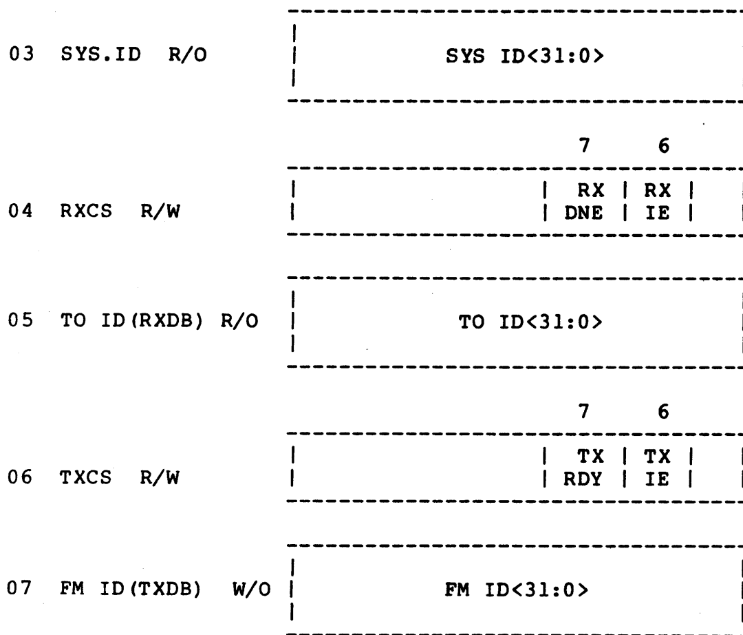
ID registers as seen by VAX 11/780 microcode
