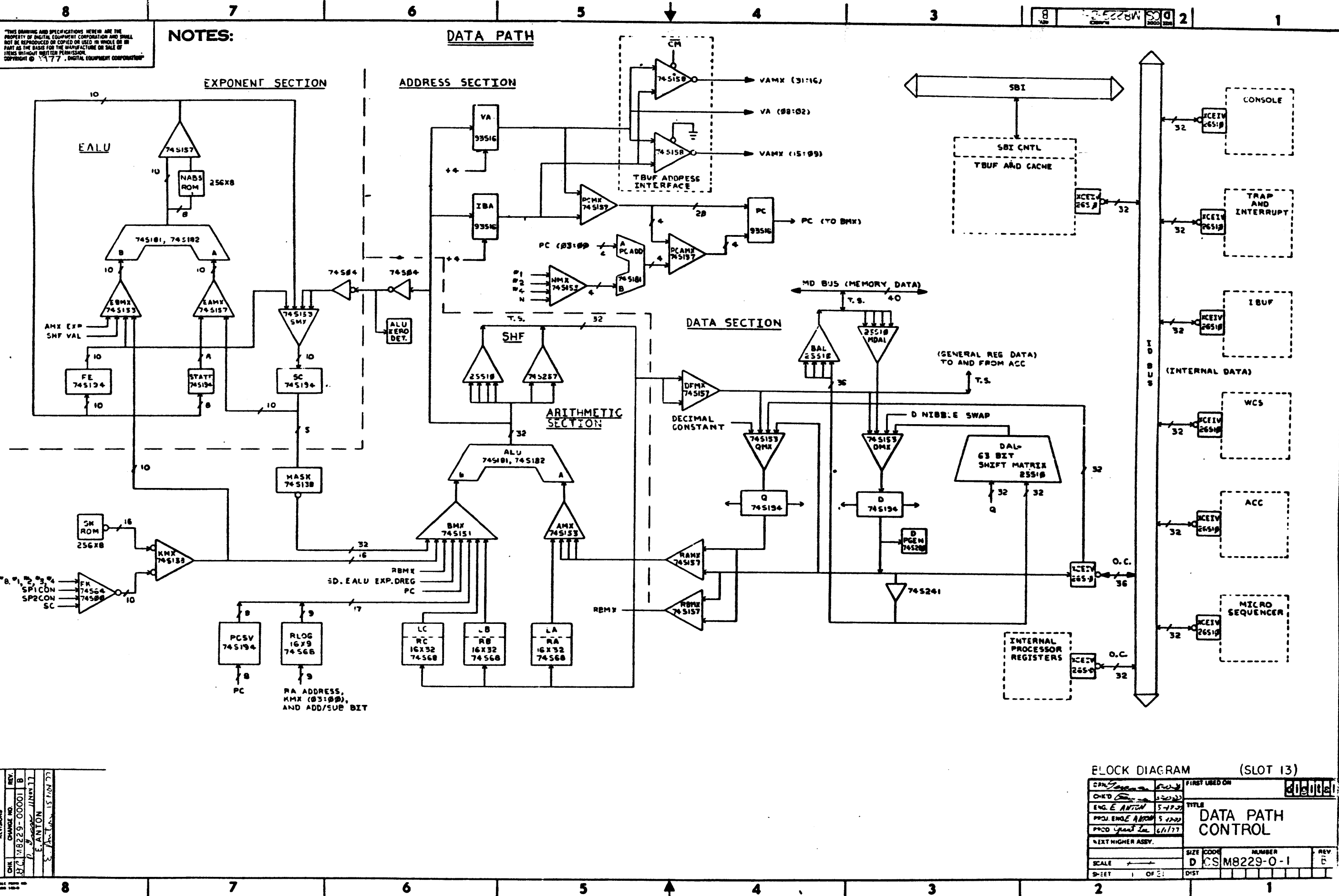
DATA PATH SPECIFICATION BLOCK DIAGRAM - FIGURE 1-1 PAGE 1-2
