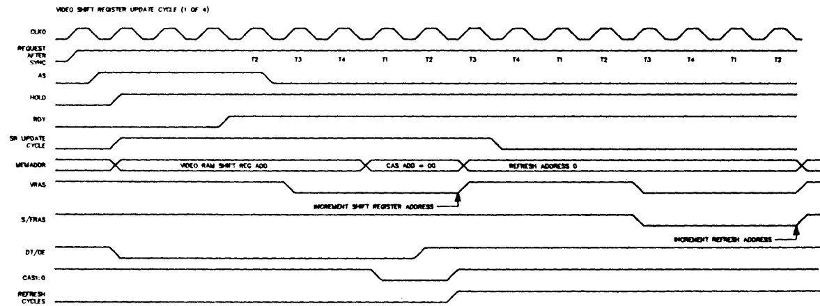
Figure A-11: Video Shift Register Update Cycle
