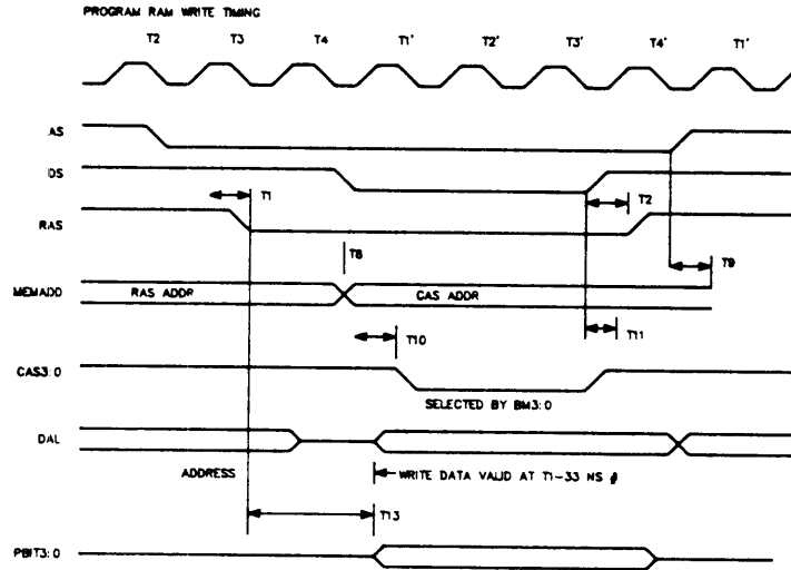
Figure A-3: Program RAM Write
