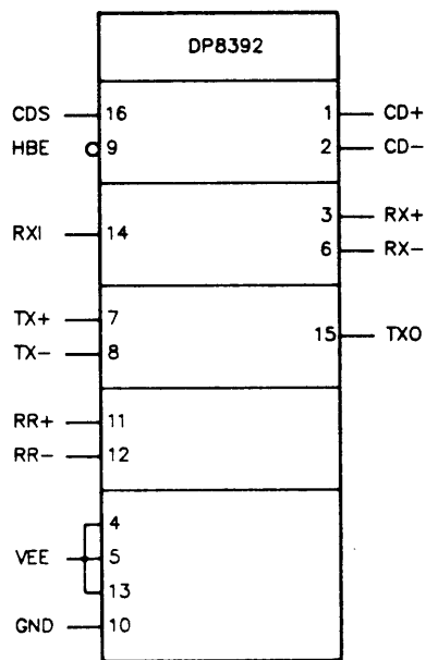
Figure 3-117: Coaxial Transceiver Interface Chip Pinout
