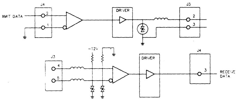
Figure 9-2: DEC423 Converter Block Diagram for Line 3
