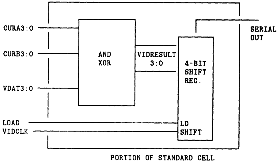
Figure 3-45: Video RAM and Cursor Block Diagram
