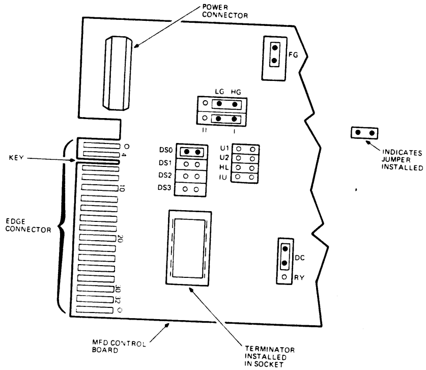
Figure 8-3: RX33 Jumper Settings
