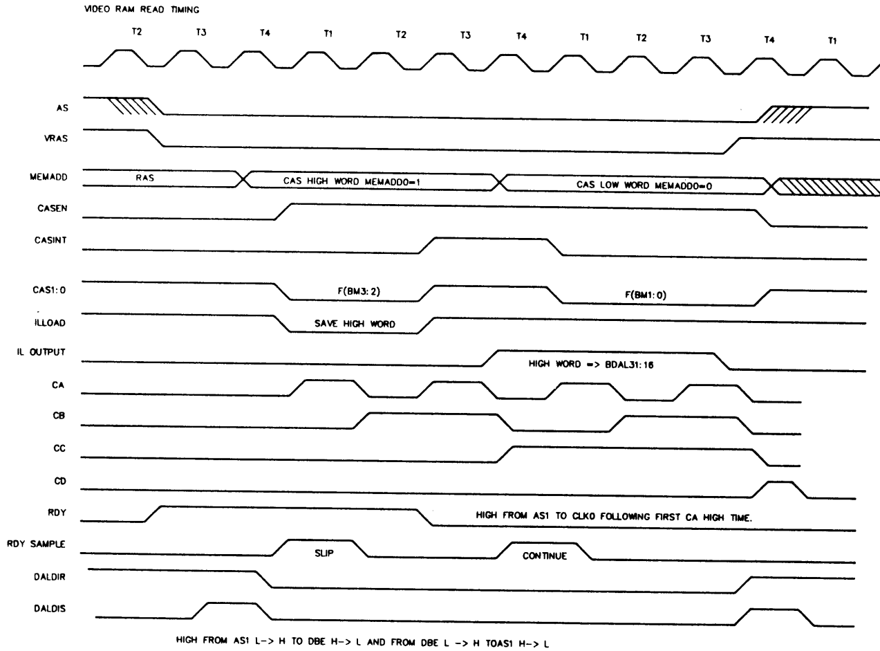
Figure A-6: Video RAM Read
