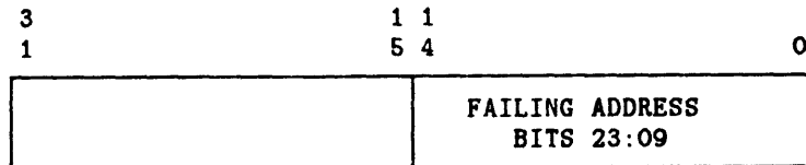
Figure 3-26: Memory Error Address Register (MEAR)
