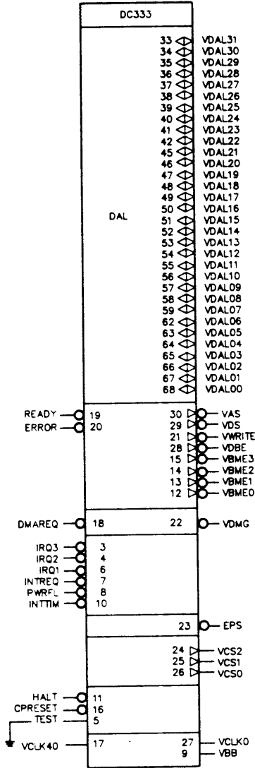
Figure 3-3: CPU Chip Pinout
