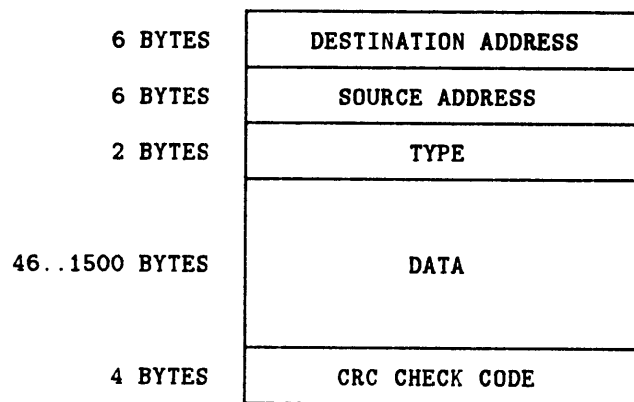
Figure 5-2: Ethernet Packet Format
