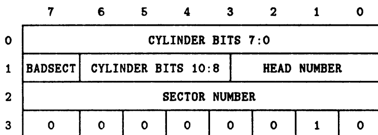
Figure 3-95: ID Field Bytes for Each Sector
