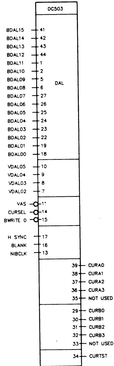
Figure 3-54: DC503 Cursor Sprite Chip Pinout
