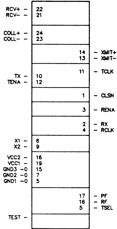
Figure 5-4: SIA Chip Pinout
