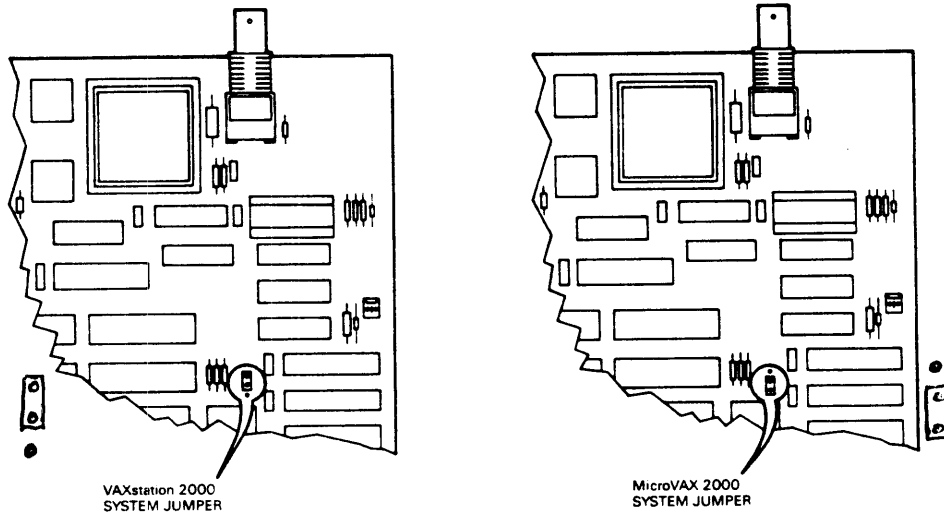
Figure 3-120: VAXstation 2000 and MicroVAX 2000 System Jumper
