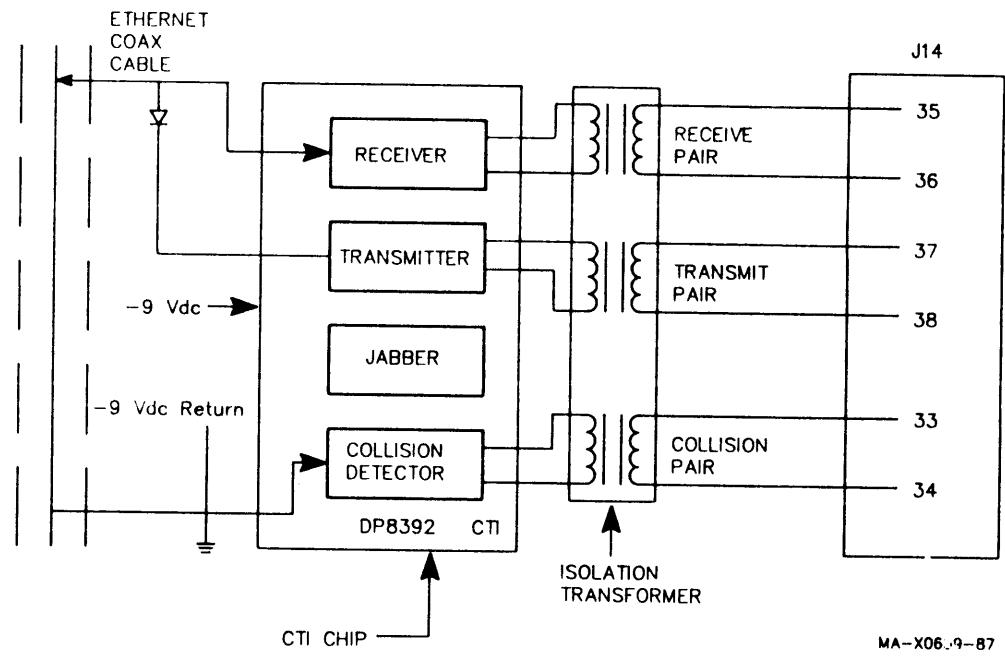
Figure 3-116: ThinWire Ethernet Transceiver Circuitry
