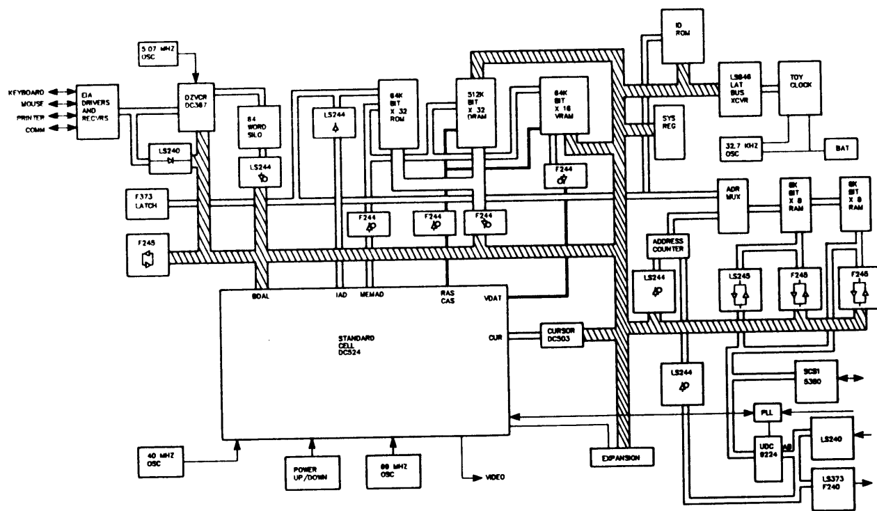
Figure 2-5: DC524 Standard Cell Functional Block Diagram
