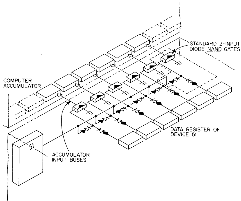
Figure 29 Loading Data into the Accumulator from an External Device
