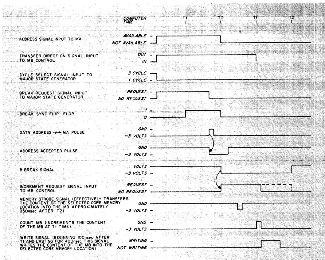
Figure 40 Memory Increment Data Break Timing Diagram
