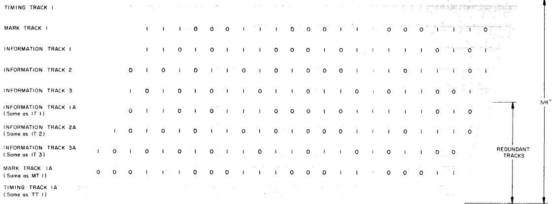
Figure 9 DECTape Track Allocations
