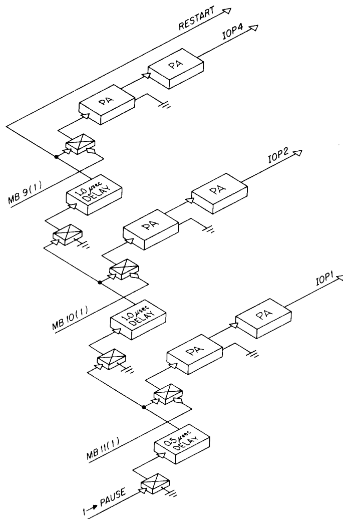
Figure 24 IOP Generator Logic
