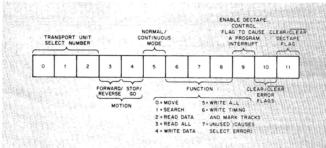
Figure 13 DECTape Status Register A Bit Assignments
