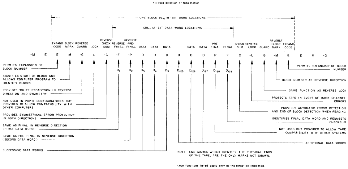
Figure 10 DECTape Mark Channel Format
