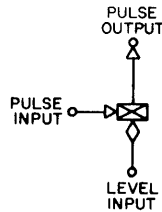
Figure 51 Diode-Capacitor-Diode Gate Logic Symbol
