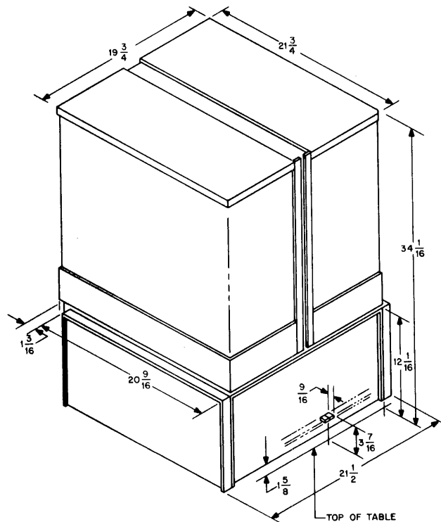
Figure 57 Table Mounted PDP-8 Installation Dimensions
