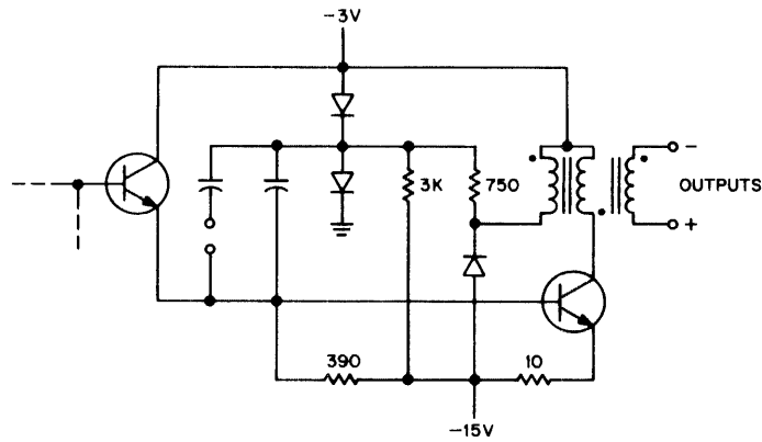
Figure 53 Pulse Amplifier Output Circuit Schematic
