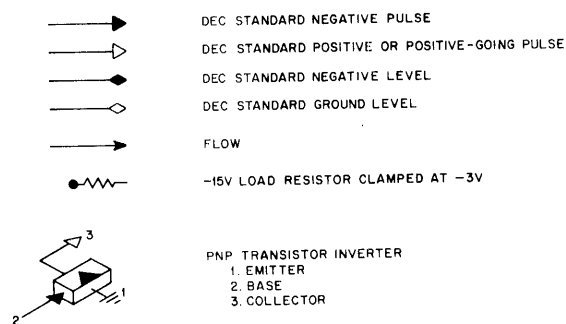
Figure 20 Logic Symbols
