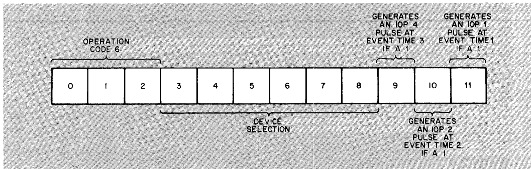
Figure 5 IOT Instruction Bit Assignments
