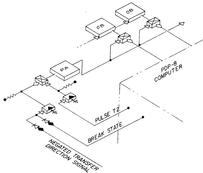
Figure 39 Device Interface for Strobing Output Data
