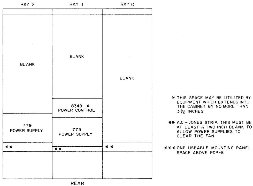
Figure 60 Typical PDP-8 System Configuration and Layoff Planning
