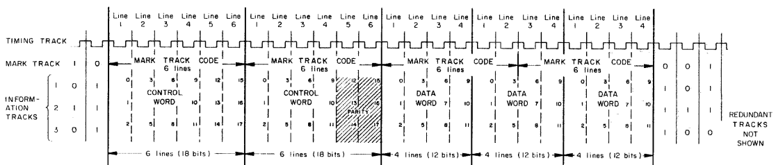
Figure 12 DECTape Format Details
