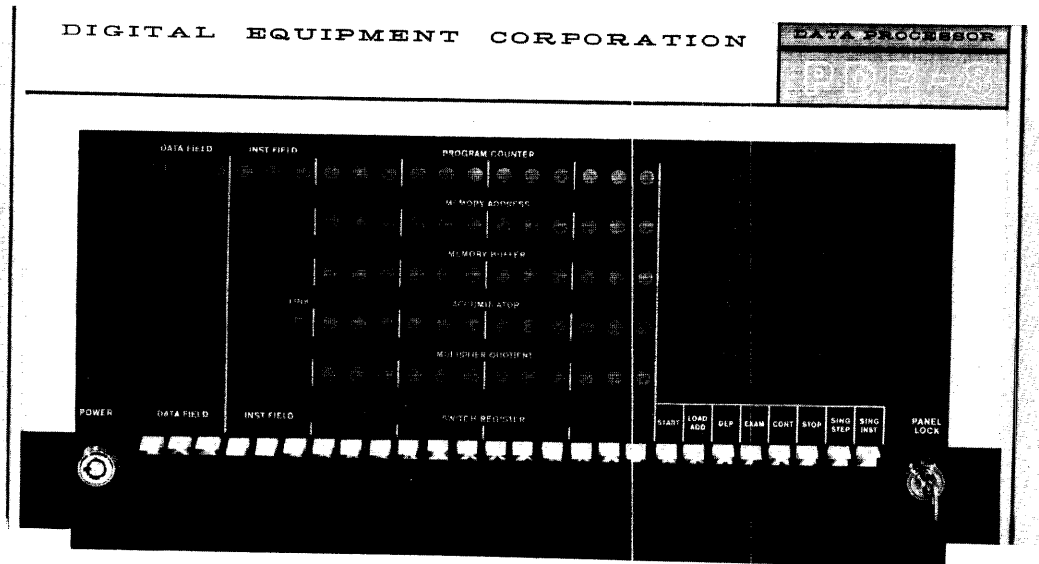
Figure 18 PDP-8 Operator Console
