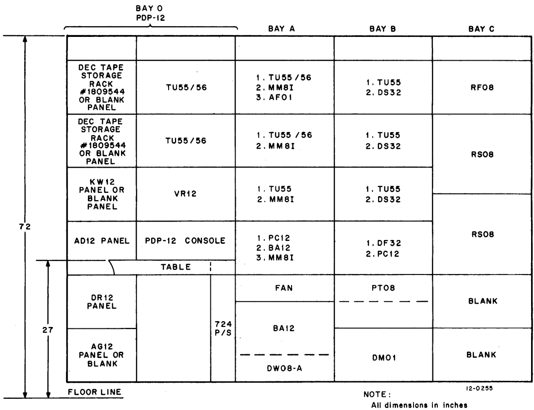
Figure 1-3 PDP-12 Expanded Equipment Layout (see Drawing PDP12-0-2)
