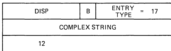
Figure A-28 Complex Relocation Entry Format
