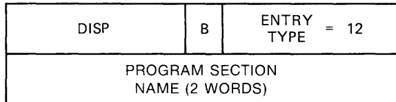
Figure A-24 Program Section Relocation Entry Format
