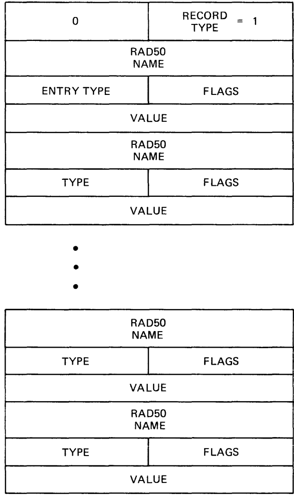
Figure A-2 Global Symbol Directory Record Format
