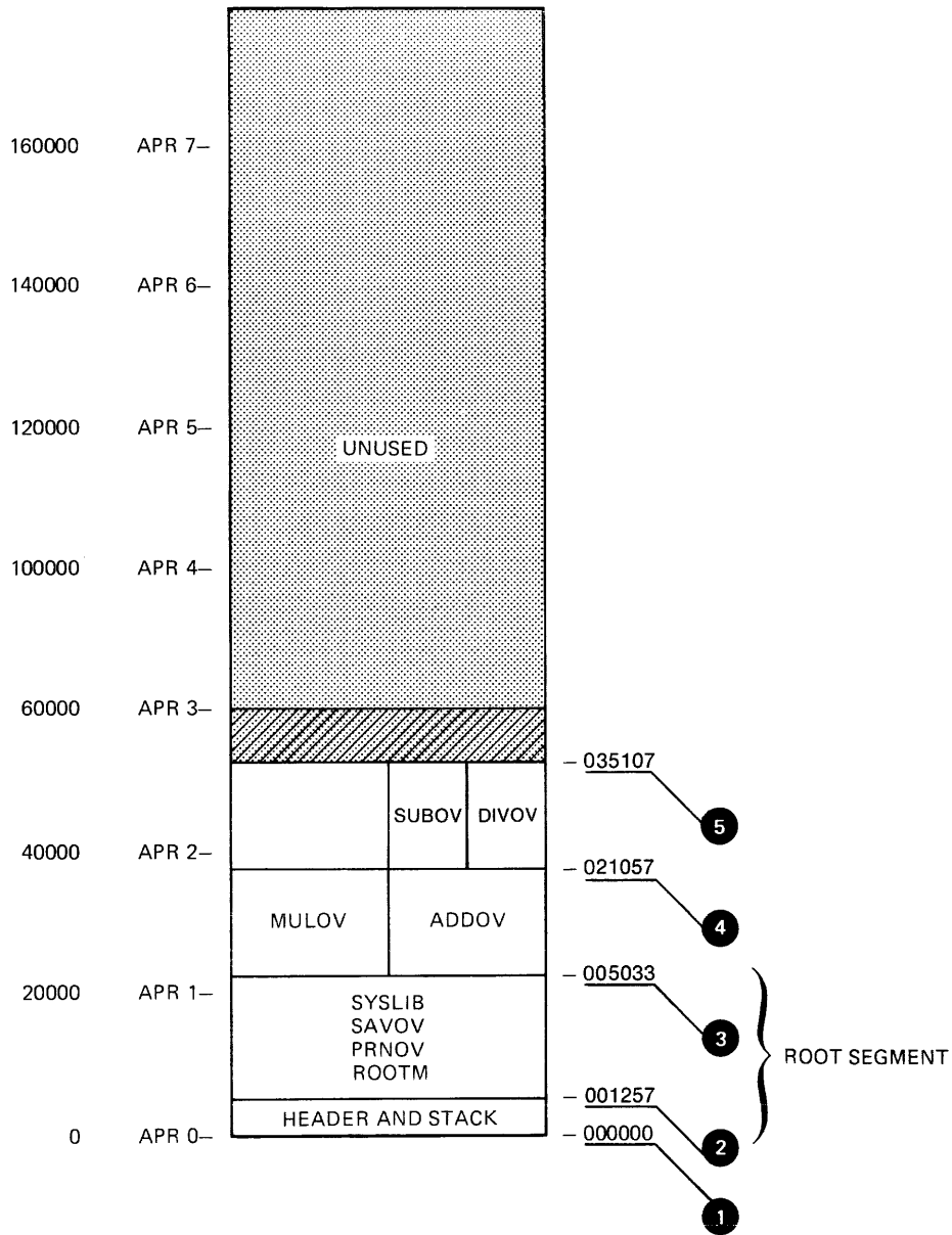
Figure 3-21 Allocation of Virtual Address Space for OVR.TSK
