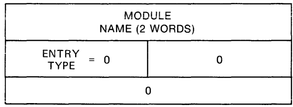
Figure A-3 Module Name Entry Format
