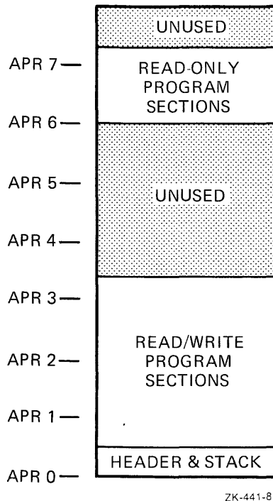
Figure 9-1 Allocation of Program Sections in a Multiuser Task
