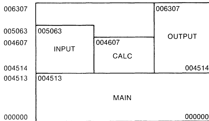
Figure 7-7 Memory Allocation Diagram for MAIN.TSK
