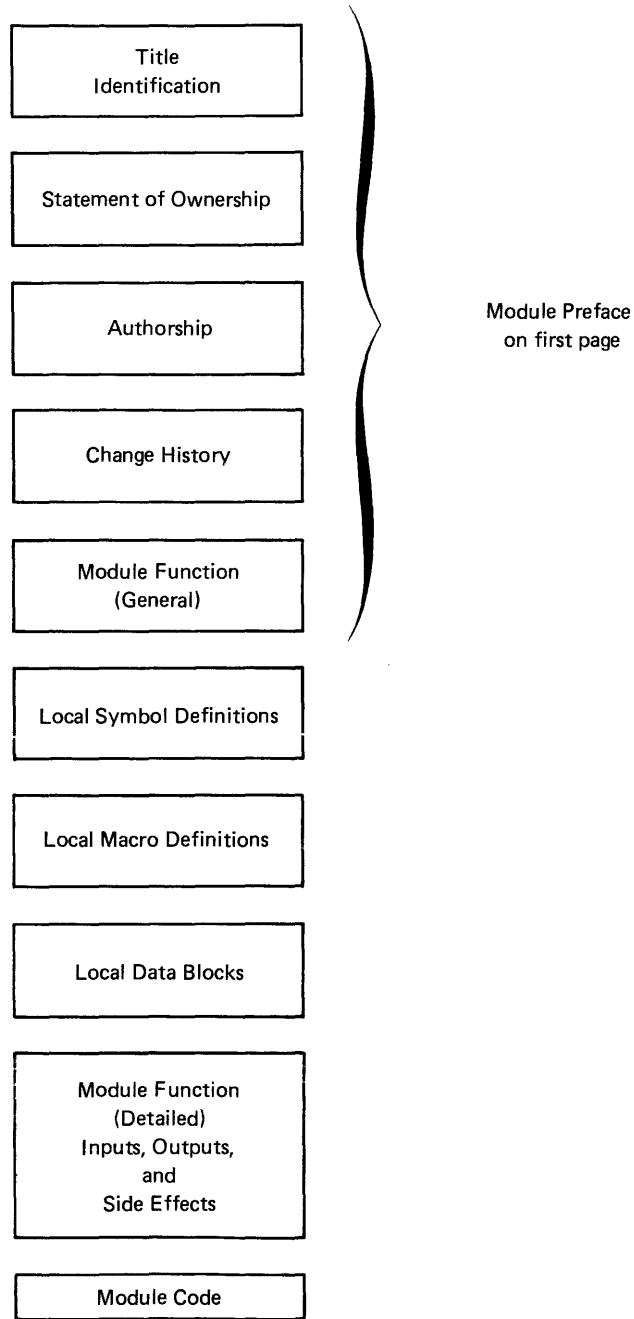
Figure 2-1 MACRO-11 Source File Format
