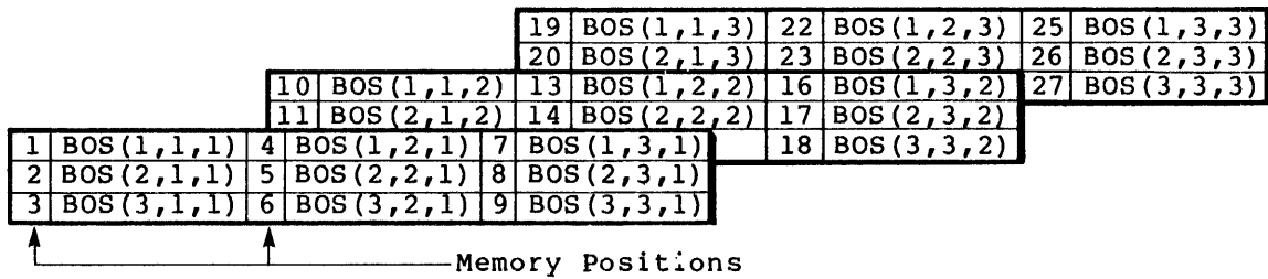
Figure 2-1: Array Storage
