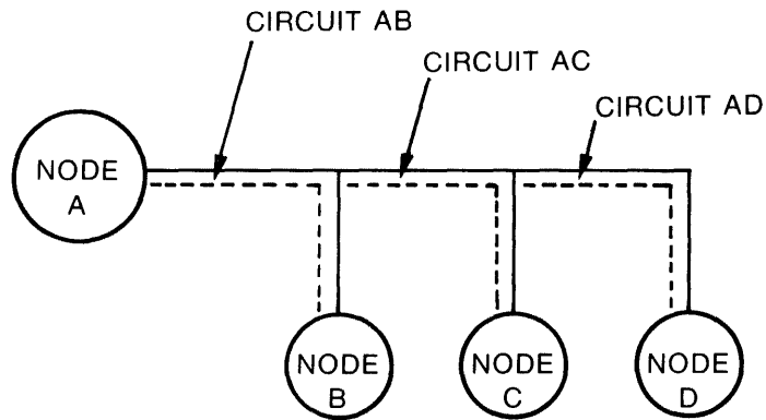
MULTIPOINT CONNECTIONS
