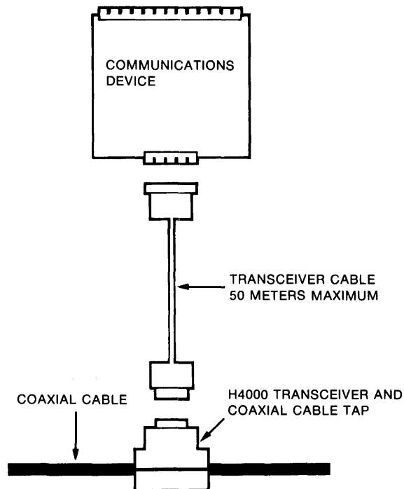
Figure 3-4: Ethernet Hardware
