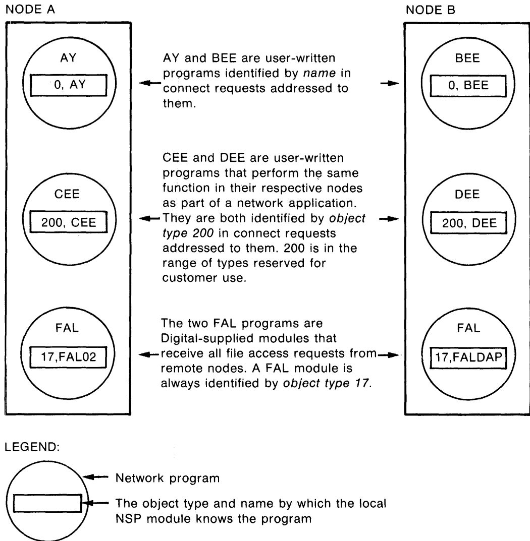
Figure 5-1: Addressing Network Objects
