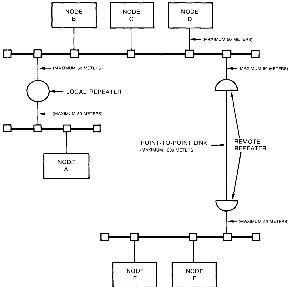
Figure 3-6: Repeaters
