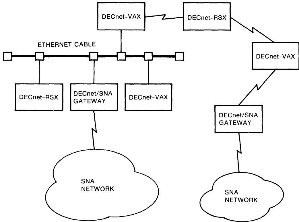
Figure 8-3: DECnet/SNA Environments
