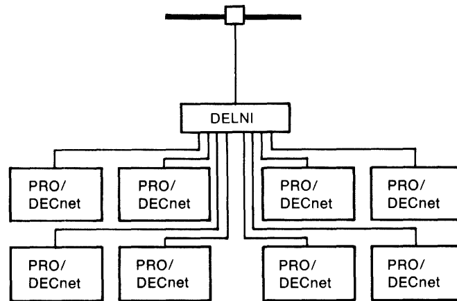
Figure 3-5: DELNI
