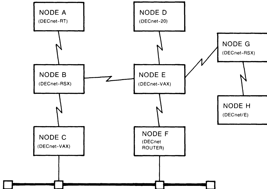
Figure 3-7: Node Routing Capabilities
