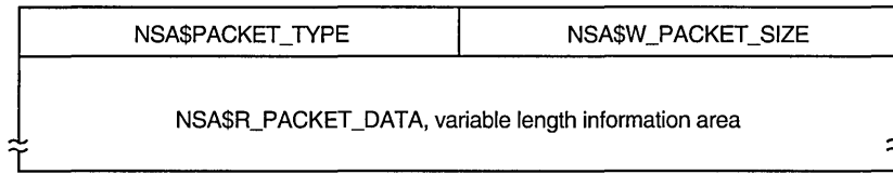
Figure G-2 Audit Data Packet Format
