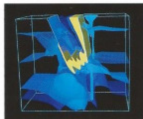
Simulation of gold mine historical mining sequence. Images show how mine safety factors change as ore is removed. The blue vertical shaft represents the mine shaft, while the yellow portion represents the home stake formation gold-bearing body.
