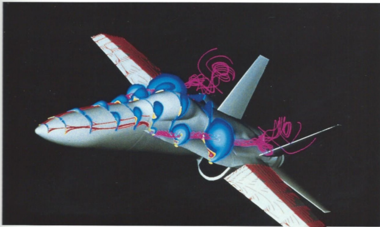
F-18 aircraft flowfield visualized using surface flow patterns, off-surface particle traces, and helicity density contours.
