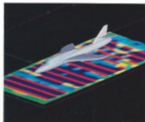
Electric field intensity around a military aircraft. The figure shows the variation (red is negative and blue is positive) of the vertical component of the electric field throughout a plane close to a military aircraft. Results obtained by EMMA T2 code. PATRAN has been used for preprocessing and visualization is via AVS.
