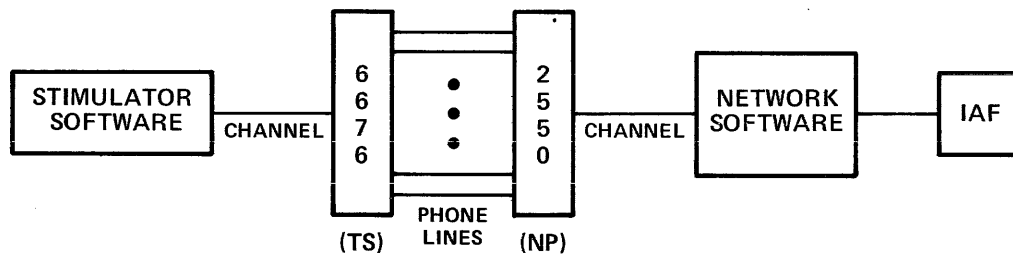
Figure 4-3. Hardware Configuration for NSTIM
