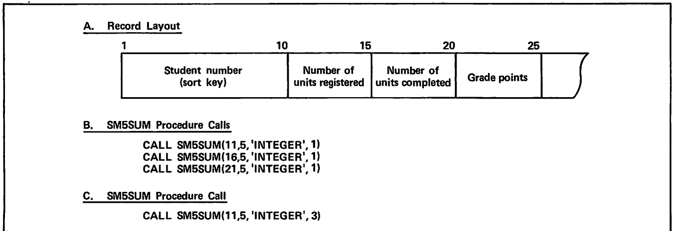
Figure 5-18. SM5SUM Procedure Call Example
