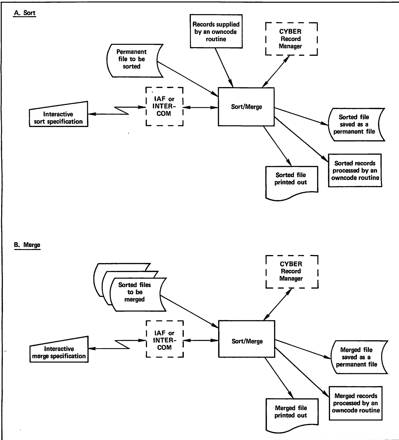
Figure 1-2. Interactive Job Flow
