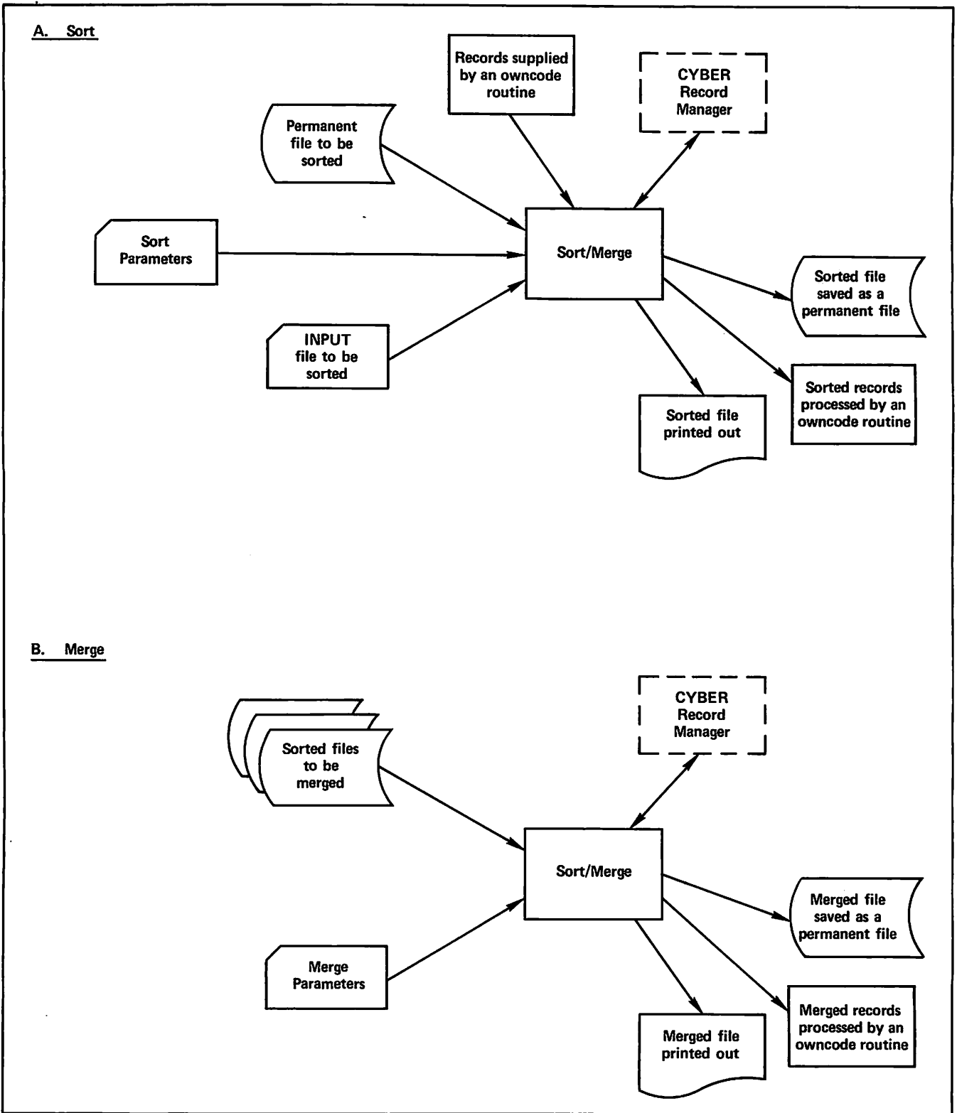
Figure 1-1. Batch Job Flow
