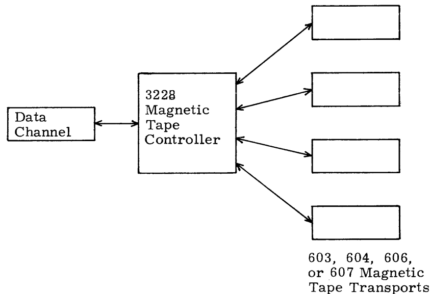
Figure C-1. Typical Configuration
