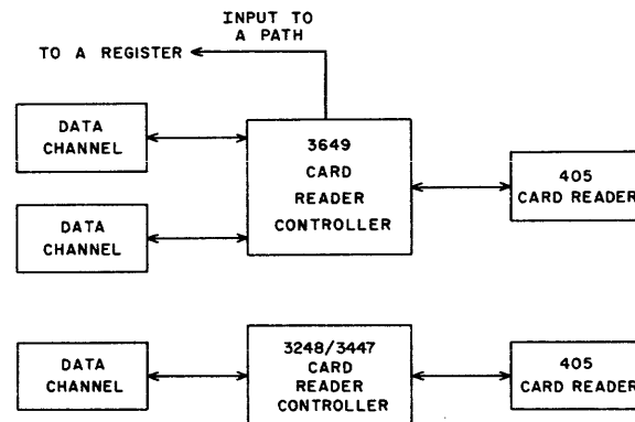
Figure C-1. Typical Configurations
