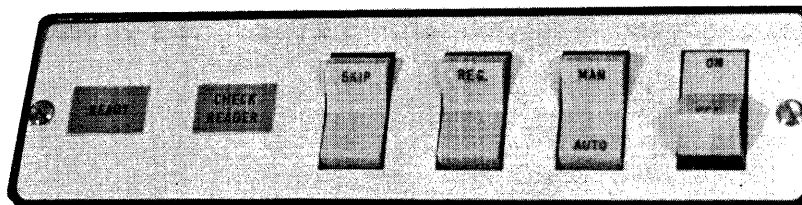
Figure D-3. NCR EM-D2 (PE) Card Reader Switches and Indicators
