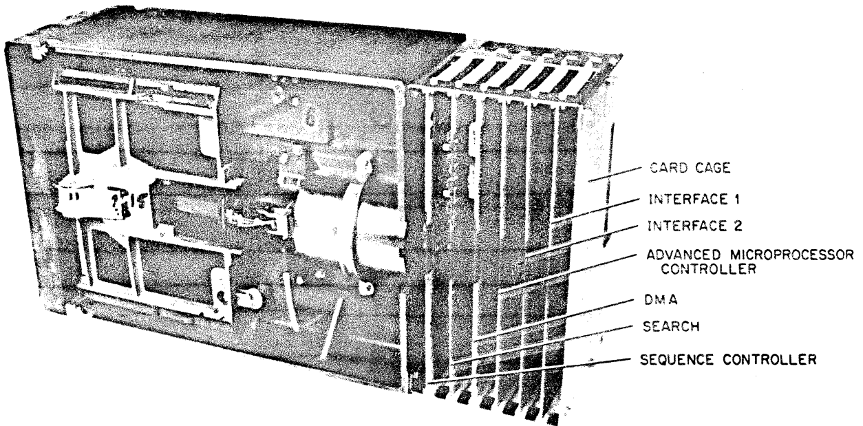
Figure 3. Drive - Right Side View
