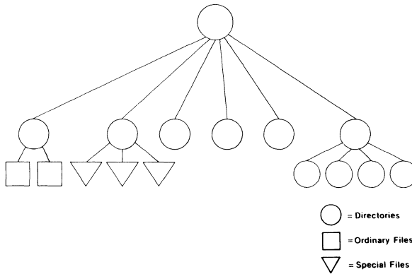
Figure 1-3: The Hierarchical Structure of the File System
