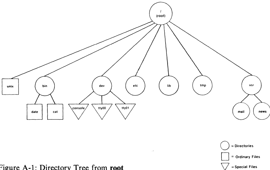
Figure A-1: Directory Tree from root
