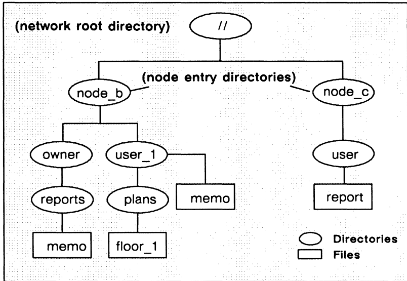
Figure 1-2. A Sample Naming Tree
