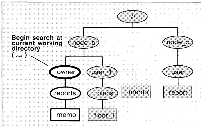
Figure 1-6. A Sample Path Beginning at the User's Home Directory
