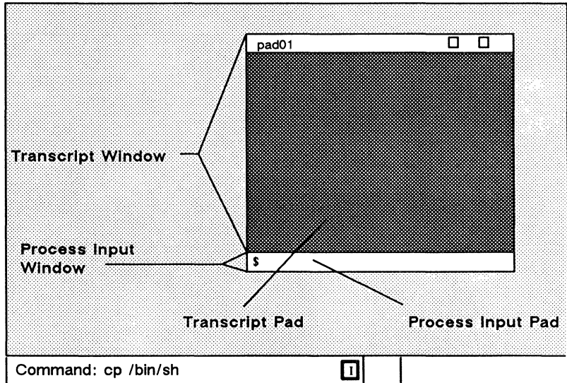
Figure 5-1. A Process Running the Bourne Shell
