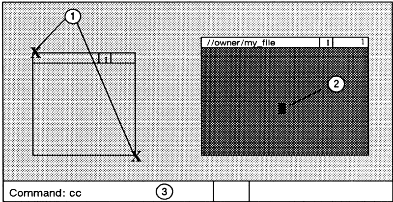
Figure 5-3. Copying a Pad and Window
