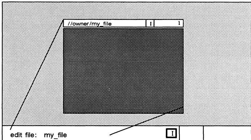
Figure 5–2. Creating an Edit Pad and Window
