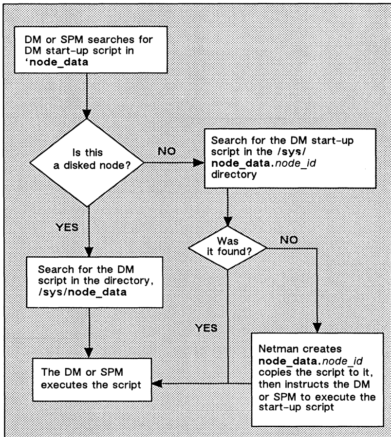
Figure 3-4. The Start-Up Script Search Sequence
