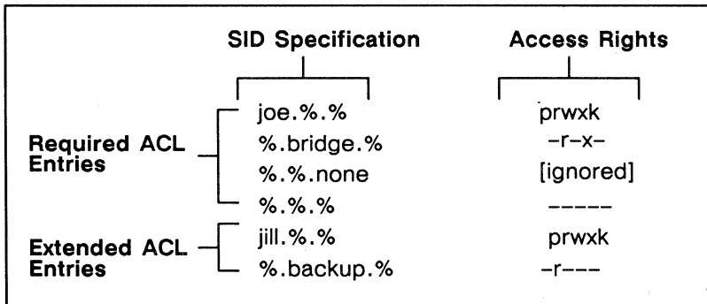
Figure 1-3. Sample Extended ACL Entries
