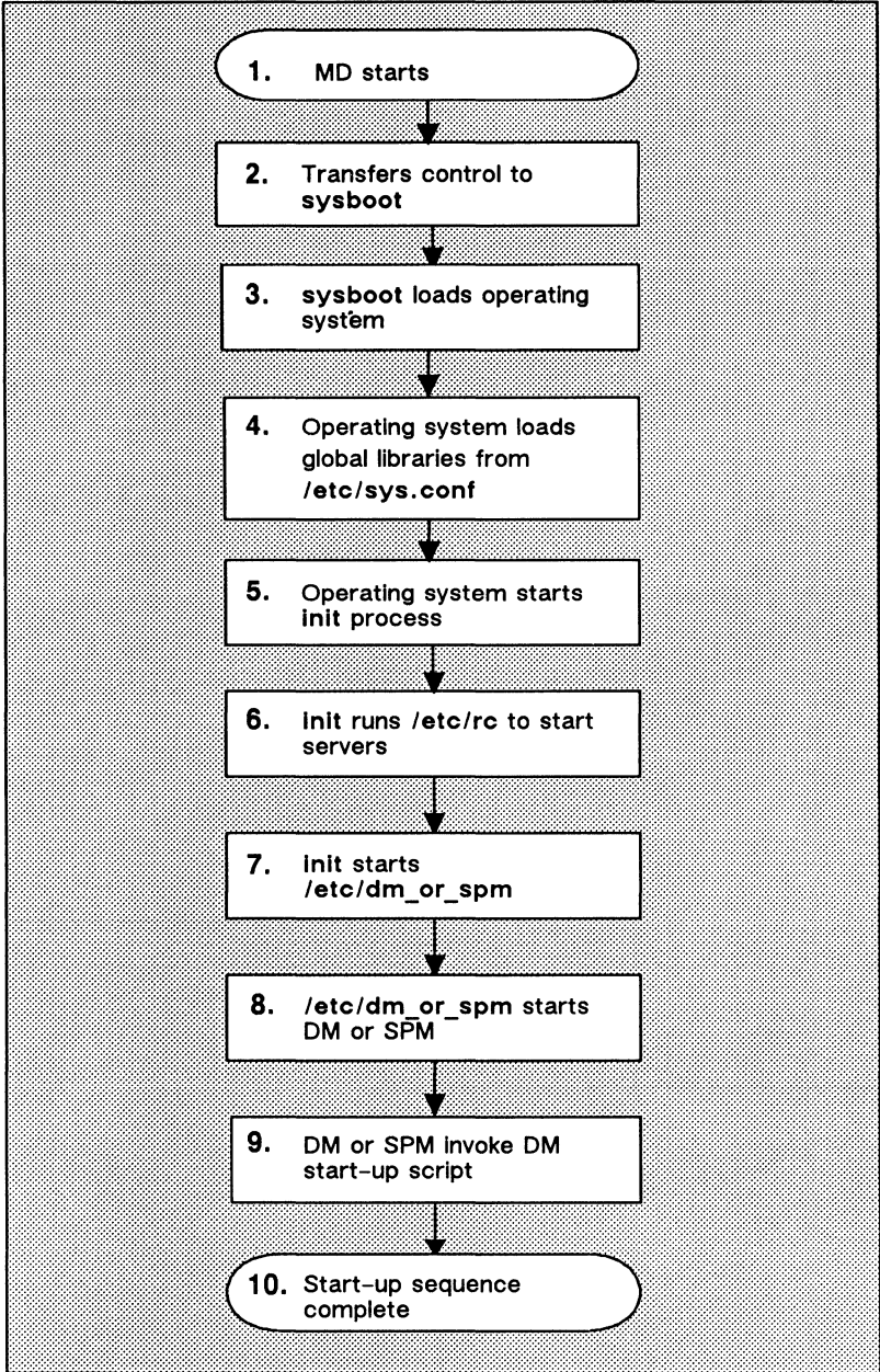
Figure 3-1. The Start-Up Sequence for Disked Nodes
