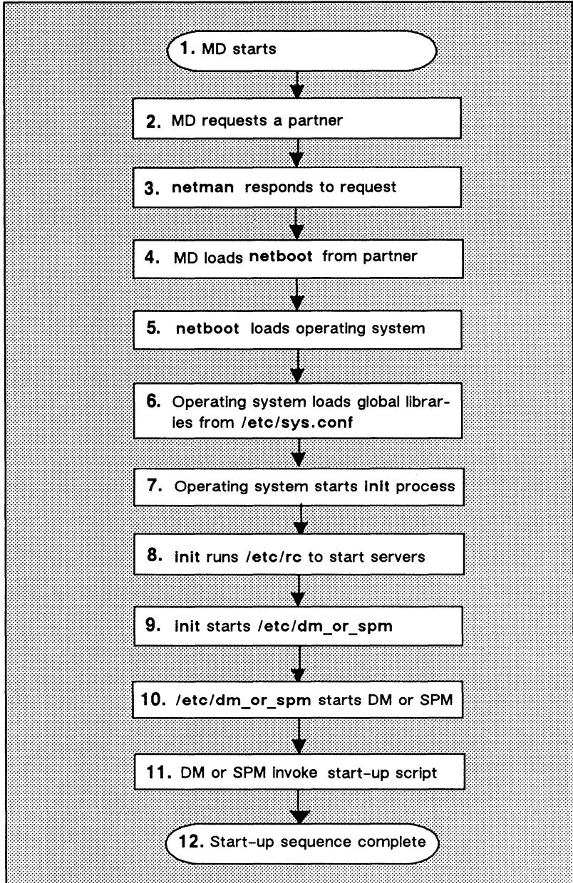
Figure 3-3. The Start-Up Sequence for a Diskless Node
