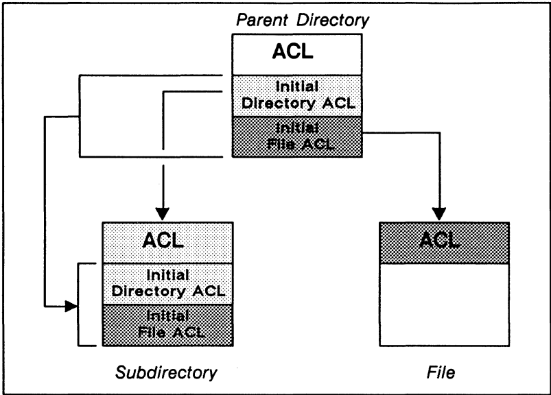
Figure 1-5. Initial ACLs for Files and Directories
