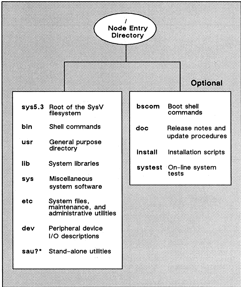
Figure A-1. The Node Entry Directory ( / ) and Subdirectories
