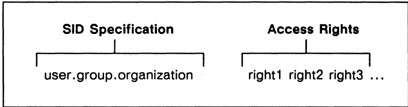
Figure 1-1. Structure of an ACL Entry
