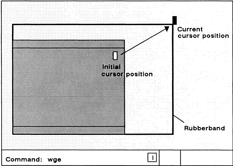
Figure 5-4. Growing a Window Using Rubberbanding
