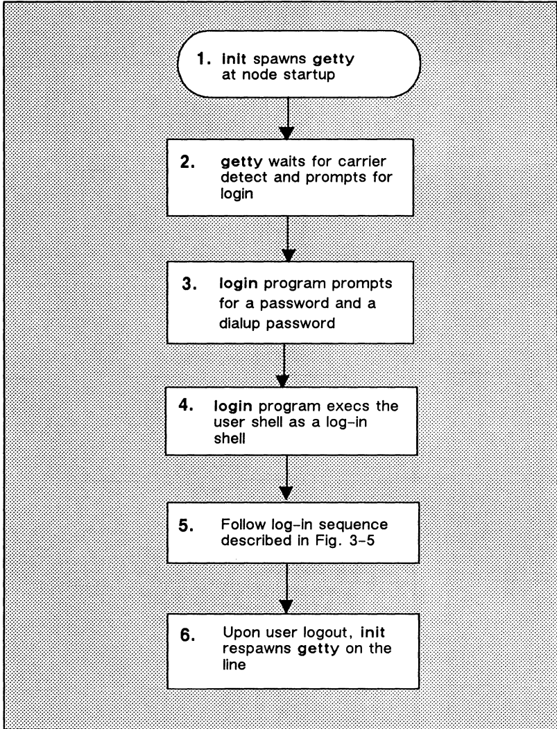
Figure 3-8. Login Over a Dialup Line
