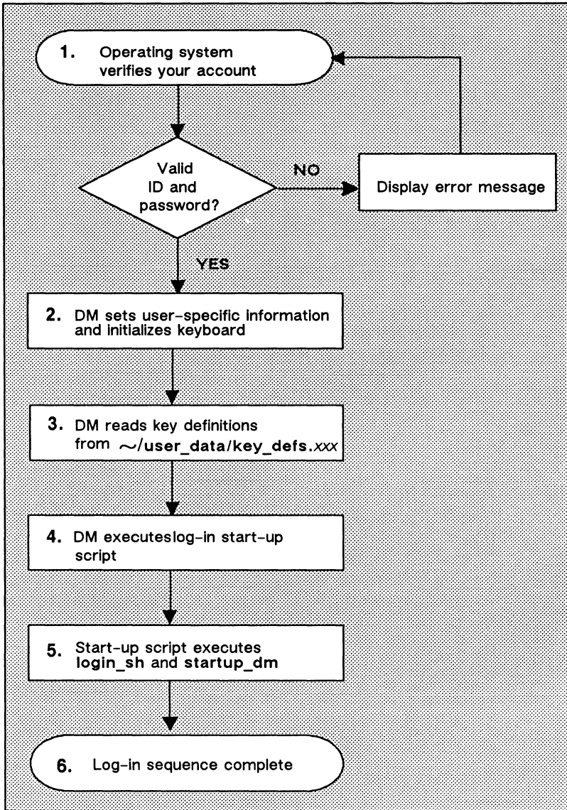
Figure 3-5. The Log-In Sequence
