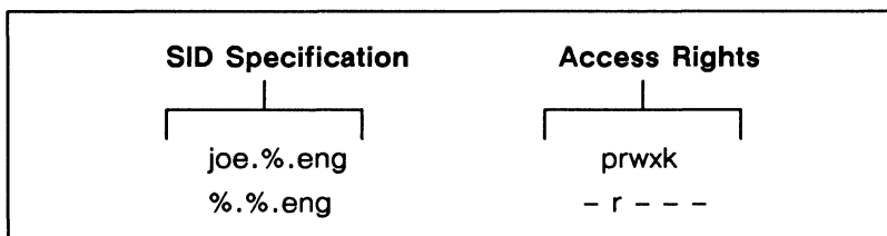
Figure 1-2. Sample ACL Entries
