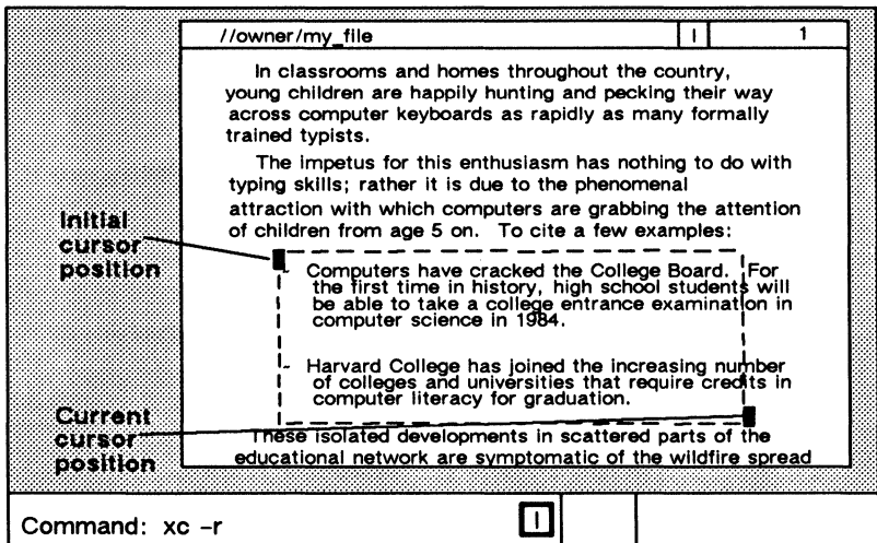
Figure 6-3. Copying Text with the xc -r Command
