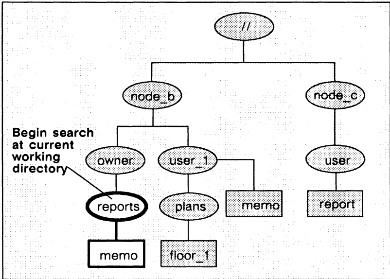
Figure 1-5. A Sample Path Beginning at the Current Working Directory
