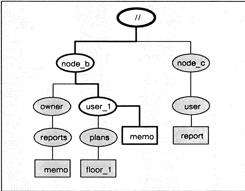
Figure 1-3. A Sample Path Through the Naming Tree
