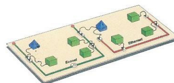
Econet and Ethernet clusters linked via a gateway (fileserver on Ethernet cluster)
