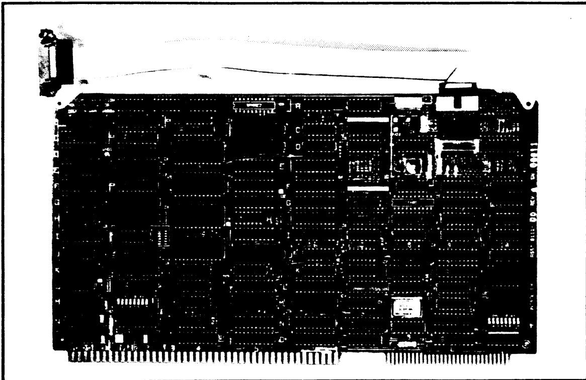
FIGURE 1-1. 3COM MULTIBUS ETHERNET CONTROLLER BOARD SET
