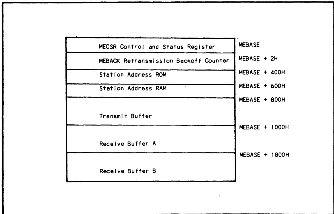
FIGURE 4-1. ME BUFFER ORGANIZATION 8K BYTES, ADDRESSES IN HEX
