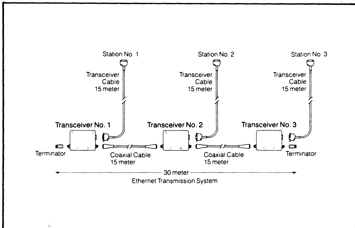
FIGURE 2-2. 3COM ETHERNET TRANSCEIVER STARTER PACKAGE
