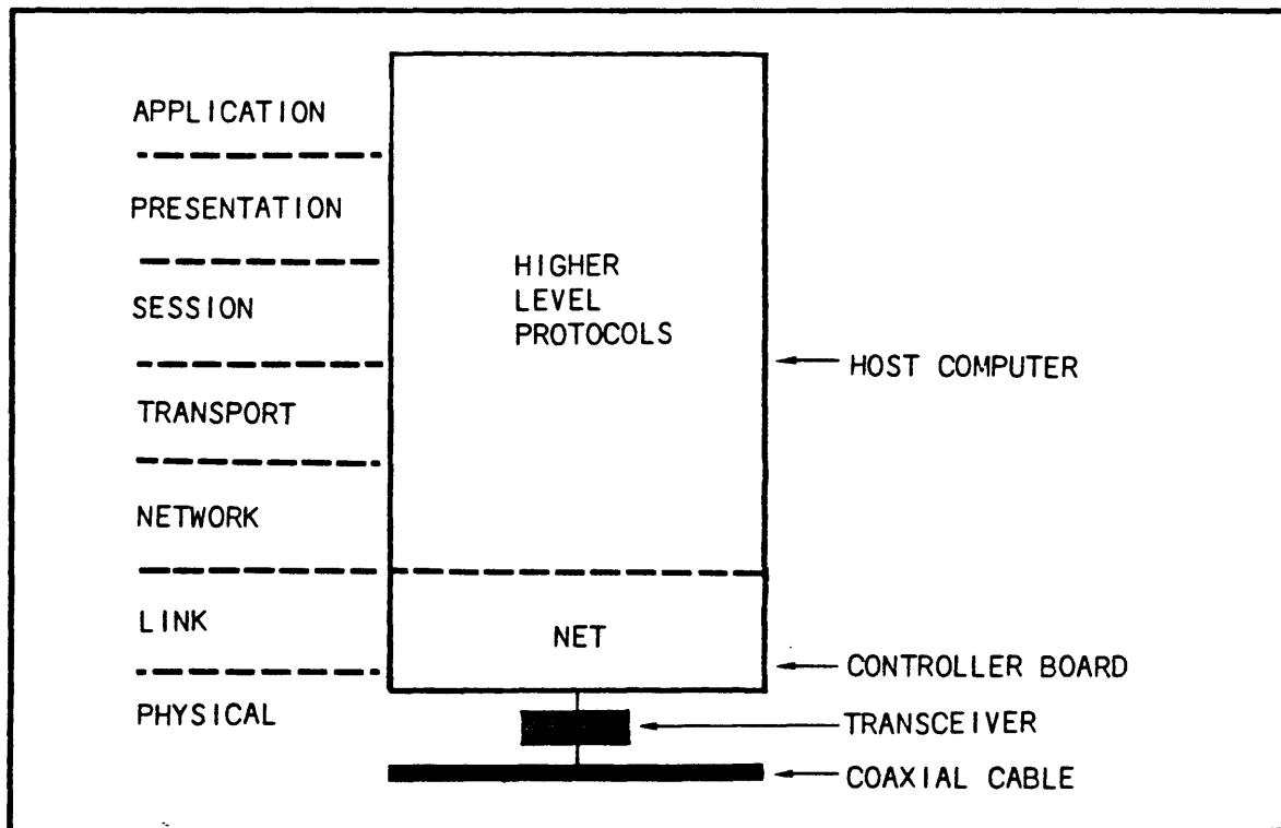
FIGURE 3-1. ISO PROTOCOL HIERARCHY
