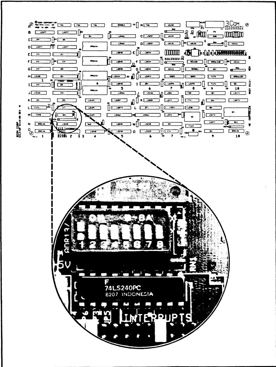
FIGURE 5-3. ADDRESS SWITCHES ADR13/ TO ADR0D/ AND TRB SWITCH
