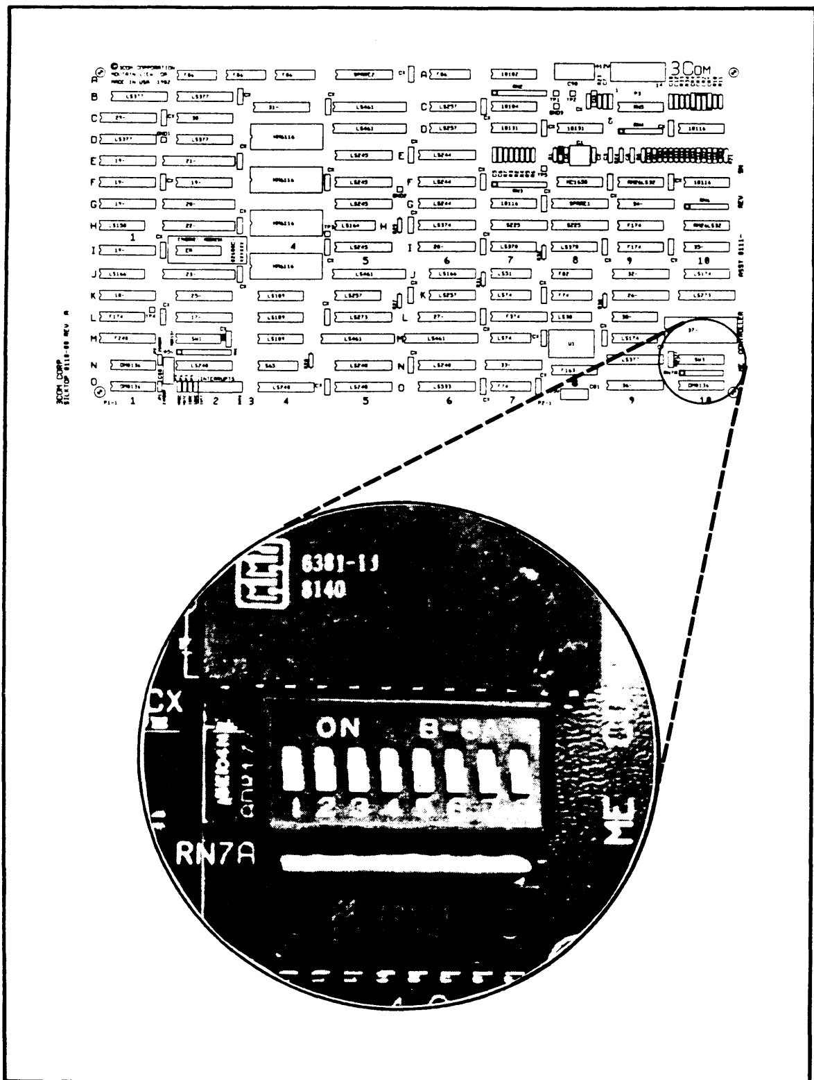
FIGURE 5-4. ADDRESS SWITCHES ADR17/ TO ADR14/
