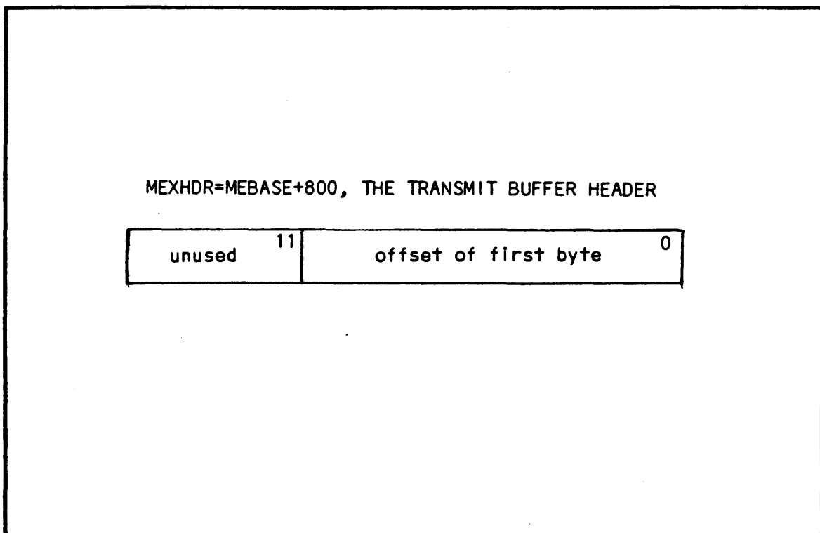
FIGURE 4-3. MEXHDR=MEBASE+800, THE TRANSMIT BUFFER
