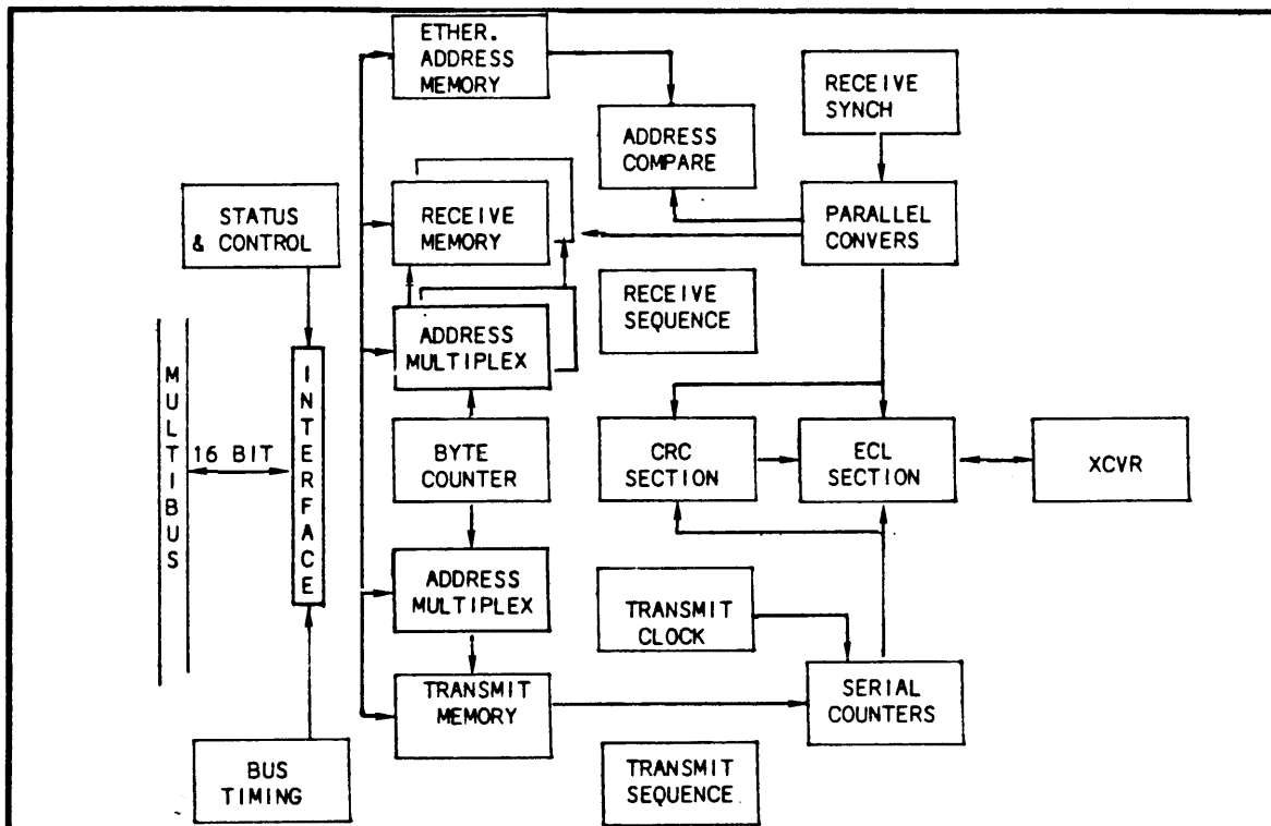
FIGURE 3-3. ME CONTROLLER FUNCTIONAL BLOCK DIAGRAM
