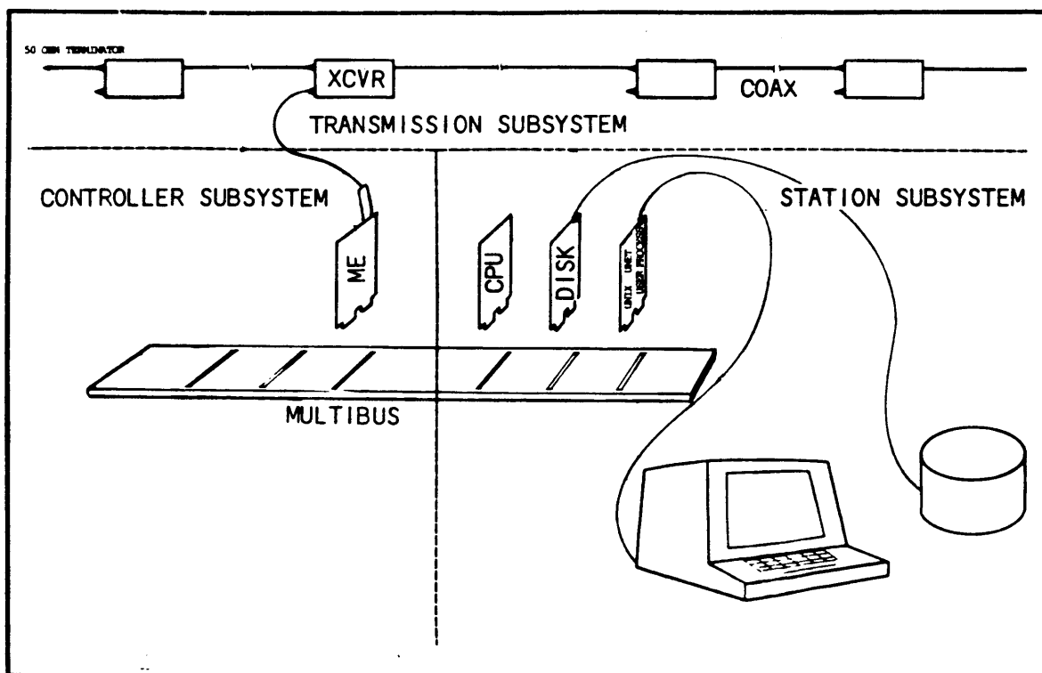
FIGURE 2-1. BASIC ETHERNET SUBSYSTEMS
