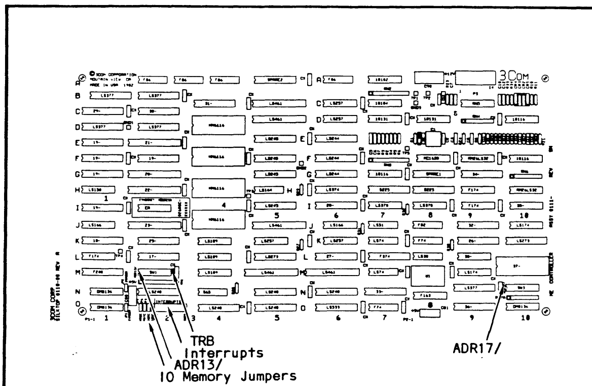
FIGURE 5-2. ME CONTROLLER BOARD LEGEND
