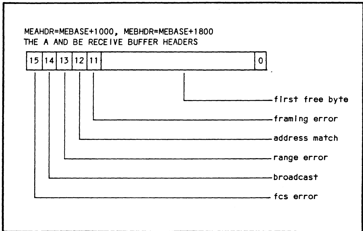
FIGURE 4-4. A AND B RECEIVE BUFFER HEADERS
