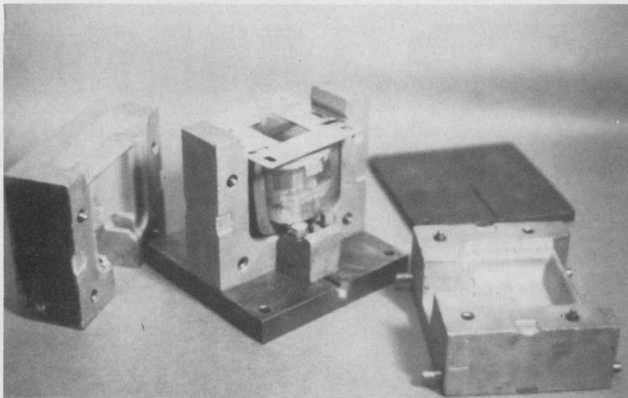
Unlike potting, casting requires no outer case. Typical is this five-piece mold, which is removed after the embedding material cures. The component, protected by the resin, needs no other housing.
