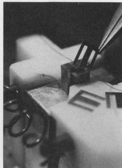
tion. Here skilled operators, using microscopes of 10 to 30 power magnification, are stacking tiny laminations in the bobbin of a Bourns 1/4-in.-cube transformer.
