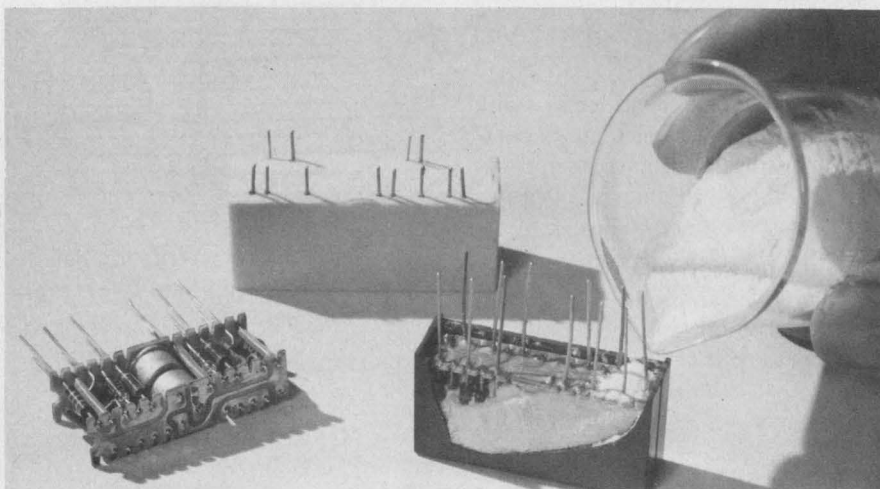
Some epoxies come in powder form, such as this one-part Eccofoam EFF-14 from Emerson & Cuming. The material is vibrated into place and cures to a fine-structured foam with a density of about 15 lb/ft 3 .
