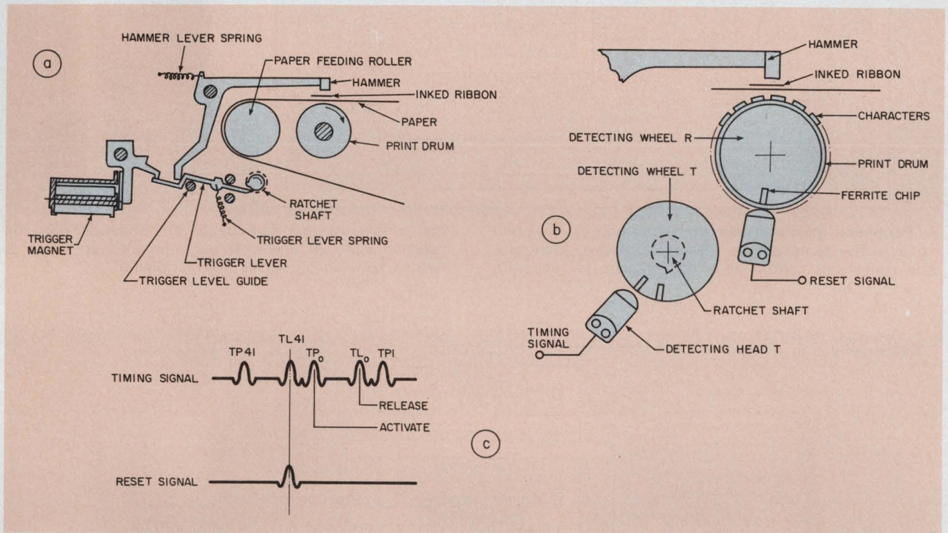
2. Column printers provide inexpensive hard copy. A drum printer requires timed signals to a trigger magnet (a). And magnetic pickups supply timing information to the controlling device (b). The timing signals indi-
