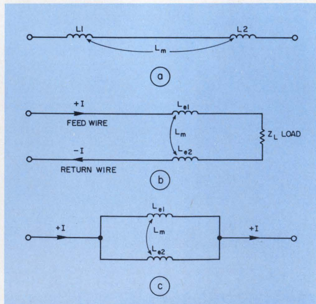
1. In calculating the inductance between wired points in a circuit, you must take into account the mutual inductance (a) to nearby current paths, such as a return path (b) or between parallel feed paths (c).
