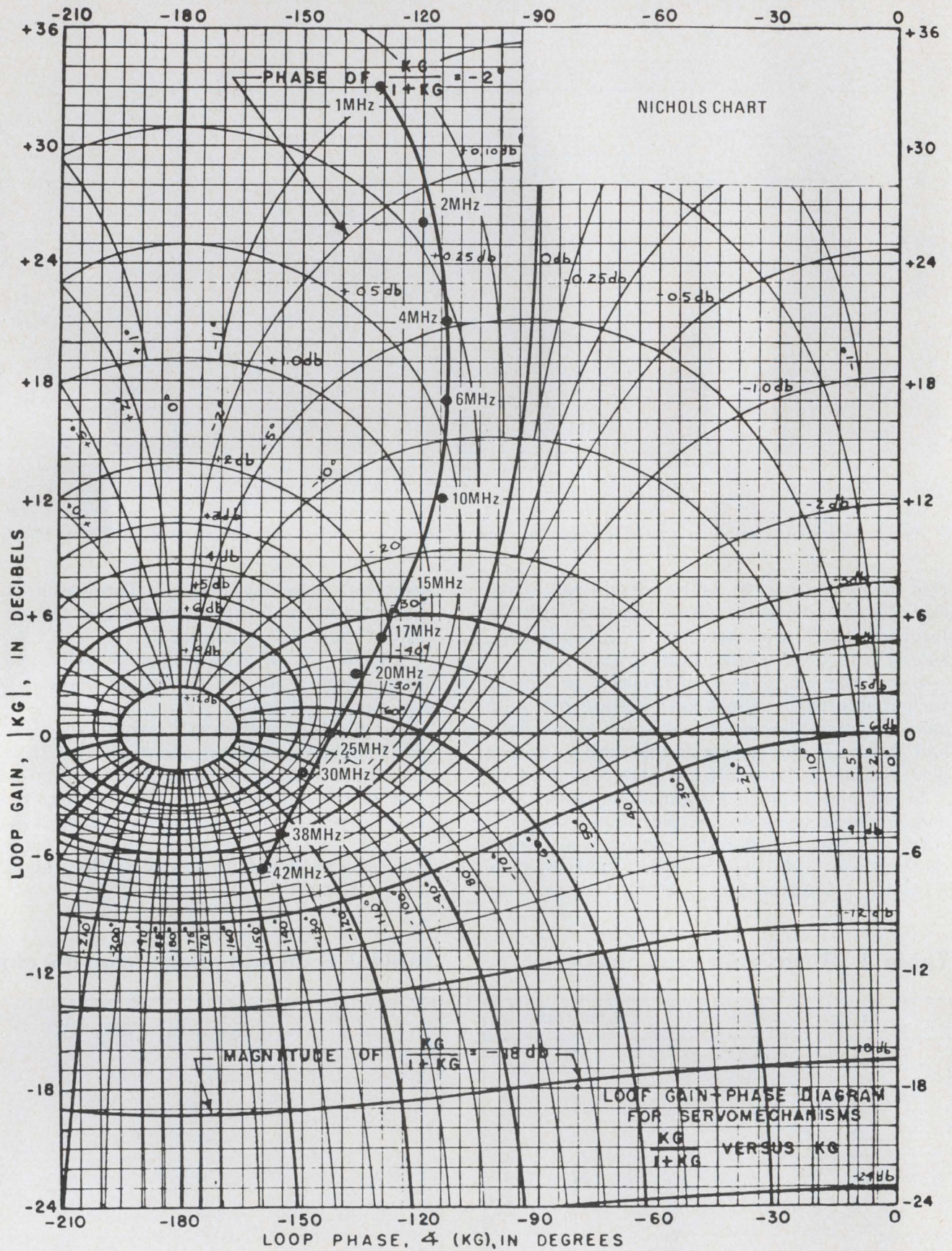
3. A plot of function GH/(1+GH) on the Nichols Chart. The curve defines performance of the amplifier under
