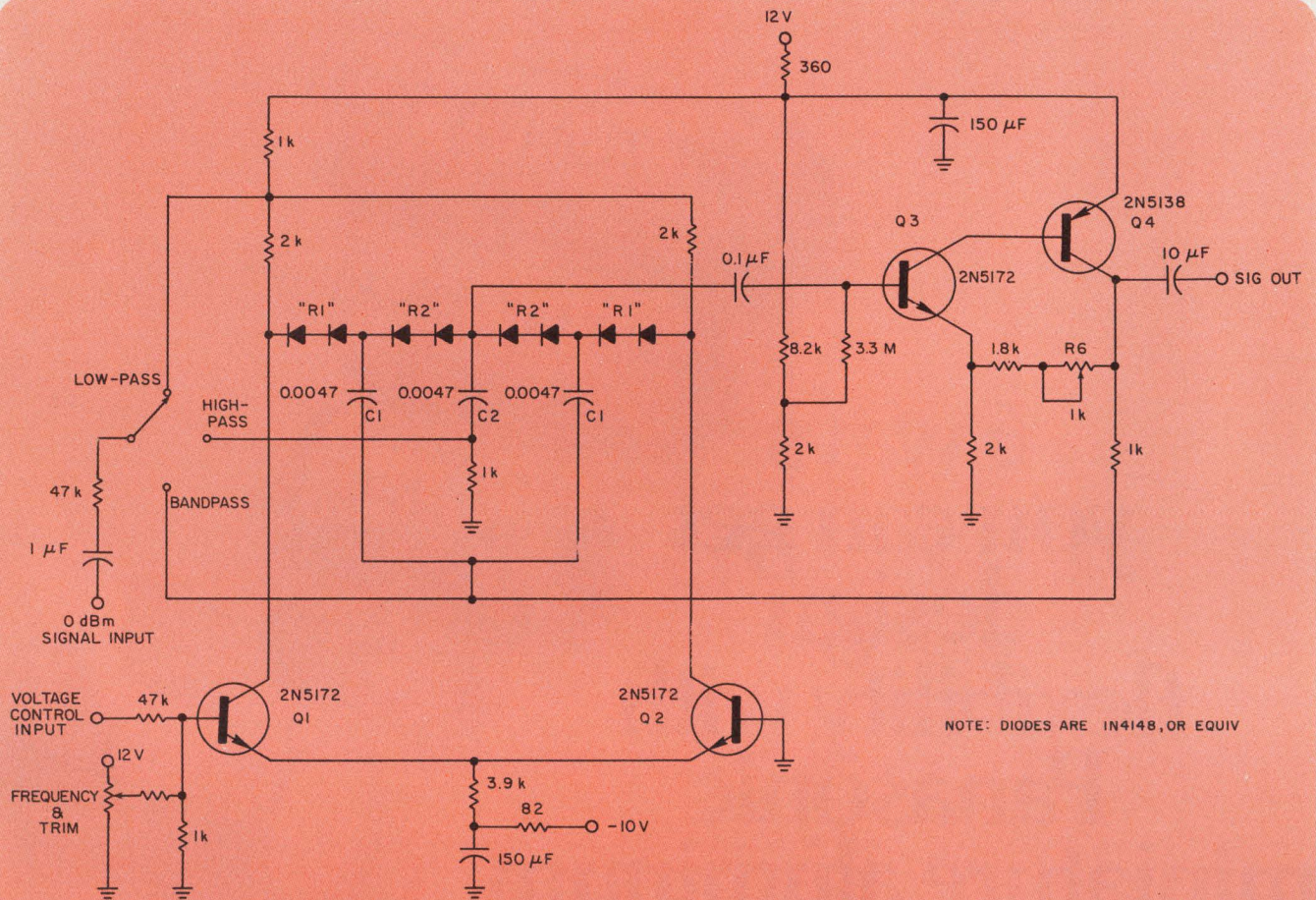
2. The Q of the voltage-tuned active filter is adjusted by R_6 . The Q remains almost constant over
