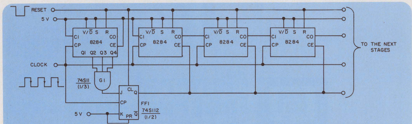
1. Schottky flip-flop FF_1 and AND gate G_1 increase the maximum frequency of cascaded 8284 count-
