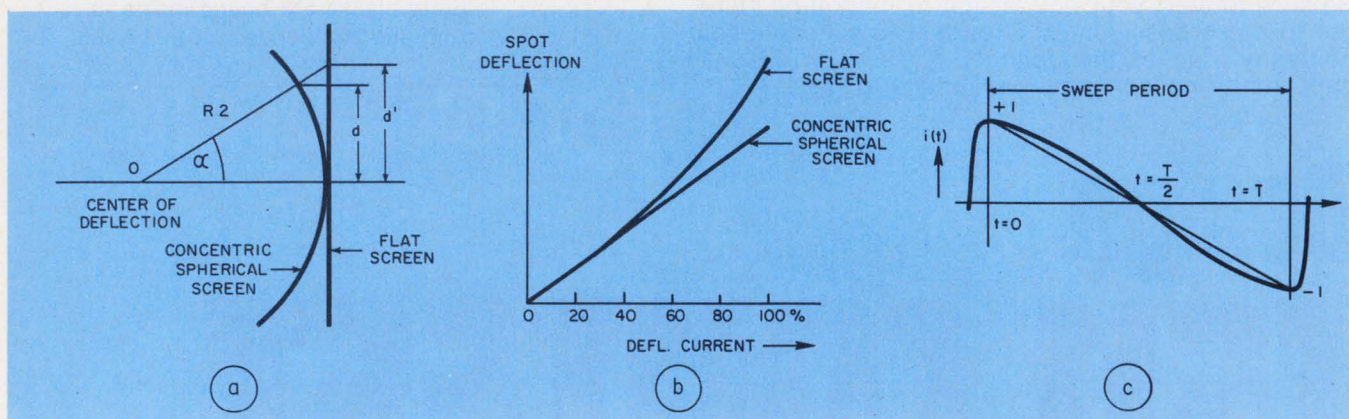
1. Large linearity errors caused by radius changes, occur in CRTs that have any screen other than a sphere (a). The nonlinearity in the spot deflection is illustrated
