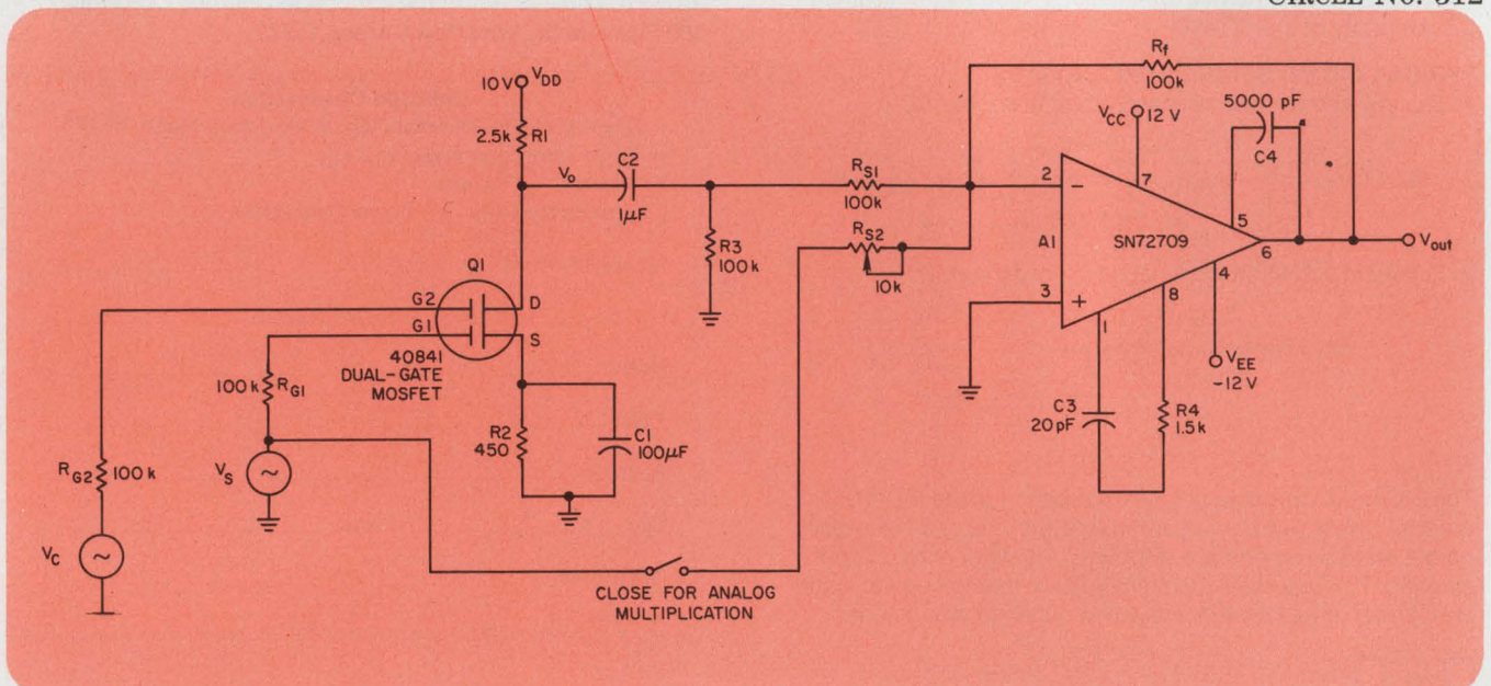
The drain circuit of MOSFET Q_1 contains the product of signal voltage V_s and control voltage V_c .
