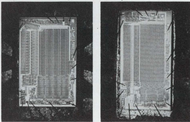
Twice the memory capacity at no increase in chip area. At left is a photo blow-up showing the circuit density of a typical Harris 1024 PROM. At right is our new HPR0M-2048, fabricated through use of our Poly-planar process, demonstrating isolation to isolation spacings half that of conventional devices and yielding a 4/1 improvement in density.
