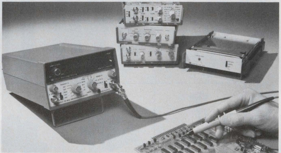
Measuring system typifies current trends in instrument design: LSI circuitry, solid-state displays, small size and easy servicing.
