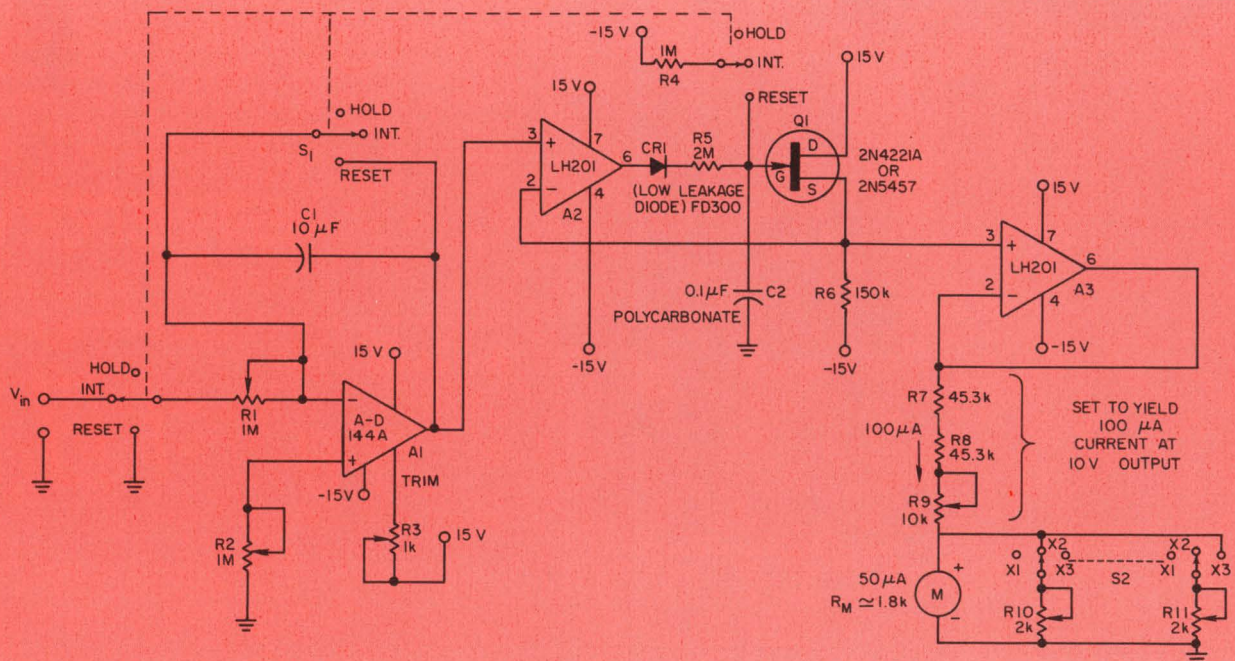
The peak value of the integral of the input voltage is read out directly on the microammeter, M,
