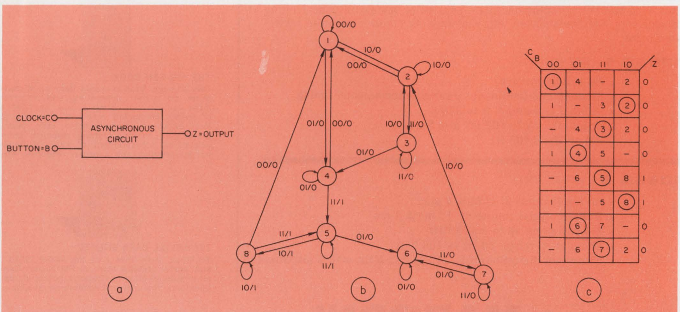
1. A single clean clock pulse passes from the clock input to the output of the asynchronous circuit (a) every time the button is pushed. This operation is de-
