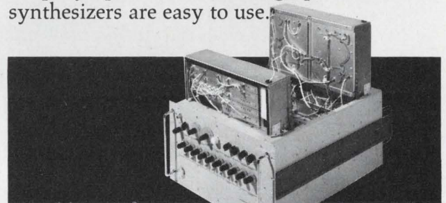
Model 645M with swing-out trays opened to demonstrate access to modular circuitry.
