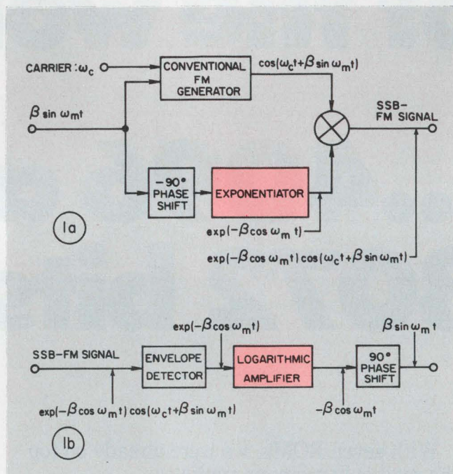
1. High-modulation indexes are difficult to obtain in SSB-FM because they require that the exponentiator in the generator (a) and the logarithmic amplifier in the detector (b) have very large dynamic ranges. For \beta=2 , for example, the required dynamic range is 34 dB.
