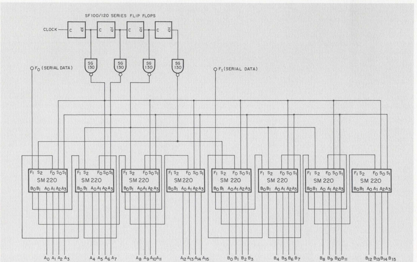
Fig. 4. SM-220 used as a serial-to-parallel converter.
