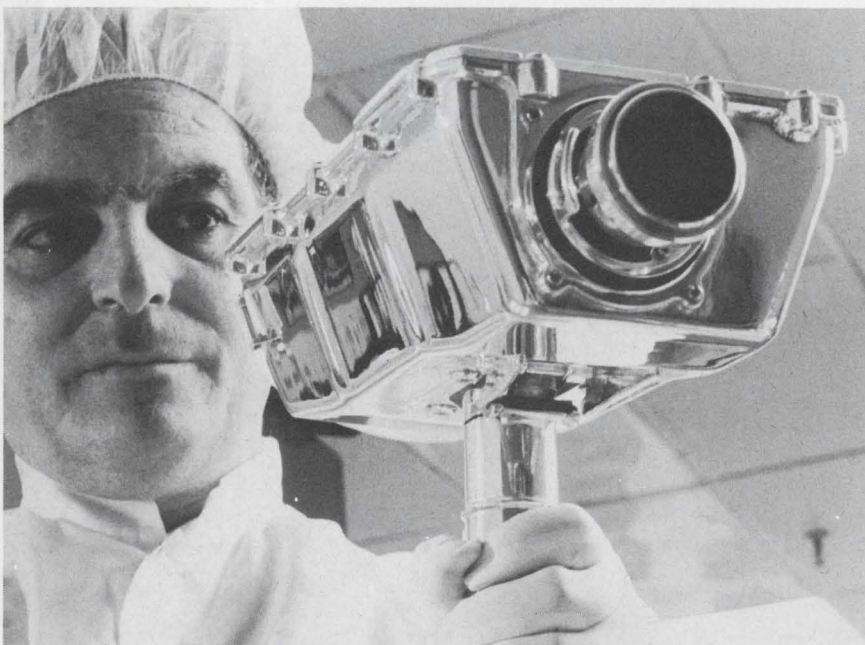
Westinghouse 7-1/4-pound moon camera passed its first flight test in Apollo 9. It uses a SEC tube for adaptability to changing light conditions.
