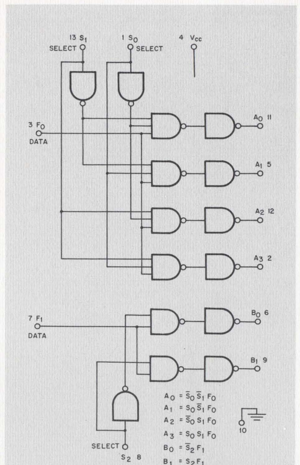
Fig. 3. Logic arrangement of SM-220 demultiplexer.
