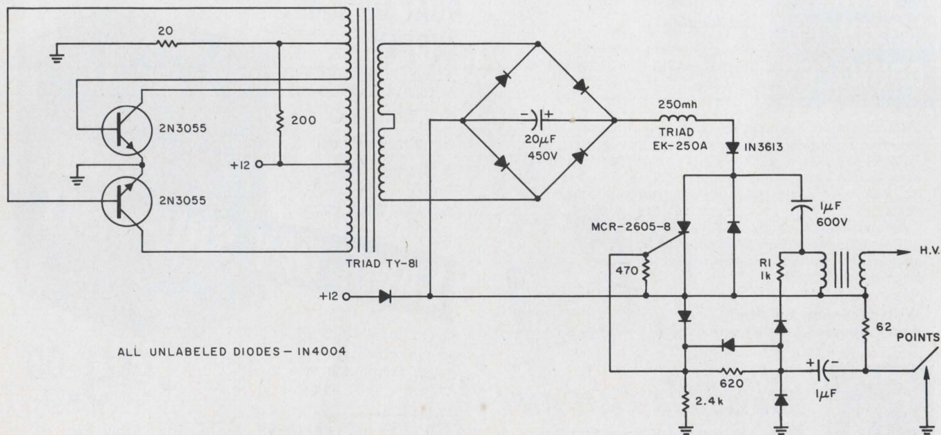
2. Complete ignition system using the resonant-charging technique provides an output voltage of 55,000 V.
