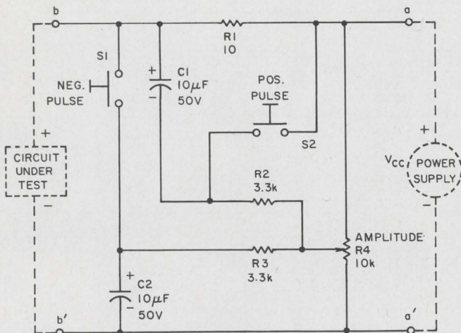
1. Positive transients are produced by switch S2 and negative transients by S1 . The amplitude of the transients is set by potentiometer R_4 .
