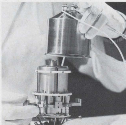
Thruster subsystem of electric ion engine is given final adjustment.
