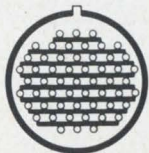
55 #23-22 contacts, #16 shell. Area—1.58 sq. in. Weight—.9 oz.
