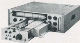
Model 6151 shown with plug-in drawer capable of holding all dc to 1 Gc oscillators.
