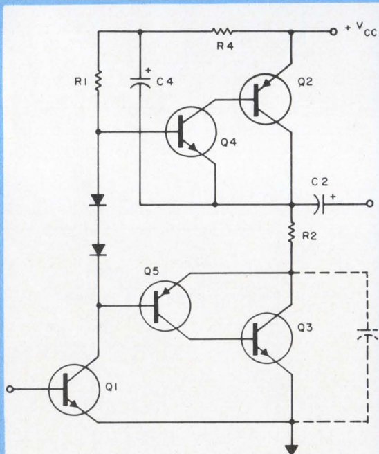
9. Negative peak voltage loss is reduced by changing Q 5 and Q 3 into an inverted Darlington, too. High-frequency parasitic (12-MHz) oscillations can be eliminated by connecting a small (0.1-μF) capacitor across Q 3 (dashed lines). This completely corrects the problem without affecting normal amplifier operation in any way.
