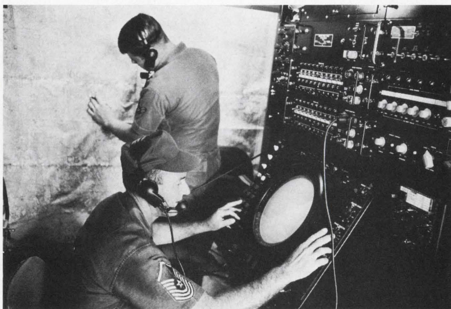
The radar operator inside the AN/TSQ-61 van spots approaching aircraft on the AN/TPS-44 search radar's remote indicator and passes position data on to an assistant, who plots the coordinates.
