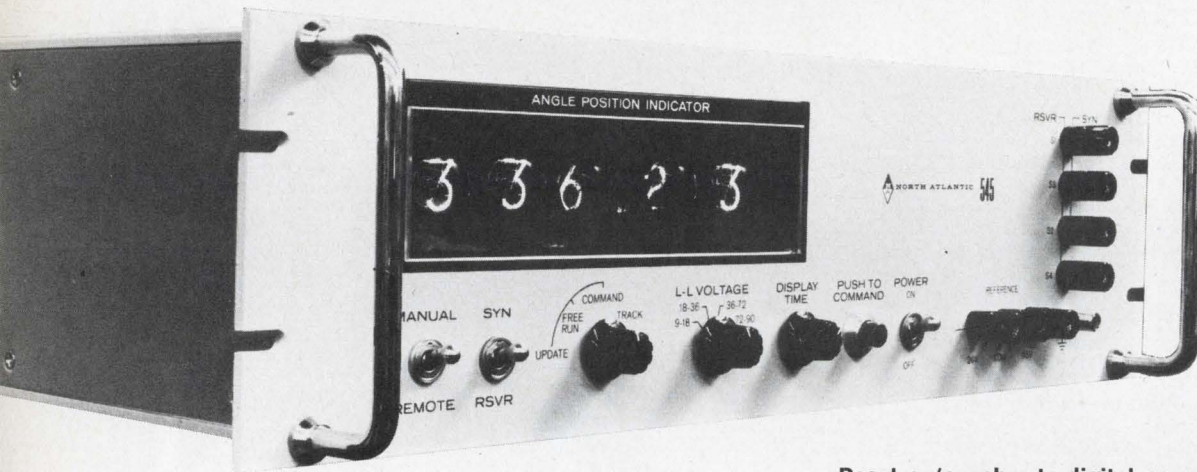
Resolver/synchro-to-digital converter tracks to 2000°/s. The six digit instrument has an updating time of 125 ms (for a 180° input step). In addition, the unit has a Velocity Constant of 20,000 to 1, a variable 0.3 to 3 second display time and three operating modes. Page U134.
