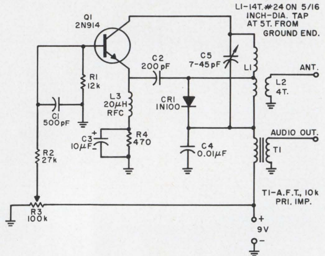
Residual oscillations are eliminated by adding a diode, CR1, to the conventional 27-MHz superregenerator. T1 is an audio transformer with 10-kΩ primary.
