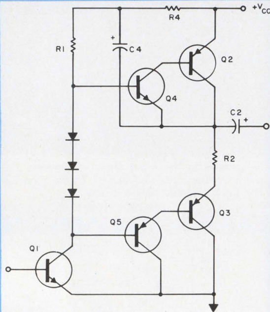
8. Using an "inverted Darlington," Q 2 and Q 4 , in the circuit of Fig. 7 results in further performance improvement. In addition to the increased gain (up to two orders of magnitude), the total positive peak voltage loss for Q 2 and Q 4 combined will be slightly greater than the emitter-base potential of Q 2 alone.
