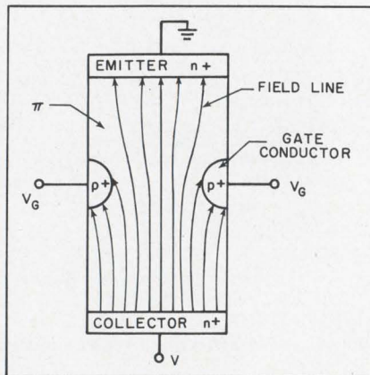
Fig. 2. Field lines in the JPL solid-state triode show its similarity to a thermionic tube. Field lines emanating from the collector terminate on the emitter and gate when V_G \leq 0 V.
