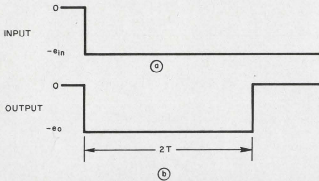
2. Input (a) and output (b) of the pulse shaper demonstrate the idea: the reflected voltage cancels the output after a time, 2T .
