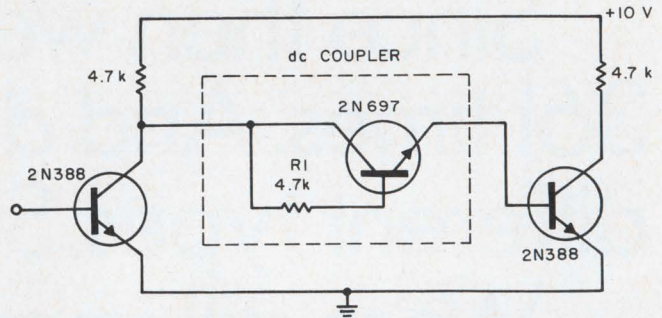
Dc coupling of transistor stages with a transistor and resistor simplifies dc amplifier design.
