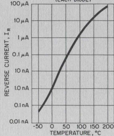
TYPICAL CHARACTERISTICS REVERSE CURRENT vs TEMPERATURE (EACH DIODE)
