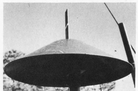
"Coolie hat," fabricated at Eglin Air Force Base, Fla., solved a poor uhf antenna pattern caused by an irregular ground plane. The irregularity was created by the hood of the jeep on which this AN/MRC-107 is mounted.
