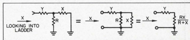
4. This circuit is the configuration that appears at any node in Fig. 3, up or down on the ladder. The terminating resistance, R_L in Fig. 3, has been replaced by X , to simulate an infinite series of sections.
