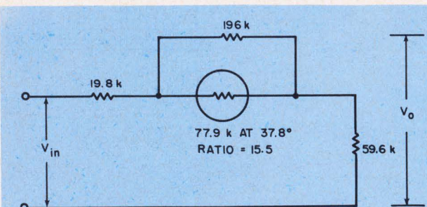
7. Normalized network is converted into a practical network by selecting an available thermistor and multiplying the normalized resistor values by the ratio of the actual thermistor's resistance to that of the normalized thermistor.
