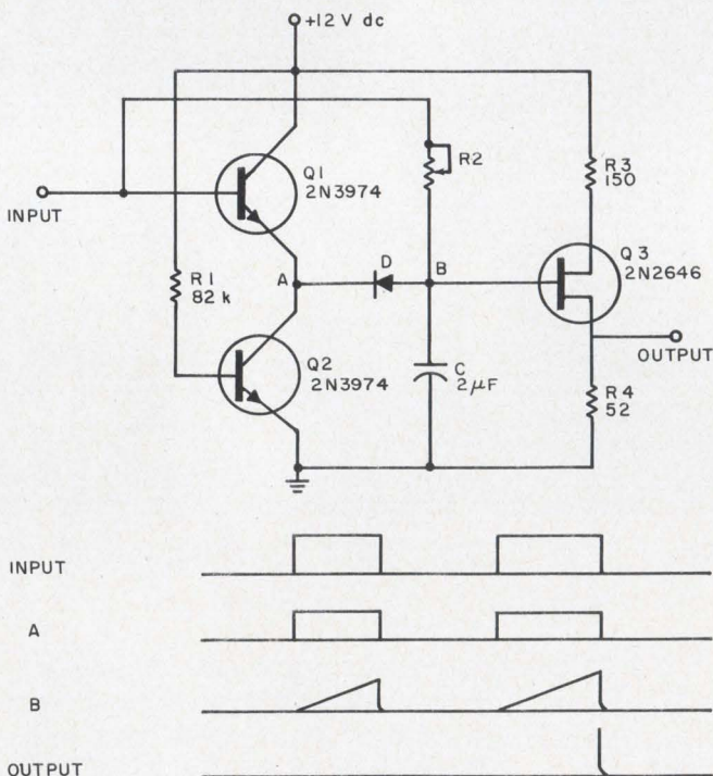
Output pulse is generated by the circuit only when the input pulse exceeds predetermined widths and amplitude. Value of C and the setting of pot R2 determine the minimum pulse characteristics required to produce an output.
