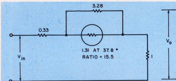
6. All resistance values are related to resistor R4 (value of 1) in the normalized network produced by the direct method of voltage-ratio-vs-temperature synthesis.
