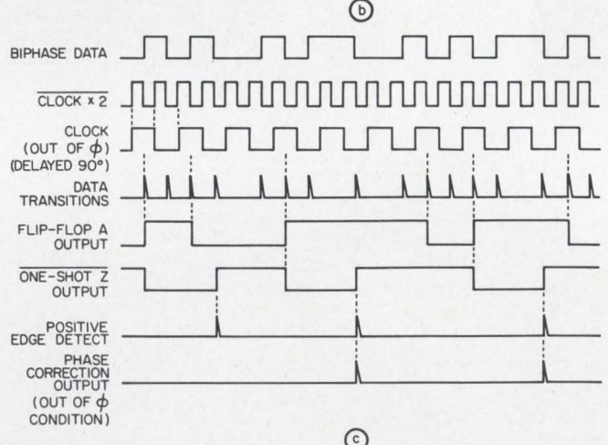
Clock phase correction for biphase PCM data is performed by the circuit shown in (a). Timing diagrams for in-phase and out-of-phase conditions appear in (b) and (c), respectively.
