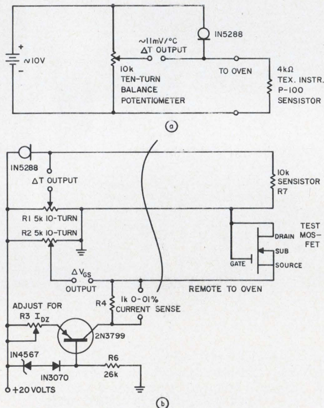
1. Simple temperature-monitoring circuit (a) is used to check p-channel enhancement MOSFET gate voltage drift versus temperature in the complete test circuit (b). The drain current is adjusted with potentiometer R3 until the desired drift characteristics are achieved.
