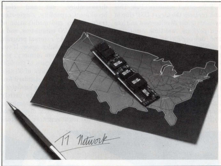
Mounted on a circuit board that's about the size of a stick of chewing gum, the T1/CEPT Line Card from Dallas Semiconductor is the first CMOS chip set that meets both the T1 and CEPT telecommunications standards.
