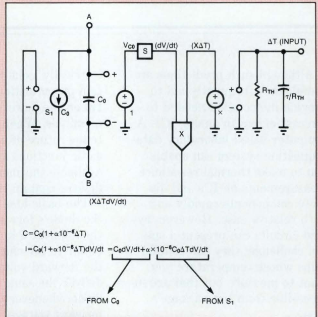
Fig B—You can model the effects of varying temperature on an integrated capacitor by shunting the capacitor with a voltage-controlled current source.
