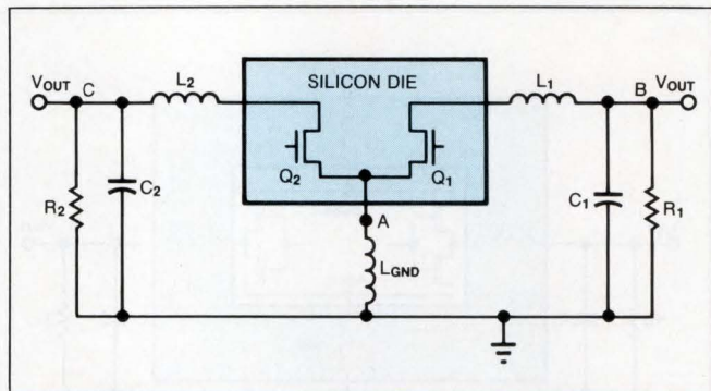
Fig 6 —Switching one output causes ringing in unswitched outputs. If Q_2 is on and Q_1 turns on, current flow from C_1 will raise the voltage at node A. This rise, in turn, will force current into C_2 , initiating ringing.
