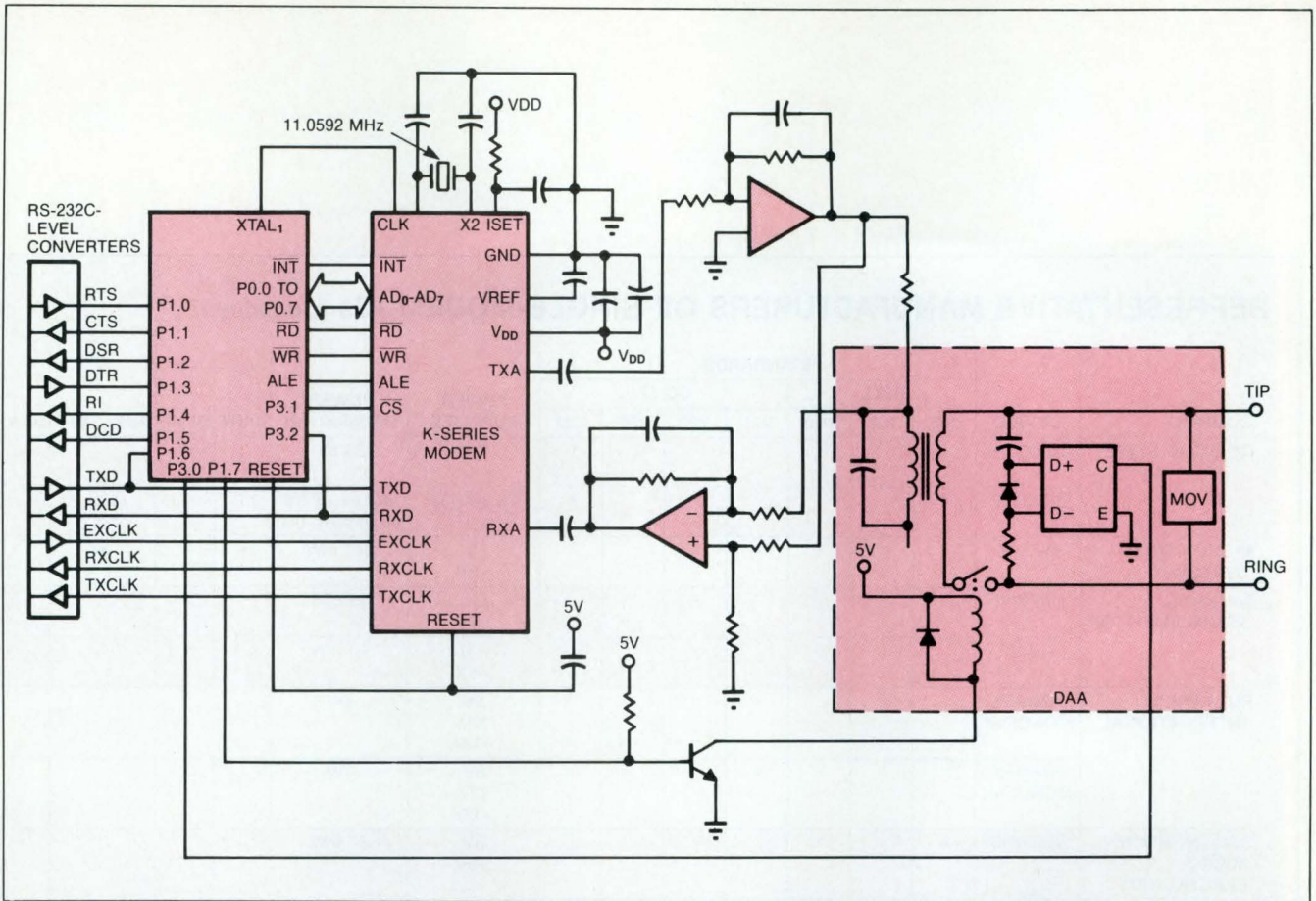
Fig 2—The K Series of single-chip modems from SSI come in packages with identical pinouts. The addition of a controller, a duplexer, and a DAA completes the design.
