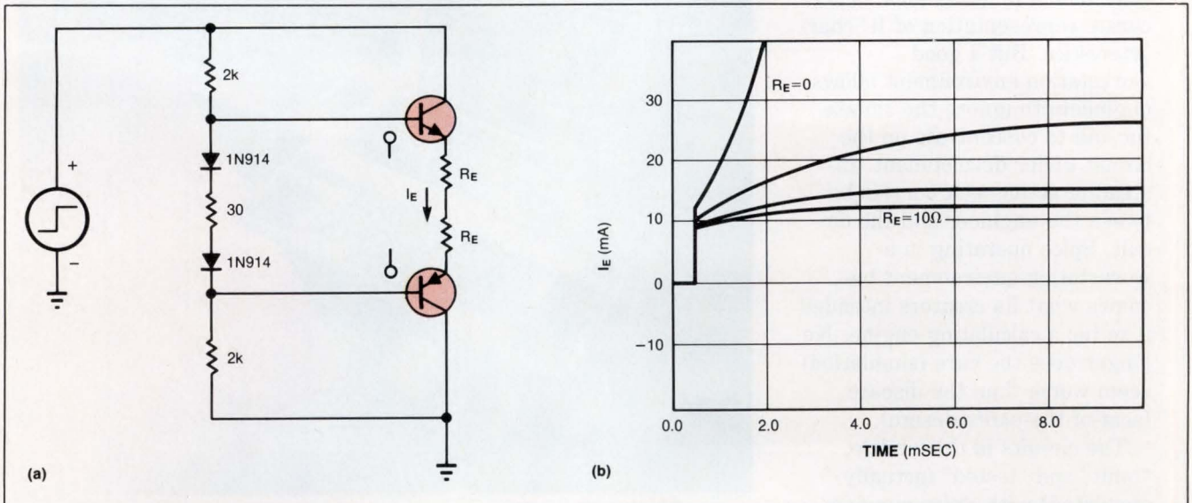
Fig 3 —If you make the degeneration resistance in the complementary output stage (a) too small, the circuit will destroy itself, as the upper curve of the current-vs-time graph (b) illustrates.
