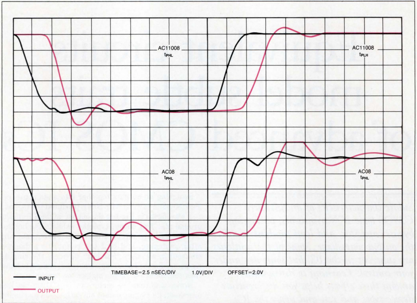
Fig 1—Switching all outputs together into a 50-pF/500Ω load produced these waveforms at the output farthest from the ground pin (HP 54110 digital scope). Notice that the outputs ring after switching, and that the ringing is a damped sinusoid in all cases. The ringing frequency for the low-to-high transitions is slightly lower than for the high-to-low transitions. The AC08 waveforms show some distortions because of reflections or a noisy ground.
