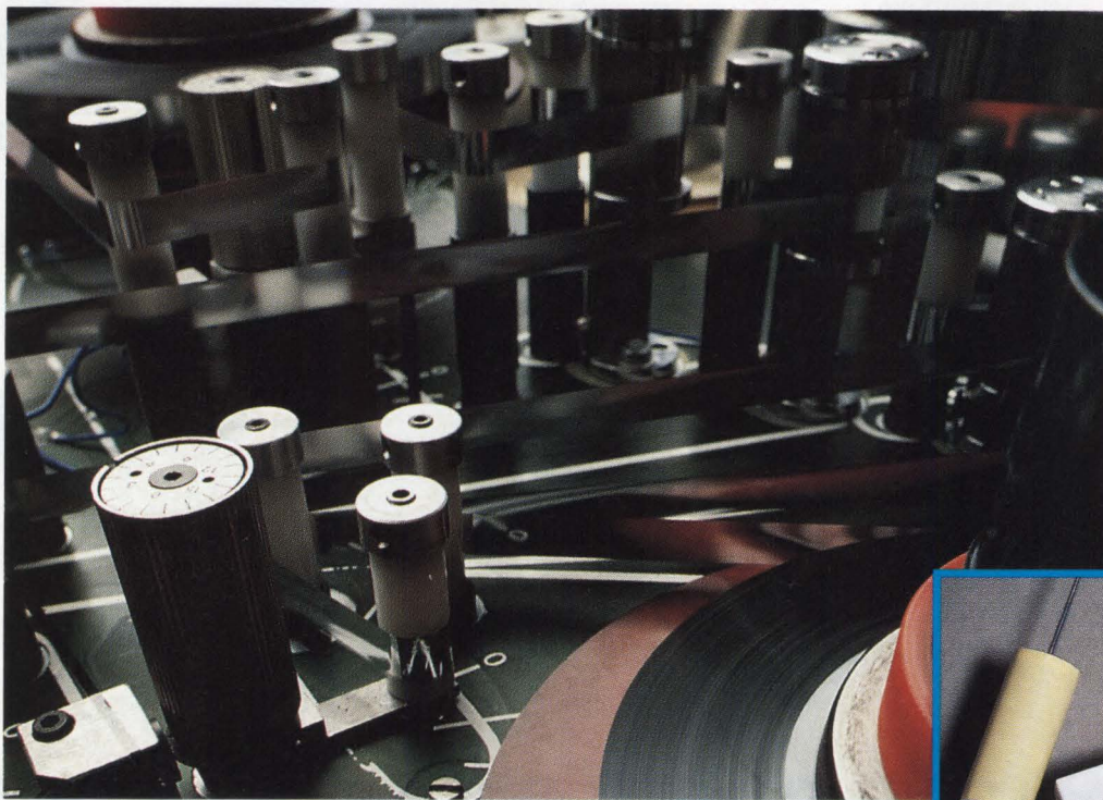
Automated high-speed winding operation for DC Film capacitors.
