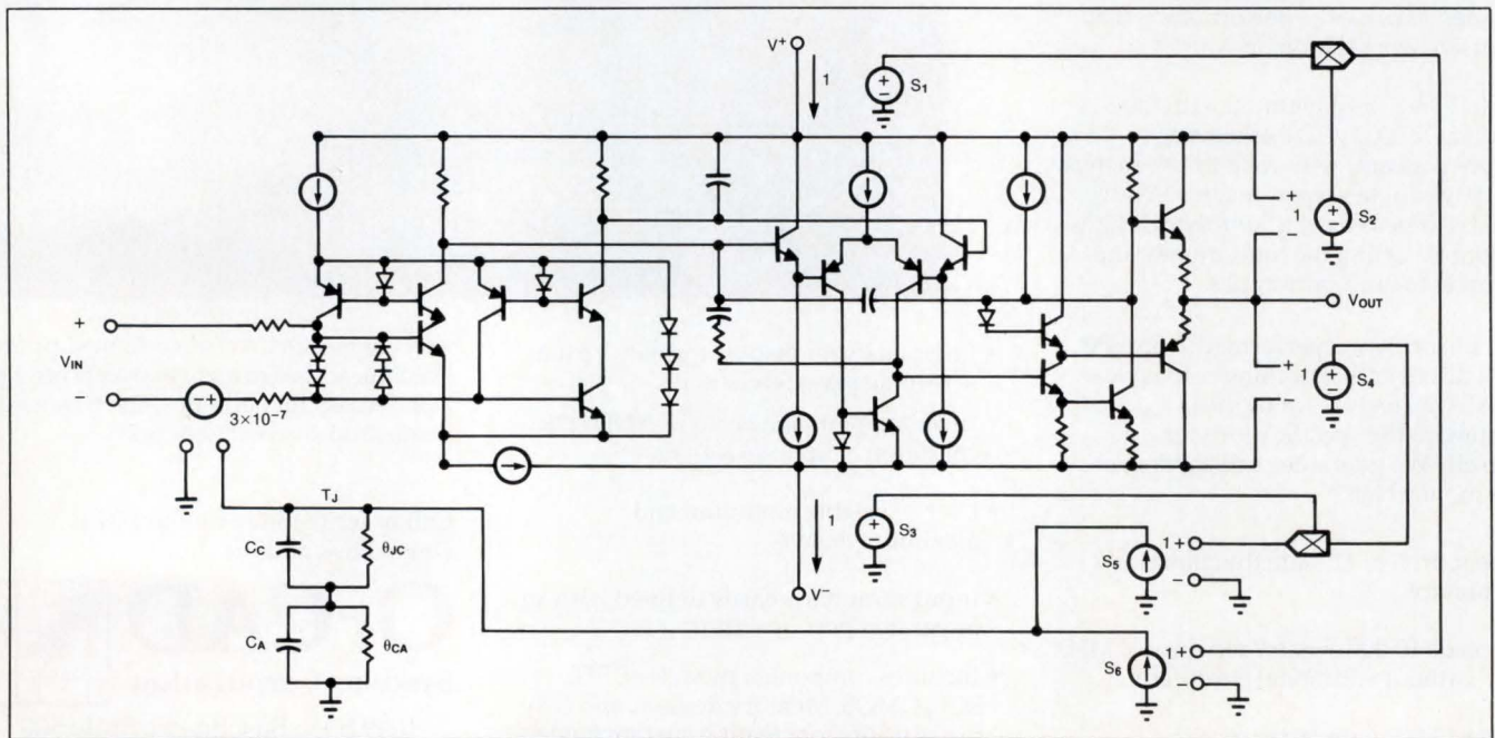
Fig 5 —Close examination of the simplified schematic of PMI's OP-77 indicates the similarity between the techniques used for thermal modeling of ICs and discrete devices.
