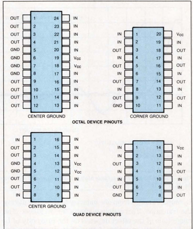
Fig 9—These pinouts are used to obtain the inductances in Table 1. The packages shown reflect the industry-standard pinouts for octal and quad logic families.
