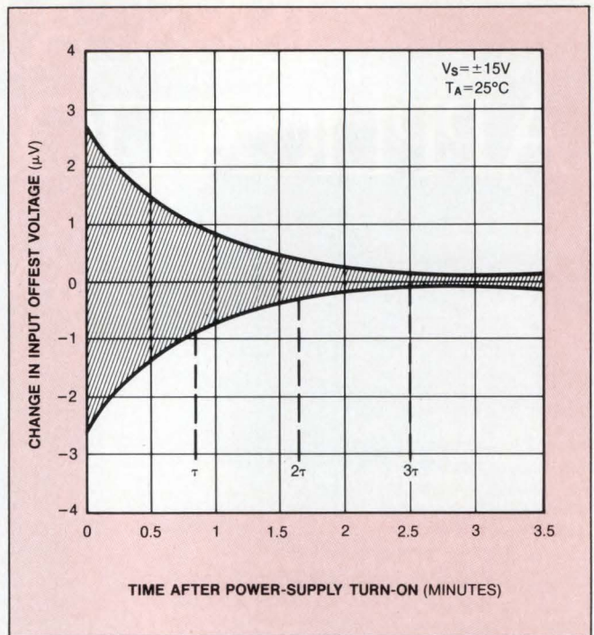
Fig 6—The offset voltage of a precision op amp (PMI's OP-77) changes as the device warms up. The curves indicate a junction-to-ambient thermal time constant of about 50 sec.
