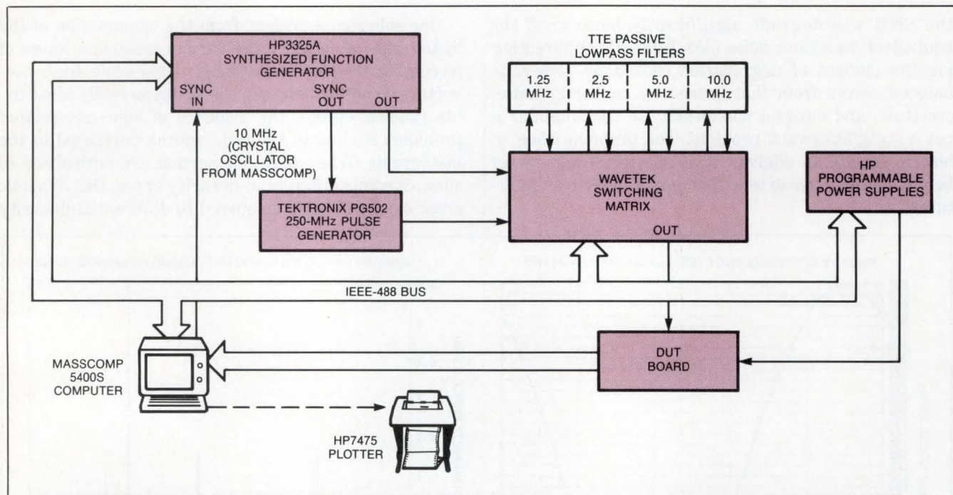
Fig 7—Reflecting the testing principles outlined in the text, this test system used at Hybrid Systems measures spuriousness and differential nonlinearity at high frequencies.
