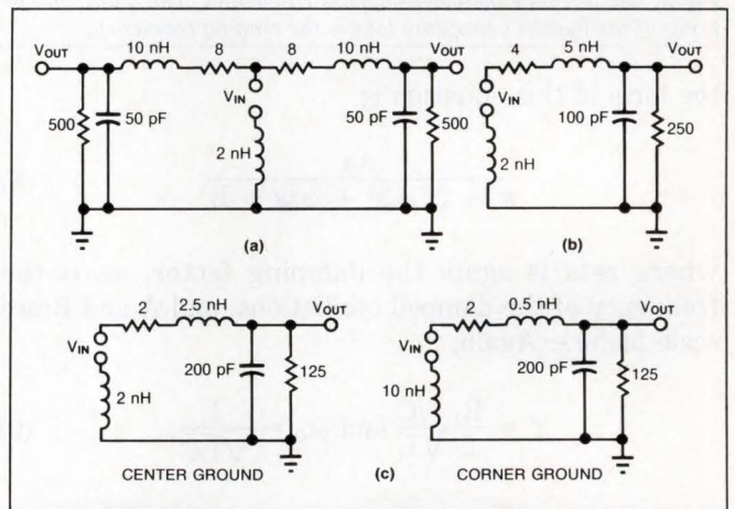
Fig 4 —The simple circuits of Fig 3 do not explain all of the devices' characteristics. Because all outputs in the low state share a common ground inductance, you cannot model them as independent circuits. In a , you see two outputs on a part that has a center-pin ground. The two 8\Omega resistors represent the on-resistance of the transistors; b is the Thevenin equivalent of the circuit in a . Finally, c shows the equivalent circuits for quad AND-gate devices.
