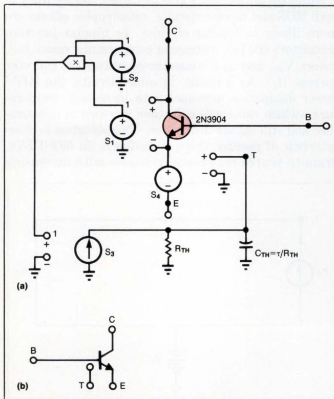
Fig 2 —A complete dynamic model (a) includes a capacitor that simulates thermal mass. You can represent the entire model as a transistor with an extra node (b) and use the synthesized device in complex circuits.
