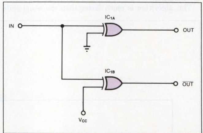
Fig 1—This simple complementary-driver circuit uses XOR gates for both the inverting and noninverting paths, and therefore the output skew is equal to the chips' manufacturing tolerance.
