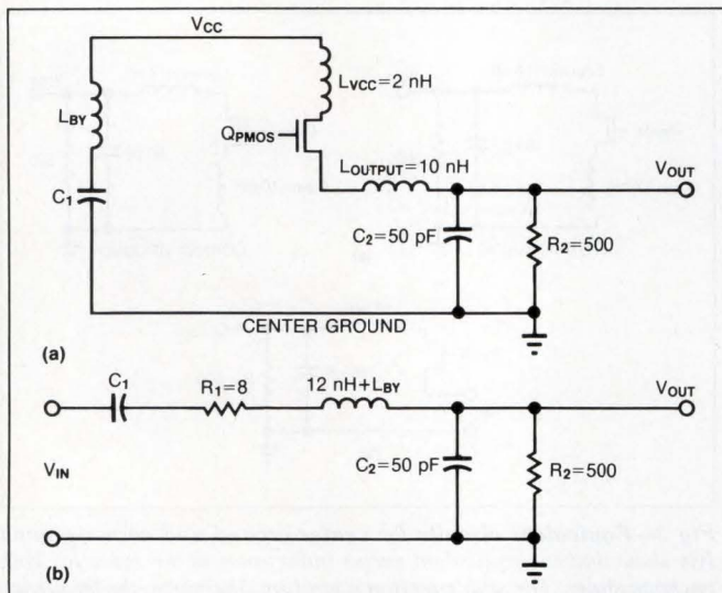
Fig 5 —The high-state circuit is similar to the low-state circuit of Fig 3, but includes the device-bypass capacitors. The added inductance of the bypass capacitors lowers the ringing frequency.
