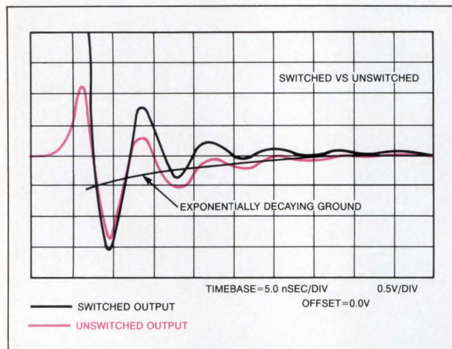
Fig 12—A miscalibrated high-impedance probe can also distort output waveforms—in this case, it introduces an exponentially decaying ground reference.
