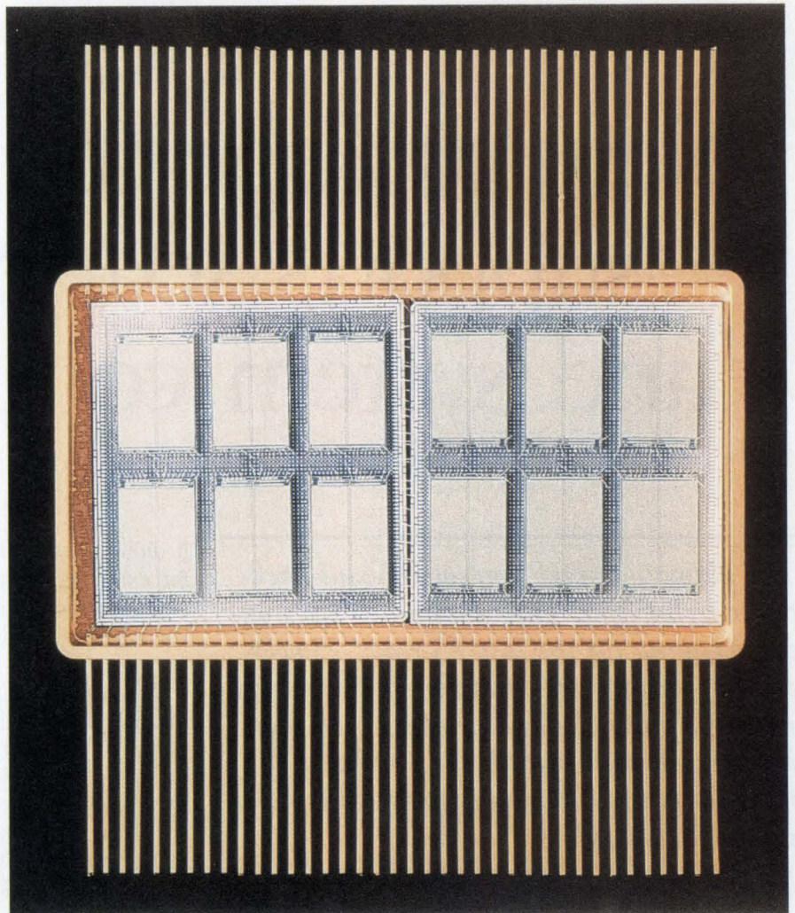
Two silicon circuit boards in a hybrid package hold twelve 32k×8-bit static RAM chips, creating a 3M-bit, 65-nsec, cache-memory module. (Photo courtesy Mosaic Systems Inc)
