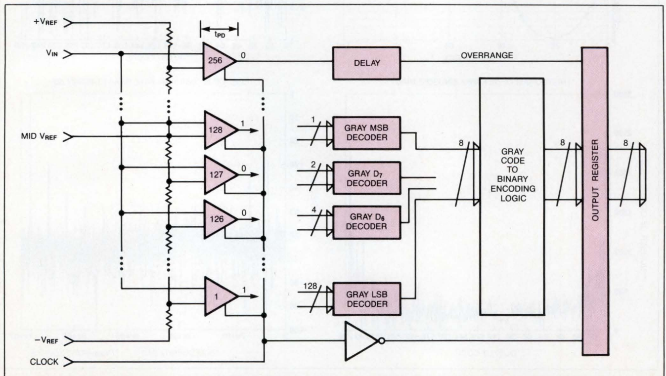
Fig 5—Equivalent "bubbles" at high slew rates cause only minimal output-code errors in a Gray-code-based flash converter.
