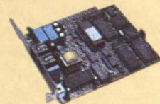
Half-Pak #24 IBM† PC Compatible Half Card 2400 bps Modem Circle No. 173
