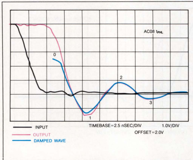
Fig 8—Overlaying the calculated and actual curves reveals that the initial peak of the model's prediction does not reach the initial voltage of the measured data. This discrepancy arises because the formulas rely on a constant-resistance model for the transistor.
