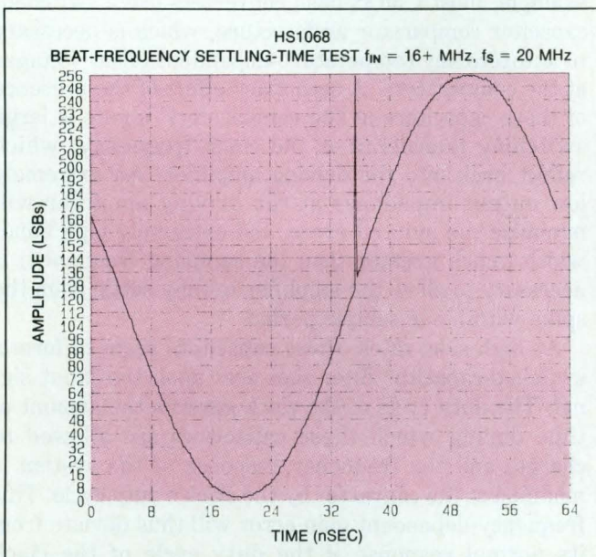
Fig 2—This classic example of a spurious-code spike is the result of exceeding the slew-rate capability of the converter.
