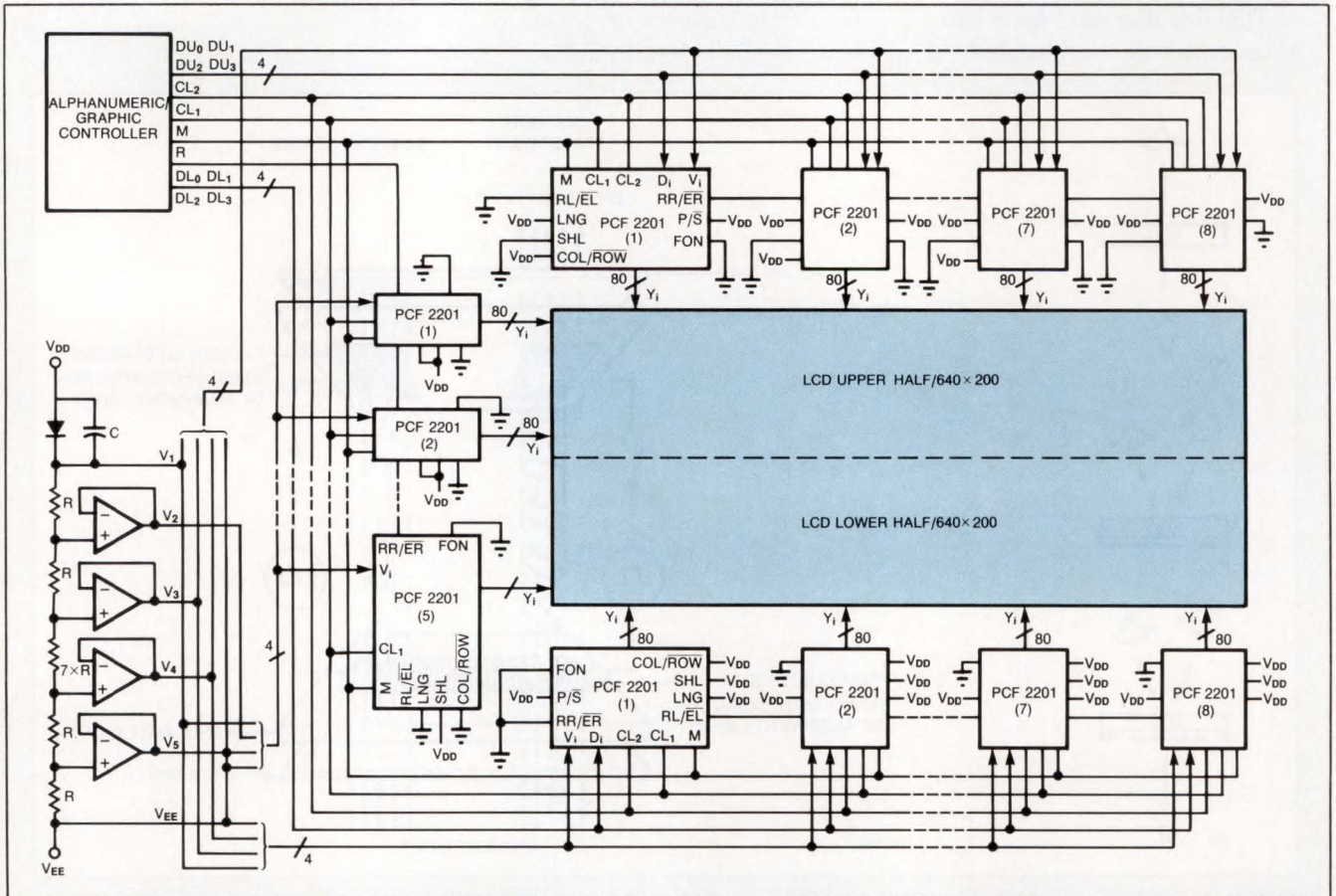
Fig 2—A typical flat-panel LCD system contains a dot matrix of 640 columns by 400 rows divided into two half screens of 640×200 pixels. The top and bottom column drivers control display data on the corresponding half screens while the row drivers provide the periodic strobe signals.
