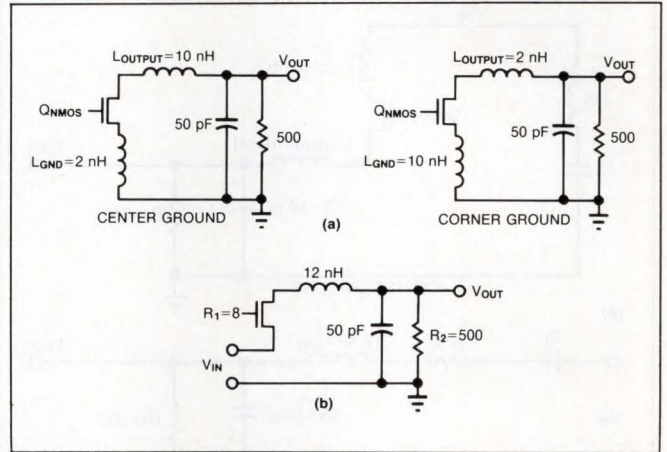
Fig 3 —Equivalent circuits for center-ground and corner-ground ICs show that the equivalent series inductance is the same for both package styles. For single-section operation, therefore, the frequency of oscillation is the same for both.
