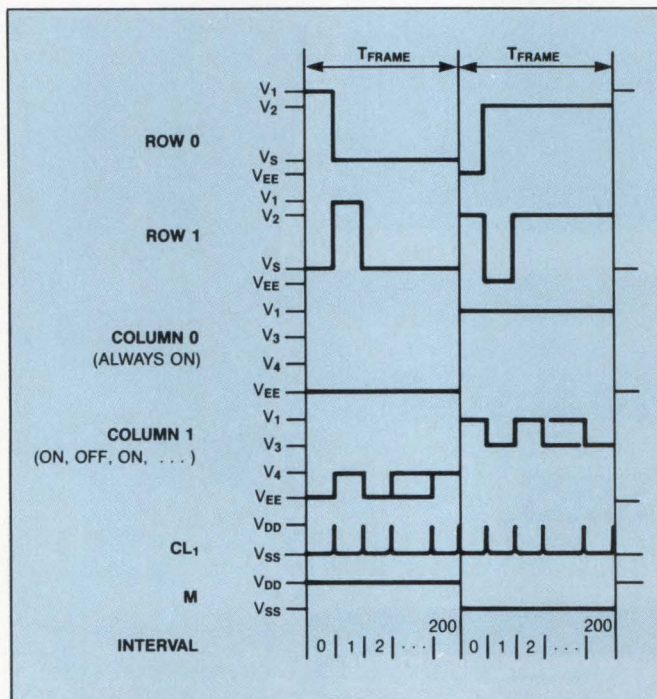
Fig 3—To control two alternate display frames, the drive electronics provides identical voltage-difference signals to the pixels but reverses polarities for the second frame.
