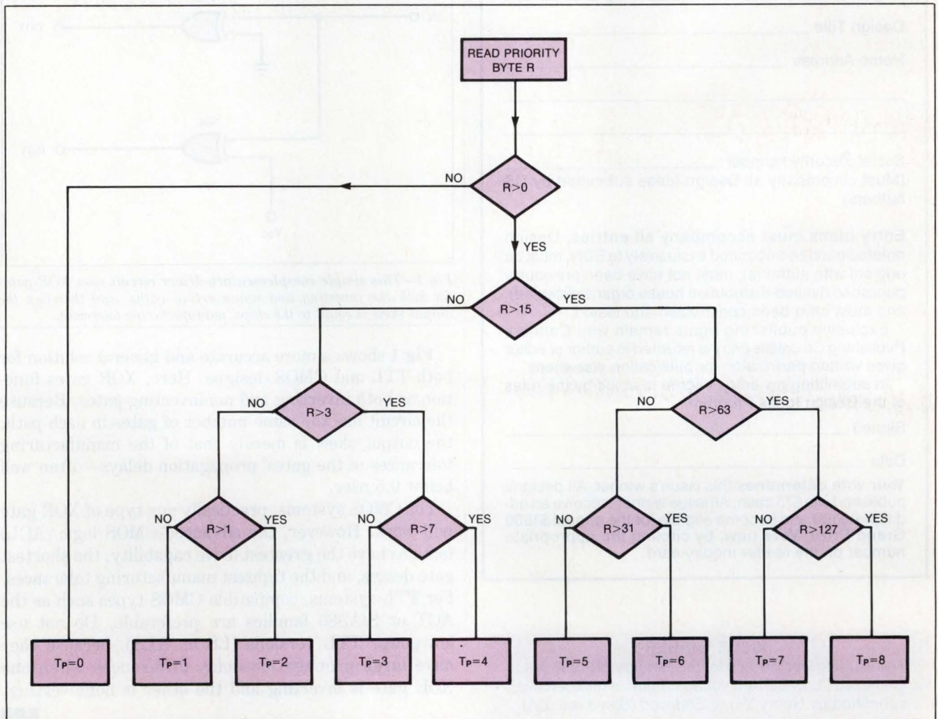
Fig 1—This easily encoded, successive-refinement algorithm homes in on the most significant asserted bit in an 8-bit word. Each asserted bit represents a prioritized task ( T_P ) requesting attention. This algorithm is faster than conventional shift-and-test methods.
