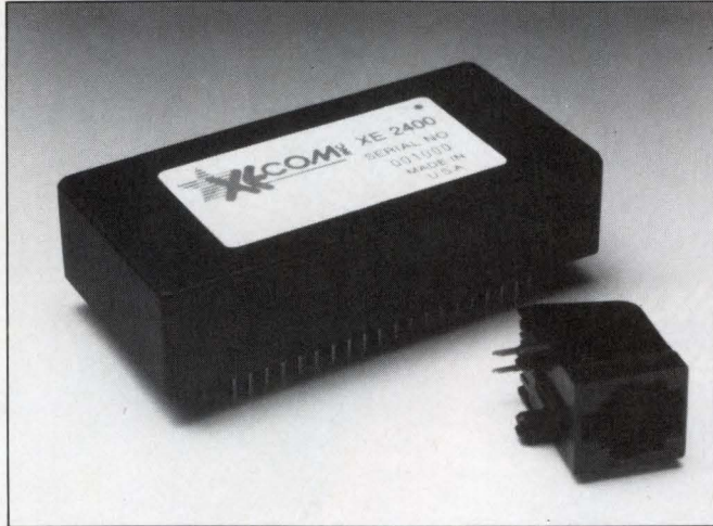
Hybrid modules, such as the XE2400 from Xecom, have built-in 2- to 4-wire hybrids and FCC-registered DAAs. Hybrid modules have the advantage of being quicker to get to market.
