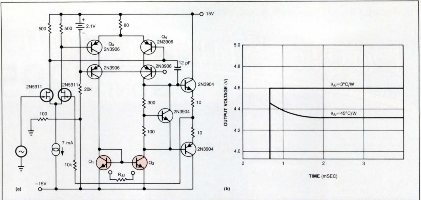
Fig 4 —If you use discrete transistors to build the current mirror consisting of Q_1 and Q_2 (a), signal-induced dissipation causes the amplifier output to exhibit a long tail, as indicated by the lower curve of the voltage-vs-time graph (b).
