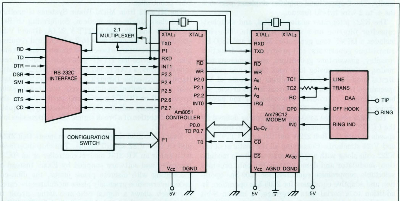
Fig 1—The Am79C12 modem has all its modem functions on one chip. You only have to add a \mu controller and a DAA to have a complete 1200-bps modem.
