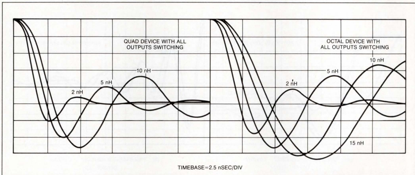
Fig 10—Quad and octal devices exhibit differing inductances. These inductance differences translate to variations in the ringing frequencies.
