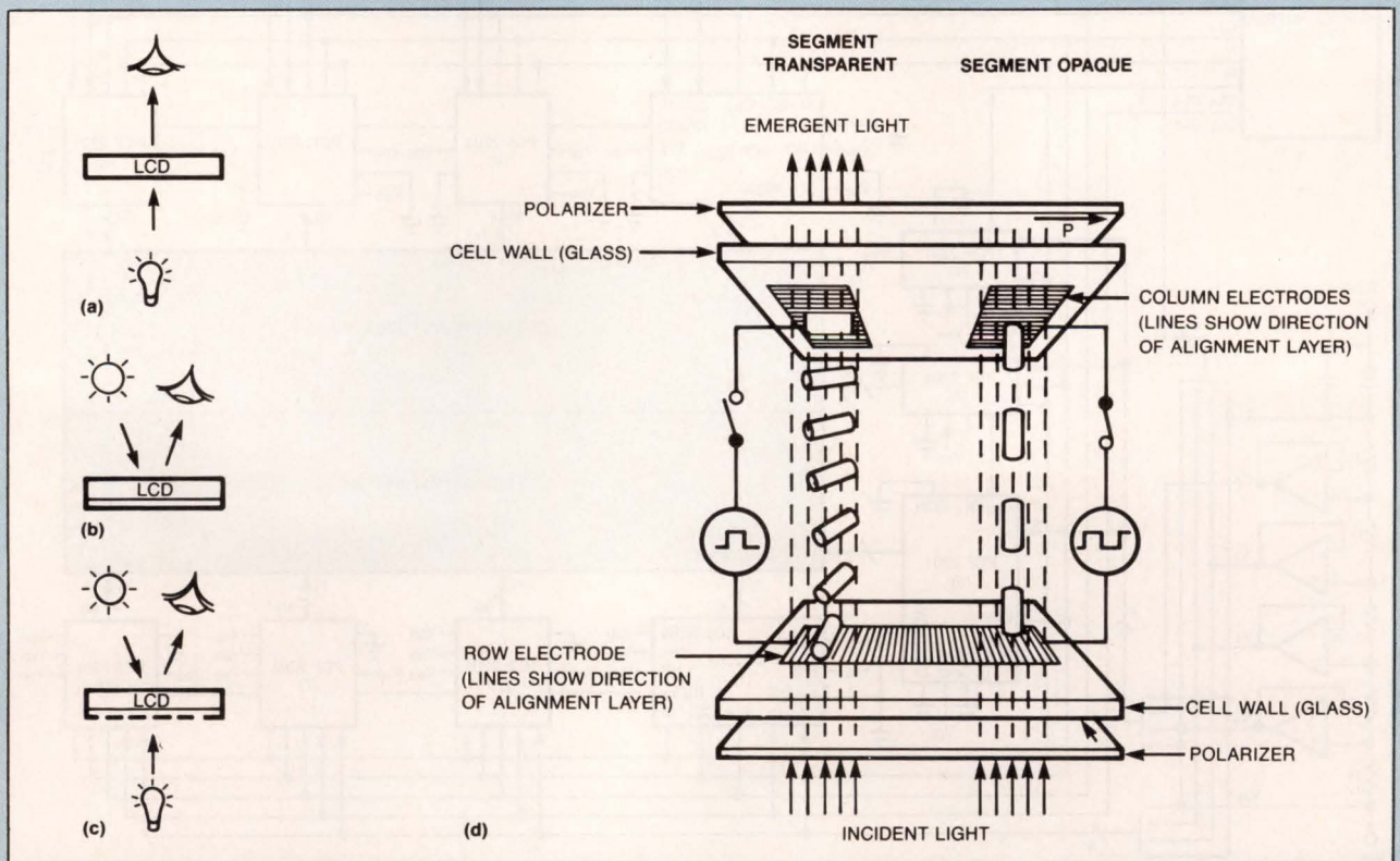
LCDs can operate in a transmissive mode (a), which requires a back light, in a reflective mode (b), which relies on ambient light, or in a transreflective mode (c), which combines features of the other two modes. A typical LCD (d) consists of a layer of liquid-crystal material sandwiched between two glass plates. Shown is the 90°-twist, or TN, version; typical STN LCDs employ a 270° twist.
