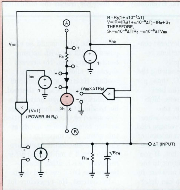
Fig A—This model of an integrated resistor uses a voltage-controlled voltage source to model the effects of temperature.
