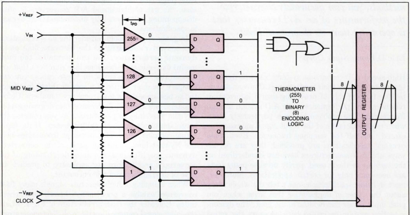
Fig 1 —"Bubbles" appear in thermometer-code lines at high input slew rates, because of mismatches in the propagation delays of the individual comparators.
