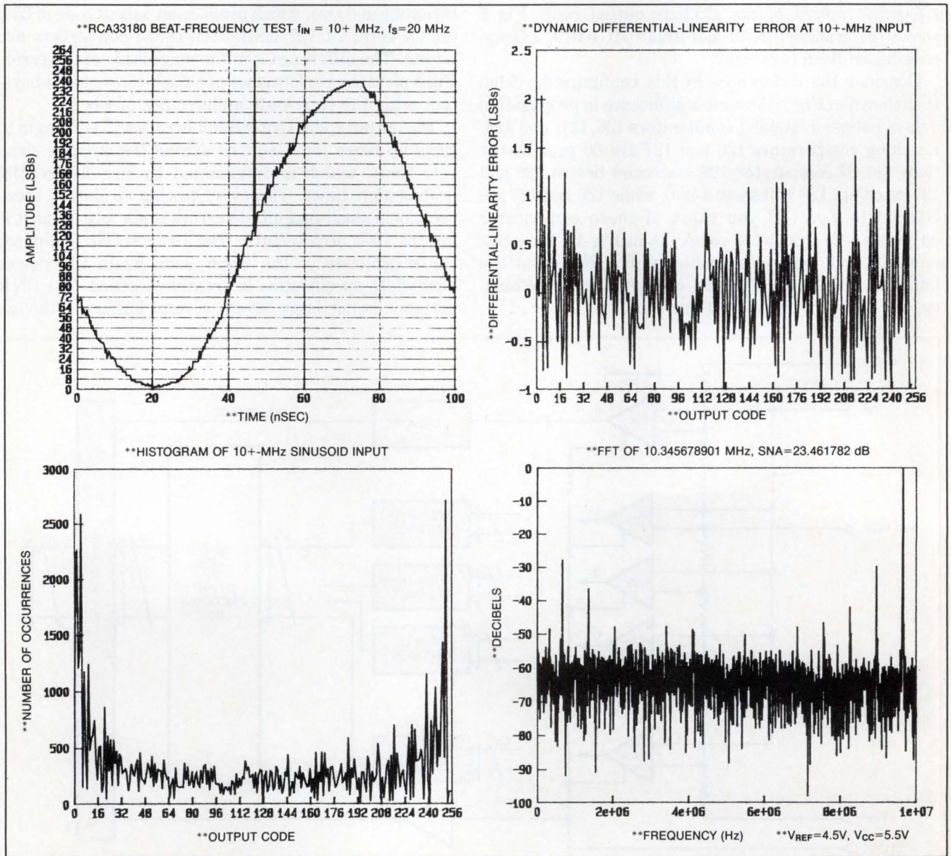
Fig 4—Spurious codes and differential-linearity degradation result when you drive a CMOS-processed flash A/D converter at frequencies beyond its capabilities.
