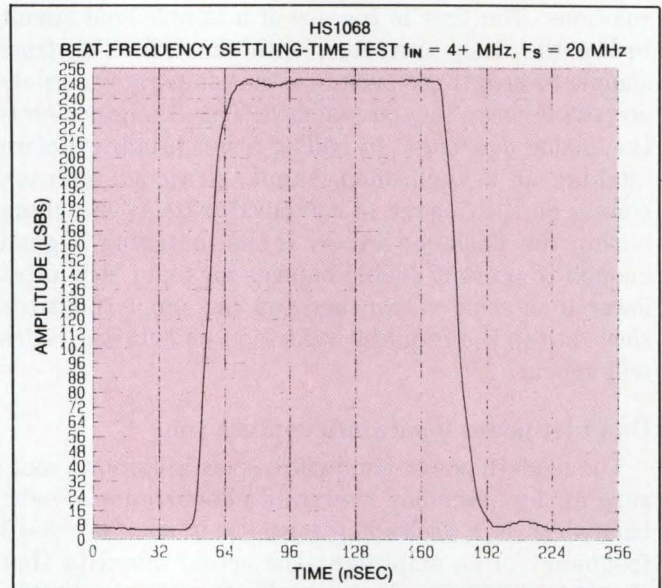
Fig 3—A settling-time plot uses a sampling-scope test. This plot for the HS1068-based subsystem uses a variation of the beat-frequency test.
