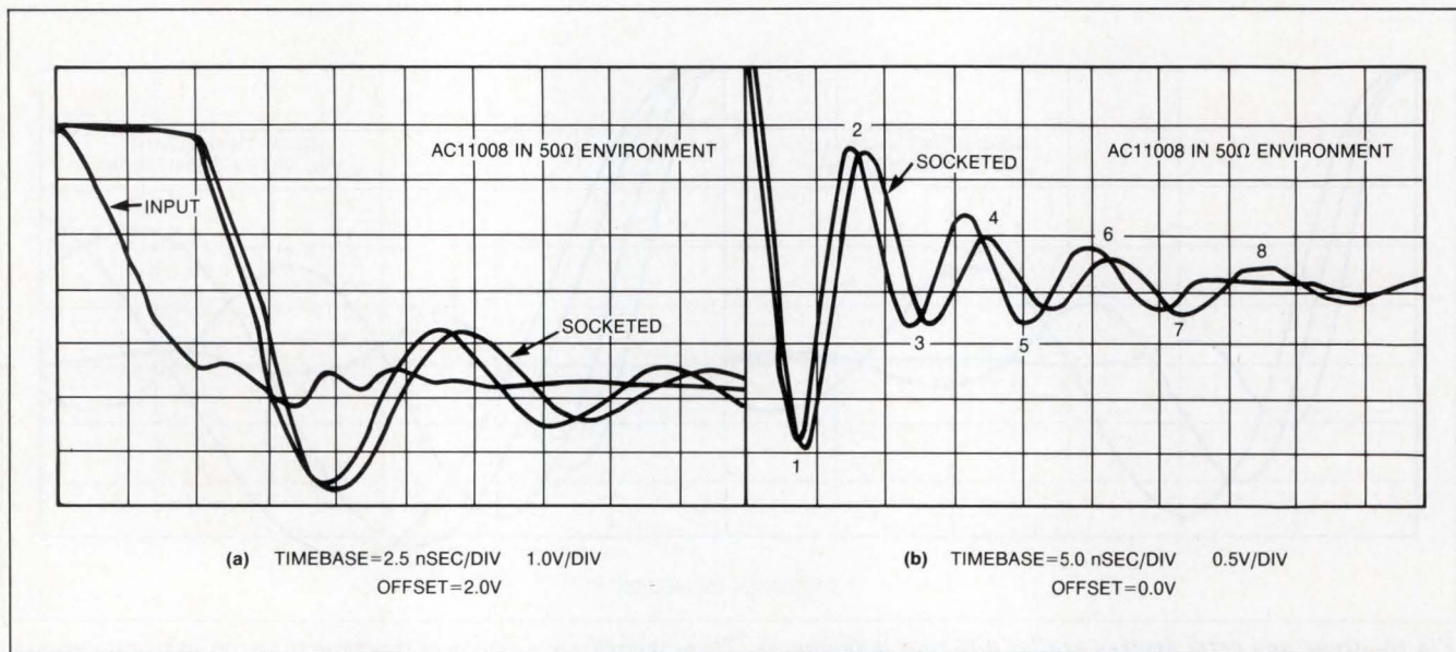
Fig 11 —Adding a socket to a test setup alters device waveforms adversely. Propagation time and overshoot increase, and the ringing frequency decreases.
