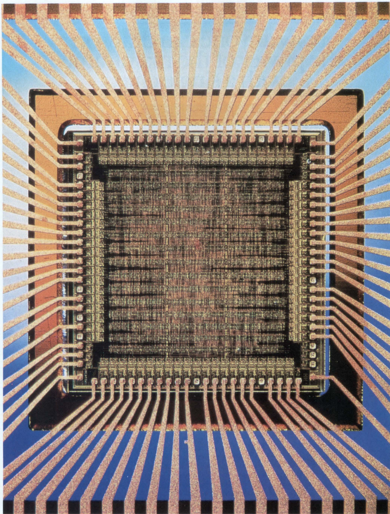
Advanced packaging will play a key role in the creation of devices and systems in the 1990s. This 84-lead IC resides in a National Semiconductor TapePak package and occupies only 0.36 in 2 of pc-board space. You can use conventional surface-mount techniques to attach the device to a pc board.
