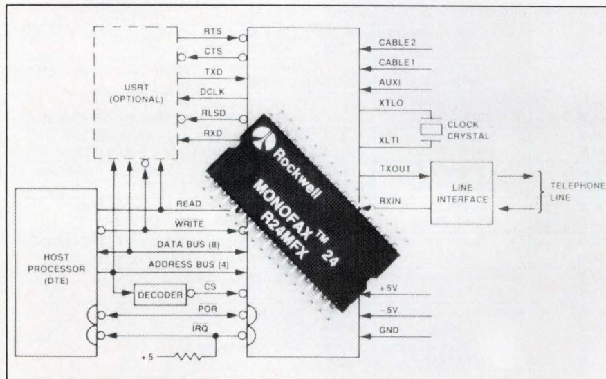
The R24MFX Monofax modem consists of two chips housed in a quad-in-line package. Manufactured by Rockwell, the IC is optimized for compact Group 3 facsimile machines.
