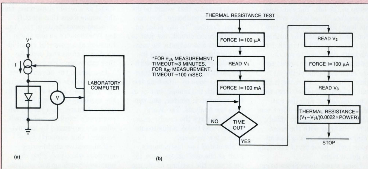
Fig A—A laboratory data-acquisition system (a) simplifies measurement of a device's thermal resistance. The flow chart (b) shows the steps required.
