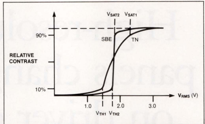
Fig 1—Because STN-type LCDs have a sharply defined on/off voltage boundary, a small change in the value of rms driving voltage produces a large change in the display's relative contrast.
