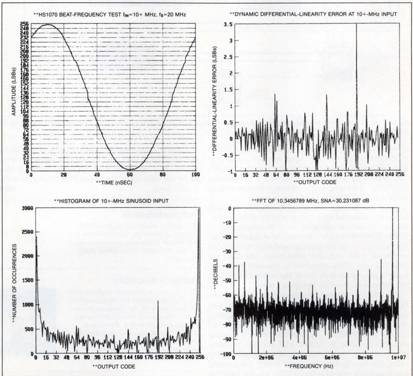
Fig 6 —These plots from a Gray-scaled flash converter show no classical spurious codes. Slew-rate-induced problems appear as missing or widened codes.
