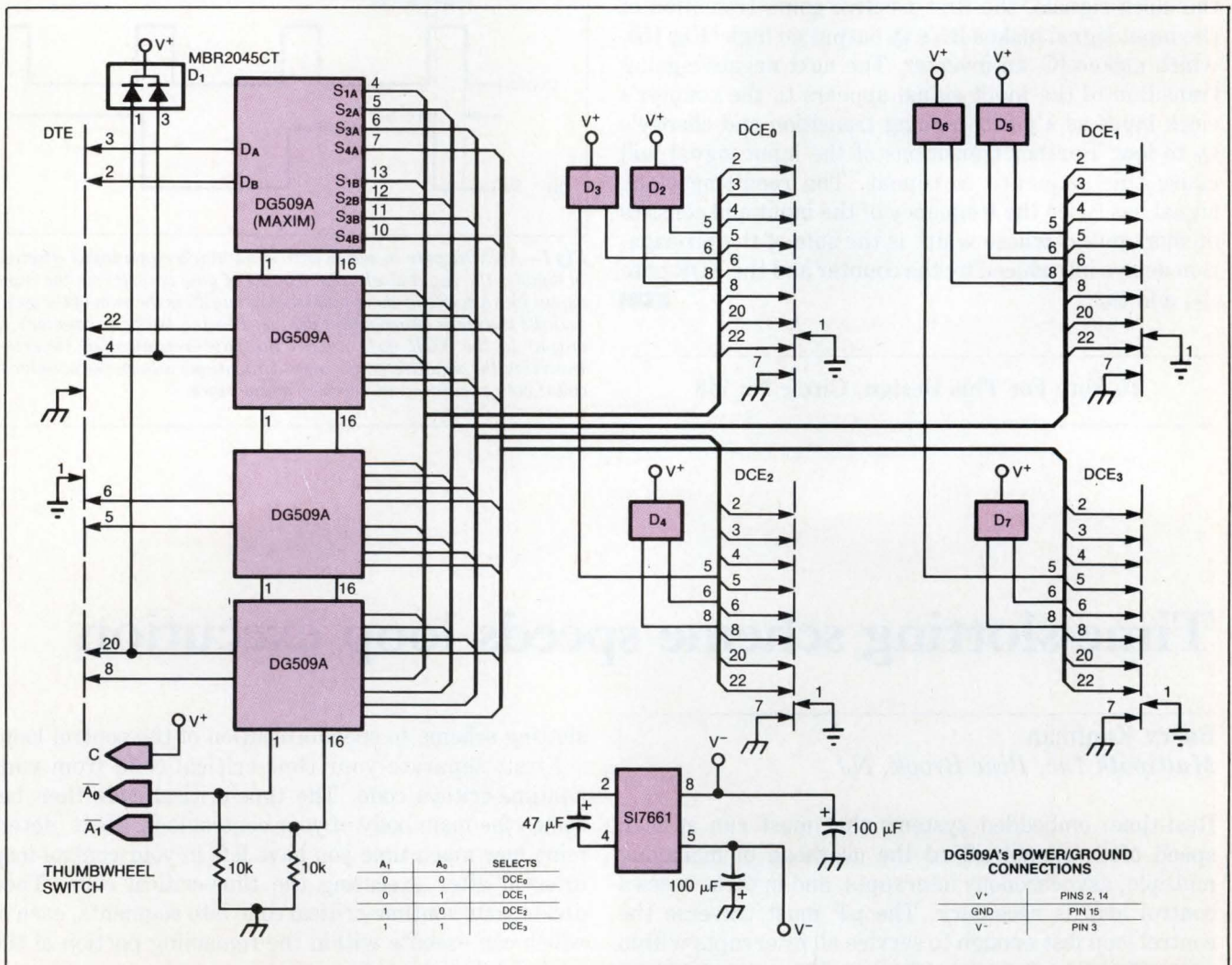
Fig 1—This signal-powered selector uses analog switches to connect one of four RS-232C devices to a terminal or personal computer.
