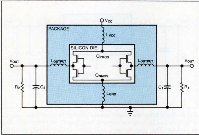
Fig 2 —This ACL-device model has two outputs and a test load. Each of the device's leads and bond wires has some amount of inductance. Leads near the end of a DIP have more inductance than leads near the center of the DIP.
