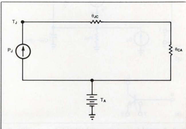
Fig 1 —A static thermal model of a bipolar junction transistor includes a power source, two thermal resistances, and the ambient temperature.
