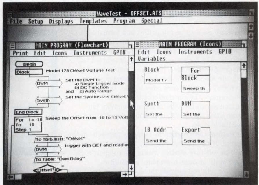
The flowchart- or module-programming techniques provided by Wavetek's Wavetest package let you use 19 standard program-module icons to program IEEE-488 systems. Where necessary, however, you can also incorporate segments of Basic code in your program.
