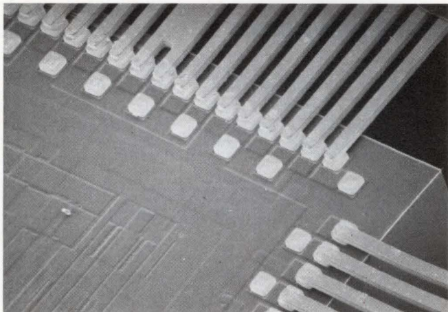
Fig 1 —TAB technology allows chip vendors to bring many more signals off an IC with connections that have lower impedance, more ruggedness, and more reliability than conventional wire bonds provide. In addition, TAB can accommodate ICs with closer pad spacing than wire-bond technology allows. (Photo courtesy Motorola Inc)
