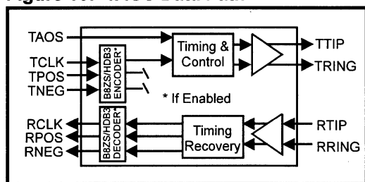
Figure 10: TAOS Data Path
