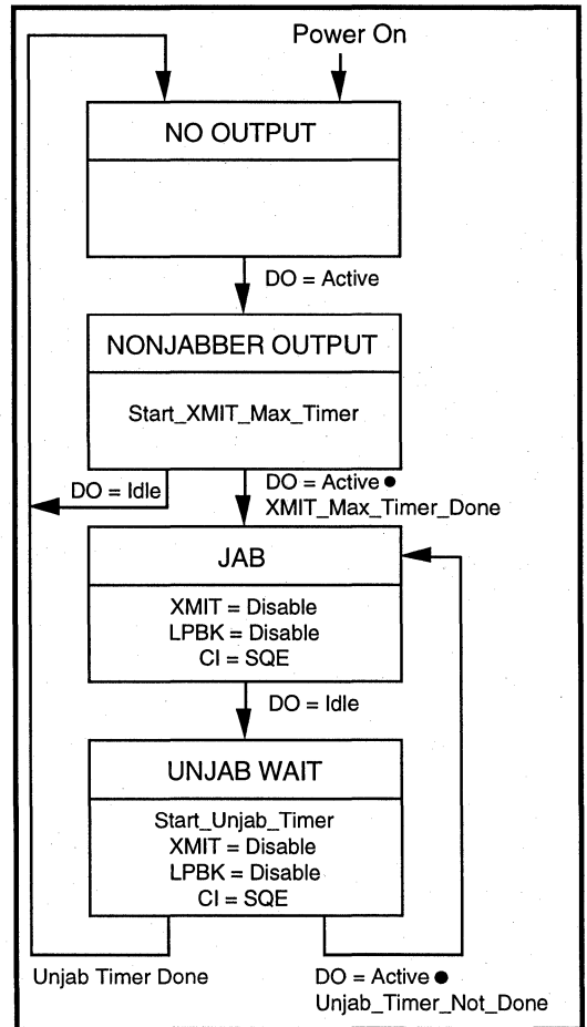
Figure 5: Jabber Control Function
