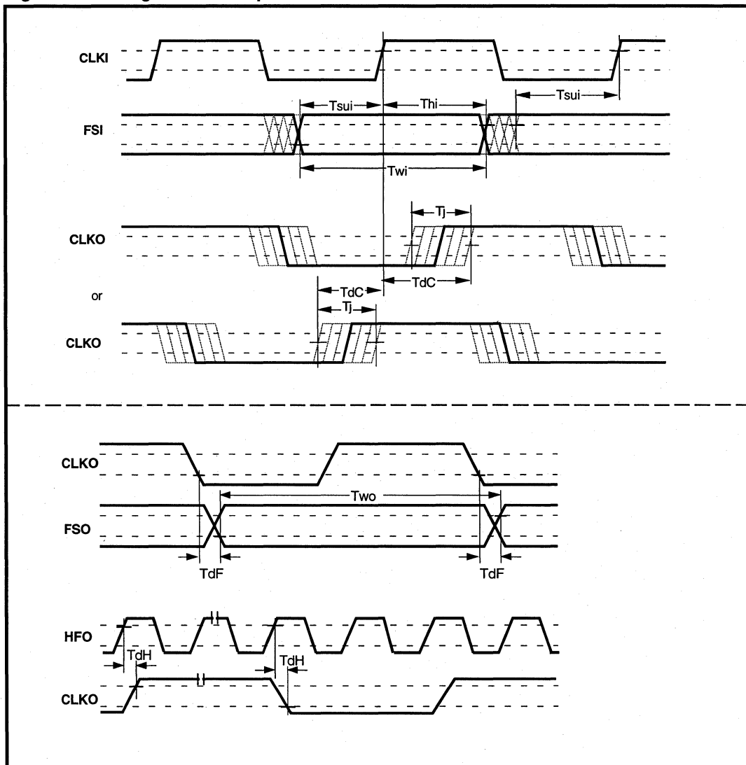
Figure 7: Timing Relationships - FSI / CLKI to CLKO / FSO and HFO
