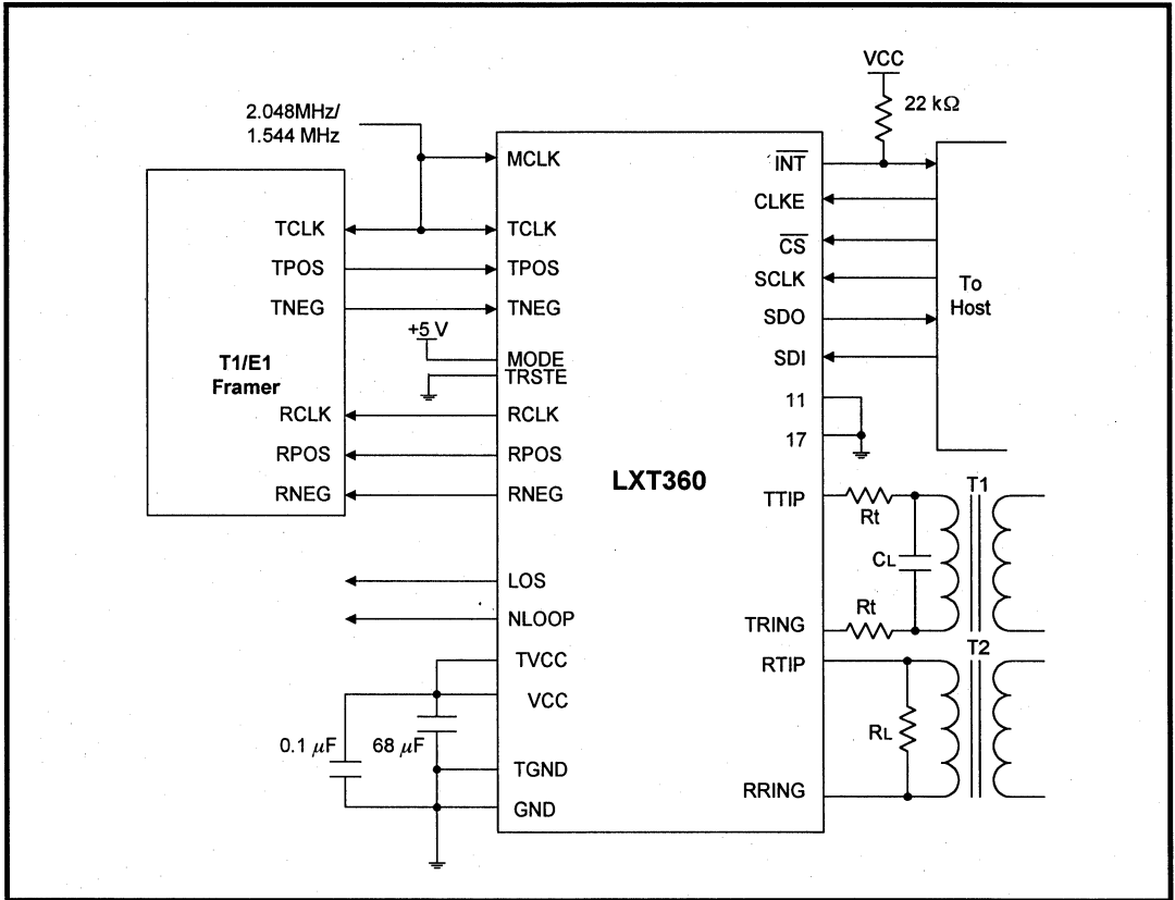
Figure 14: Typical T1/E1 LXT360 Host Mode Application
