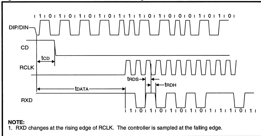
Figure 10: Mode 2 RCLK/End-of-Frame Timing
