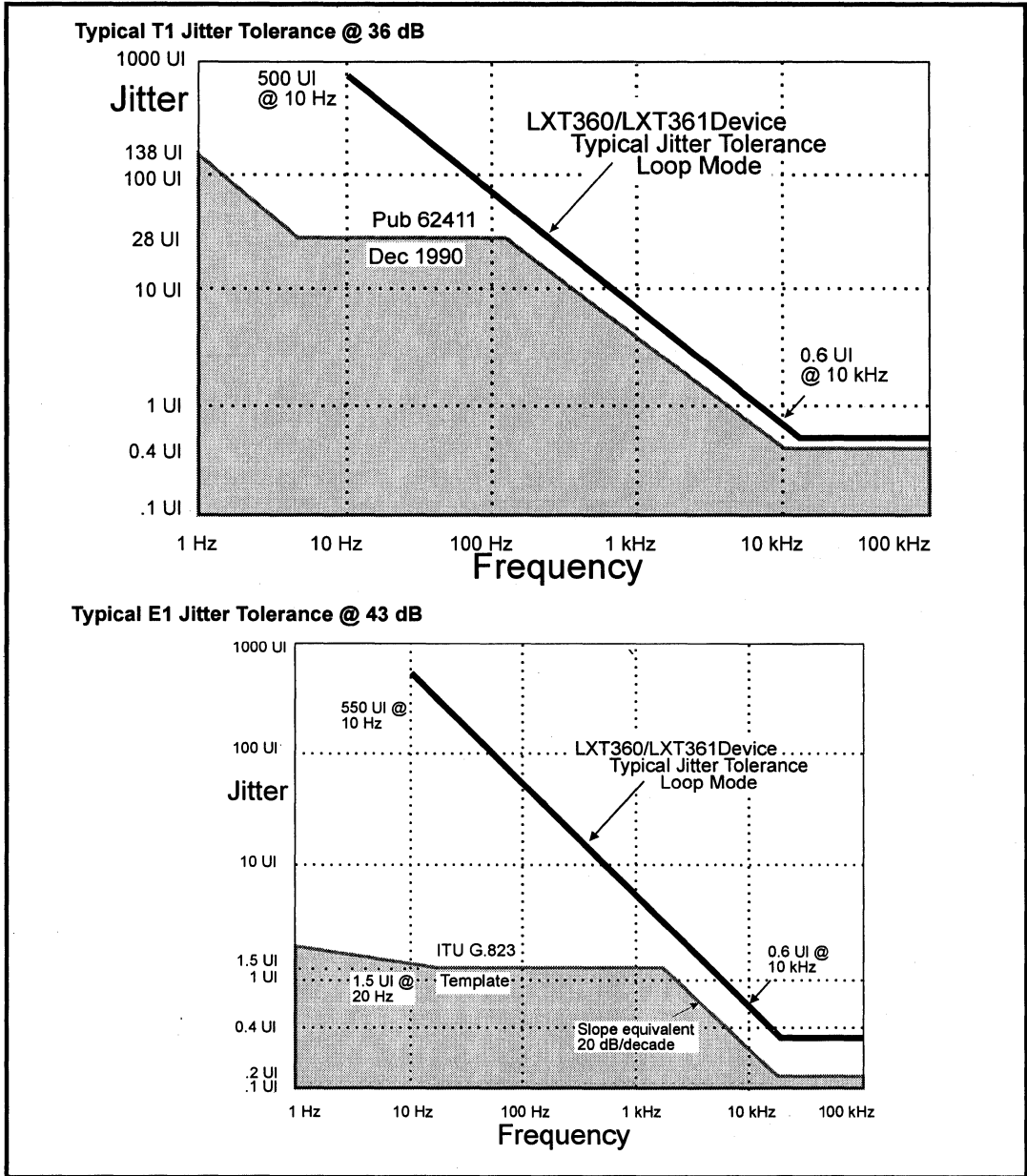
Figure 24: Jitter Tolerance (Typical)
