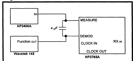
Figure 3: Filter Calibration
