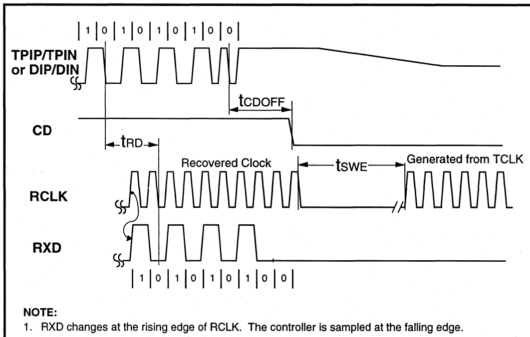
Figure 28: Mode 3 RCLK/End-of-Frame Timing
