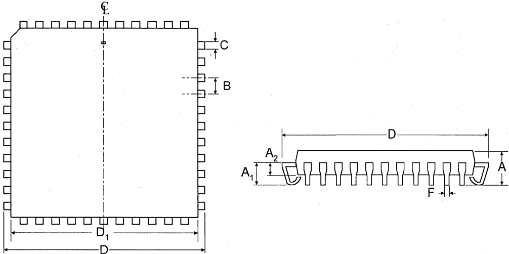
Plastic Leaded Chip Carriers
