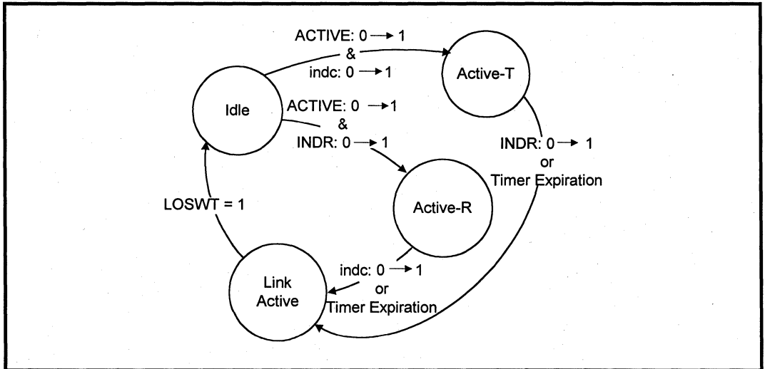
Figure 10: HTU-R HDSL Framer Activation State Machine
