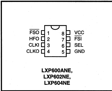
Figure 1: Pin Assignments
