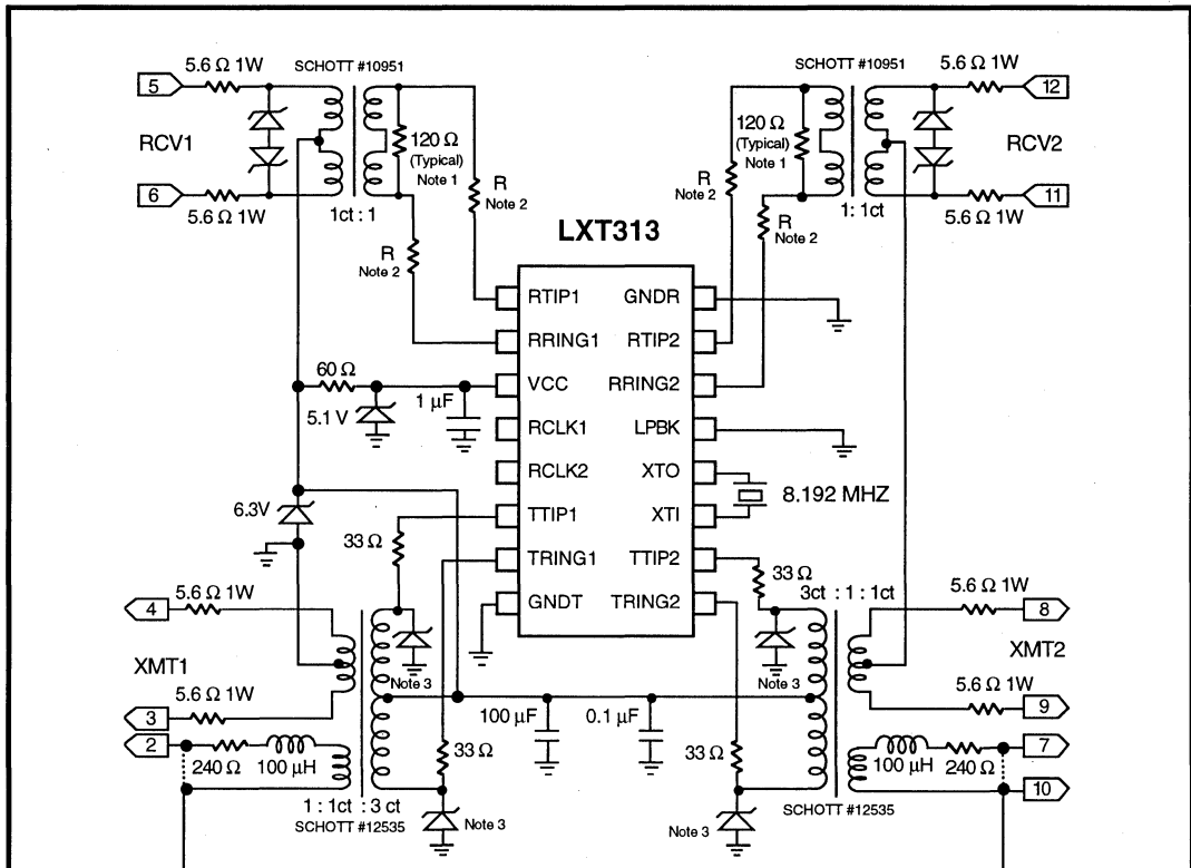
Figure 2: Typical E1 Dual Repeater/Transceiver Application Diagram
