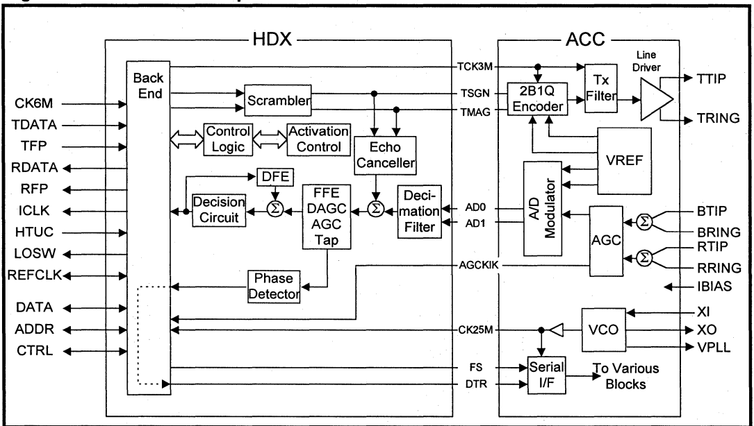
Figure 3: HDSL Data Pump Block Architecture
