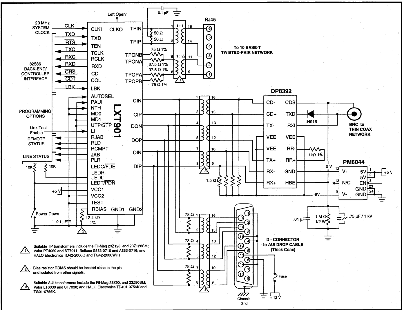
Figure 13: Three Media Application
