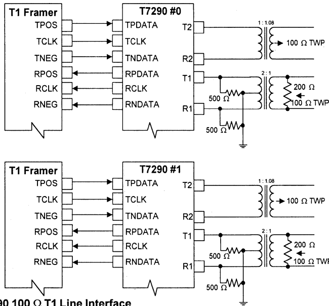
Figure 1A: T7290 100 Ω T1 Line Interface
