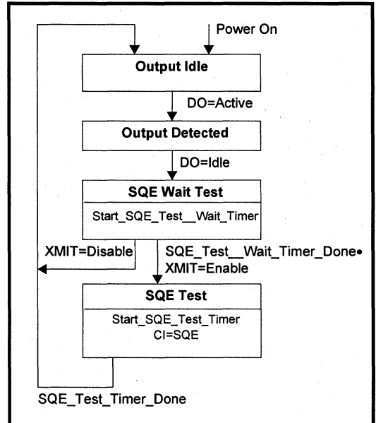
Figure 4: Signal Quality Error
