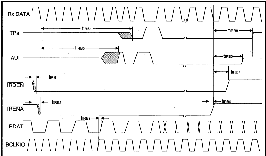
Figure 8: Inter-Repeater Bus Timing
