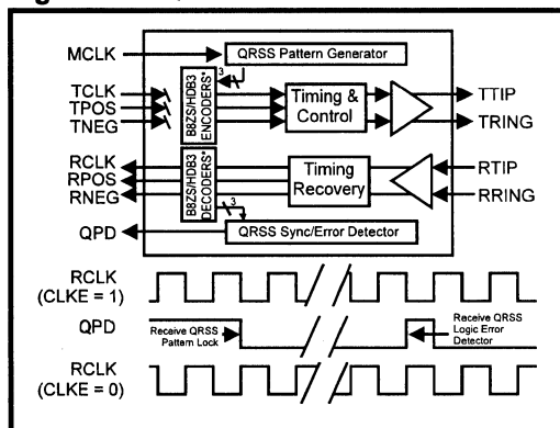
Figure 11: QRSS Mode
