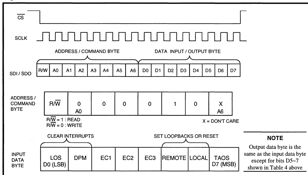
Figure 3: LXT304A Serial Interface Data Structure
