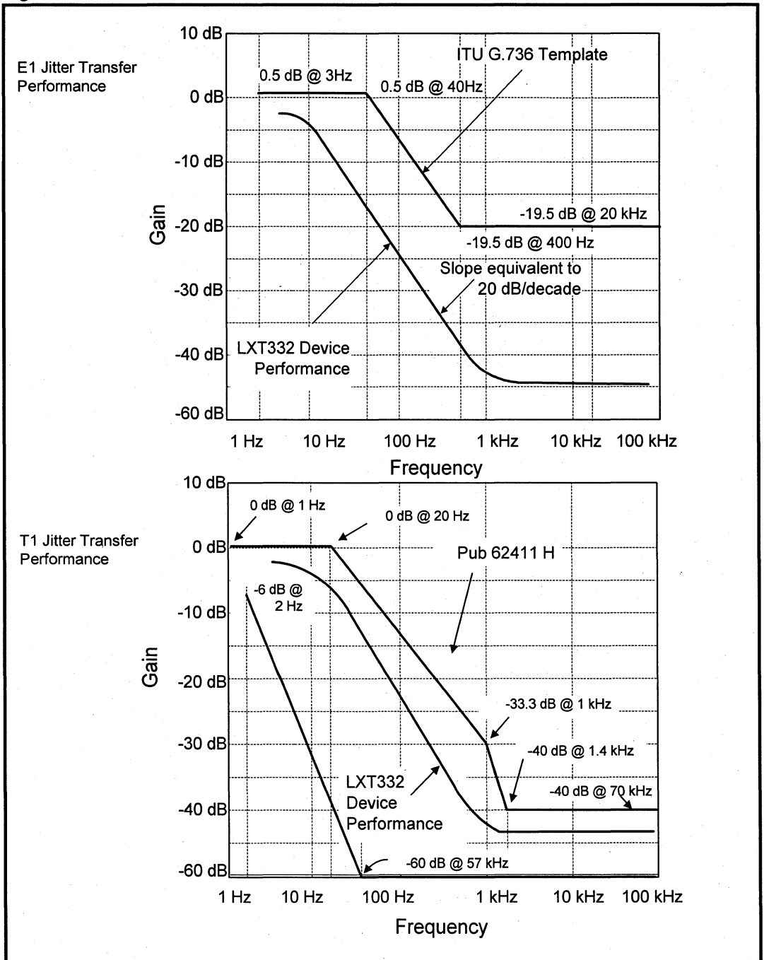
Figure 21: Jitter Transfer Performance
