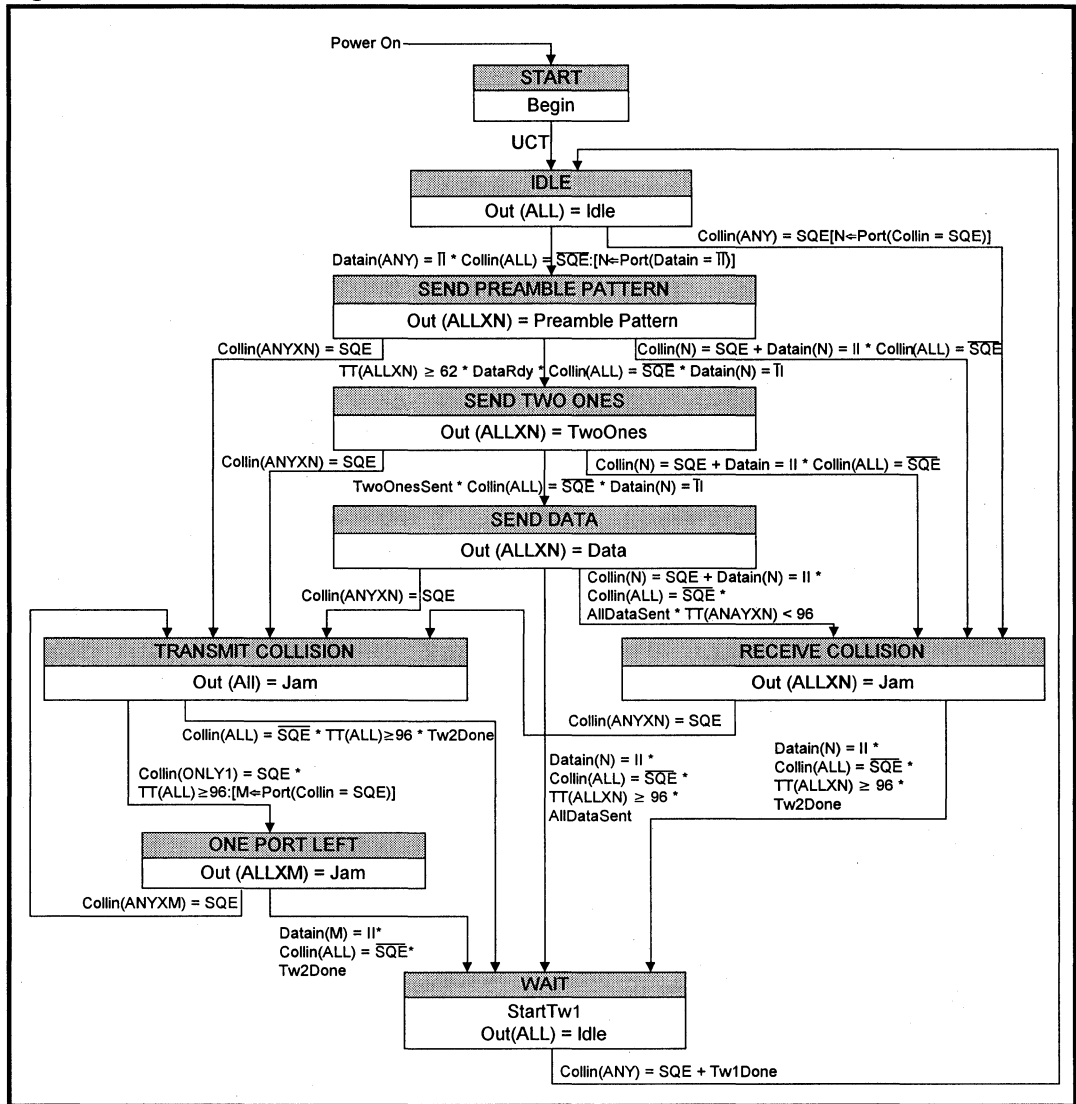
Figure 2: Global State Machine
