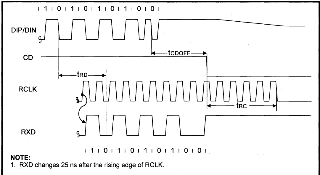
Figure 4: Mode 1 RCLK/End-of-Frame Timing
