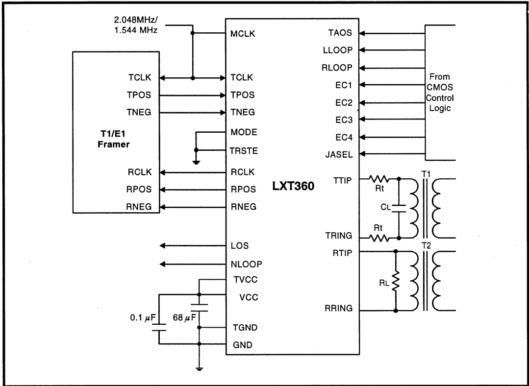
Figure 13: Typical T1/E1 LXT360 Hardware Mode Application
