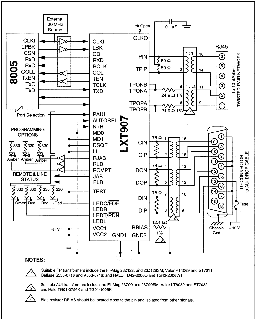
Figure 12: Manual Port Select with Seeq 8005 Controller
