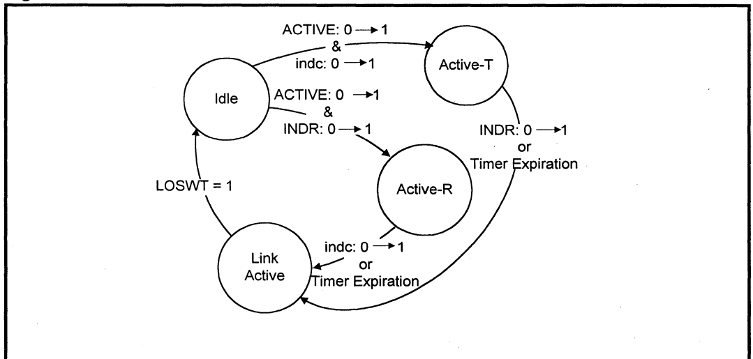
Figure 10: NTU HDSL Framing Activation State Machine
