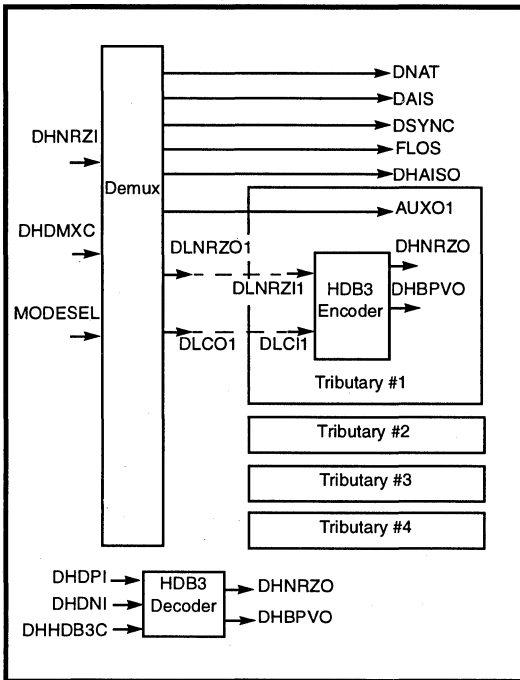
Figure 5: SXT6234 Demultiplexing Function
