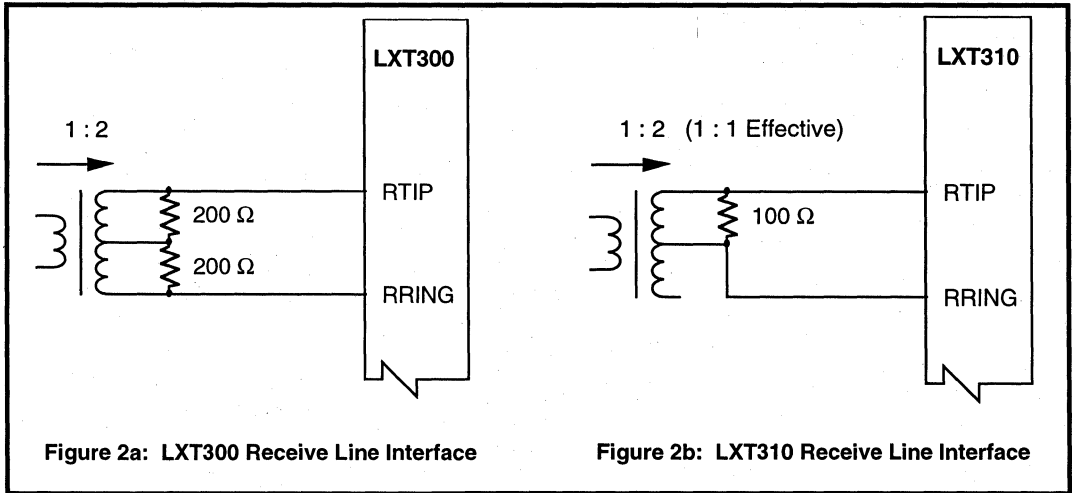
Figure 2: Receive Line Interface
