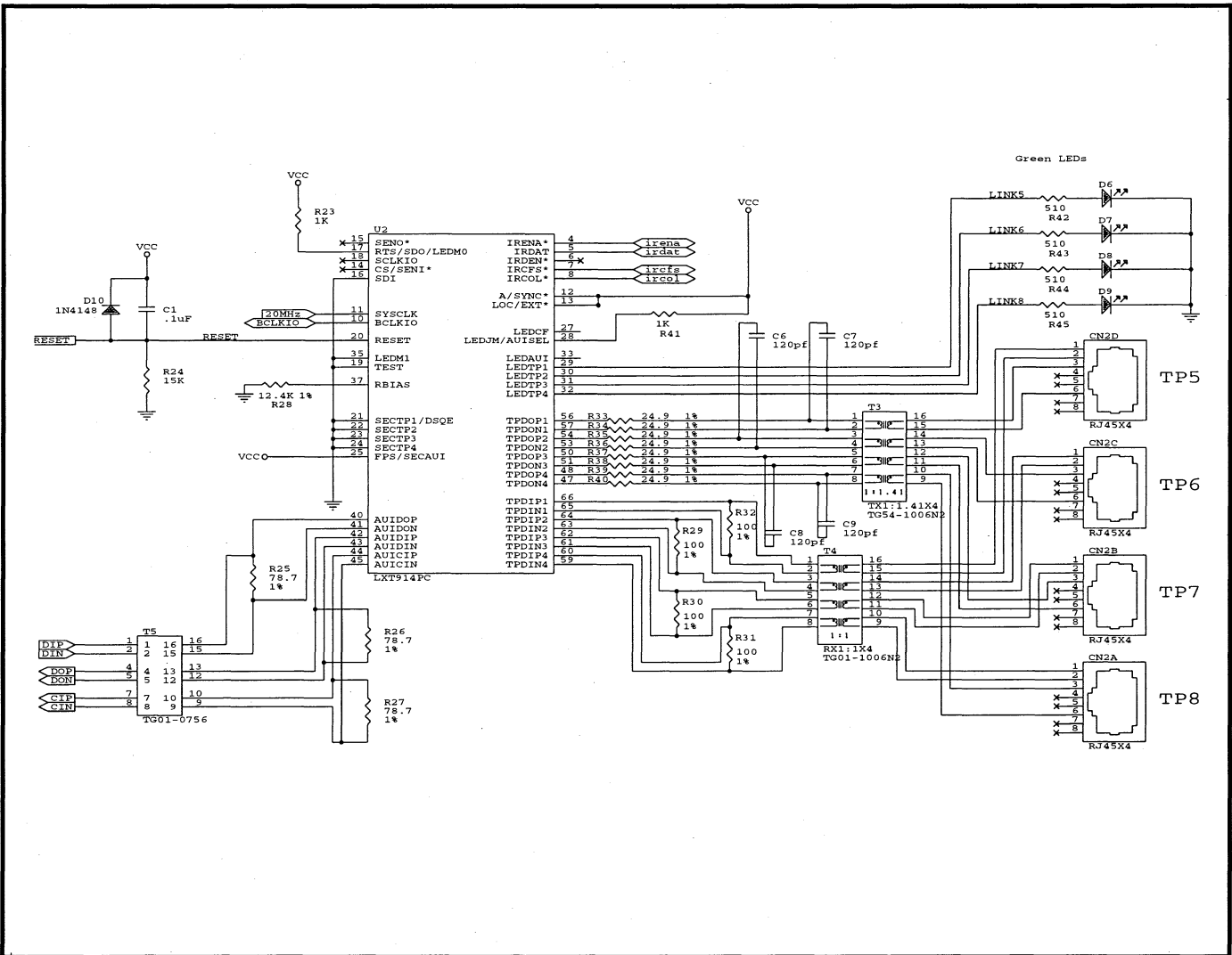
Figure 6: 8-Port Application Schematic, LED Mode 1 with AUISEL = MAU (Sheet 2 of 2)
