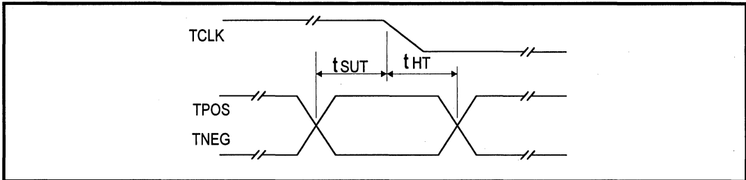
Figure 12: LXT317 Transmit Clock Timing
