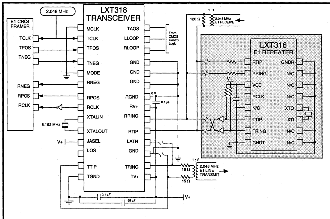
Figure 1: Long-Haul E1 1-Chip Solution (LXT318)
