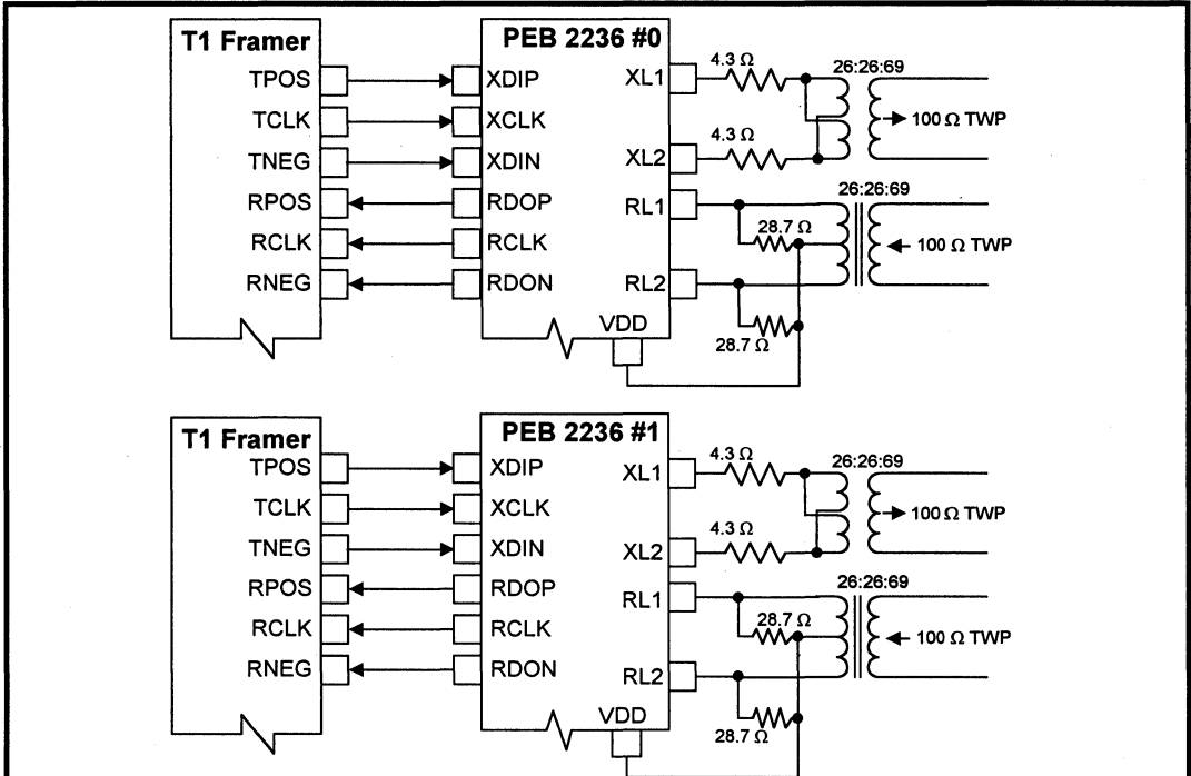
Figure 1A: PEB 2236 100 Ω T1 Line Interface
