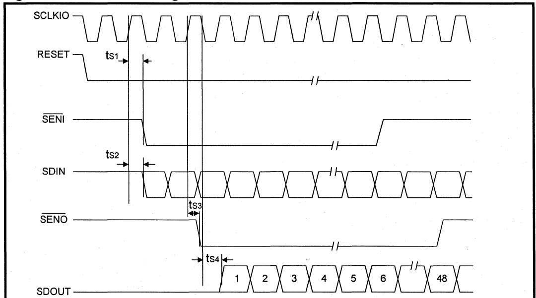
Figure 7: Serial Port Timing
