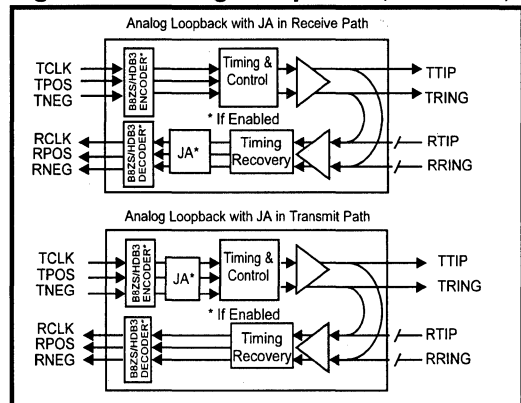
Figure 7: Analog Loopback (JA Selected)
