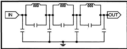
Figure 10: LXT902 Internal MAU Application Diagram
