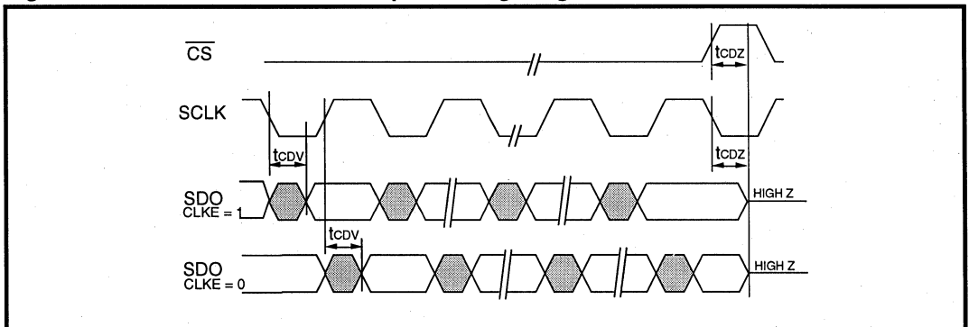
Figure 12: LXT310 Serial Data Output Timing Diagram
