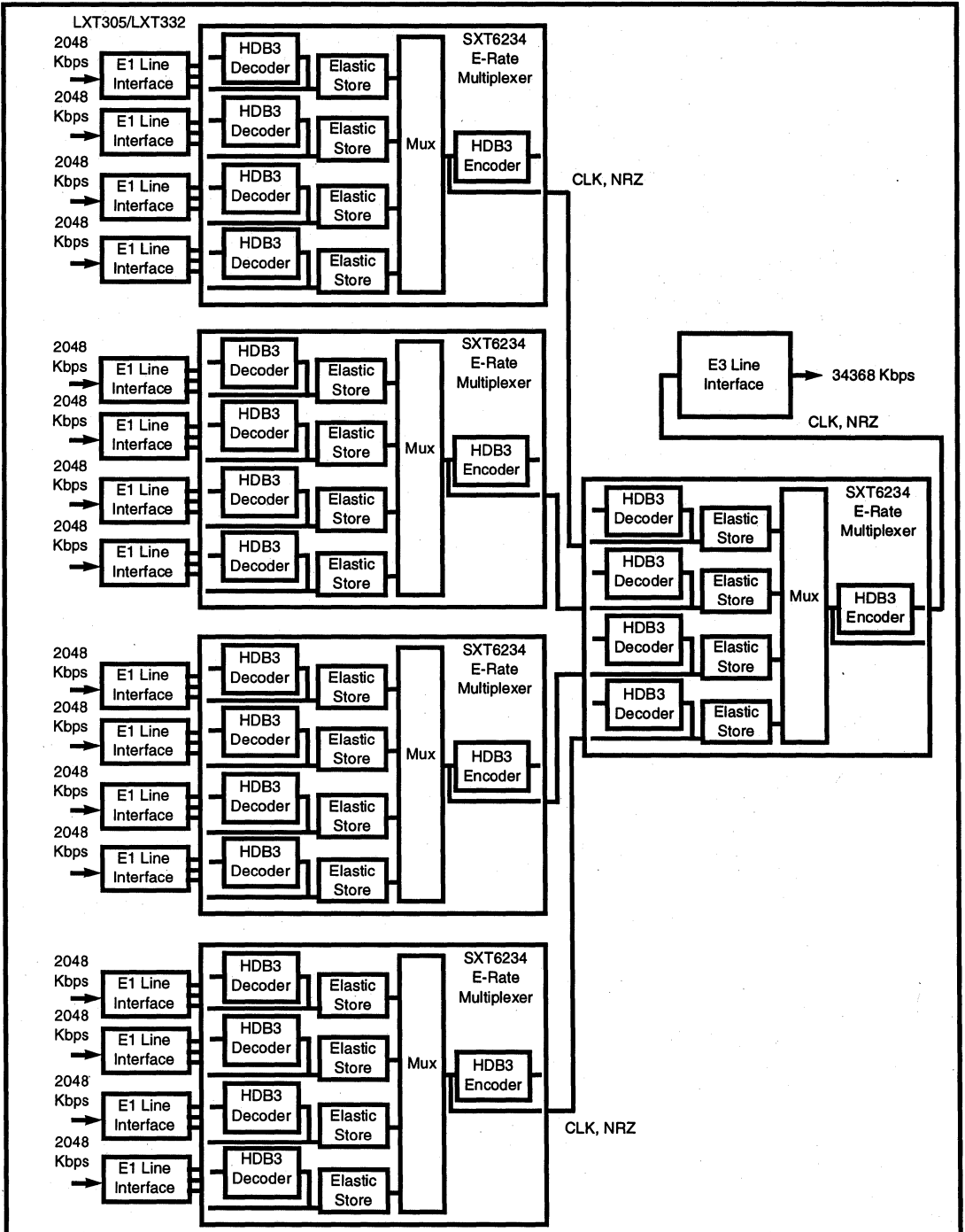
Figure 4: E1/E3 Multiplexer
