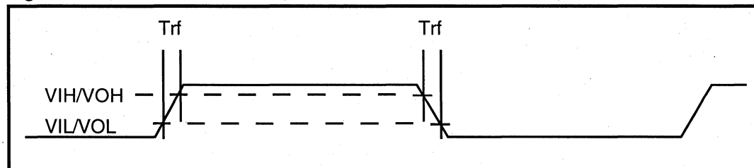
Figure 6: Rise and Fall Times
