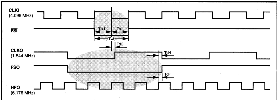
Figure 8: LXP604 High to Low Frequency Conversion Frame Sync Alignment
