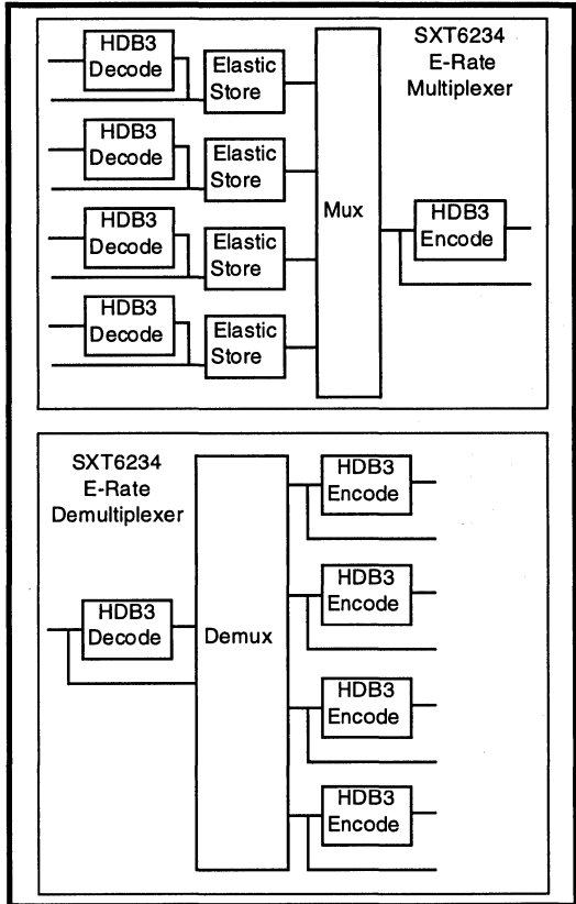
Figure 1: SXT6234 E-Rate Multiplexer
