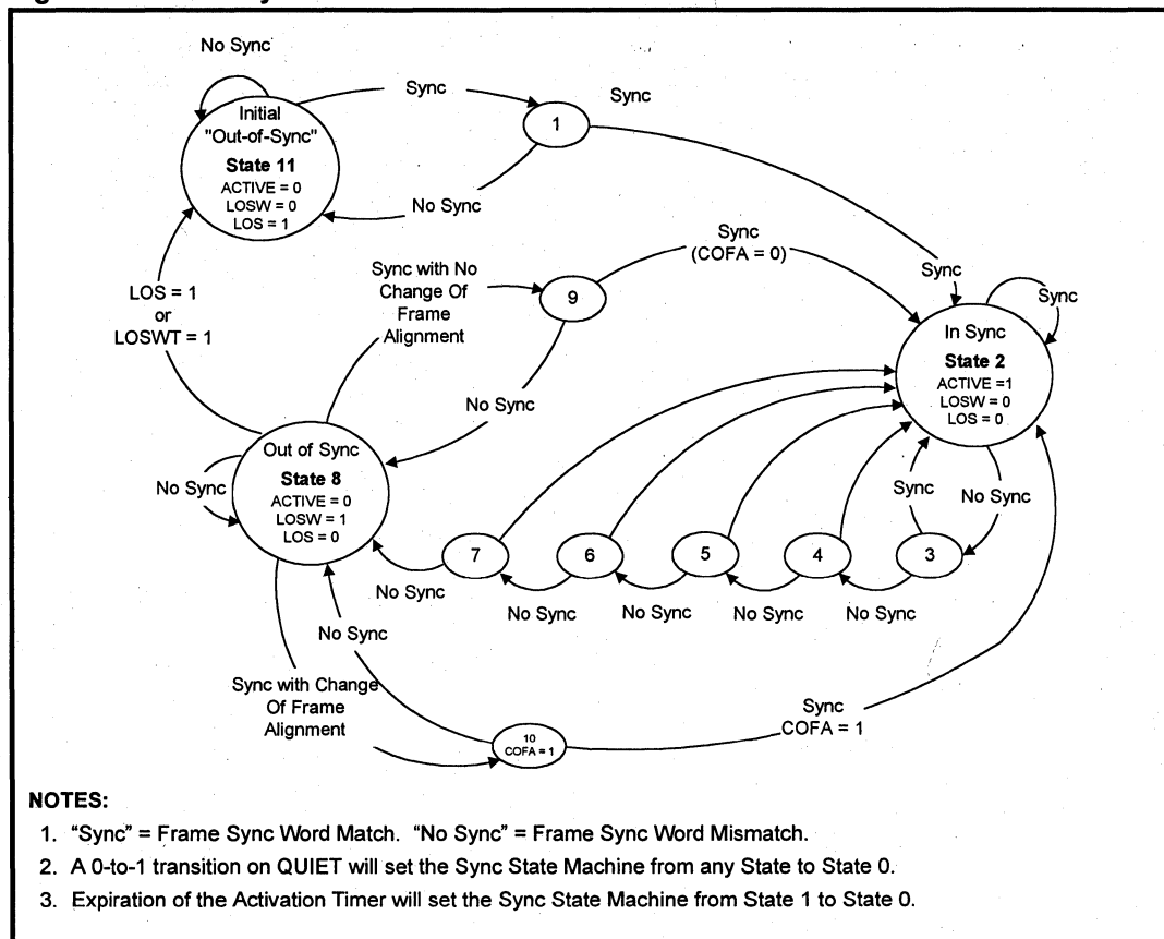
Figure 11: HDSL Synchronization State Machine
