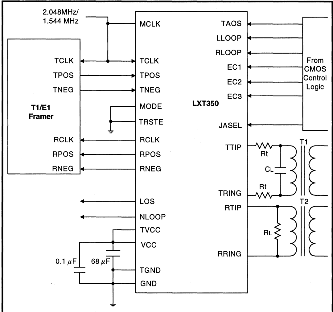
Figure 13: Typical T1/E1 LXT350 Hardware Mode Application
