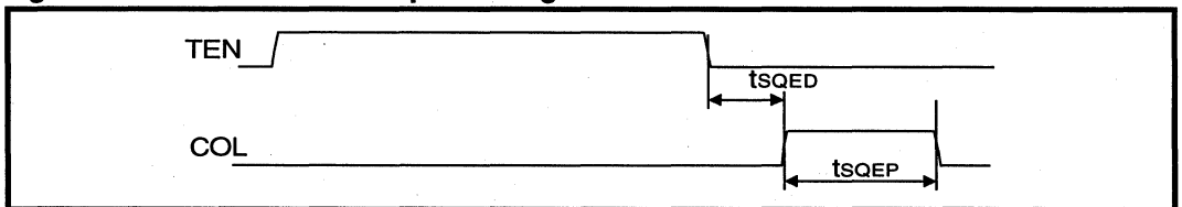
Figure 8: Mode 1 Loopback Timing
