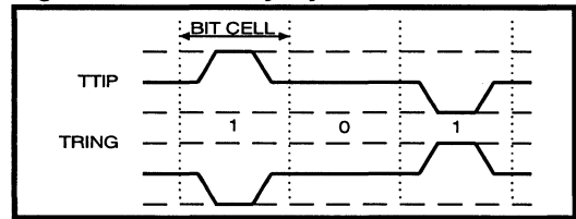
Figure 2: 50% Duty Cycle Transmit Pulse
