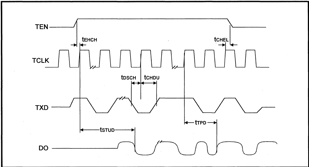
Figure 25: Mode 4 COL Output Timing
