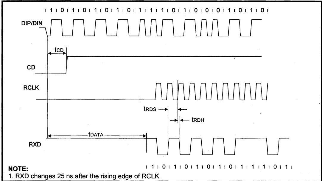
Figure 3: Mode 1 RCLK/Start-of-Frame Timing
