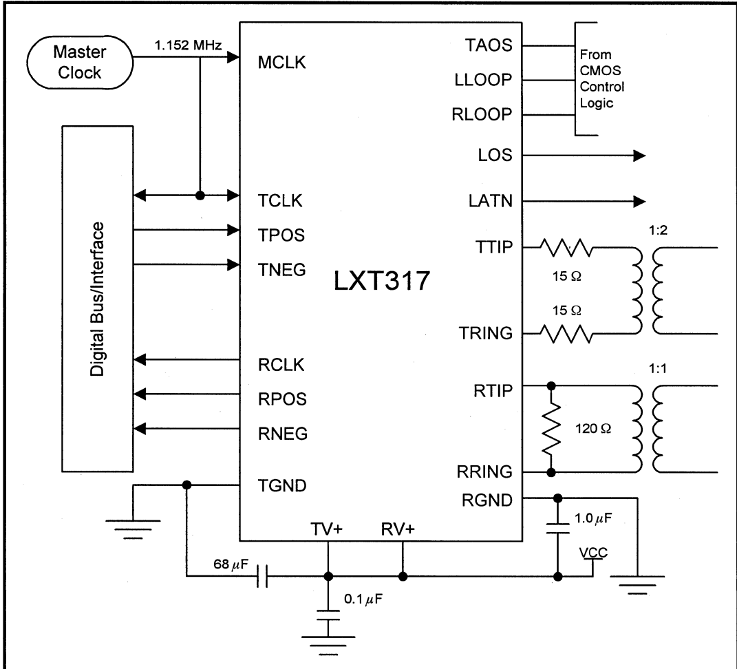
Figure 10: Typical LXT317 DECT Application
