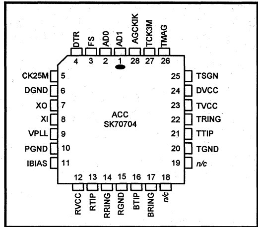
Figure 1: SK70704 ACC Pin Locations
