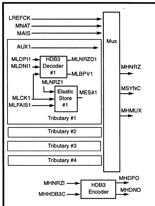
Figure 3: SXT6234 Multiplexing Function
