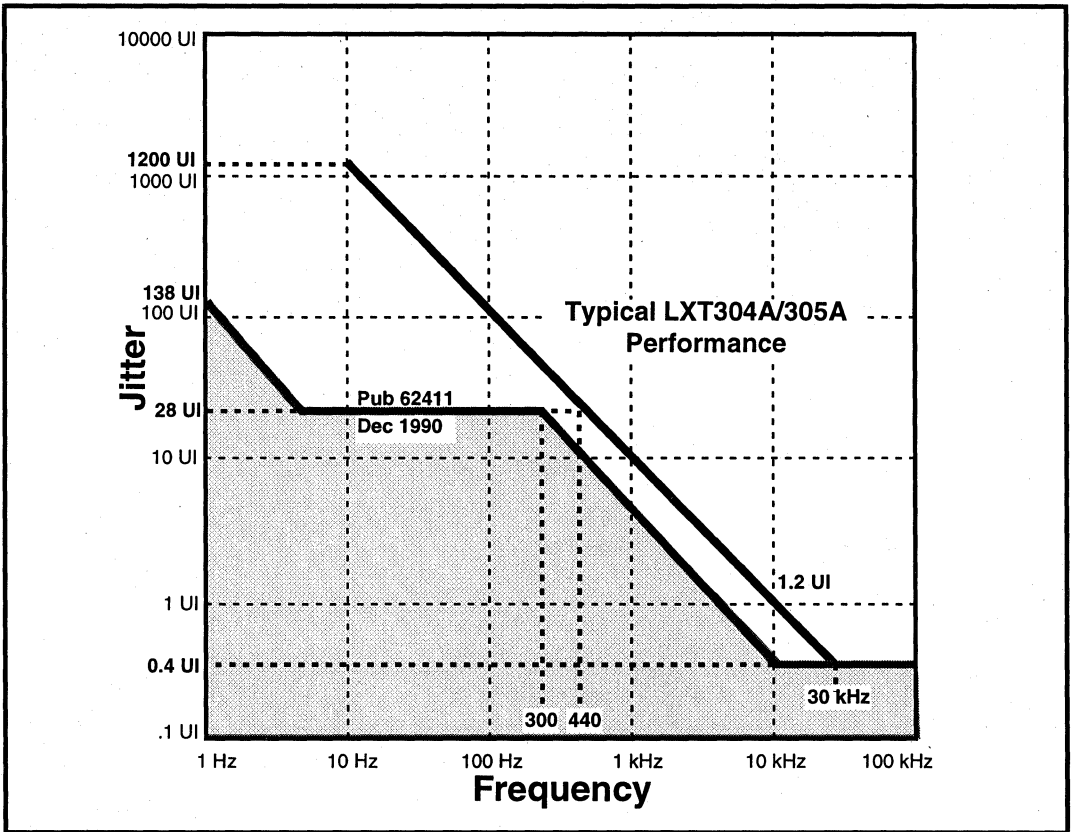
Figure 3: Charting Input Jitter Tolerance Test Results
