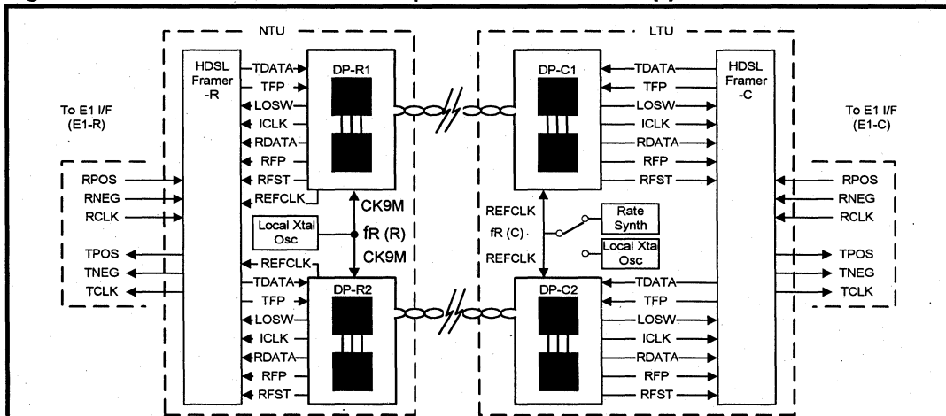
Figure 6: Model for HDSL Data Pump and HDSL Framer Applications
