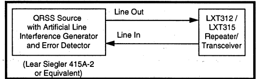
Figure 9: Receiver Gaussian Noise Immunity Test Setup
