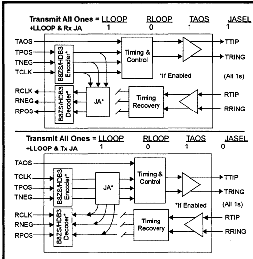
Figure 9: Local Loopback with Selectable JA
