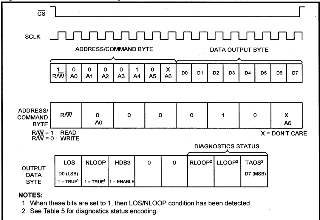
Figure 5: LXT318 Serial I/O Output Data Structure
