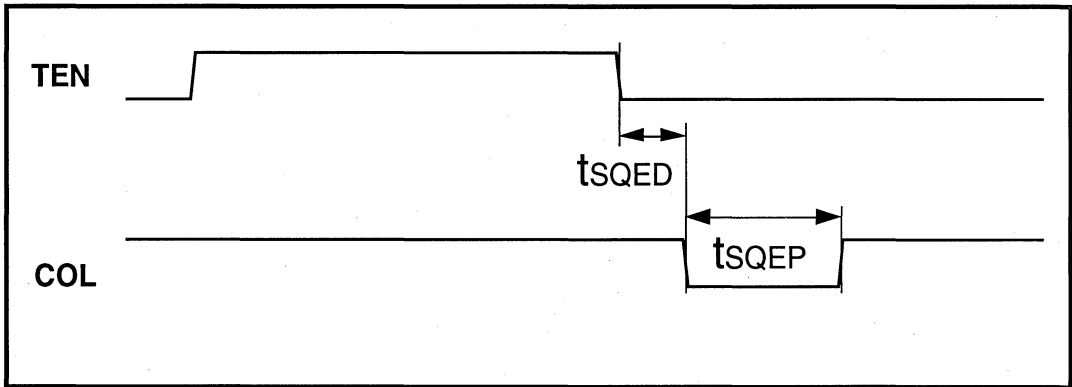
Figure 25: Mode 4 COL Output Timing
