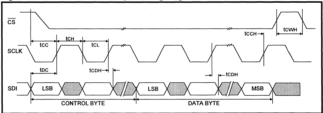
Figure 15: LXT307 Serial Data Input Timing Diagram
