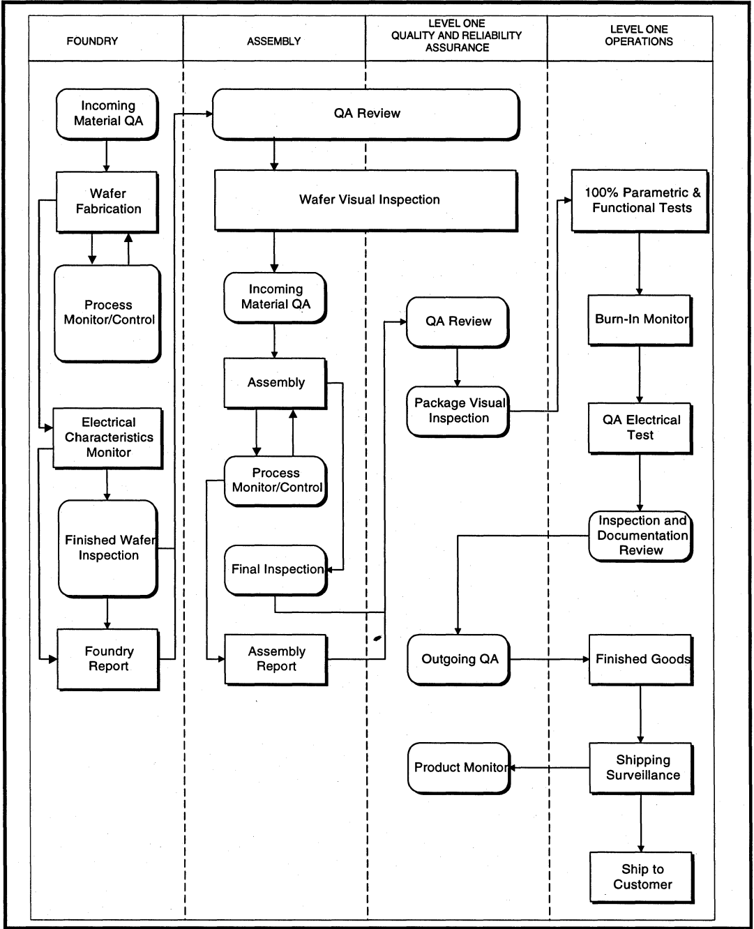
Figure 1: Level One Production Flow
