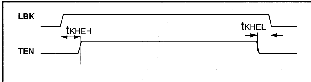
Figure 32: Mode 3 Loopback Timing
