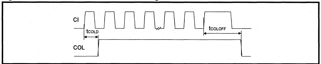
Figure 25: Mode 4 COL/CI Output Timing
