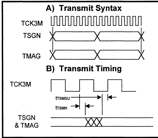
Figure 15: ACC Transmitter Timing
