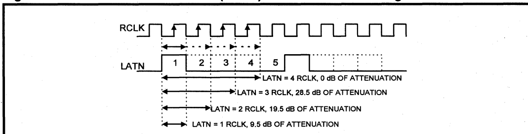
Figure 3: LXT318 Line Attenuation (LATN) Pulse Width Encoding
