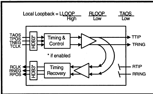
Figure 6: Local Loopback
