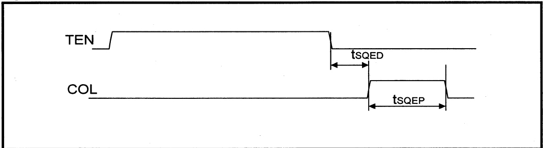
Figure 13: Mode 1 COL Output Timing
