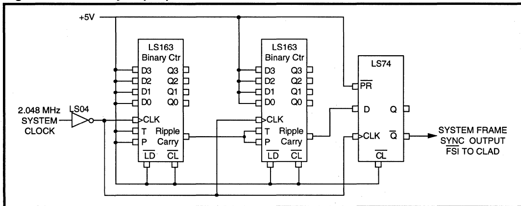
Figure 3: Frame Sync (FSI) Generation Circuit
