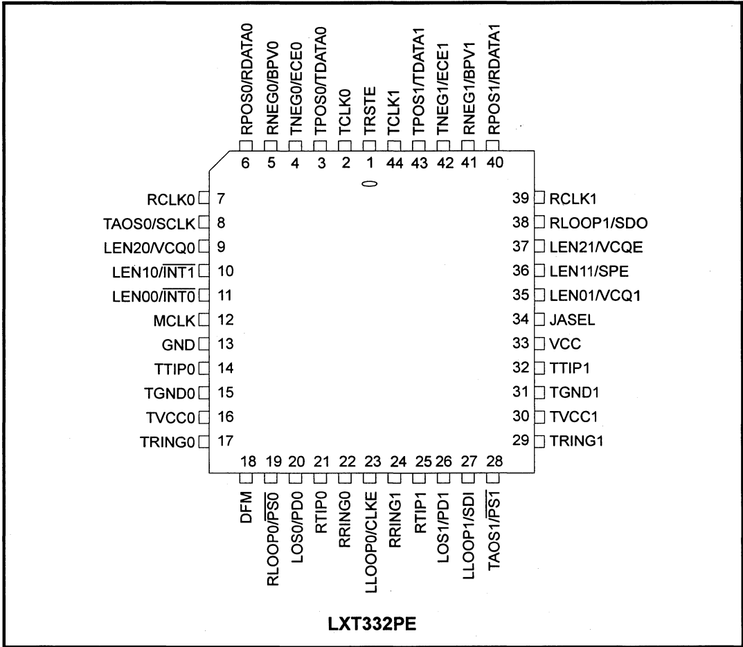
Figure 1: LXT332 Pin Assignments (PLCC Package)
