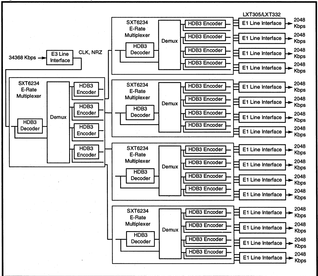
Figure 4: E1/E3 Demultiplexer
