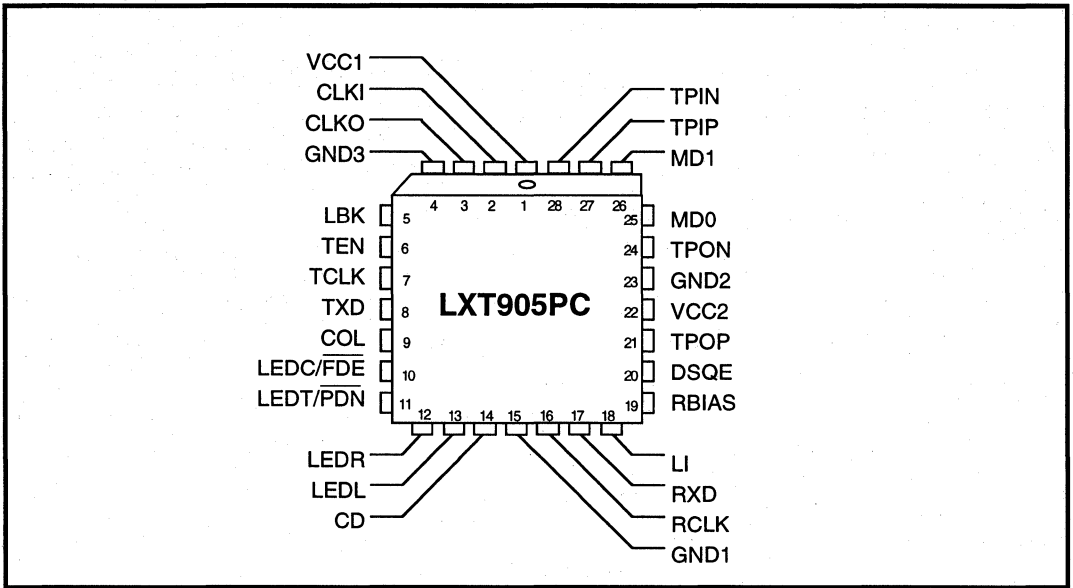
Figure 1: Pin Assignments
