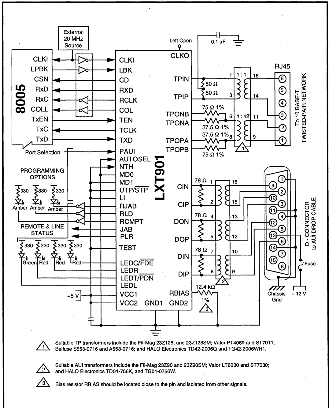
Figure 11: Manual Port Select with Seqq 8005 Controller
