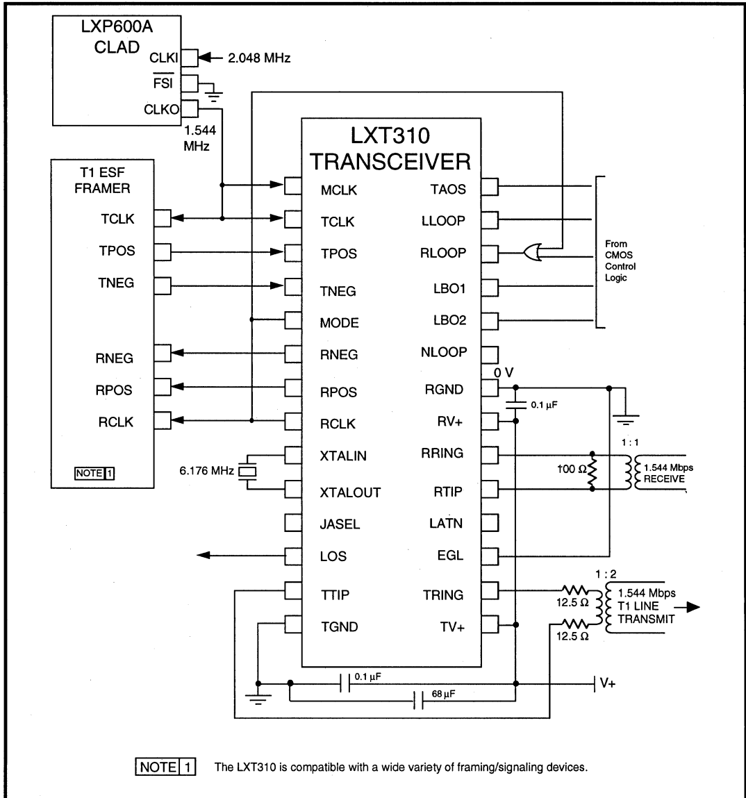
Figure 7: Typical LXT310 Hardware Mode Application
