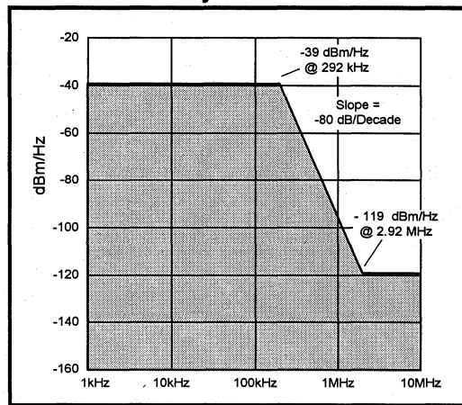
Figure 17: Transmit Power Spectral Density
