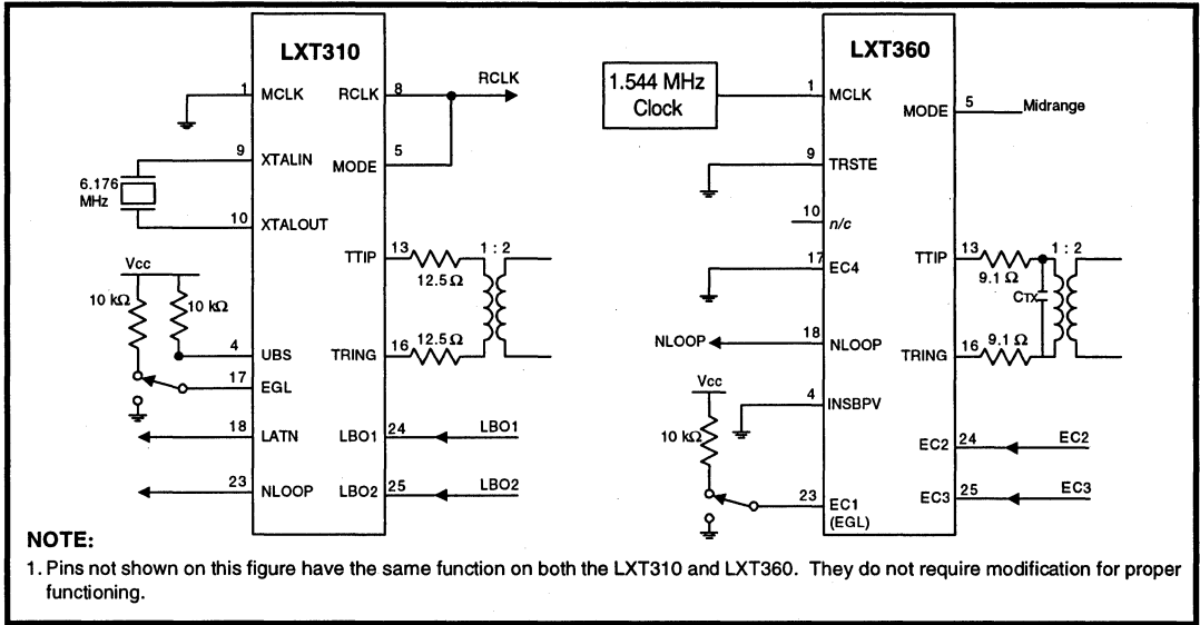
Figure 3: Unipolar Mode (with B8ZS Zero Suppression) 1
