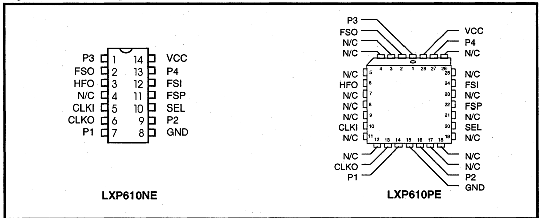
Figure 1: Pin Assignments
