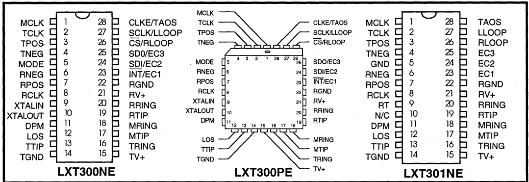
Figure 1: Pin Assignments
