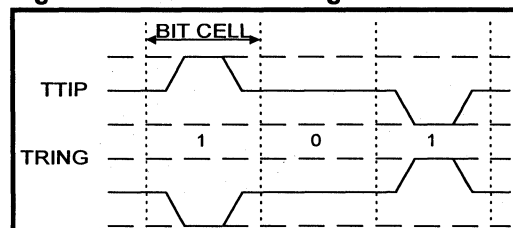
Figure 2: 50% AMI Coding
