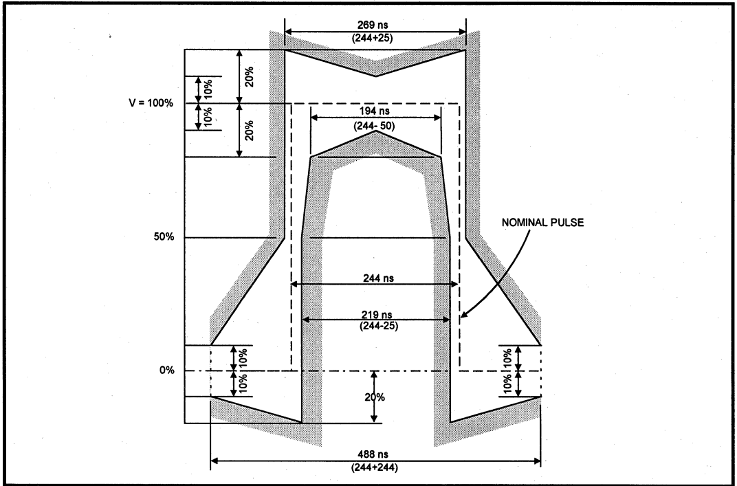
Figure 22: 2.048 Mbps Pulse Mask
