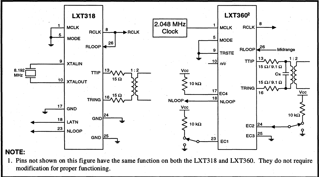
Figure 4: Bipolar Mode 1
