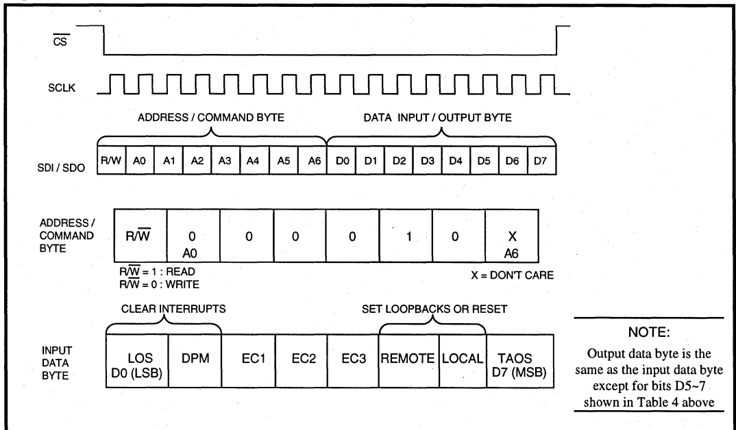
Figure 4: LXT300Z Serial Interface Data Structure
