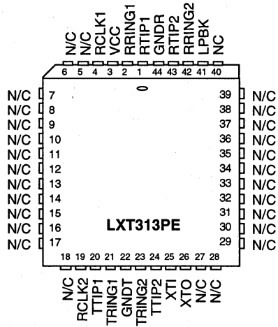
Figure 1: LXT313/316 Repeater/Transceiver Pin Assignments
