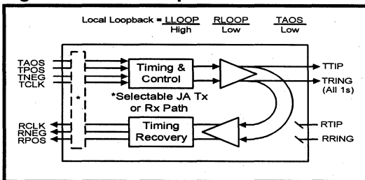
Figure 8: Local Loopback
