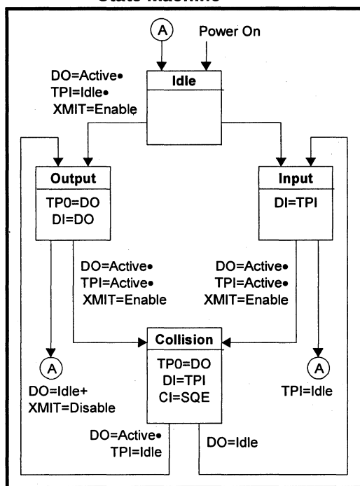
Figure 5: LXT944 Collision Detection State Machine
