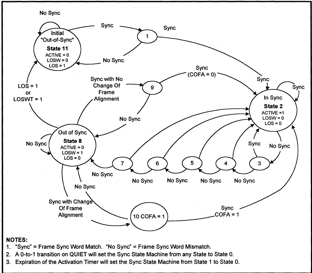
Figure 11: HDSL Synchronization State Machine
