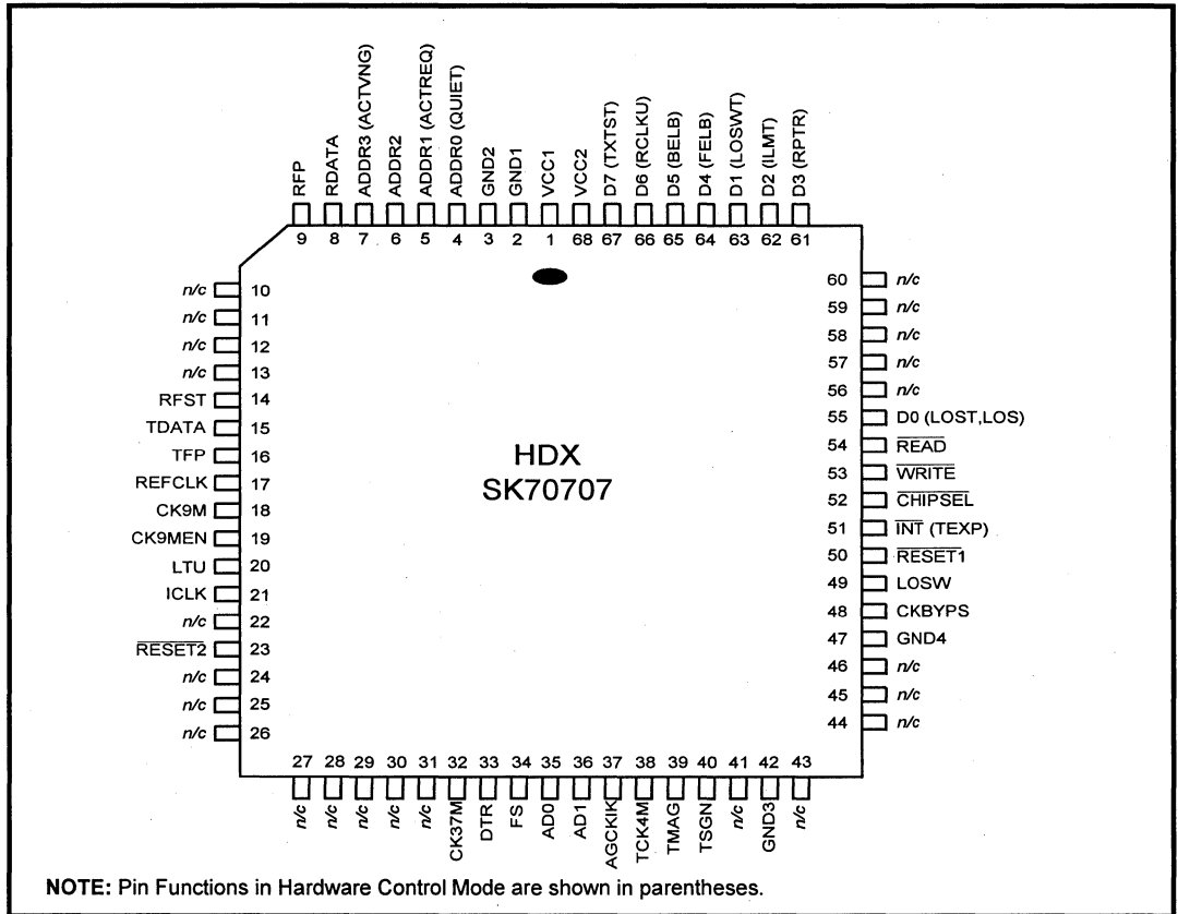
Figure 2: SK70707 HDX Pin Assignments
