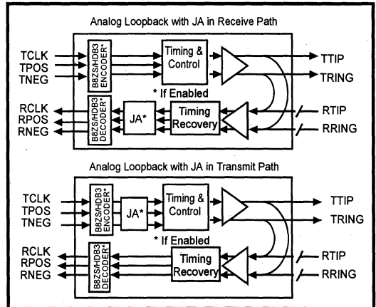
Figure 7: Analog Loopback (JA Selected)
