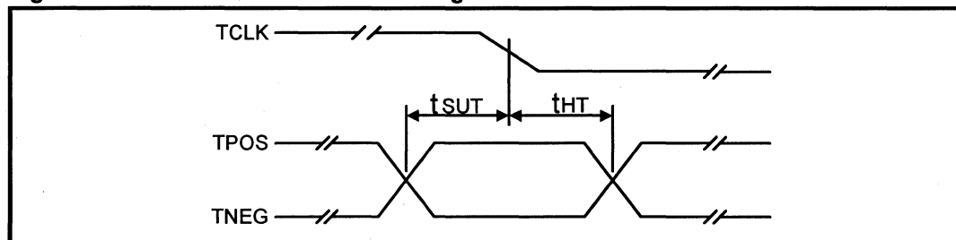
Figure 14: LXT318 Transmit Clock Timing
