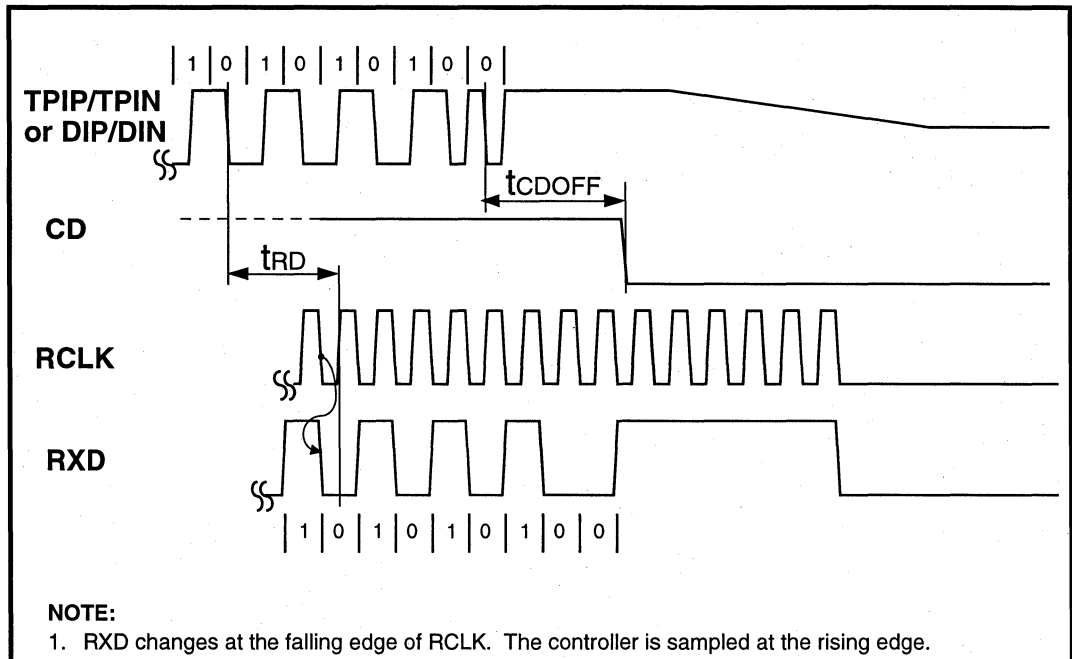
Figure 34: Mode 4 RCLK/End-of-Frame Timing
