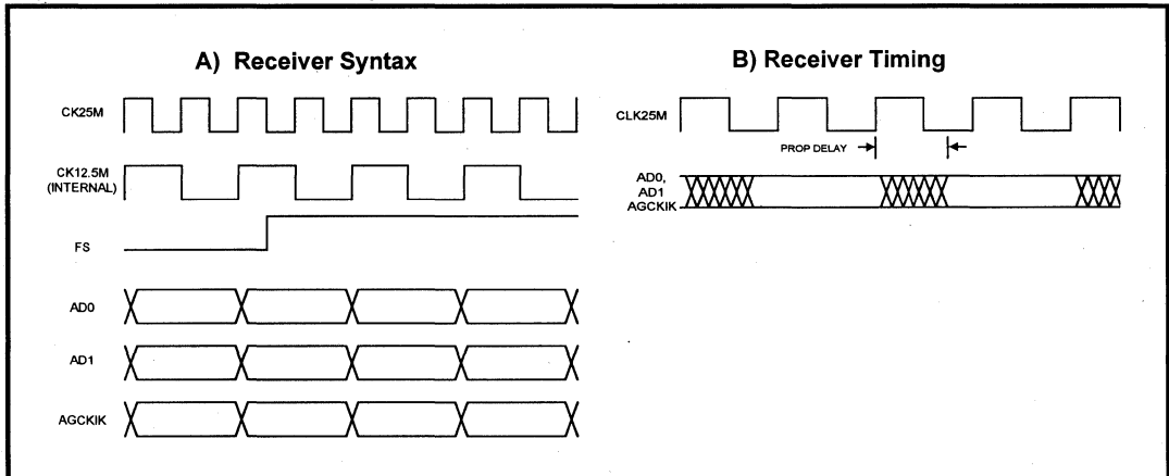
Figure 17: ACC Receiver Syntax and Timing
