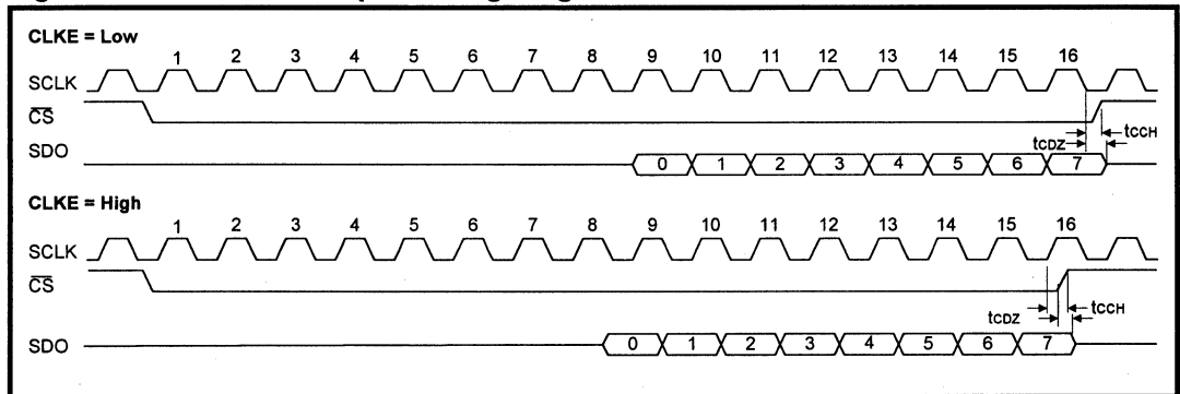
Figure 21: Serial Data Output Timing Diagram
