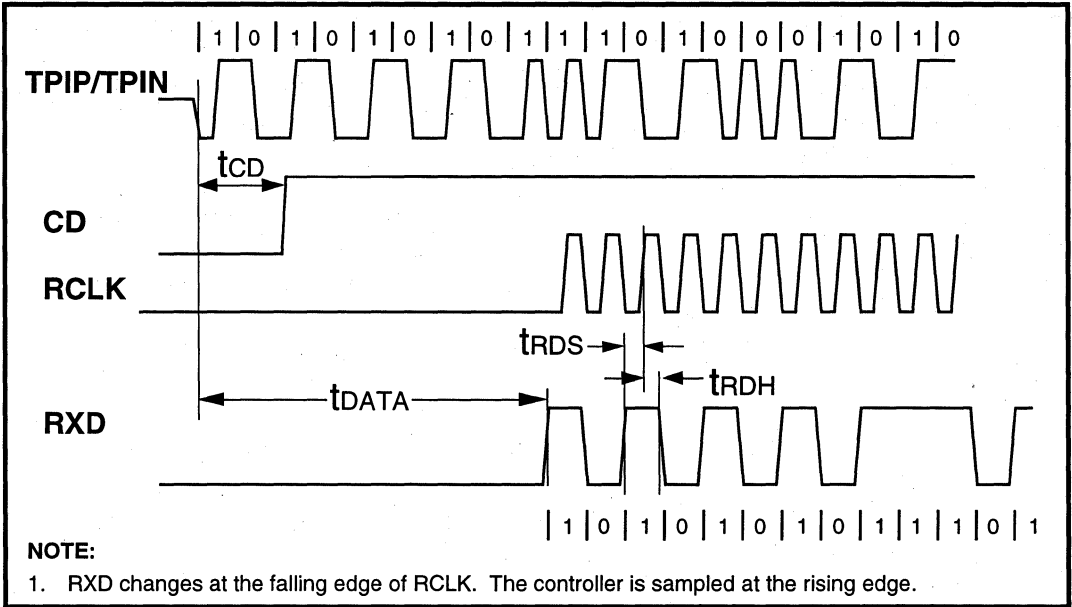
Figure 22: Mode 4 RCLK/Start of Frame Timing
