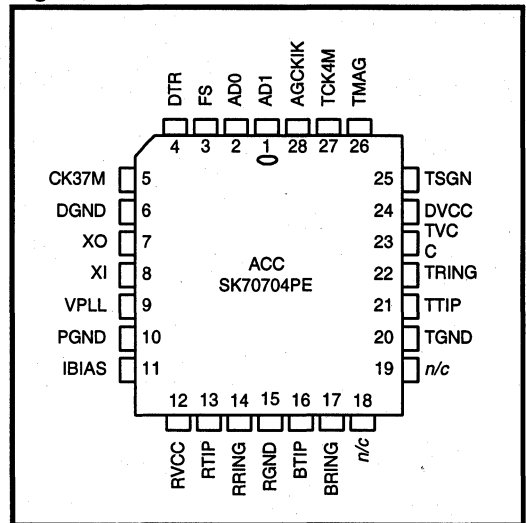
Figure 1: SK70704 ACC Pin Locations
