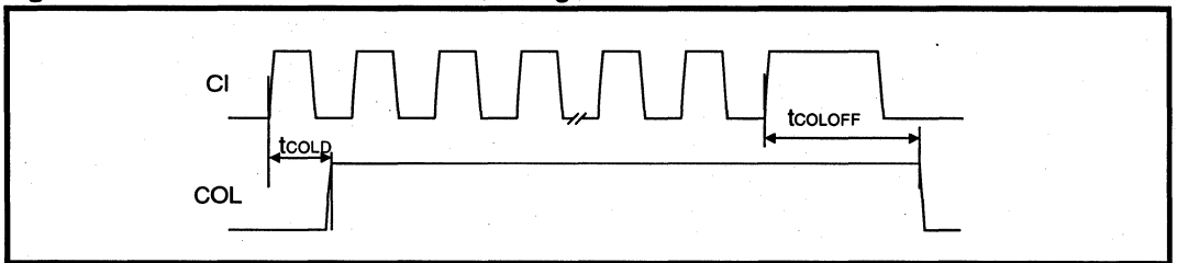
Figure 7: Mode 1 COL/CI Output Timing
