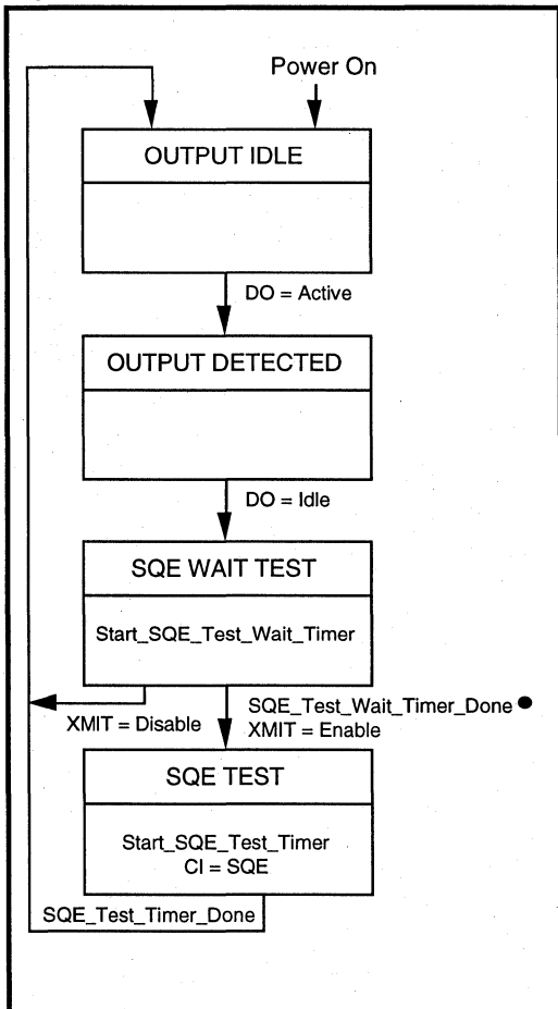
Figure 4: SQE Test Function
