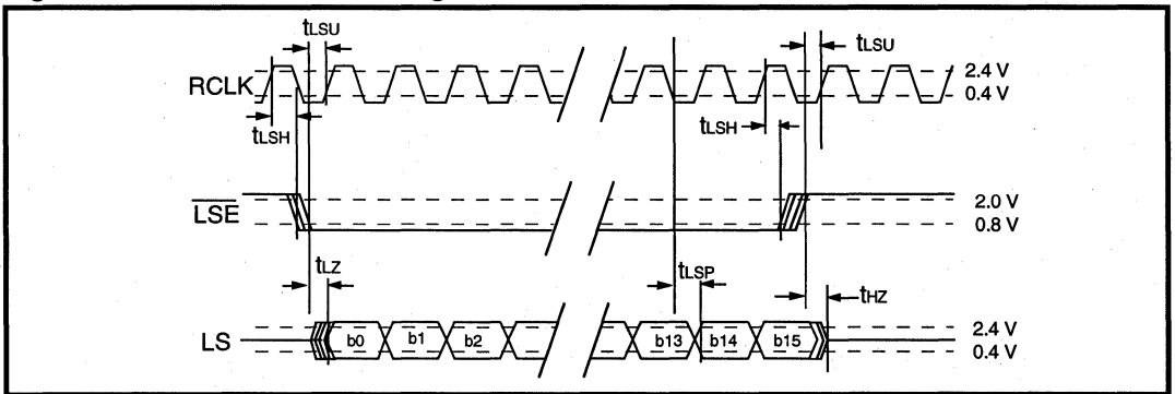
Figure 13: LS Serial Port Timing - 16-Bit Word
