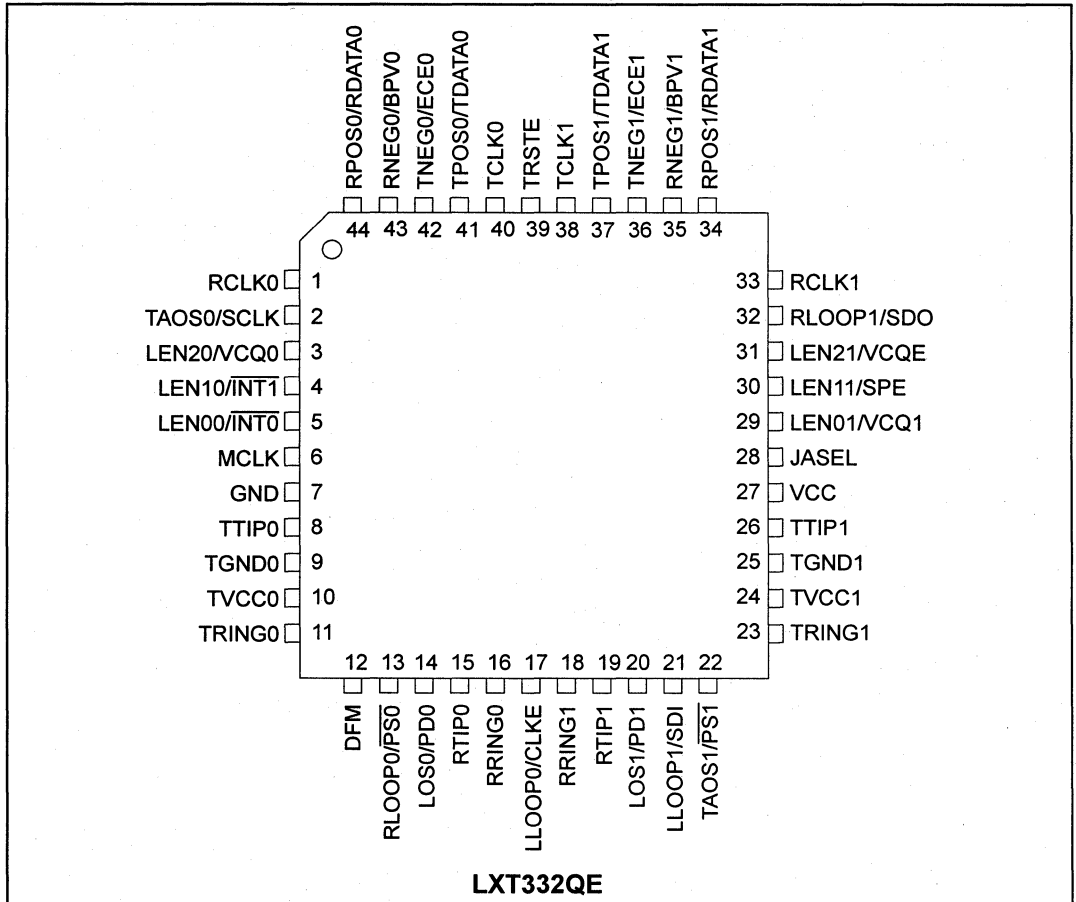
Figure 2: LXT332 Pin Assignments (QFP Package)
