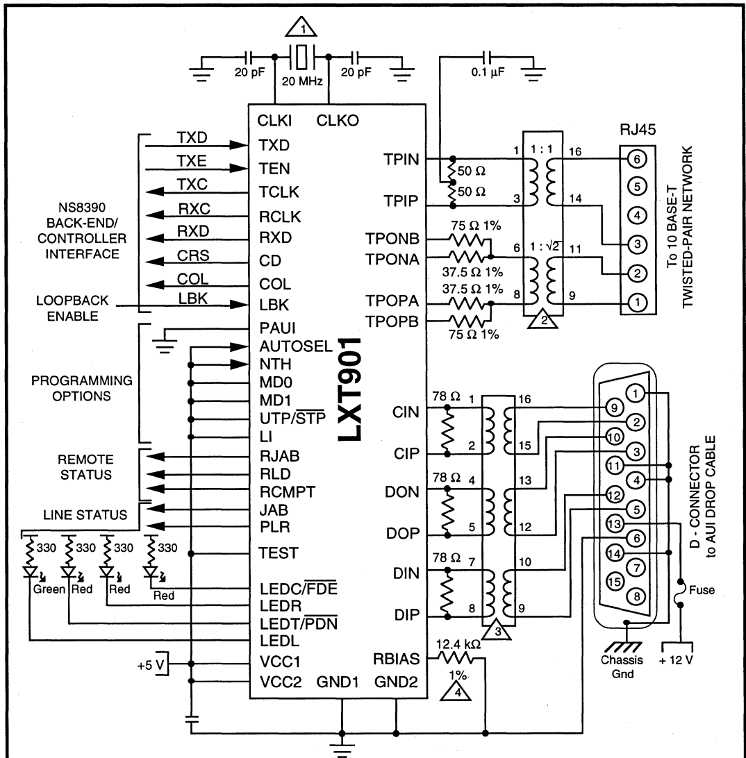
Figure 8: LAN Adapter Board - Auto Port Select with External LPBK Control
