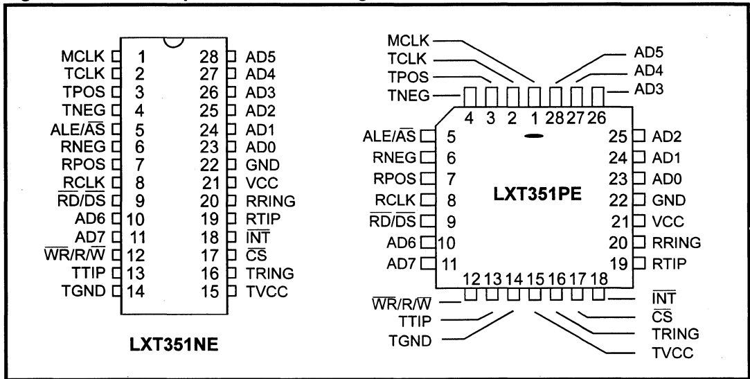
Figure 2: LXT351 Bipolar Mode Pin Assignments
