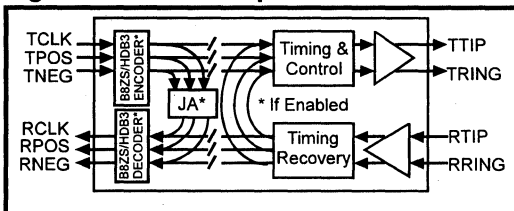
Figure 9: Dual Loopback
