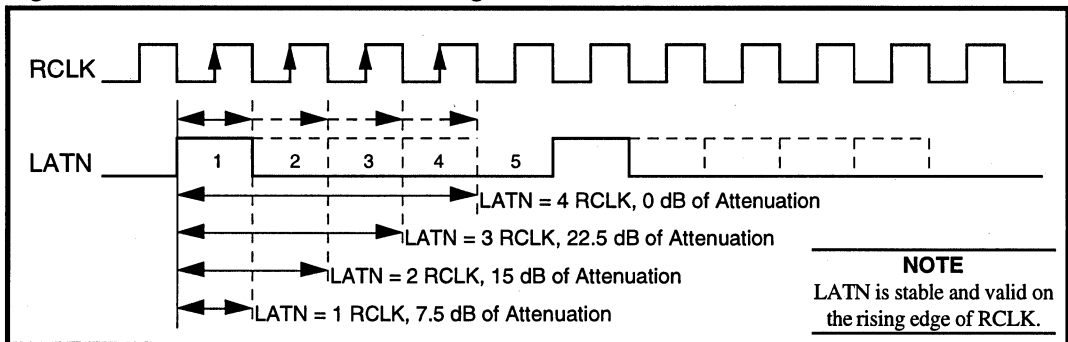
Figure 2: LATN Pulse Width Encoding
