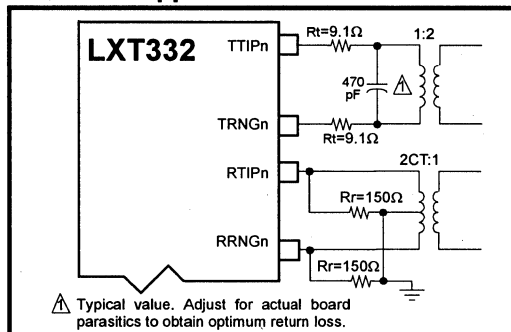
Figure 14: Line Interface for E1 Coax Applications
