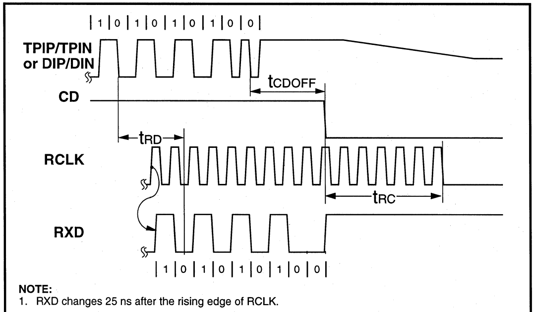
Figure 16: Mode 1 RCLK/End-of-Frame Timing
