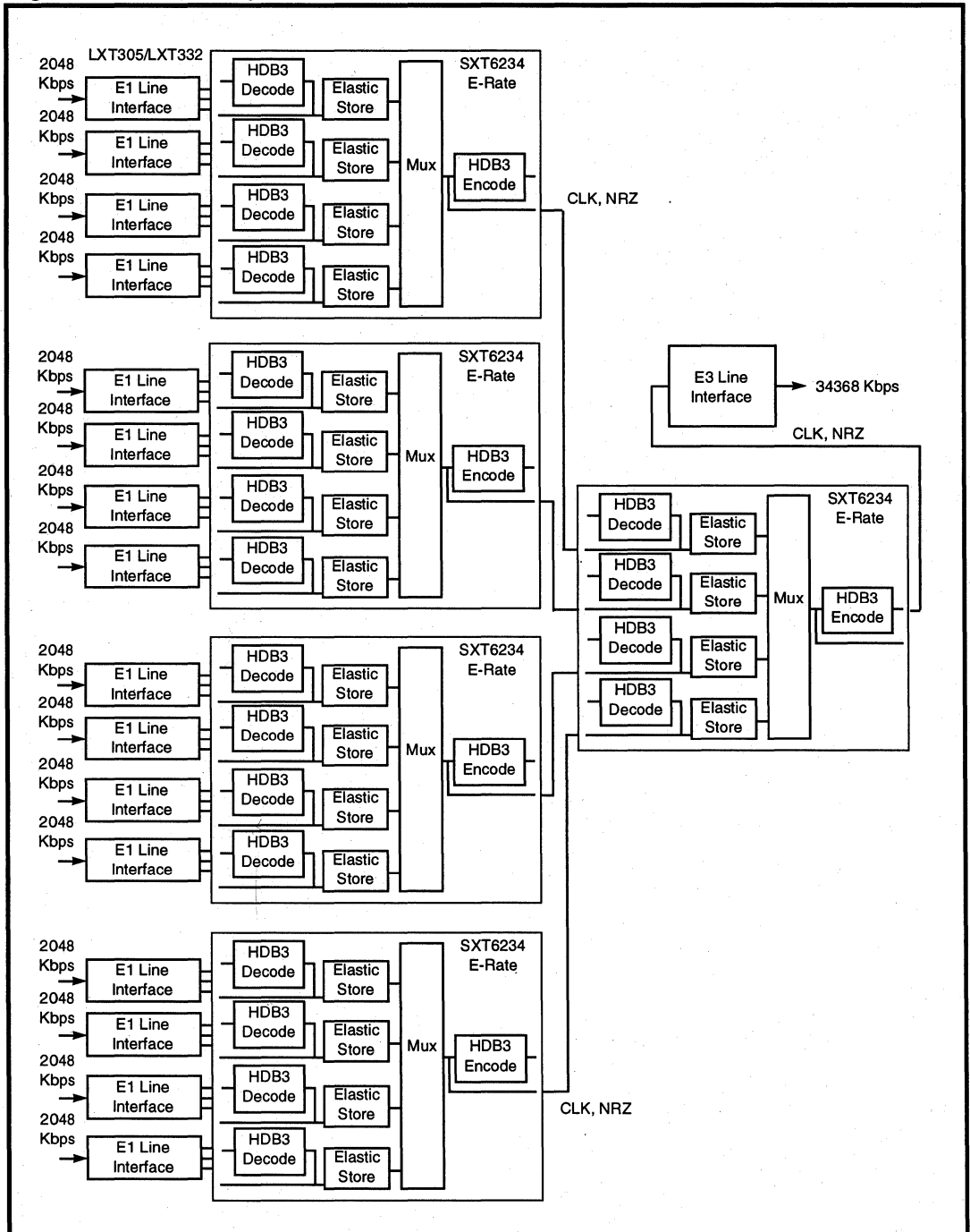
Figure 2: E1/E3 Multiplexer
