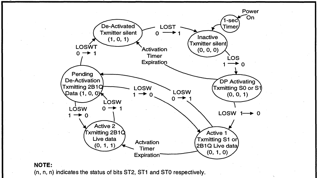
Figure 7: HTU-C Data Pump Activation State Machine
