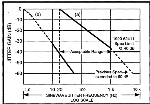
Figure 5: Jitter Transfer Template
