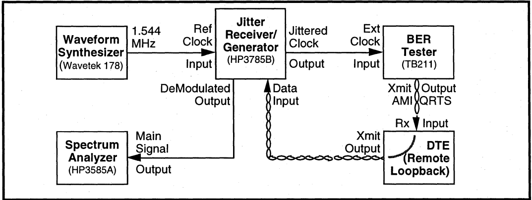
Figure 6: Jitter Attenuation Test Setup
