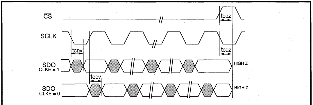
Figure 15: LXT300Z Serial Data Output Timing Diagram
