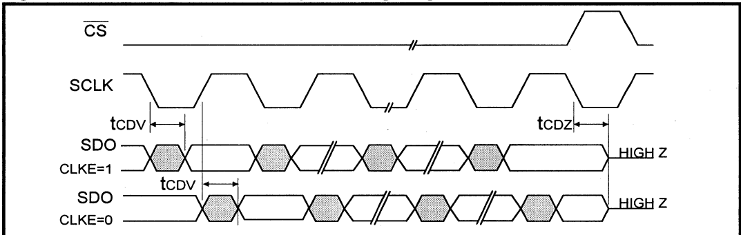
Figure 17: LXT318 Serial Data Output Timing Diagram
