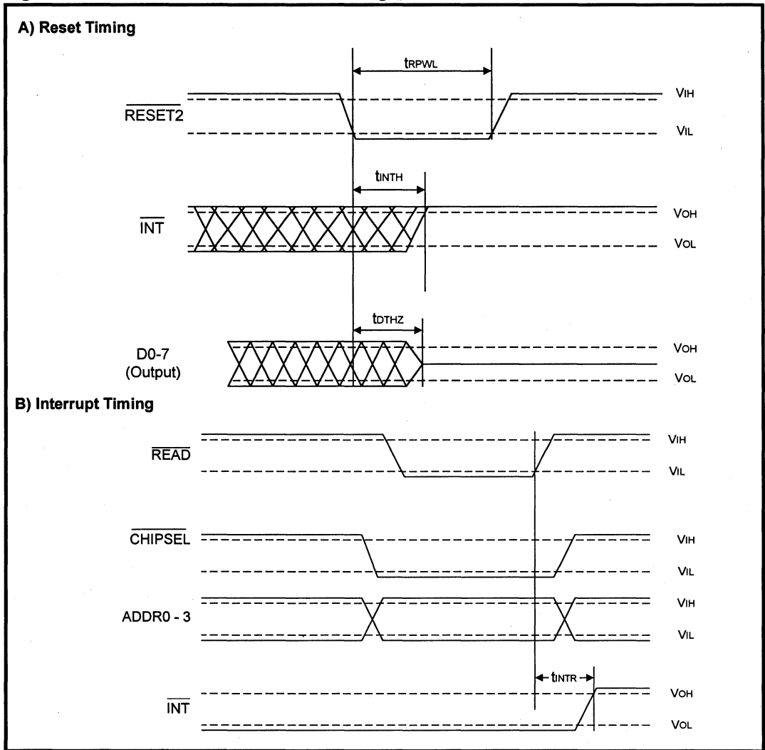
Figure 20: RESET and INTERRUPT Timing ( \mu P Control Mode)
