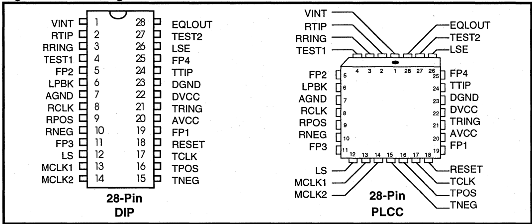
Figure 1: Pin Assignments
