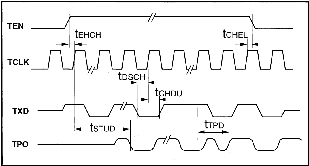
Figure 24: Mode 4 Transmit Timing
