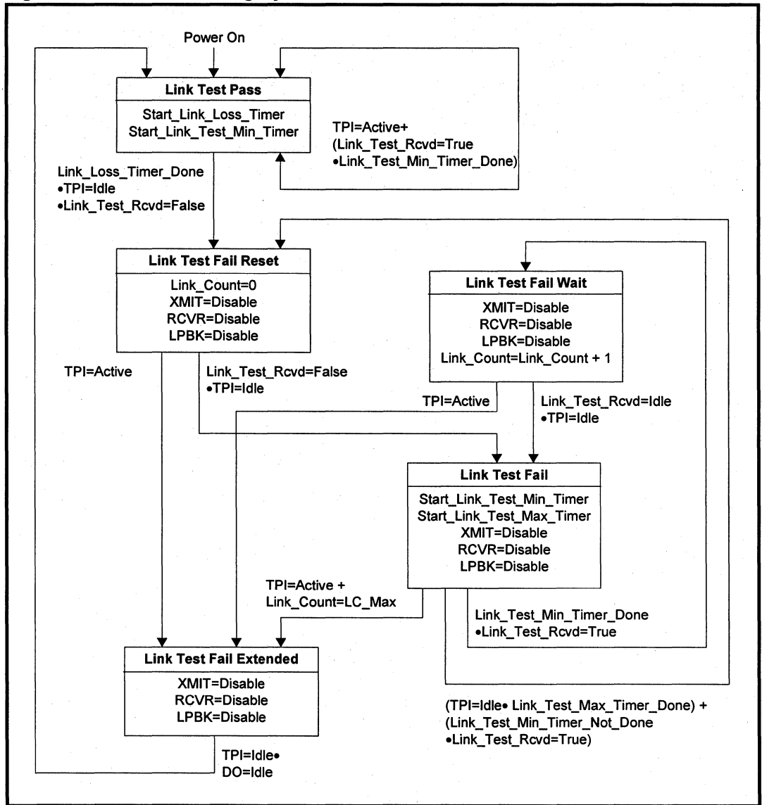
Figure 6: LXT944 Link Integrity Test Function State Machine
