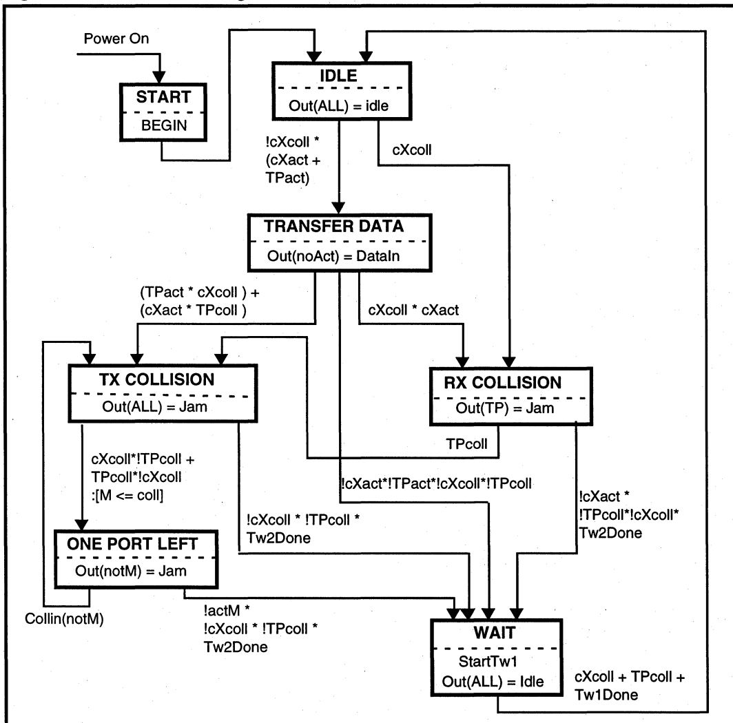
Figure 4: LXT906 State Diagram
