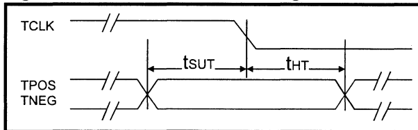
Figure 18: Transmit Clock Timing
