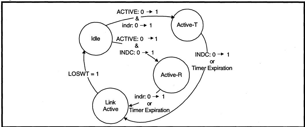
HTU-R Data Pump Activation
