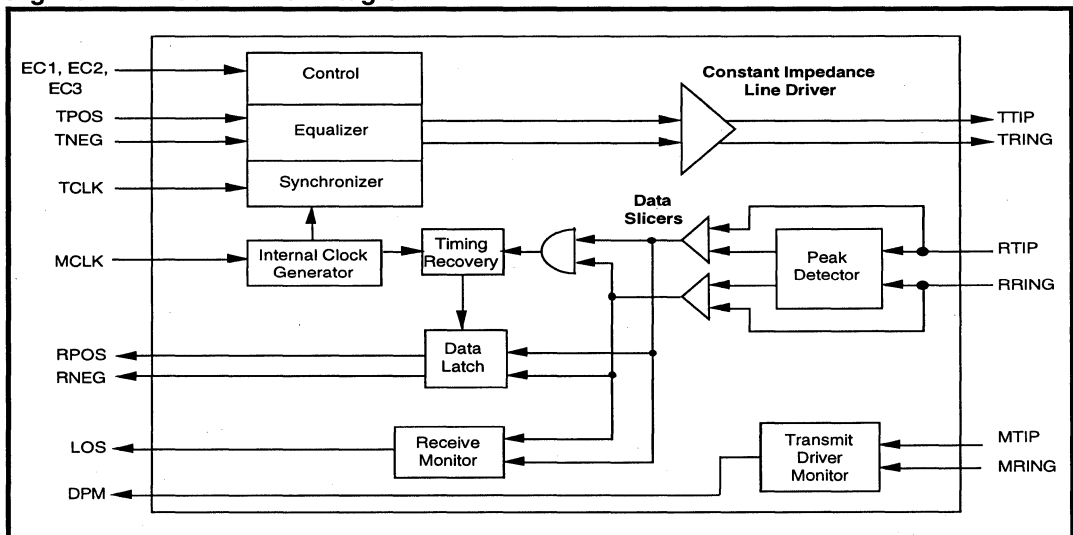
Figure 2: LXT301Z Block Diagram
