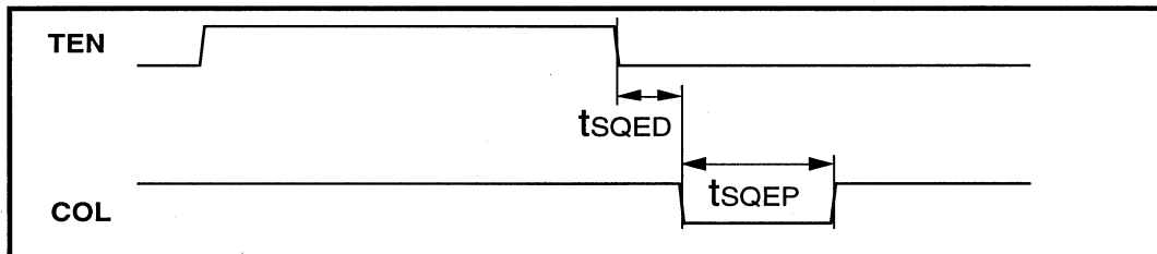
Figure 31: Mode 3 COL/CI Output Timing
