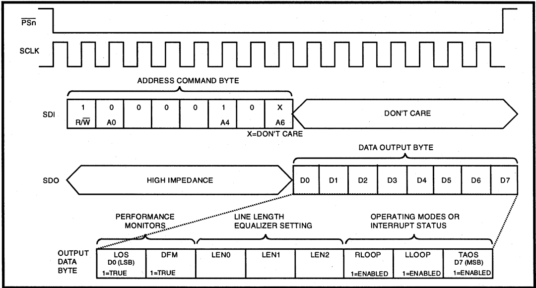
Figure 5: LXT332 SIO Read Operation
