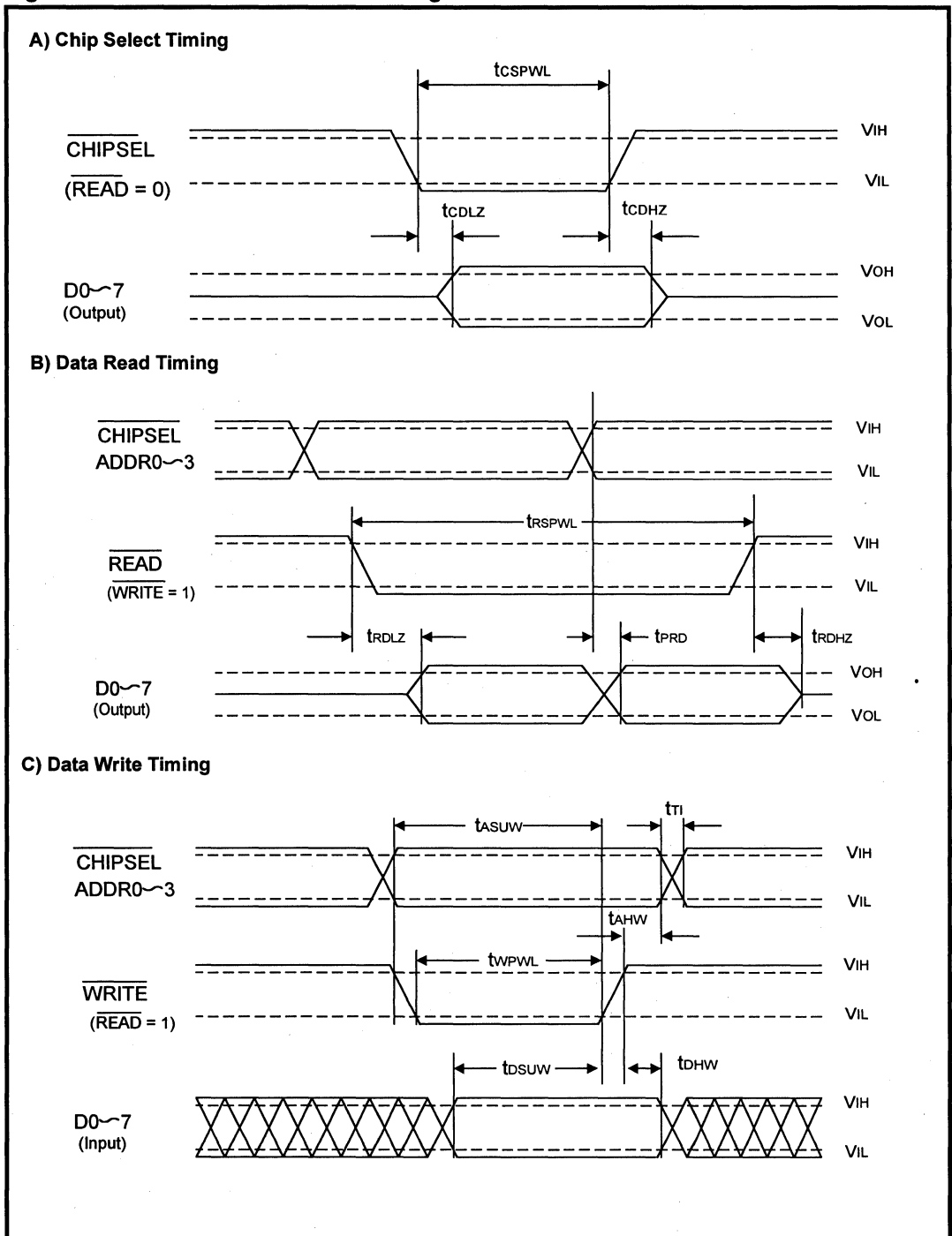
Figure 20: Parallel Data Channel Timing
