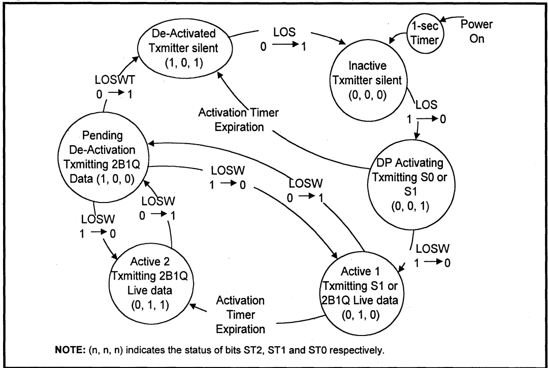
Figure 10: NTU HDSL Framing Activation State Machine
