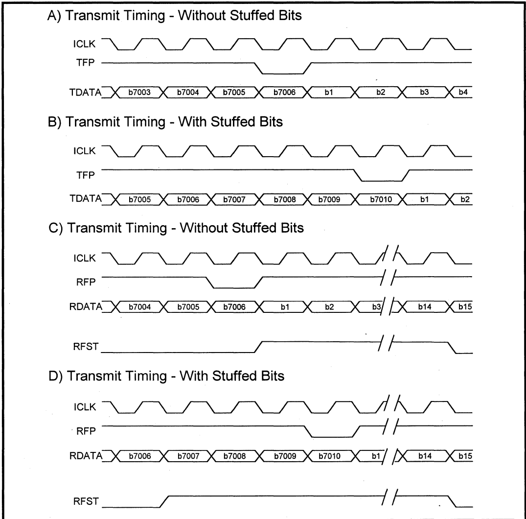
Figure 5: HDX/ACC Framer Interface – Relative Timing
