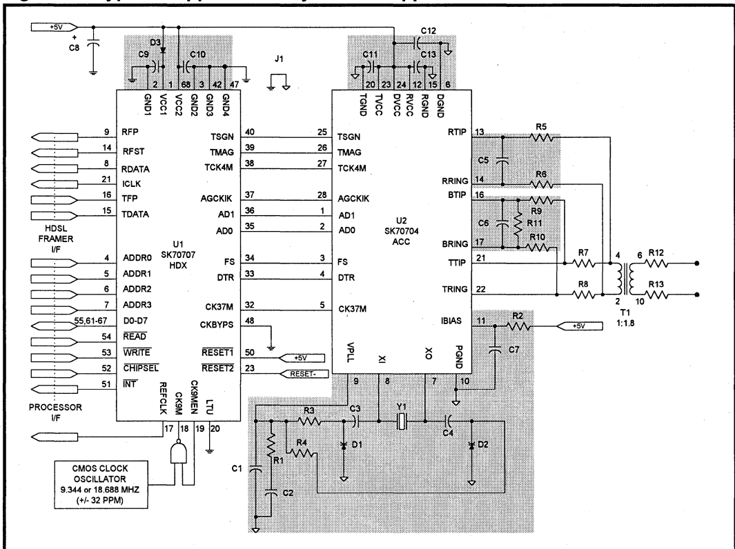
Figure 14: Typical Support Circuitry for NTU Applications
