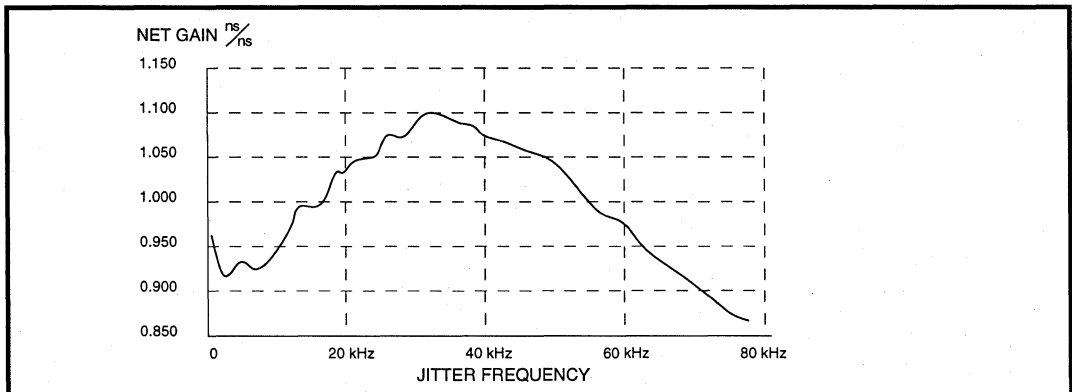
Figure 5: Nominal Jitter Transfer - 1.544 MHz CLKI to 2.048 MHz CLKO (Input Jitter = 0.25 UI)
