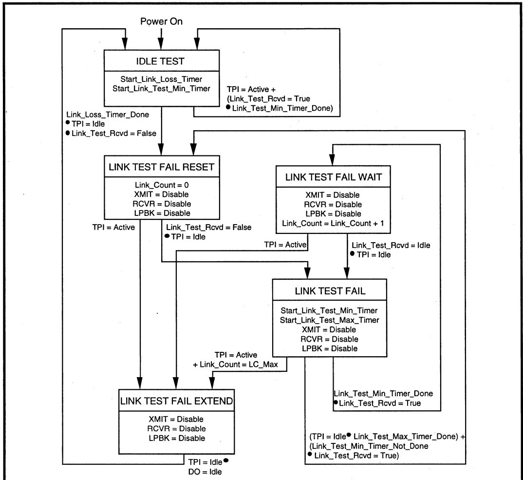
Figure 6: Link Integrity Test Function
