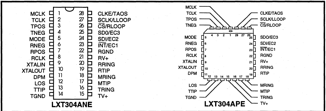
Figure 1: Pin Assignments
