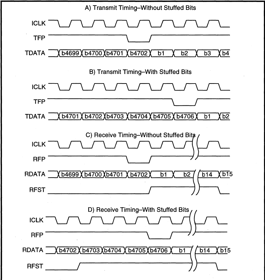
Figure 5: HDX/ACC Framer Interface – Relative Timing
