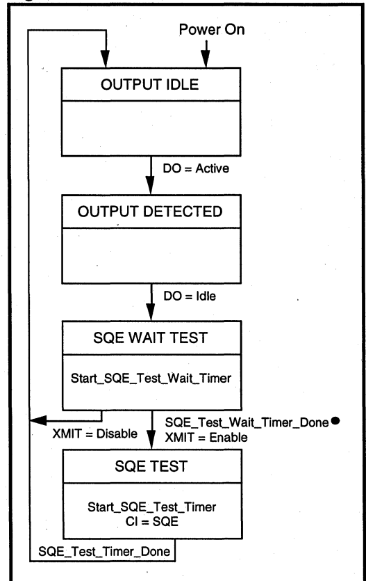
Figure 4: SQE Function
