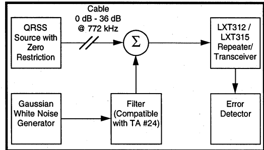
Figure 9: Receiver Gaussian Noise Immunity Test Setup
