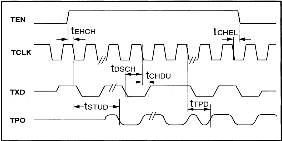
Figure 20: Mode 3 Transmit Timing
