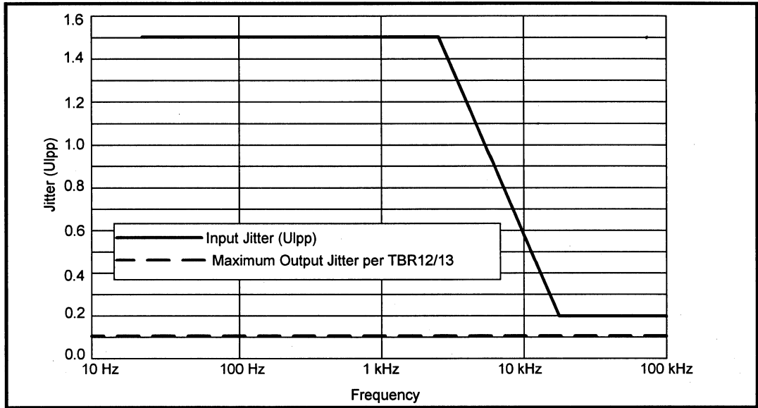
Figure 21: LXT318 Jitter Attenuation Performance (Typical-Measured Against TBR12/13)
