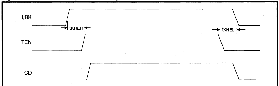
Figure 20: Mode 3 Loopback Timing
