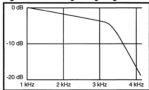
Figure 2: C-Message Weighting
