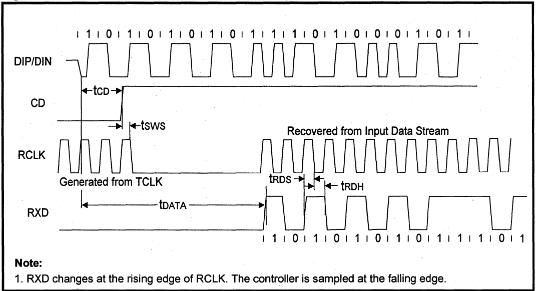
Figure 19: Mode 3 RCLK/End-of-Frame Timing
