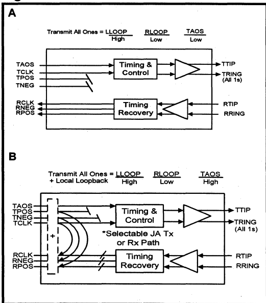
Figure 8: Local Loopback
