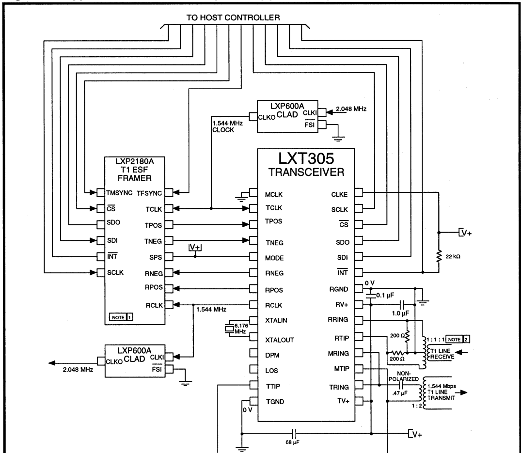
Figure 4: Typical LXT305 1.544 Mbps T1 Application (Host Mode)
