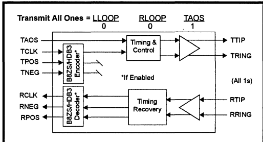
Figure 8: TAOS with LLOOP & Selectable JA
