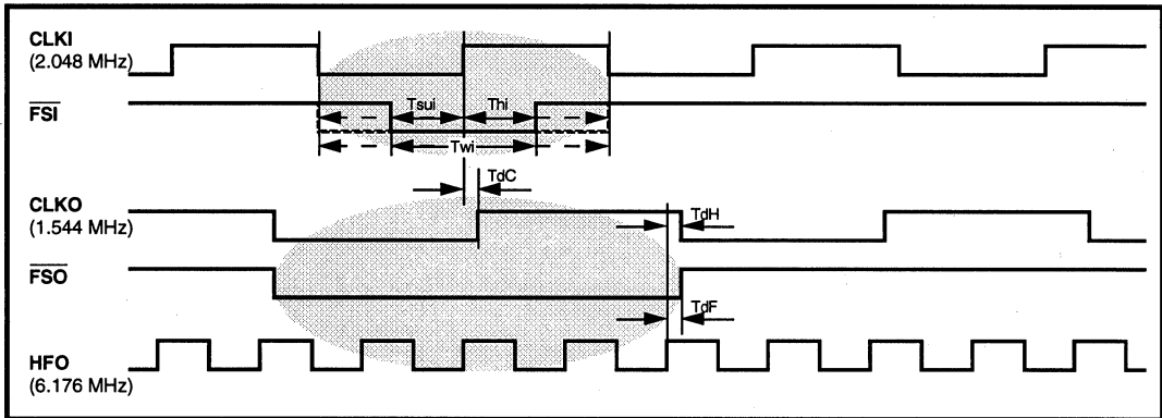
Figure 7: LXP600A and LXP602 High to Low Frequency Conversion Frame Sync Alignment
