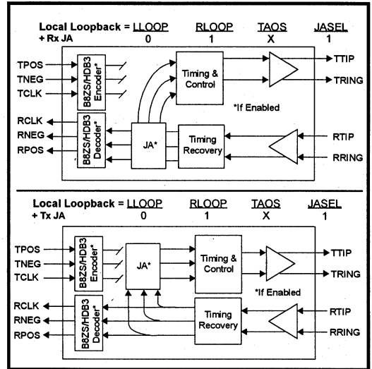
Figure 11: Dual Loopback
