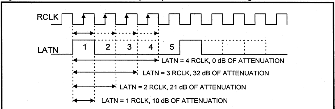
Figure 5: LXT317 Line Attenuation (LATN) Pulse Width Encoding
