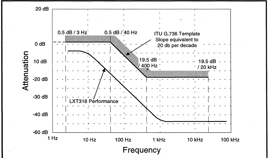
Figure 19: LXT318 Jitter Attenuation (Typical)
