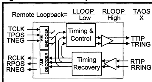
Figure 9: Remote Loopback
