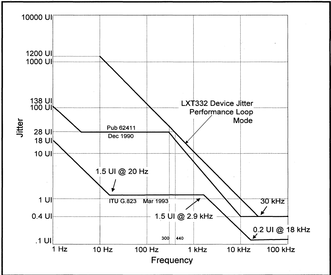
Figure 20: Typical Receiver Input Jitter Tolerance (Loop Mode)
