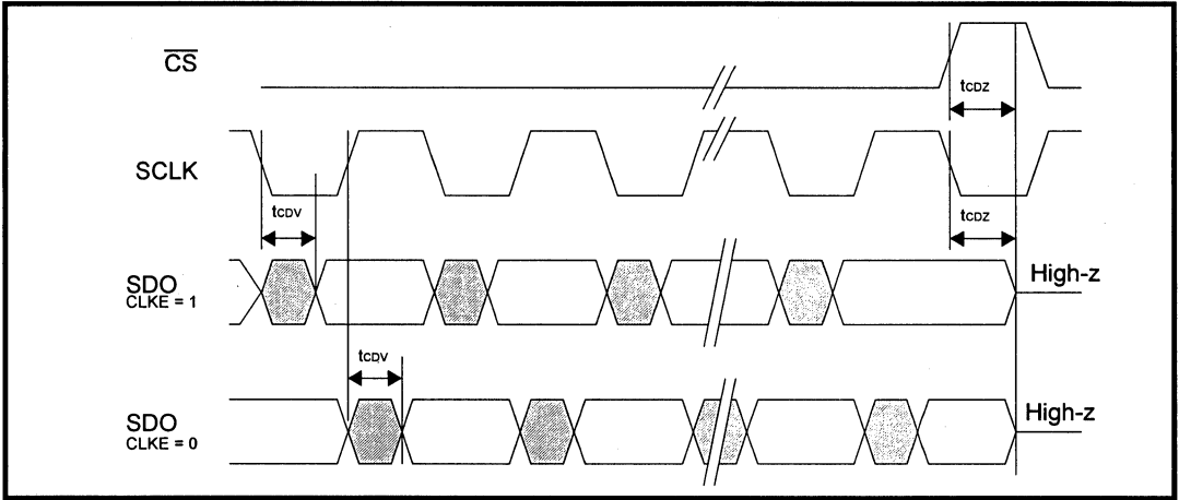
Figure 17: LXT332 Serial Data Output Timing Diagram
