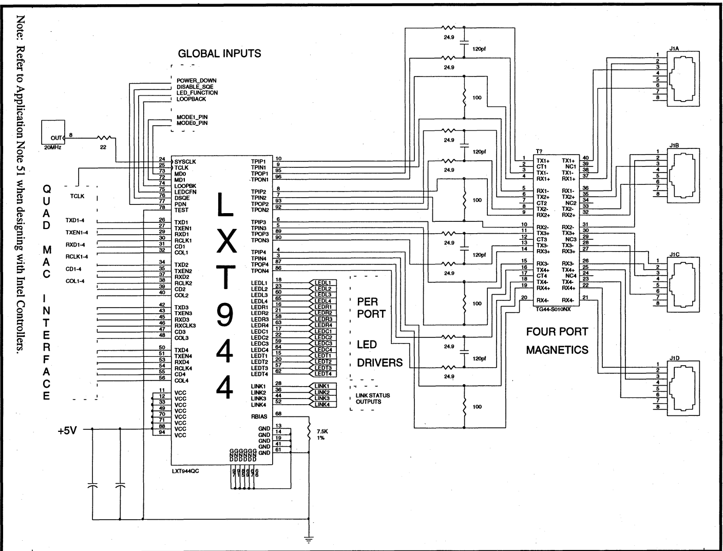
Figure 9: Single, 40-pin Octal Transformer Application
