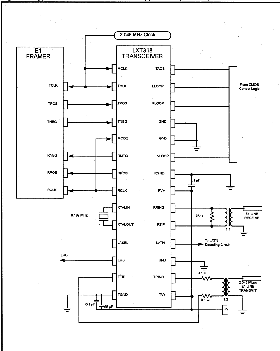
Figure 13: Typical LXT318 Hardware Mode Application (75 Ω Coax)
