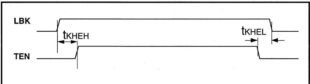
Figure 38: Mode 4 Loopback Timing
