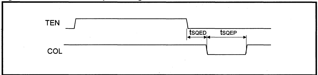
Figure 21: Mode 3 COL Output Timing
