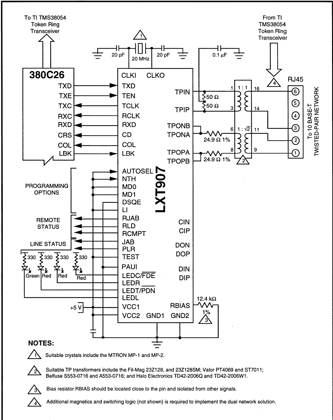
Figure 10: LXT907/380C26 Interface for Dual Network Support of 10BASE-T and Token Ring
