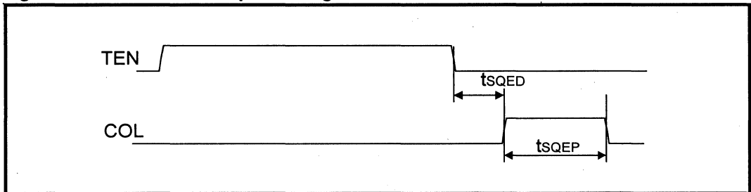
Figure 25: Mode 4 COL Output Timing
