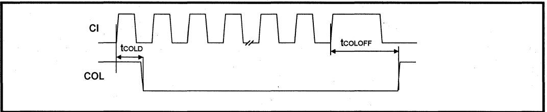
Figure 13: Mode 2 COL/CI Output Timing
