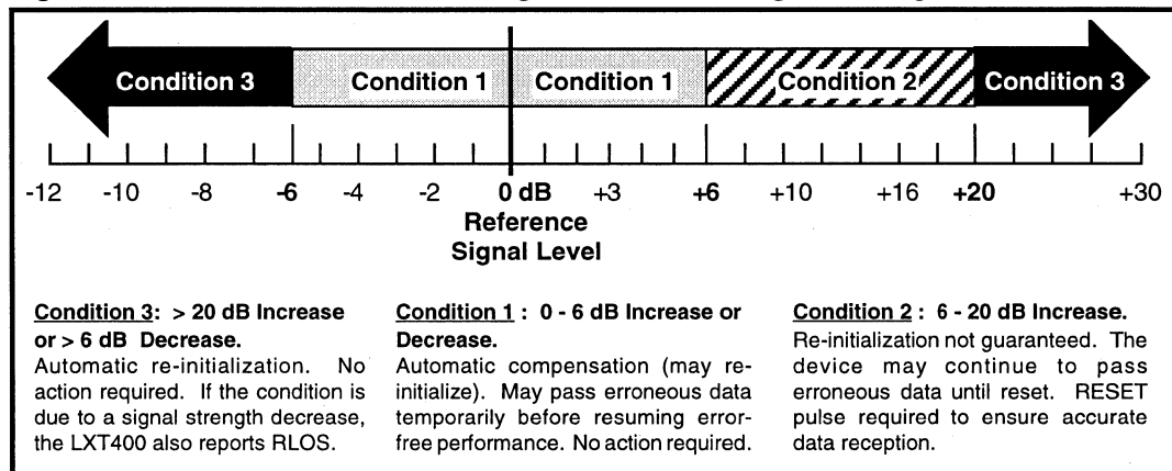
Figure 4: Conditions Based on Changes in Received Signal Strength
