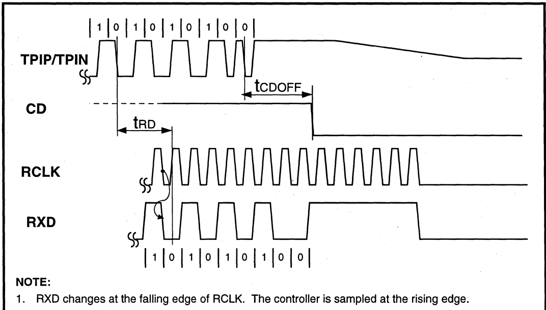
Figure 23: Mode 4 RCLK/End of Frame Timing
