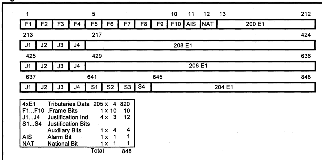
Figure 2: E2 Frame
