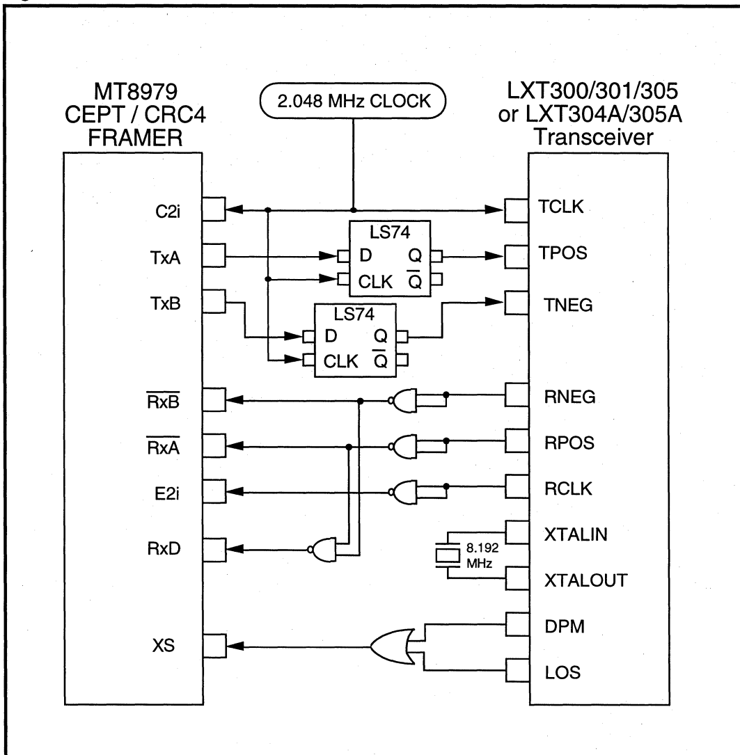
Figure 1: LXT300 Interface to MT8979 E1 CRC Framer
