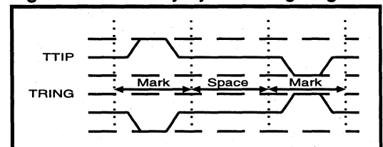
Figure 4: 50% Duty Cycle Coding Diagram
