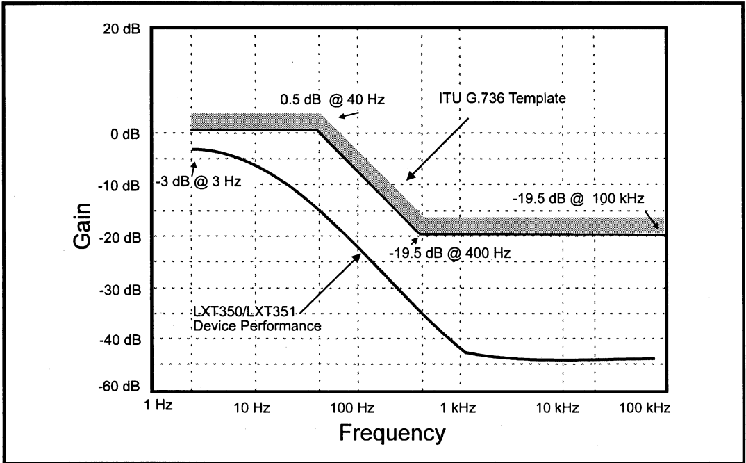
Figure 25: E1 Jitter Transfer Performance (Typical)
