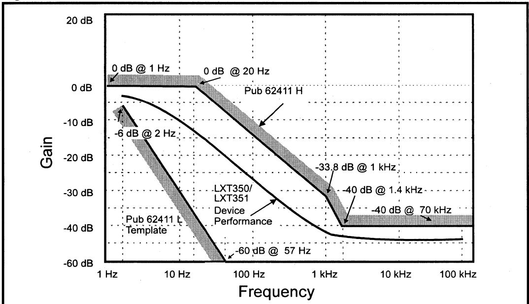
Figure 26: T1 Jitter Transfer Performance (Typical)
