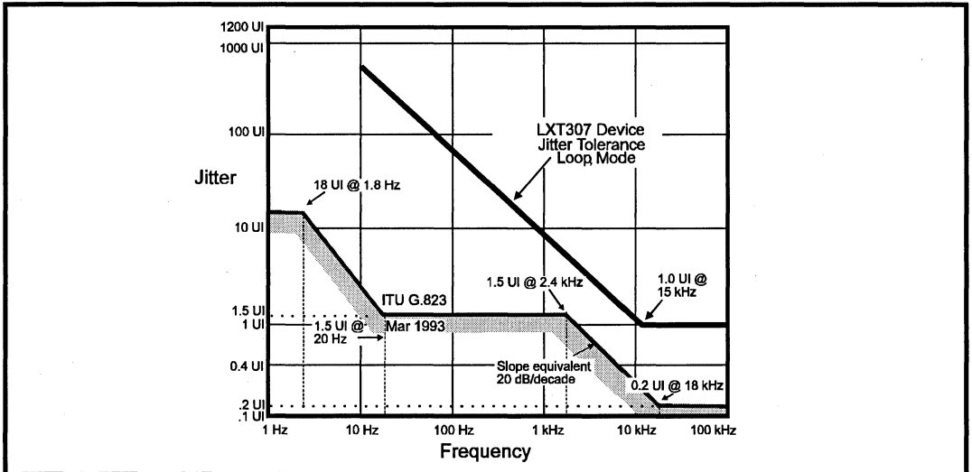
Figure 17: Typical Receiver Input Jitter Tolerance (Loop Mode)
