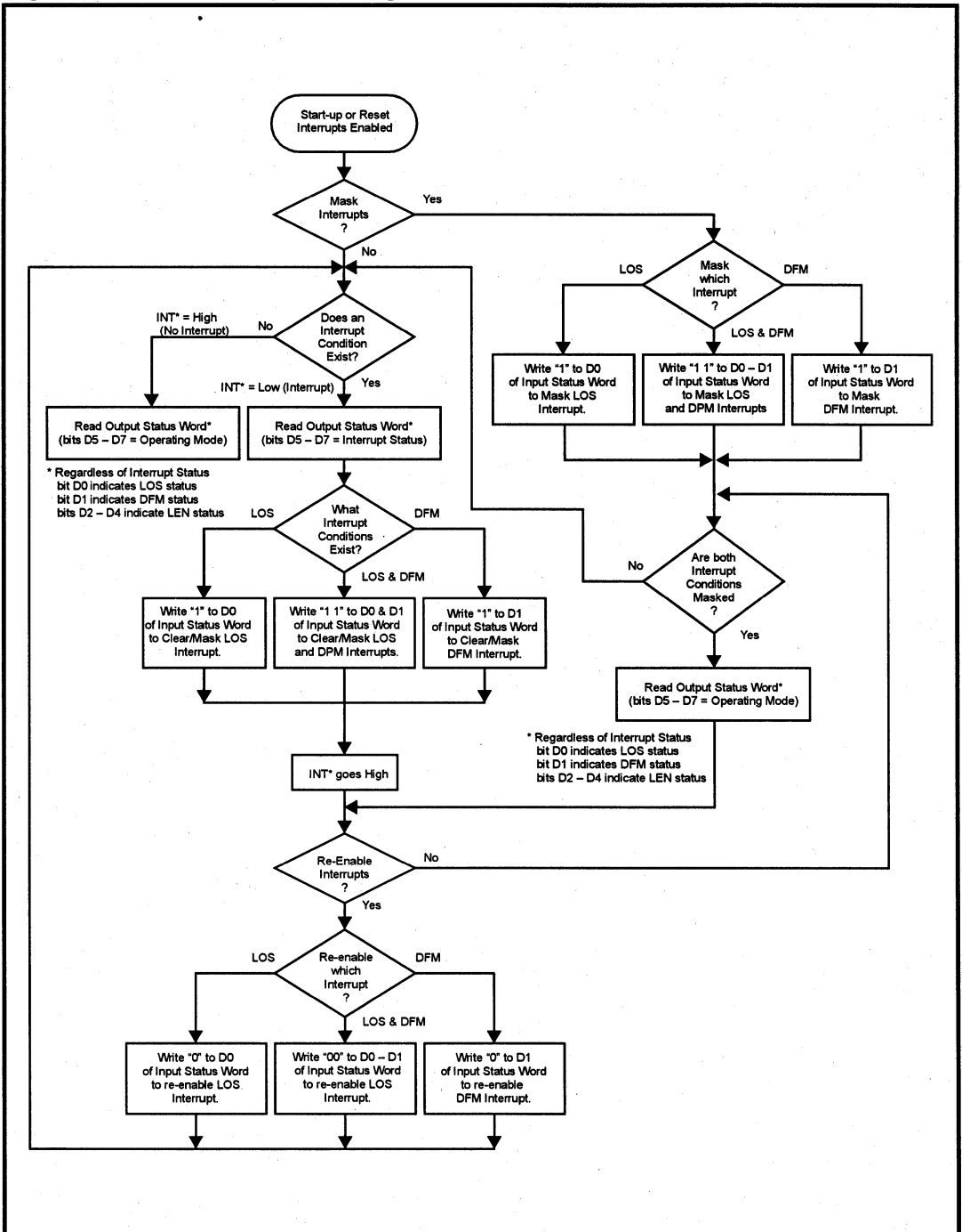
Figure 6: LX332 Interrupt Handling
