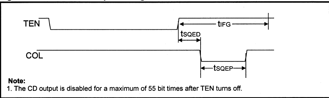
Figure 17: Mode 2 COL Output Timing
