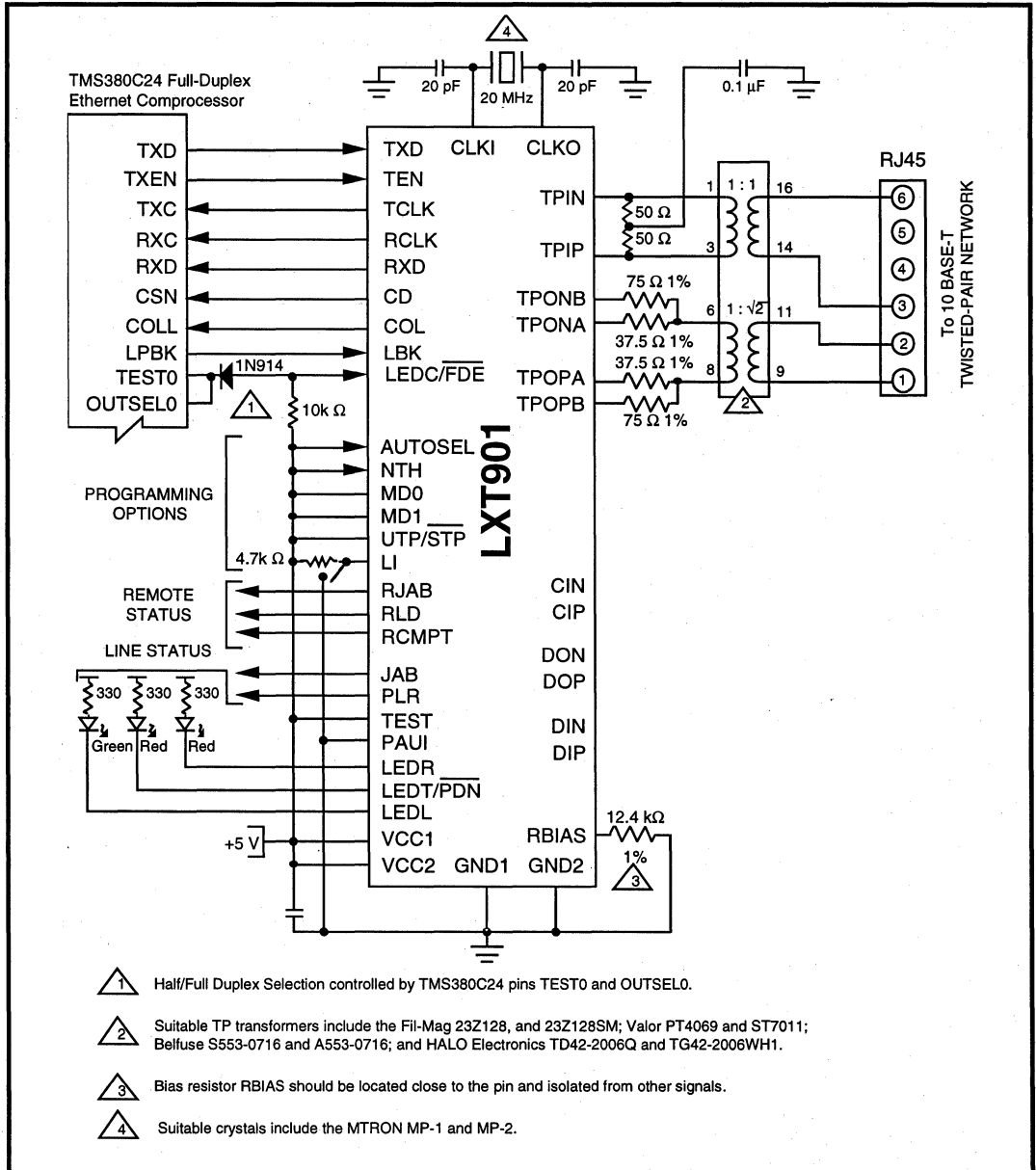
Figure 15: Full-Duplex Application
