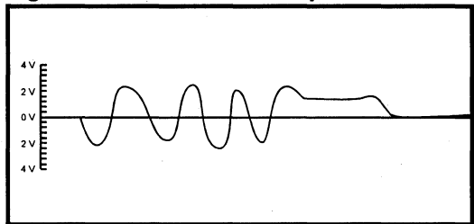
Figure 2: LXT944 TPO Output Waveform
