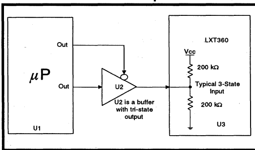
Figure 1: Typical Circuit for LXT360 Three-State Inputs
