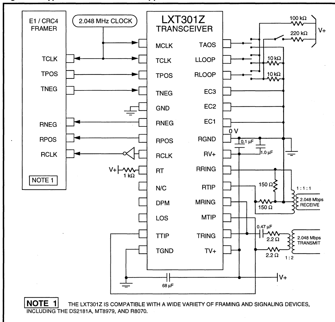
Figure 8: Typical LXT301Z 75 Ω E1 Application
