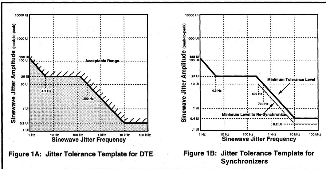
Figure 1: Input Jitter Tolerance Specified by AT&T Publication 62411
