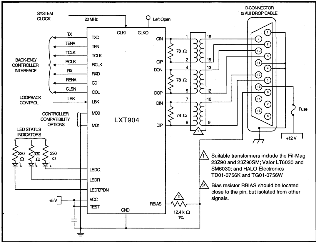
Figure 2: Typical LXT904 Application
