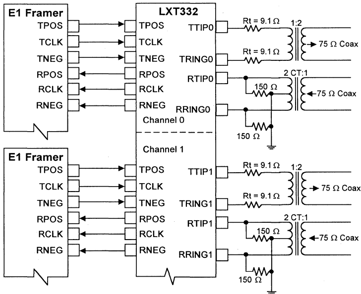
Figure 3B: LXT332 75 Ω E1 Line Interface
