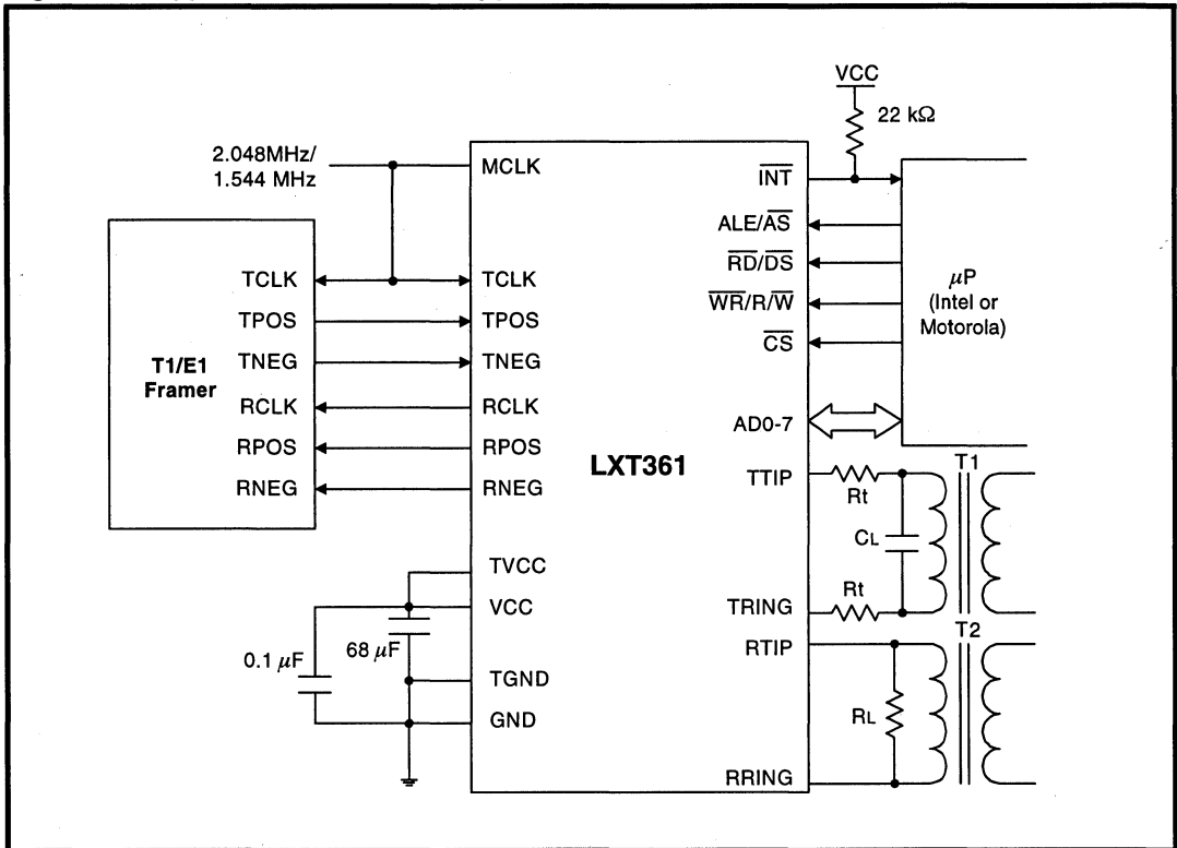
Figure 15: Typical T1/E1 LXT361 Application
