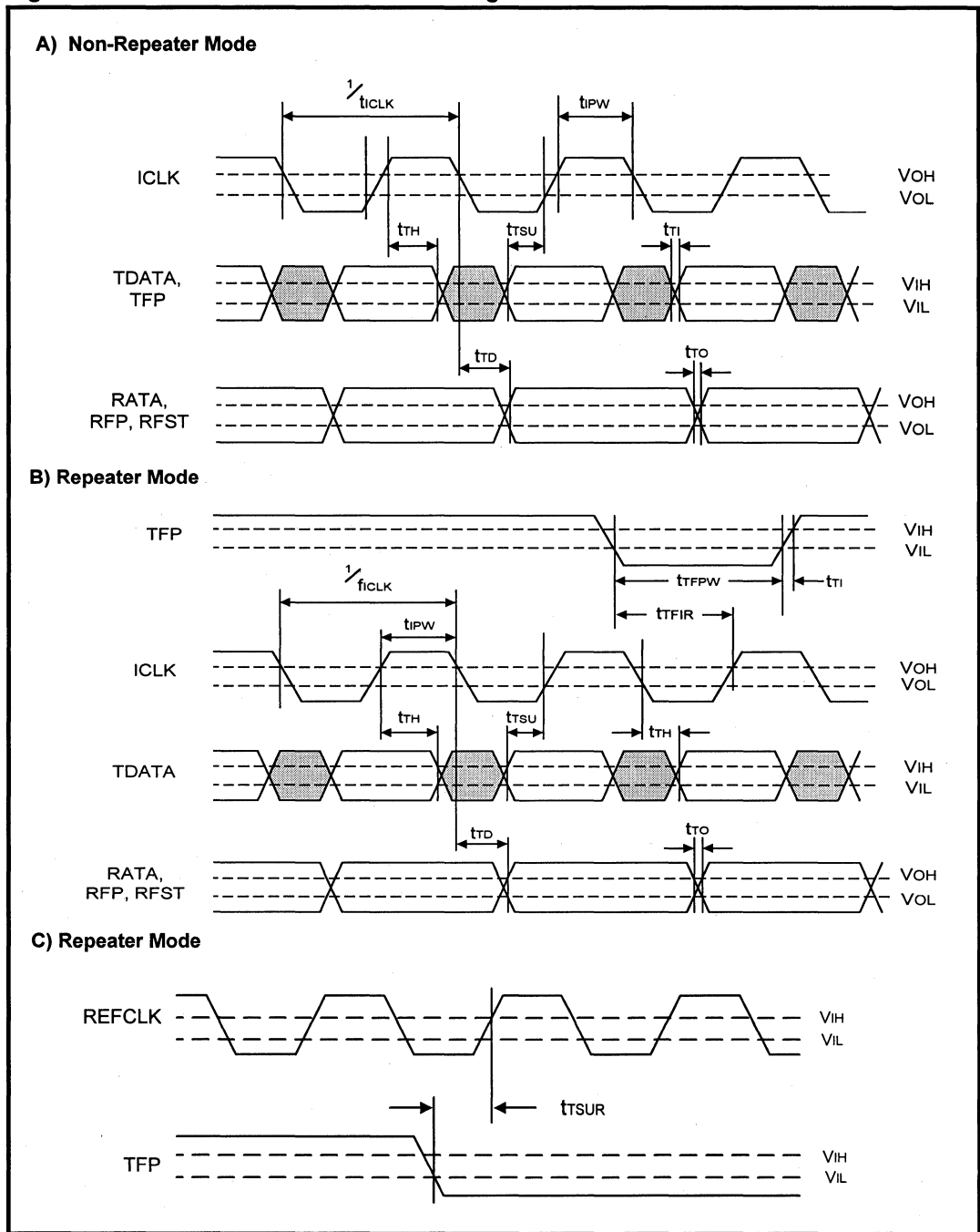
Figure 19: HDX/HDSL Data Interface Timing
