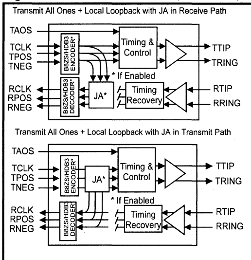
Figure 5: TAOS with LLOOP (JA Selected)
