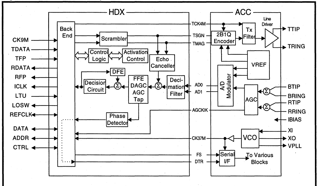
Figure 3: HDSL Data Pump Block Architecture
