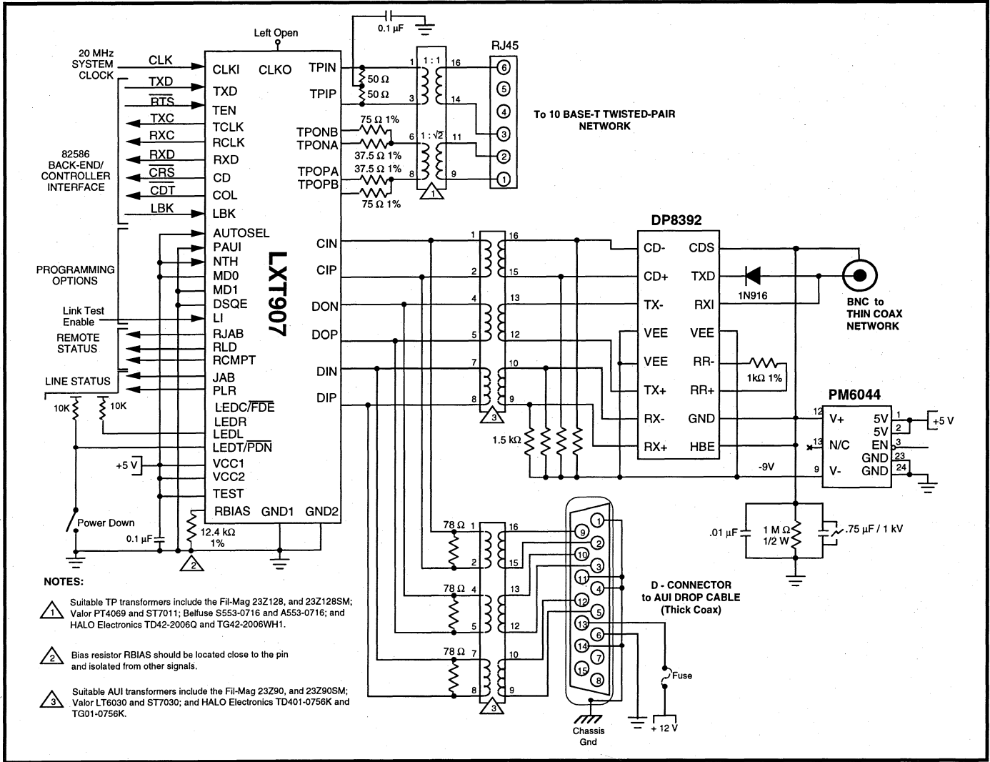
Figure 13: Three Media Application
