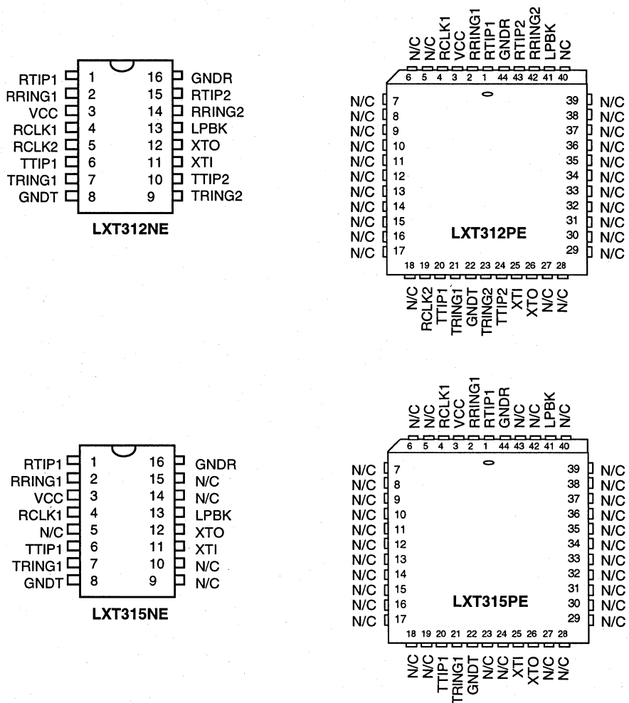
Figure 1: LXT312/315 Repeater/Transceiver Pin Assignments
