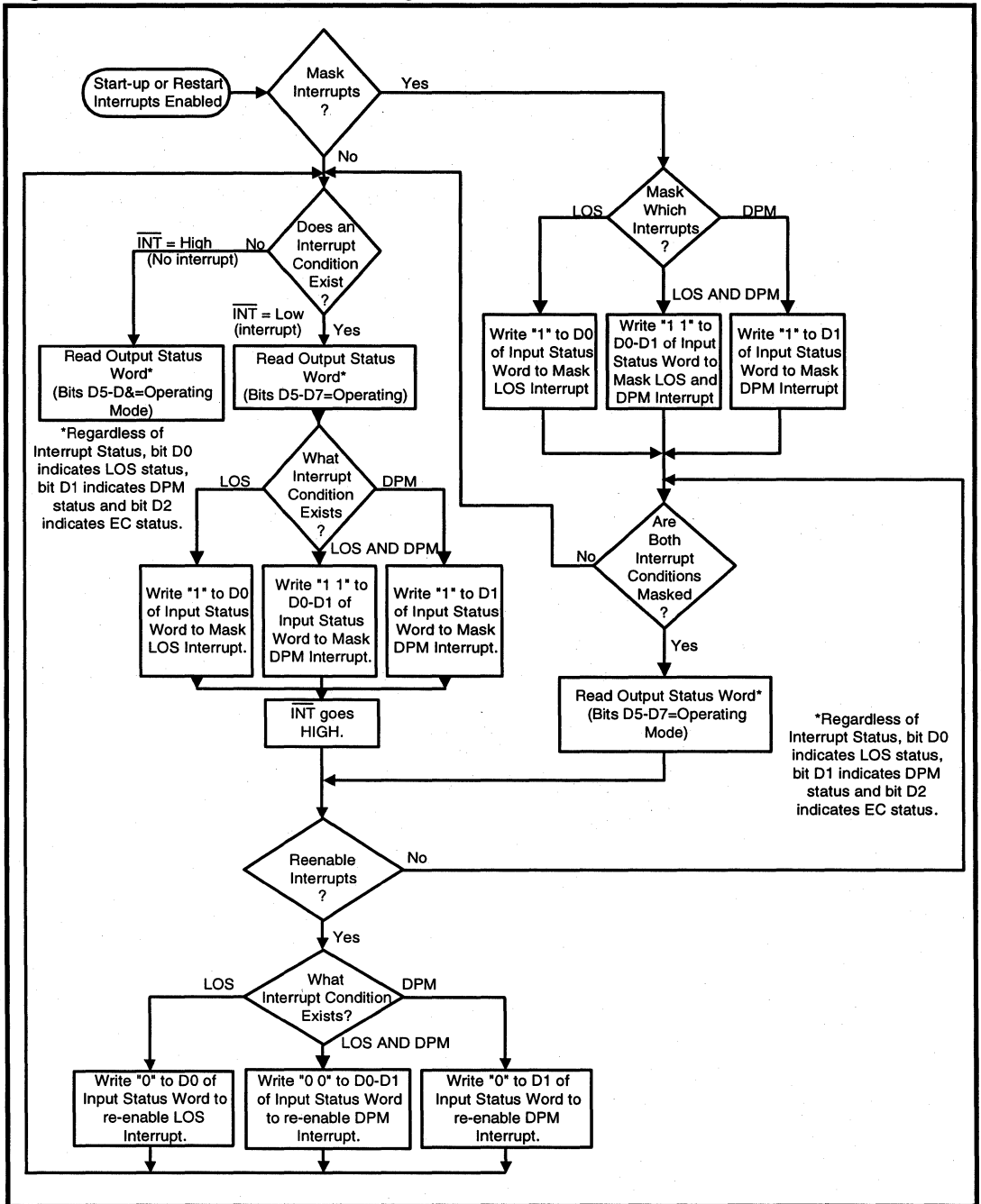
Figure 5: LXT307 Interrupt Handling
