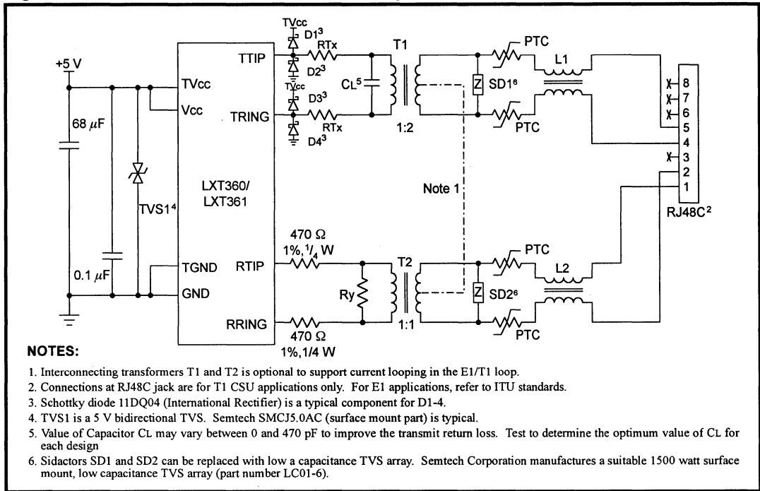
Figure 1: Enhanced Line Protection Circuitry
