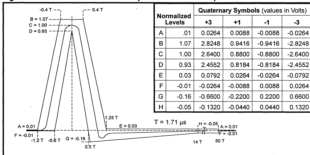
Figure 15: ACC Normalized Pulse Amplitude Transmit Template
