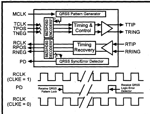
Figure 11: QRSS Mode
