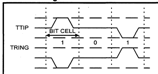
Figure 4: 50% Duty Cycle Coding Diagram
