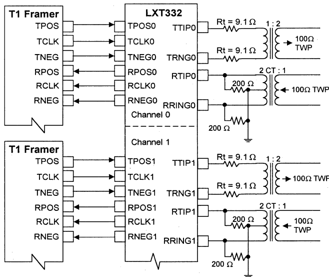
Figure 1B: LXT332 100 Ω T1 Line Interface
