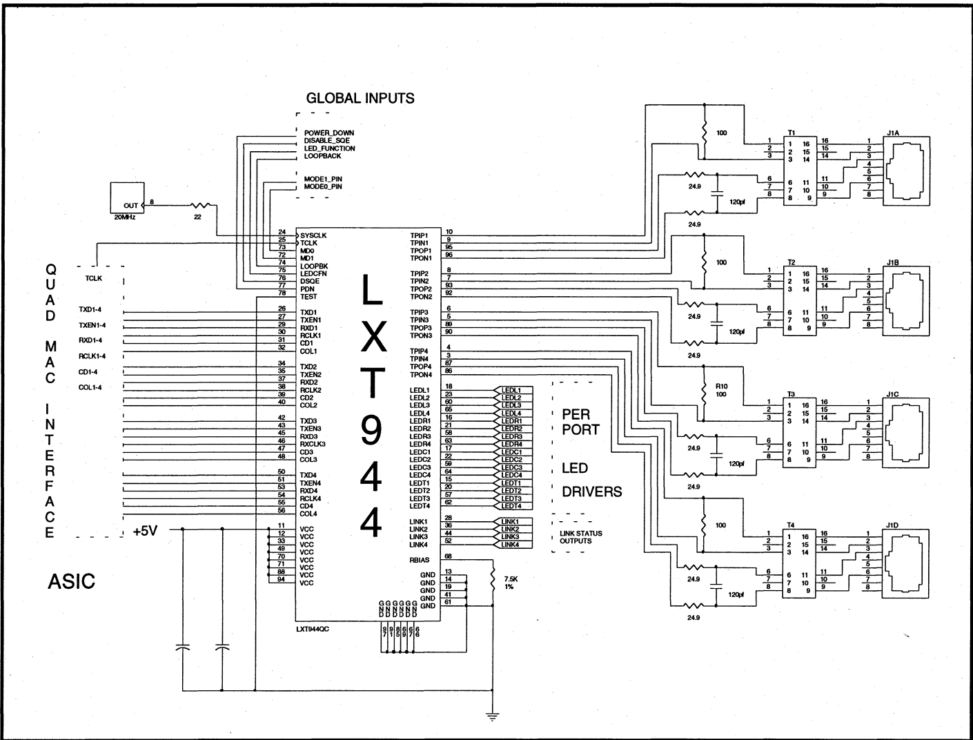
Figure 7: Simple Receiver/Transmit on Each Port Application
