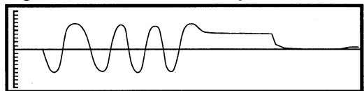
Figure 2: LXT907 TPO Output Waveform
