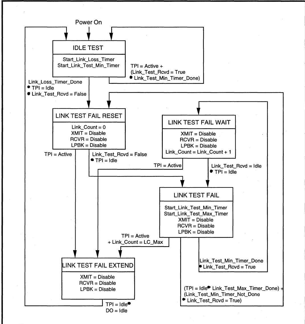
Figure 6: Link Integrity Test Function
