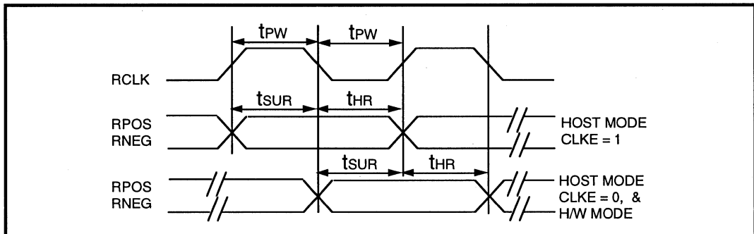
Figure 8: LXT304A Receive Clock Timing Diagram
