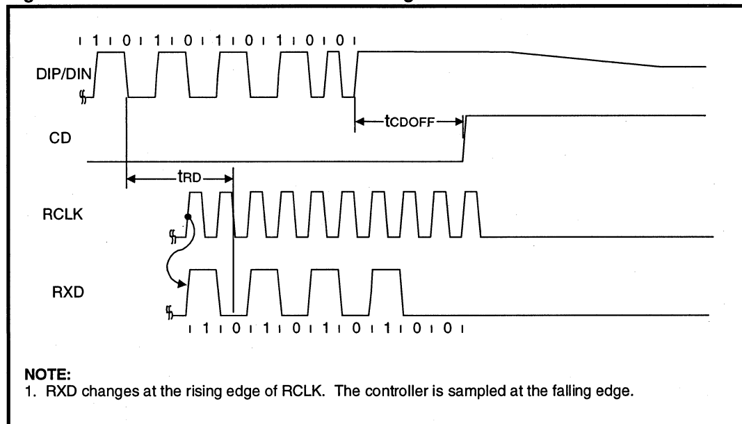
Figure 10: Mode 2 RCLK/End-of-Frame Timing
