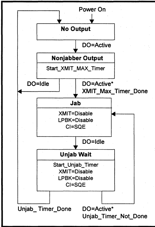
Figure 3: LXT944 Jabber Control Function
