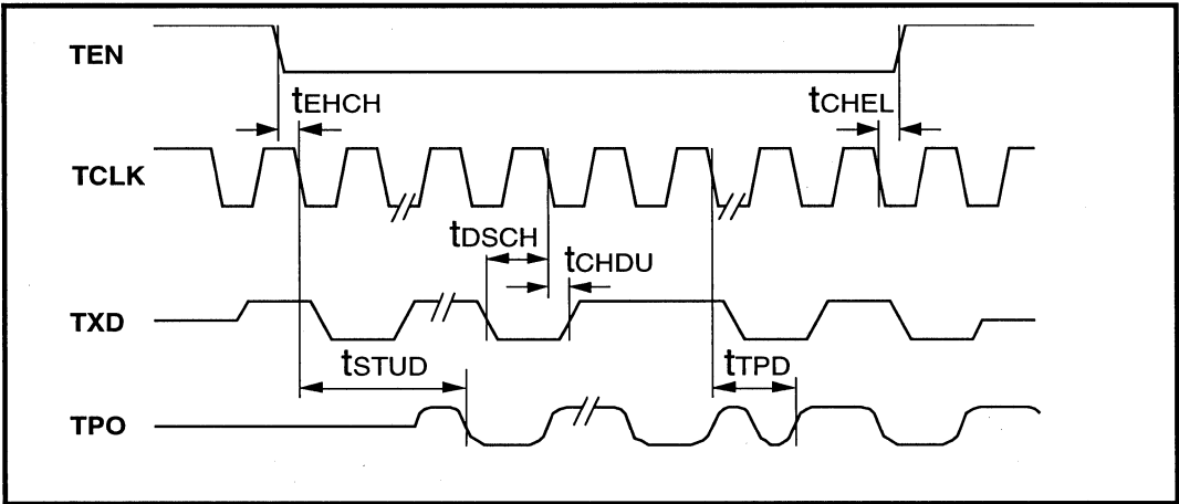
Figure 24: Mode 2 Collision Detect Timing
