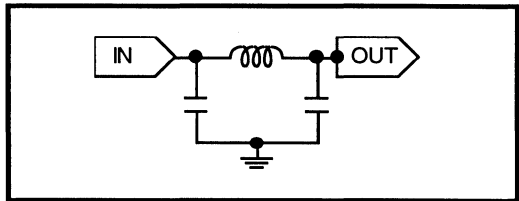
Figure 9: Receive Filter Diagram
