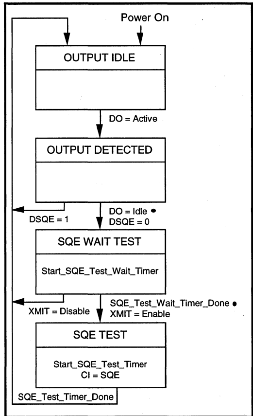
Figure 4: SQE Function
