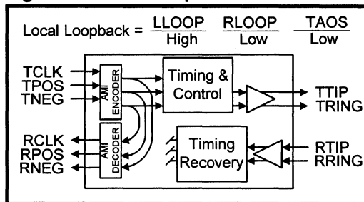
Figure 8: Local Loopback
