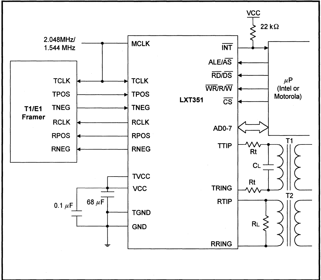
Figure 15: Typical T1/E1 LXT351 Application
