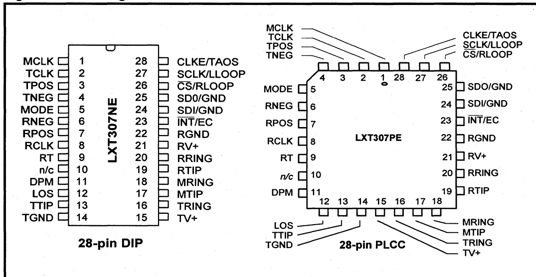
Figure 1: Pin Assignments
