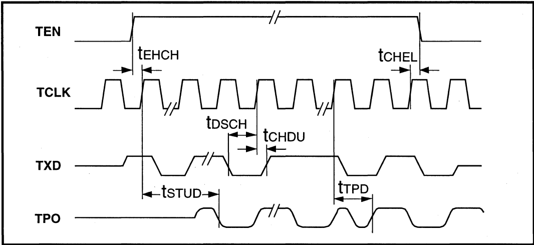
Figure 18: Mode 1 Collision Detect Timing
