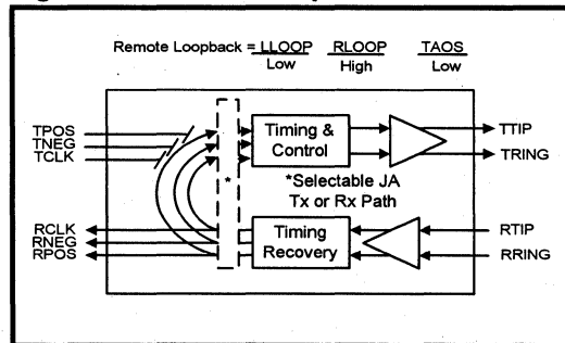
Figure 9: Remote Loopback
