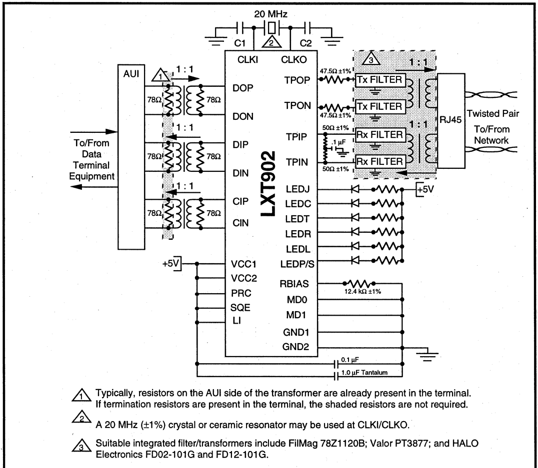
Figure 7: LXT902 External MAU Application Diagram
