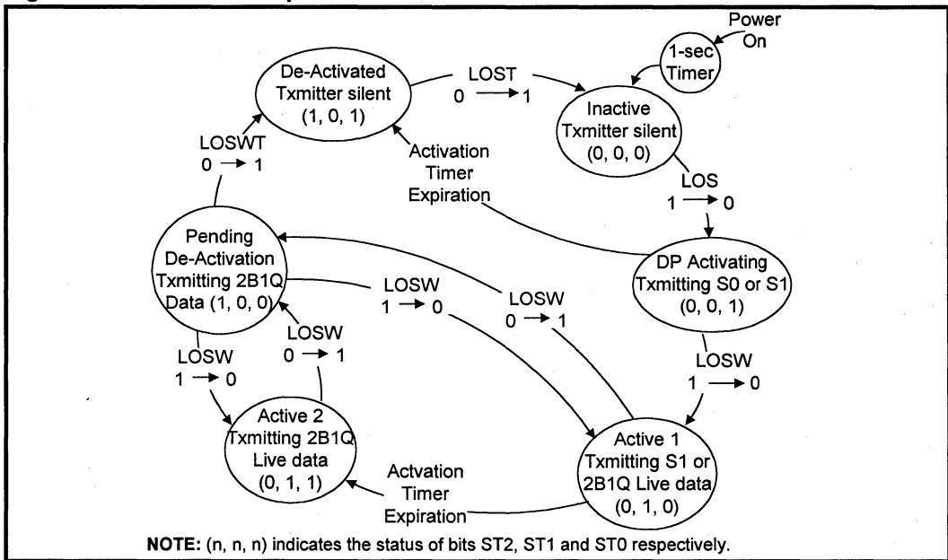
Figure 7: LTU Data Pump Activation State Machine
