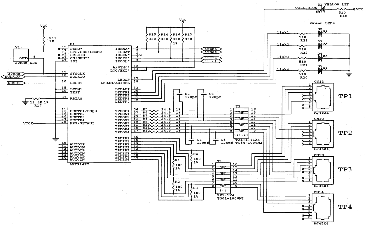
Figure 6: 8-Port Application Schematic, LED Mode 1 with AUISEL = MAU (Sheet 1 of 2)
