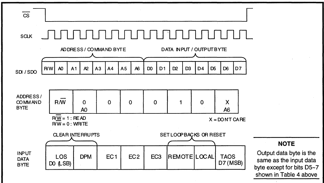
Figure 3: LXT305A Serial Interface Data Structure
