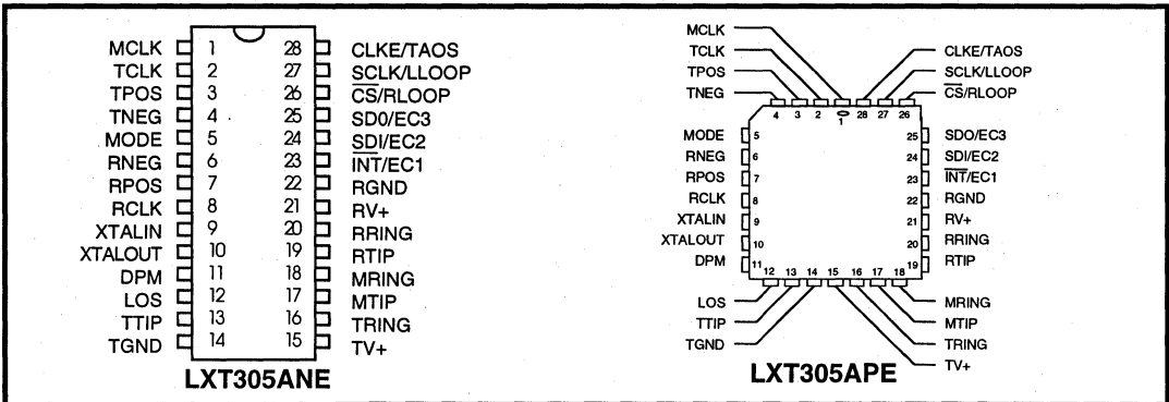
Figure 1: Pin Assignments
