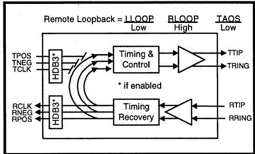
Figure 7: Remote Loopback
