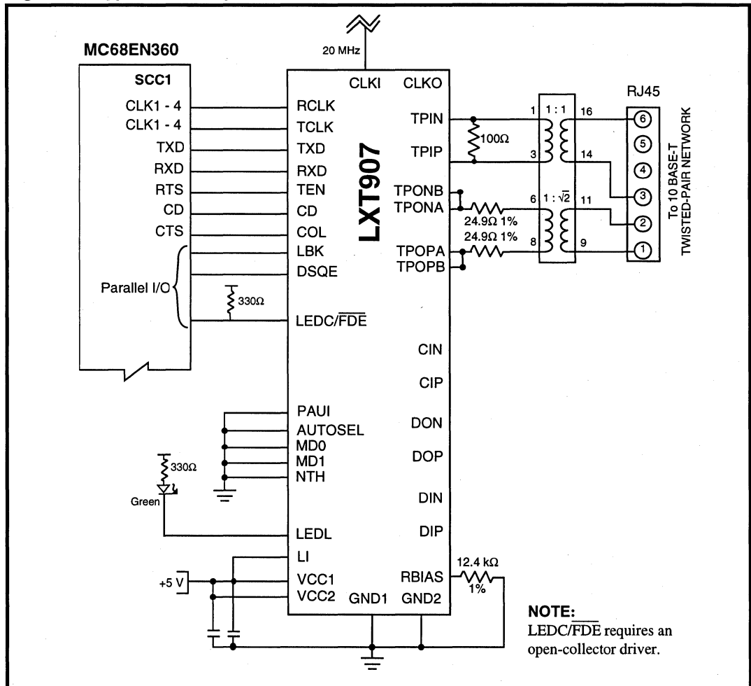
Figure 1: Typical Full Duplex 10BASE-T Connection
