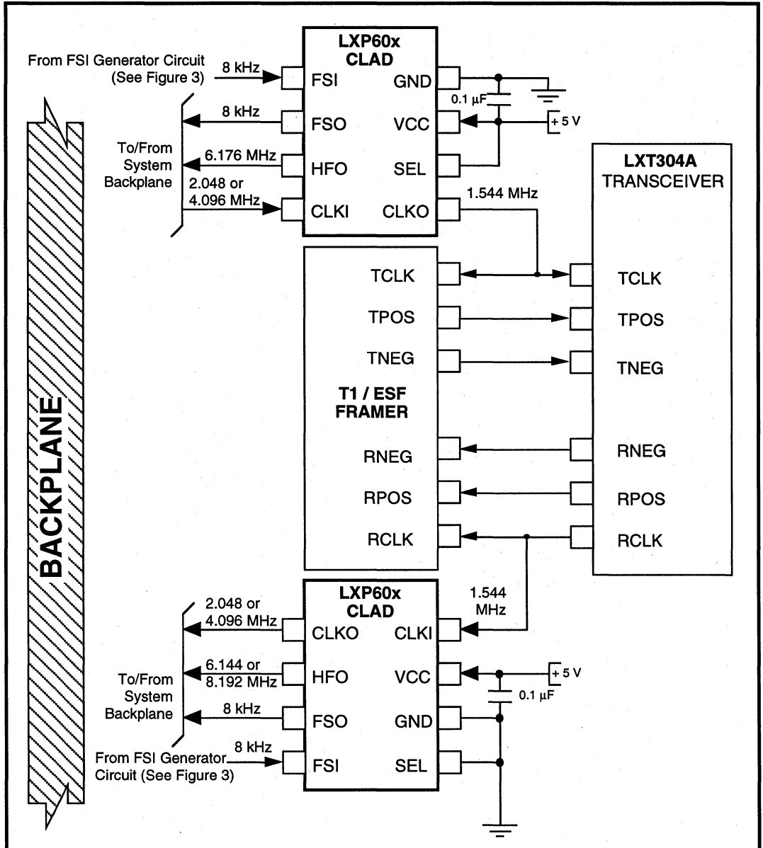
Figure 2: Typical CLAD Application Circuit
