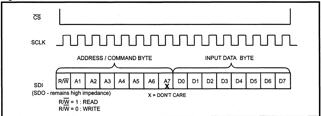
Figure 12: LXT360 Serial Interface Data Structure
