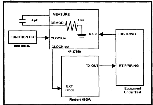
Figure 2: Conformance Test Configuration
