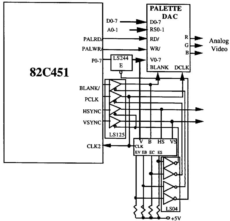
Block Diagram – Inmos Palette DAC (MSG176/178)
