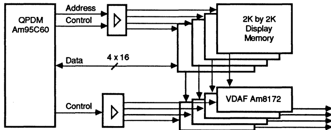
Figure 3.1-1 Block Diagram of a 4-Plane 2K by 2K Display Memory System
