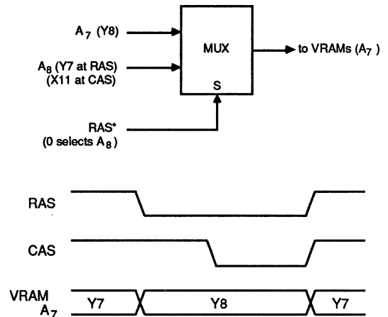
Figure 3.3-4 Logic Diagram
