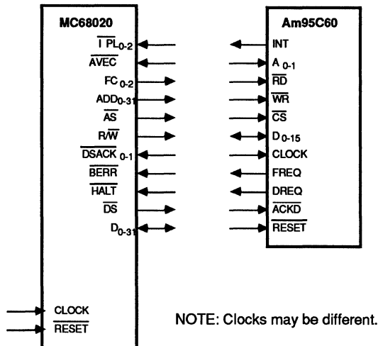
Figure 2.3-5 QPDM to 68020 Interface Signals
